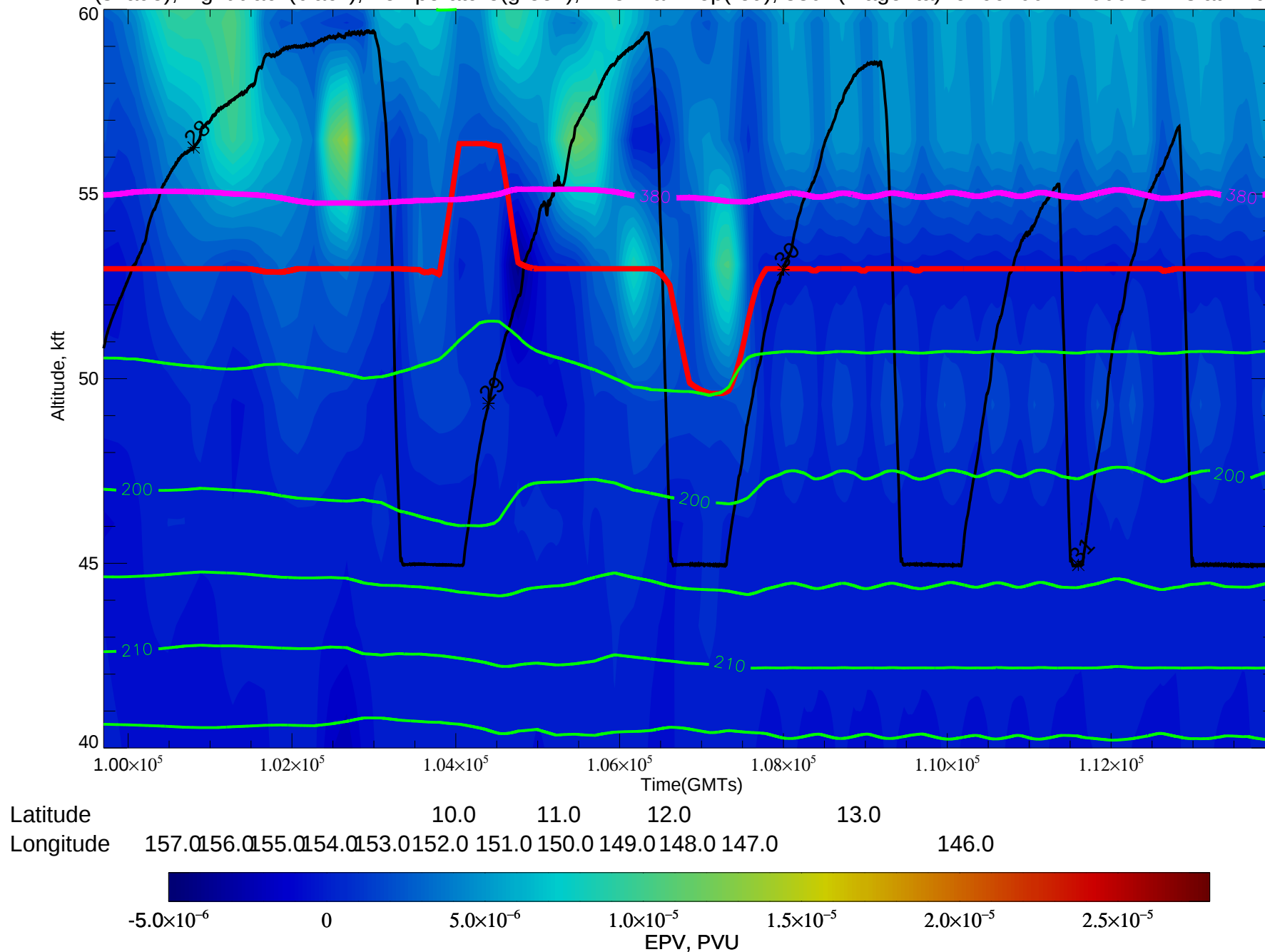
EPV(shade), flight track(black), Temperature(green), Thermal Trop(red), 380K(magenta) for 99700-114000 GMTs at 14031206
