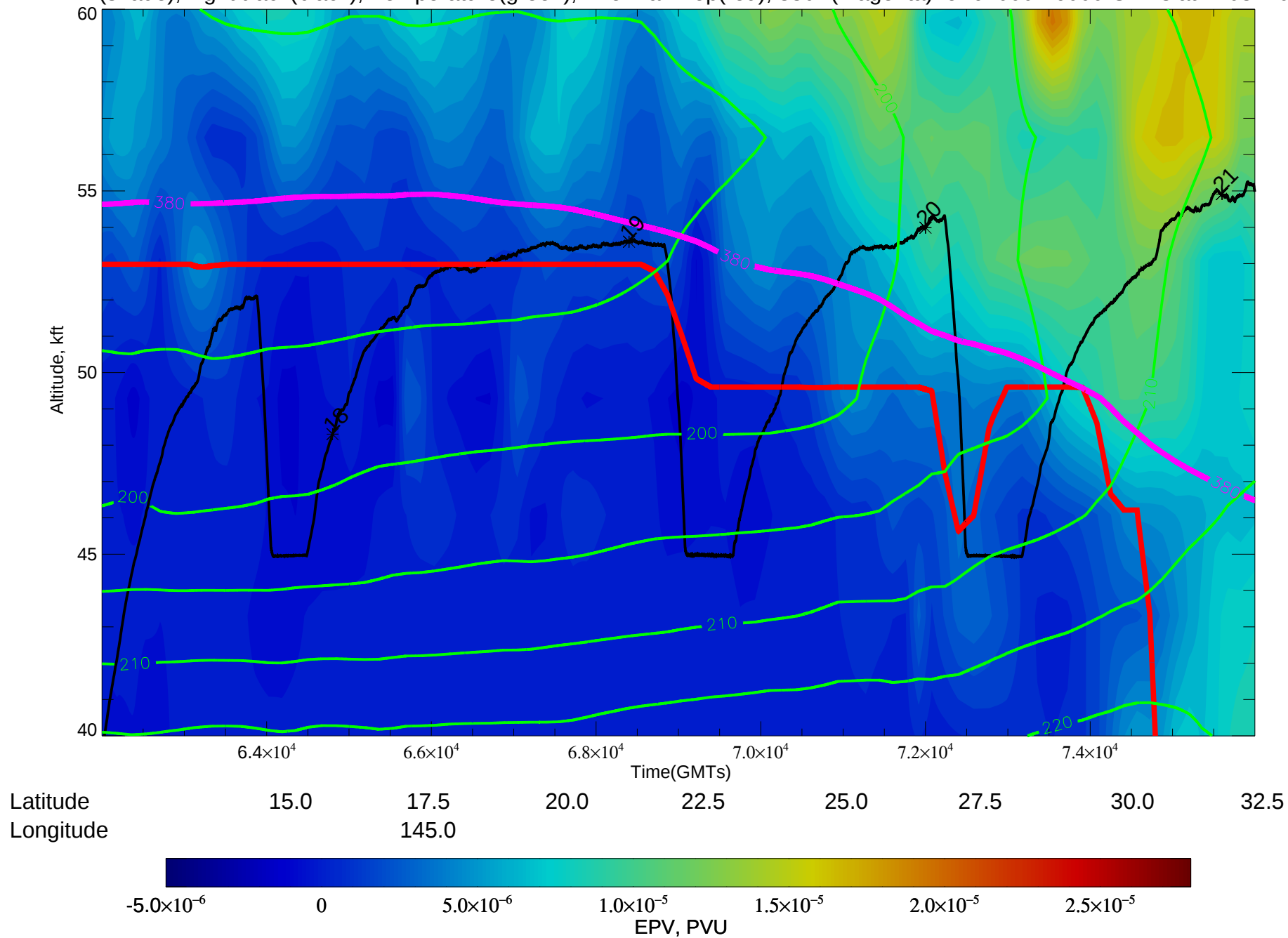
EPV(shade), flight track(black), Temperature(green), Thermal Trop(red), 380K(magenta) for 62000-76000 GMTs at 14031200
