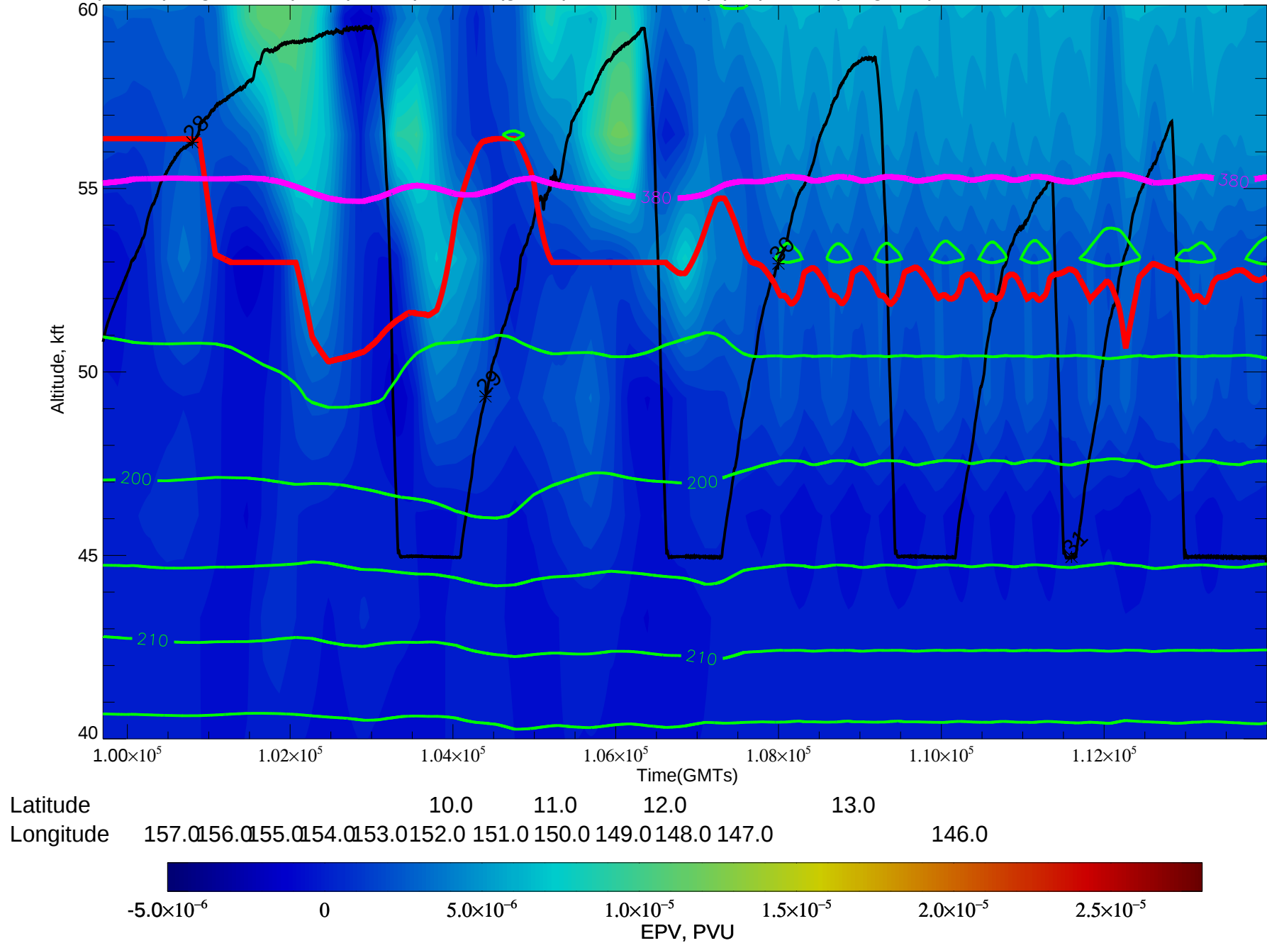
EPV(shade), flight track(black), Temperature(green), Thermal Trop(red), 380K(magenta) for 99700-114000 GMTs at 14031212
