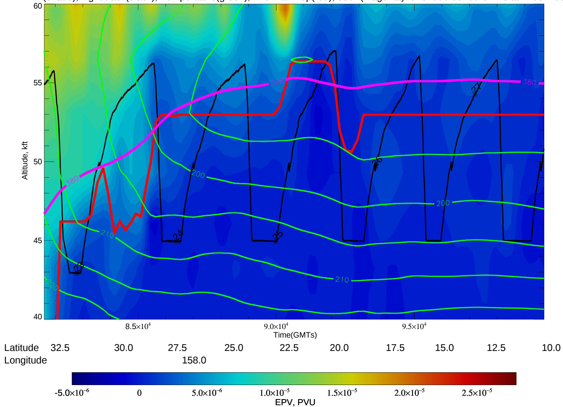
EPV(shade), flight track(black), Temperature(green), Thermal Trop(red), 380K(magenta) for 81600-99700 GMTs at 14031206
