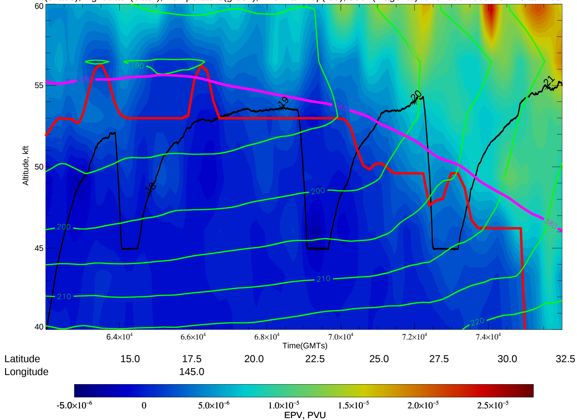
EPV(shade), flight track(black), Temperature(green), Thermal Trop(red), 380K(magenta) for 62000-76000 GMTs at 14031118
