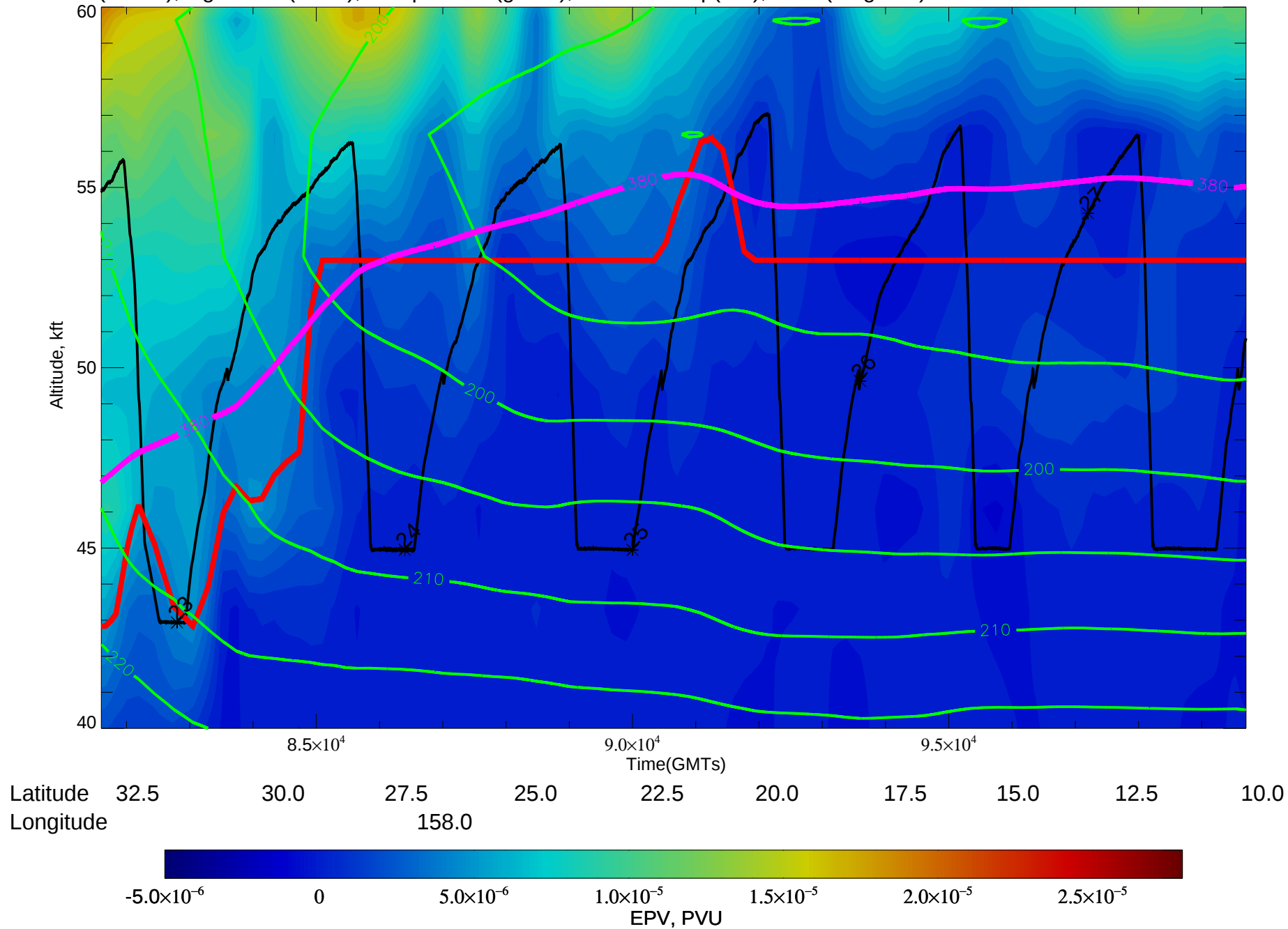
EPV(shade), flight track(black), Temperature(green), Thermal Trop(red), 380K(magenta) for 81600-99700 GMTs at 14031200
