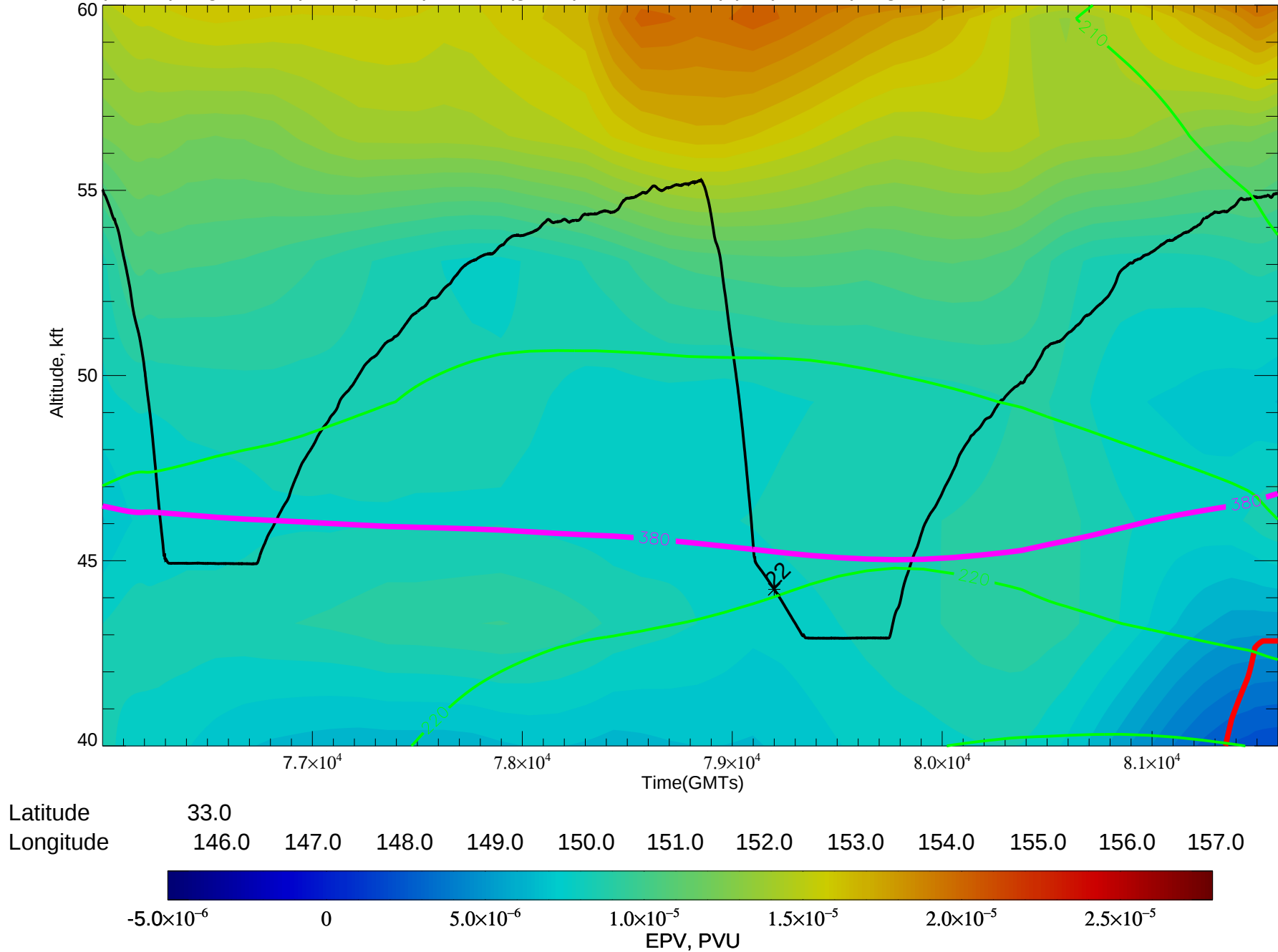
EPV(shade), flight track(black), Temperature(green), Thermal Trop(red), 380K(magenta) for 76000-81600 GMTs at 14031200
