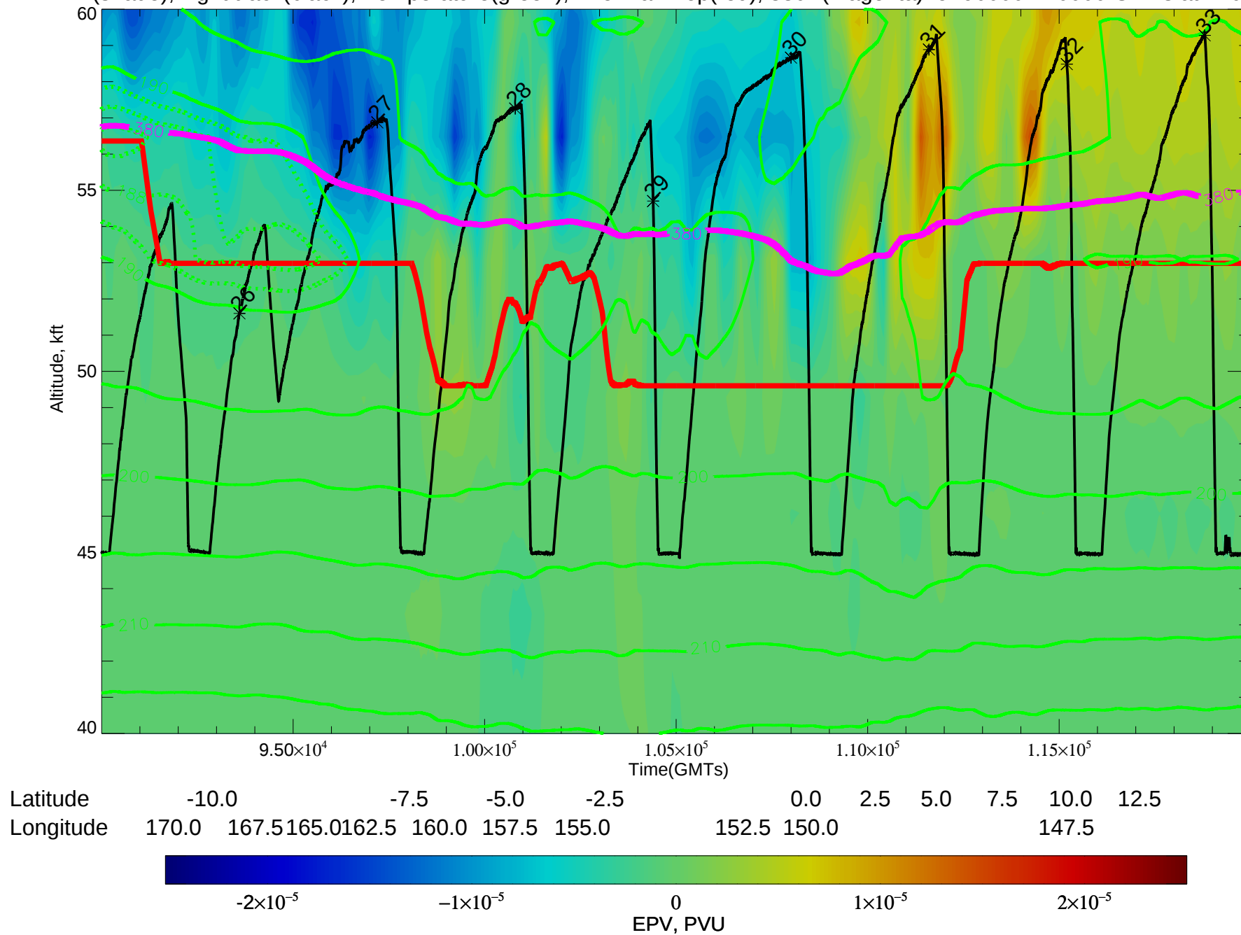
EPV(shade), flight track(black), Temperature(green), Thermal Trop(red), 380K(magenta) for 90000-120000 GMTs at 14031006
