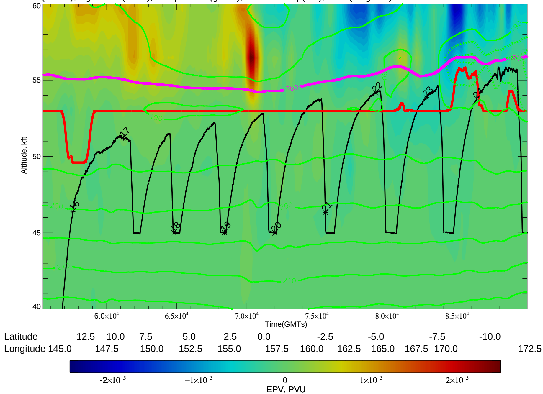
EPV(shade), flight track(black), Temperature(green), Thermal Trop(red), 380K(magenta) for 55000-90000 GMTs at 14030918
