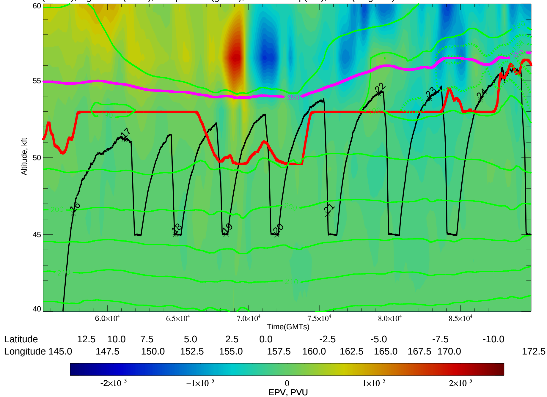
EPV(shade), flight track(black), Temperature(green), Thermal Trop(red), 380K(magenta) for 55000-90000 GMTs at 14031000
