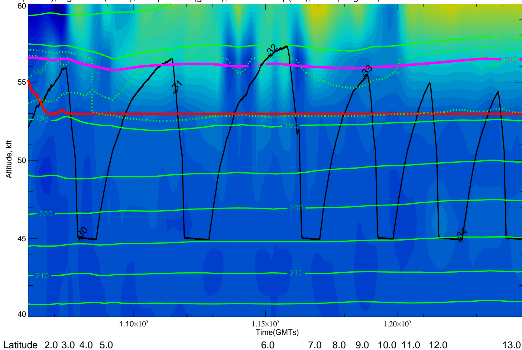
EPV(shade), flight track(black), Temperature(green), Thermal Trop(red), 380K(magenta) for 106000-125000 GMTs at 14021312
