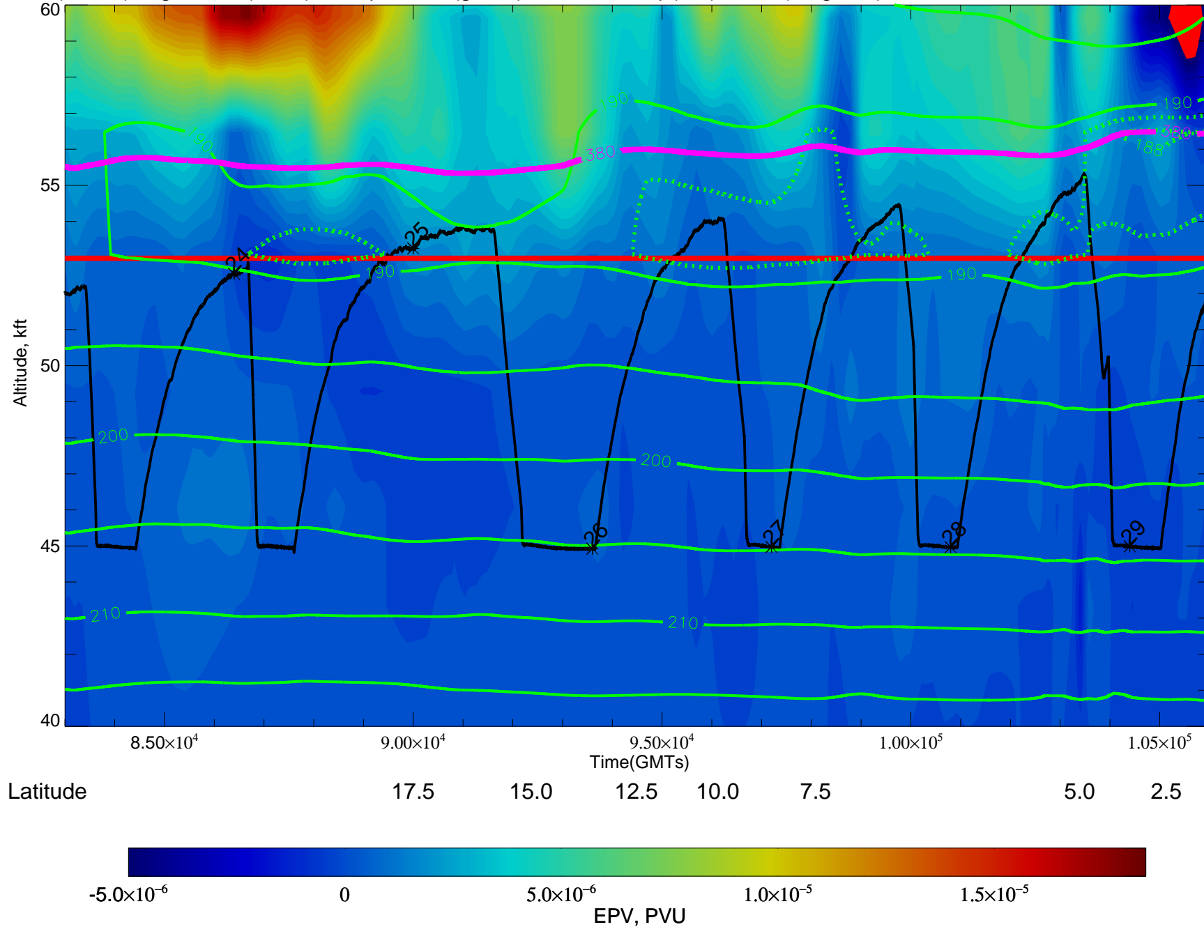
EPV(shade), flight track(black), Temperature(green), Thermal Trop(red), 380K(magenta) for 83000-106000 GMTs at 14021306
