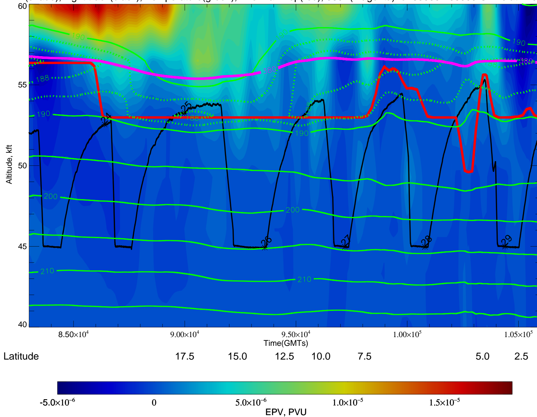
EPV(shade), flight track(black), Temperature(green), Thermal Trop(red), 380K(magenta) for 83000-106000 GMTs at 14021218
