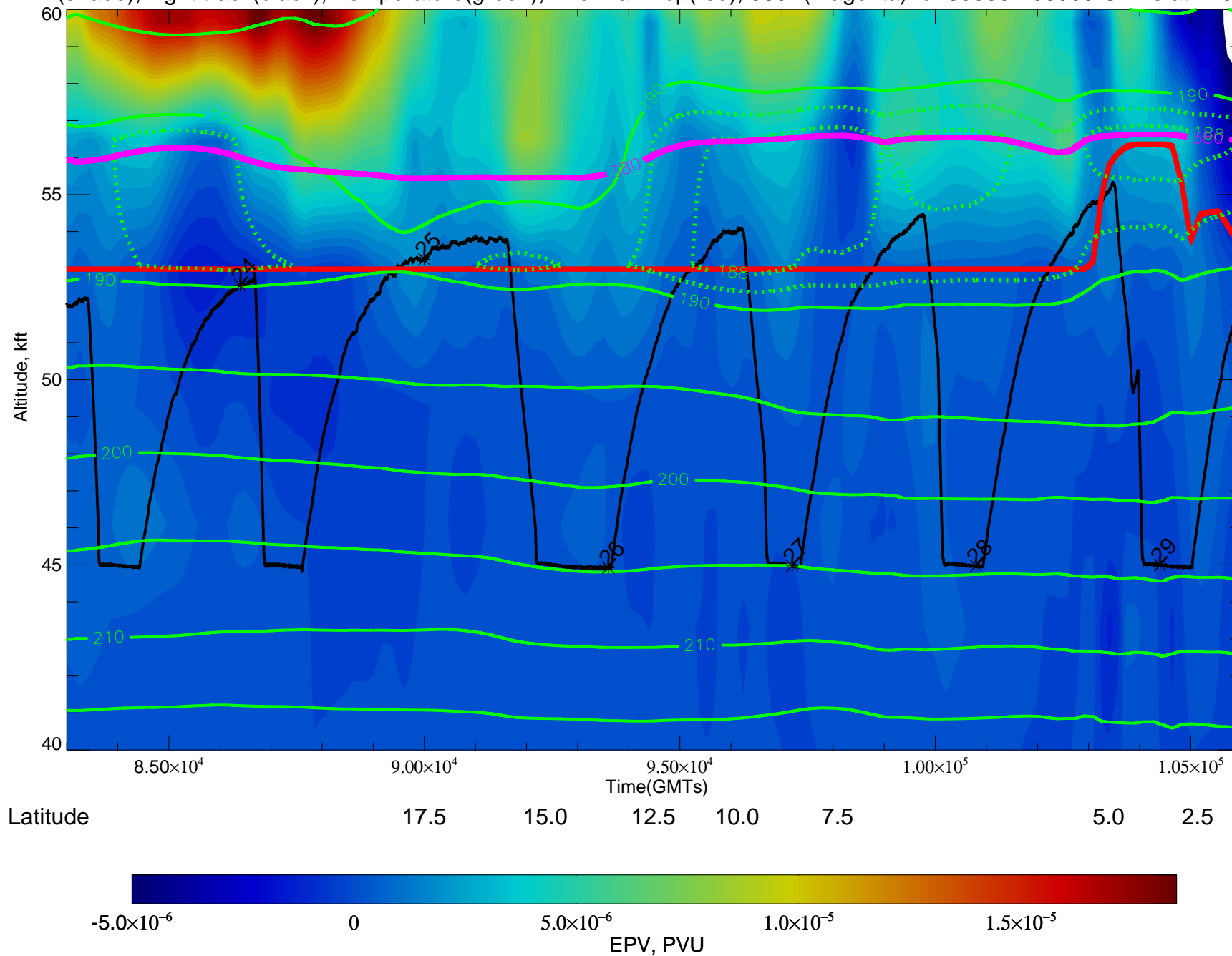
EPV(shade), flight track(black), Temperature(green), Thermal Trop(red), 380K(magenta) for 83000-106000 GMTs at 14021300
