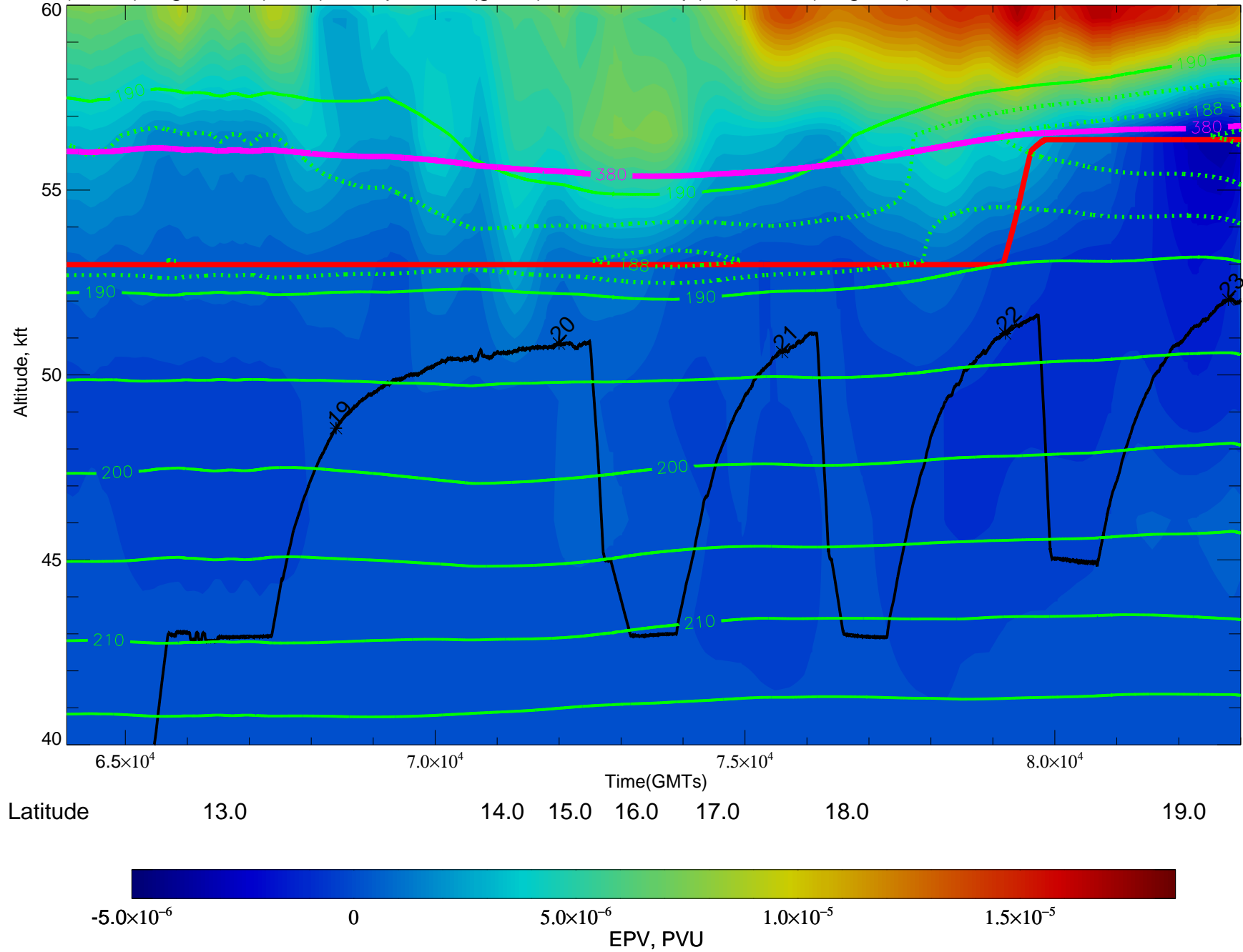
EPV(shade), flight track(black), Temperature(green), Thermal Trop(red), 380K(magenta) for 64000-83000 GMTs at 14021218
