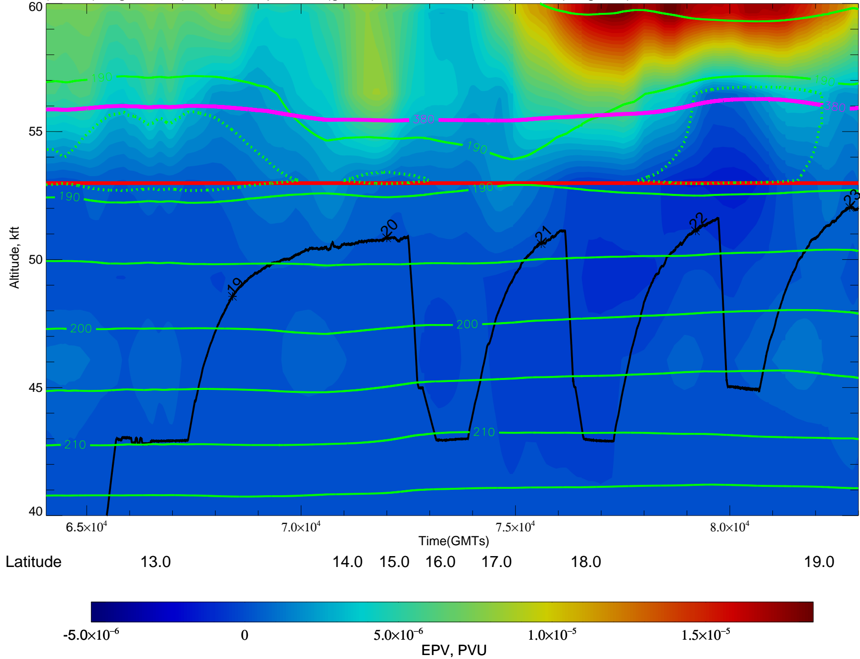
EPV(shade), flight track(black), Temperature(green), Thermal Trop(red), 380K(magenta) for 64000-83000 GMTs at 14021300
