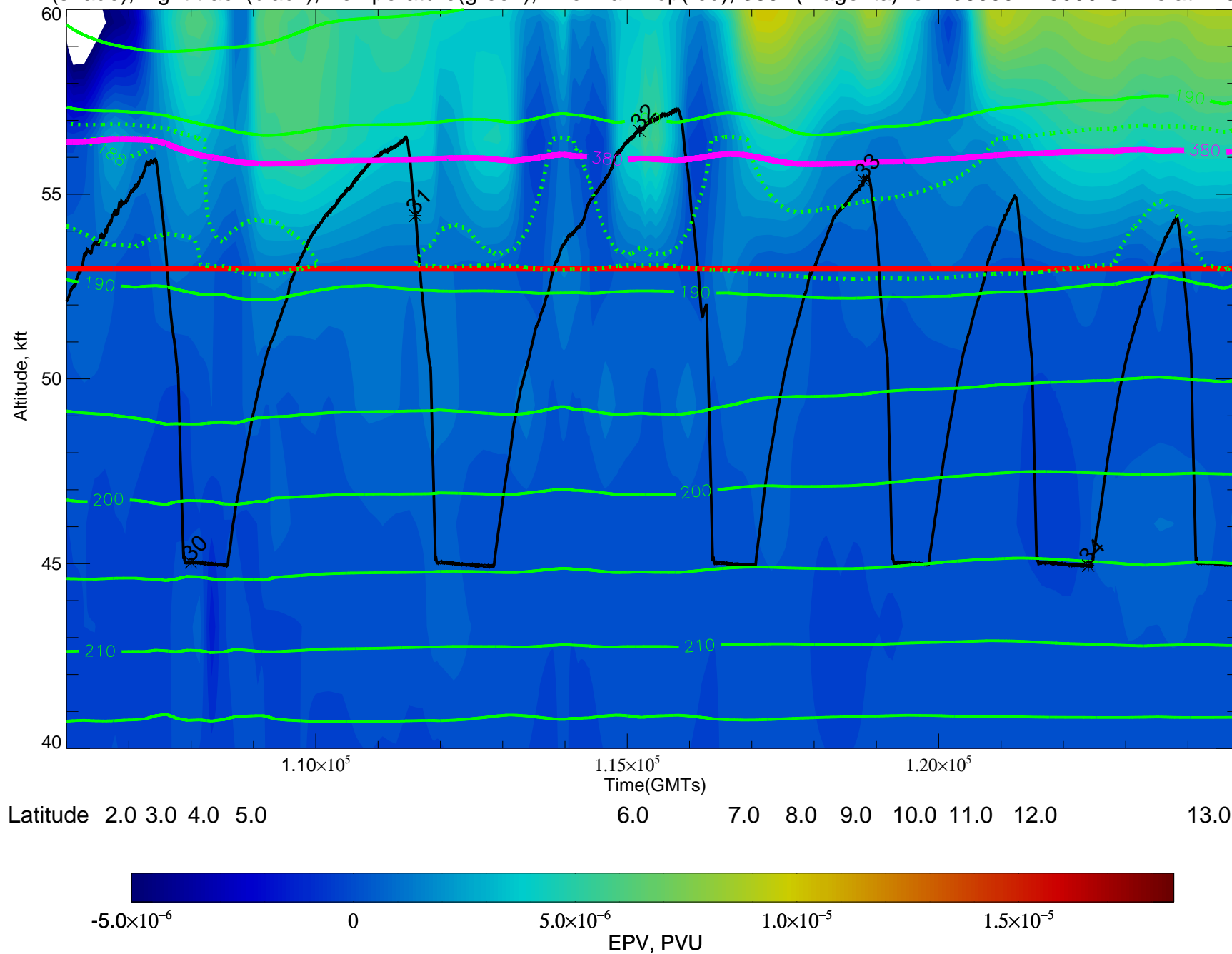
EPV(shade), flight track(black), Temperature(green), Thermal Trop(red), 380K(magenta) for 106000-125000 GMTs at 14021306
