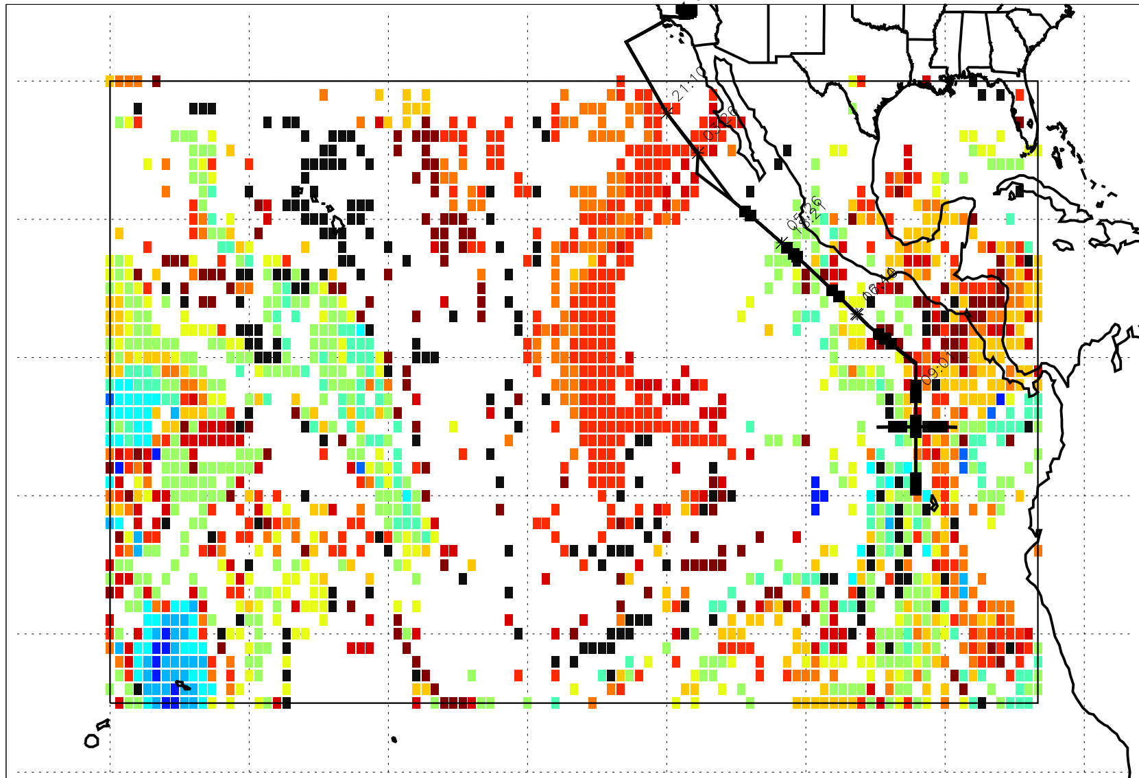
Fig. 1: End locations of trajectories influenced by convection in the past 14 days. Time since most recent convection in color.
