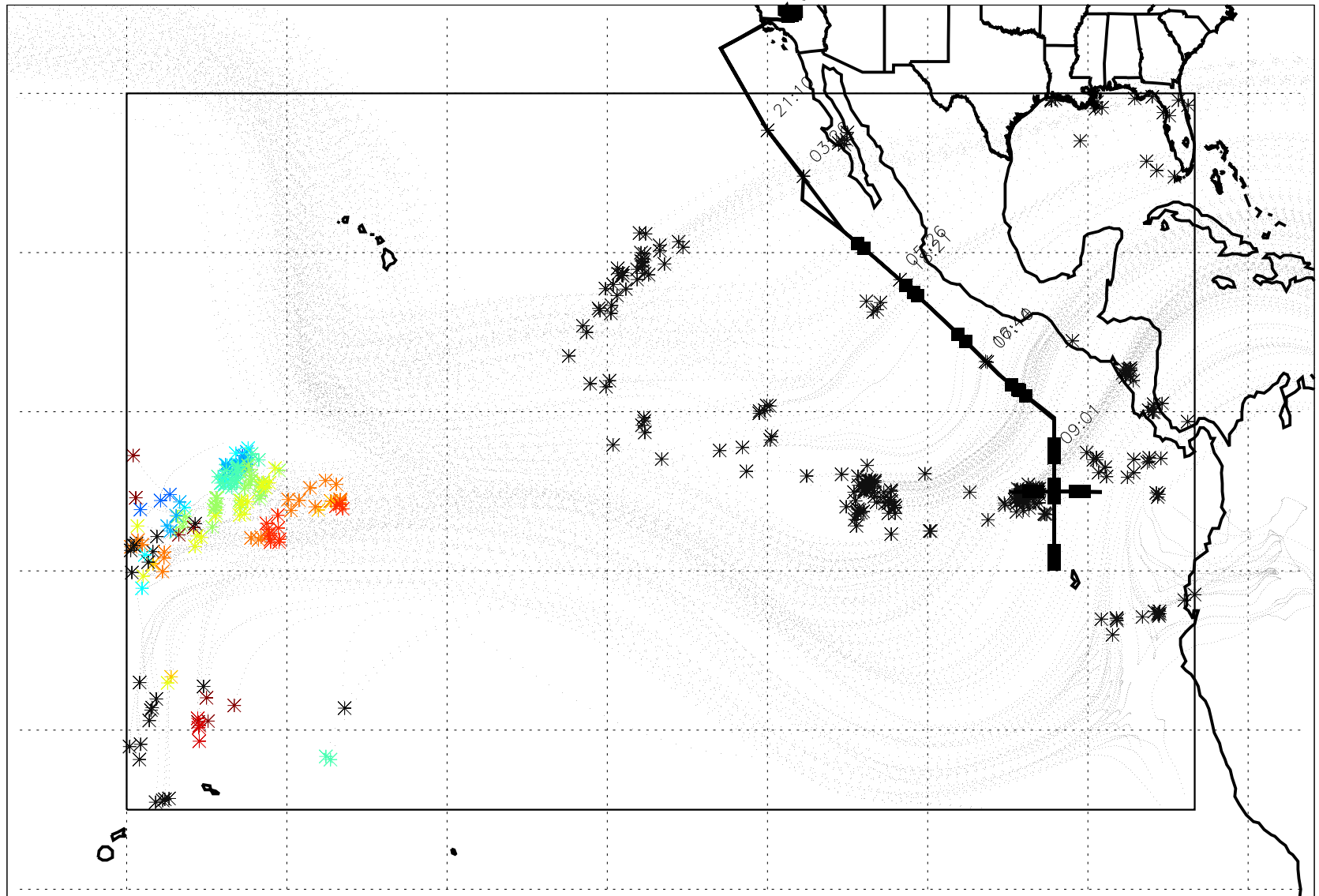
Fig. 3: Locations of most recent convection that occurs within or near boxed region (same as X in Fig. 2).
