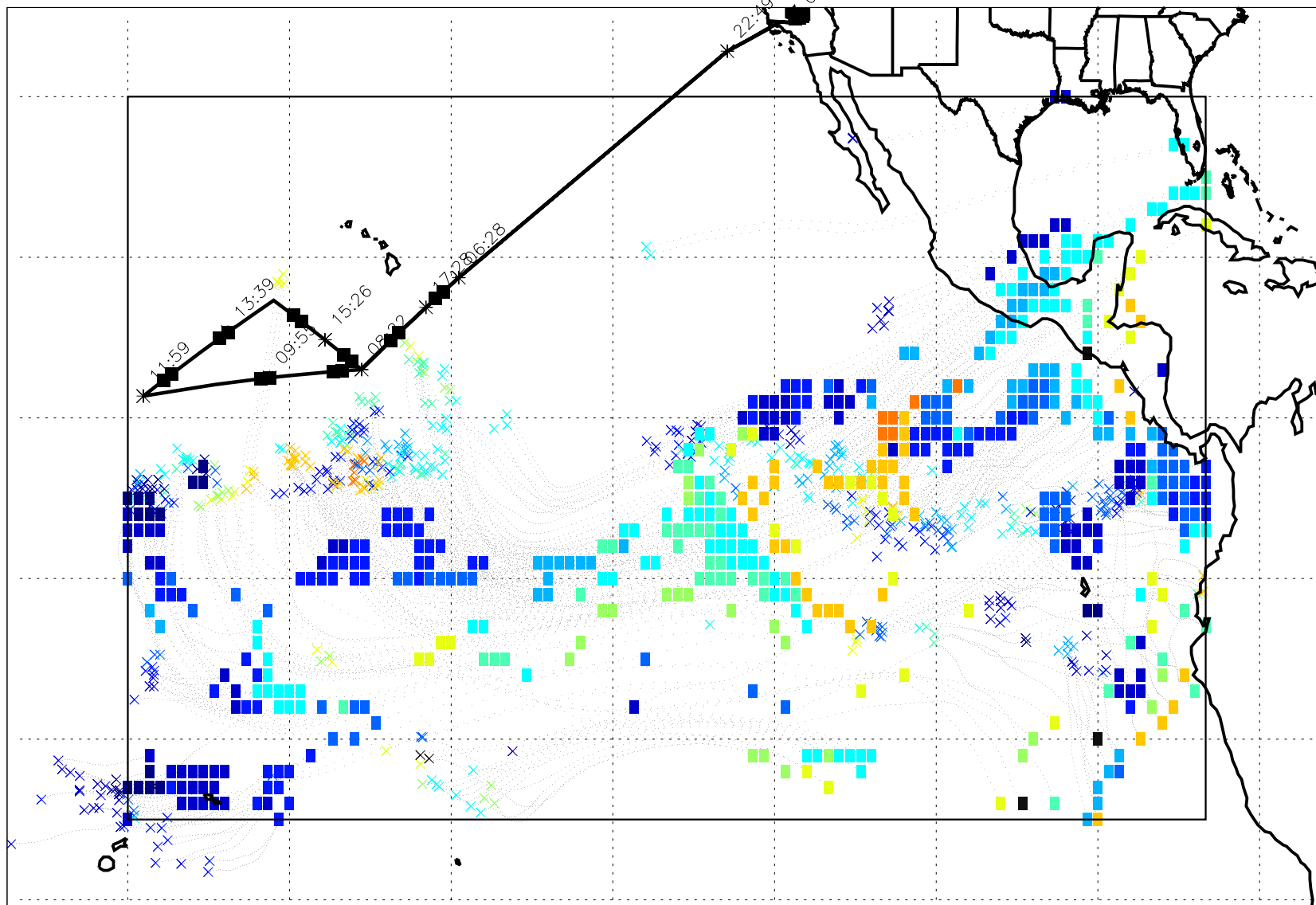
Fig. 2: Trajectories influenced by most recent convection that occurs within or near boxed region at location X.
