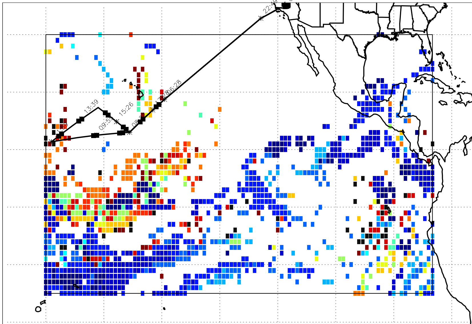
Fig. 1: End locations of trajectories influenced by convection in the past 14 days. Time since most recent convection in color.
