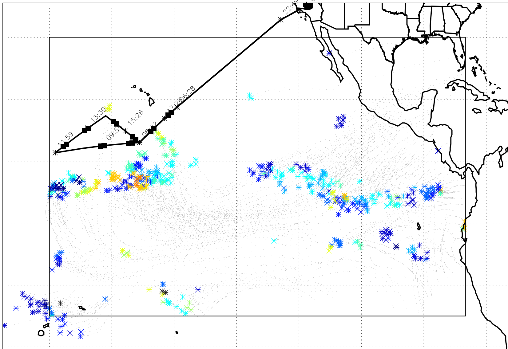
Fig. 3: Locations of most recent convection that occurs within or near boxed region (same as X in Fig. 2).
