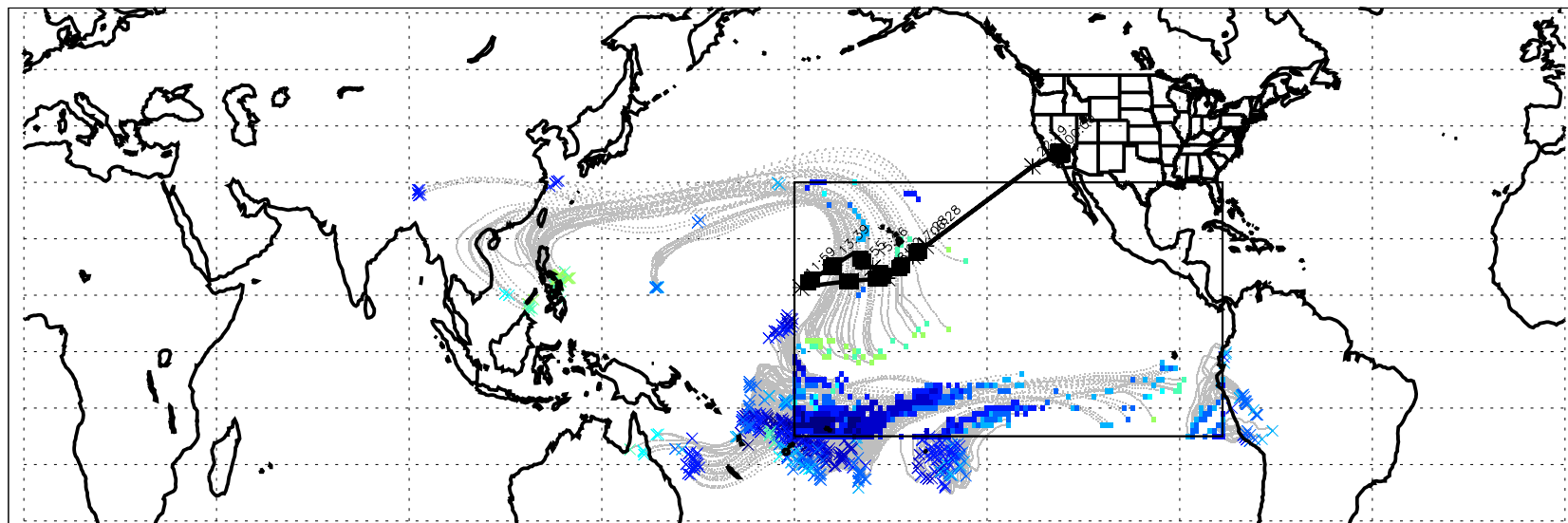
Fig. 4: Trajectories influenced by most recent convection that occurs outside of boxed region at location X.
