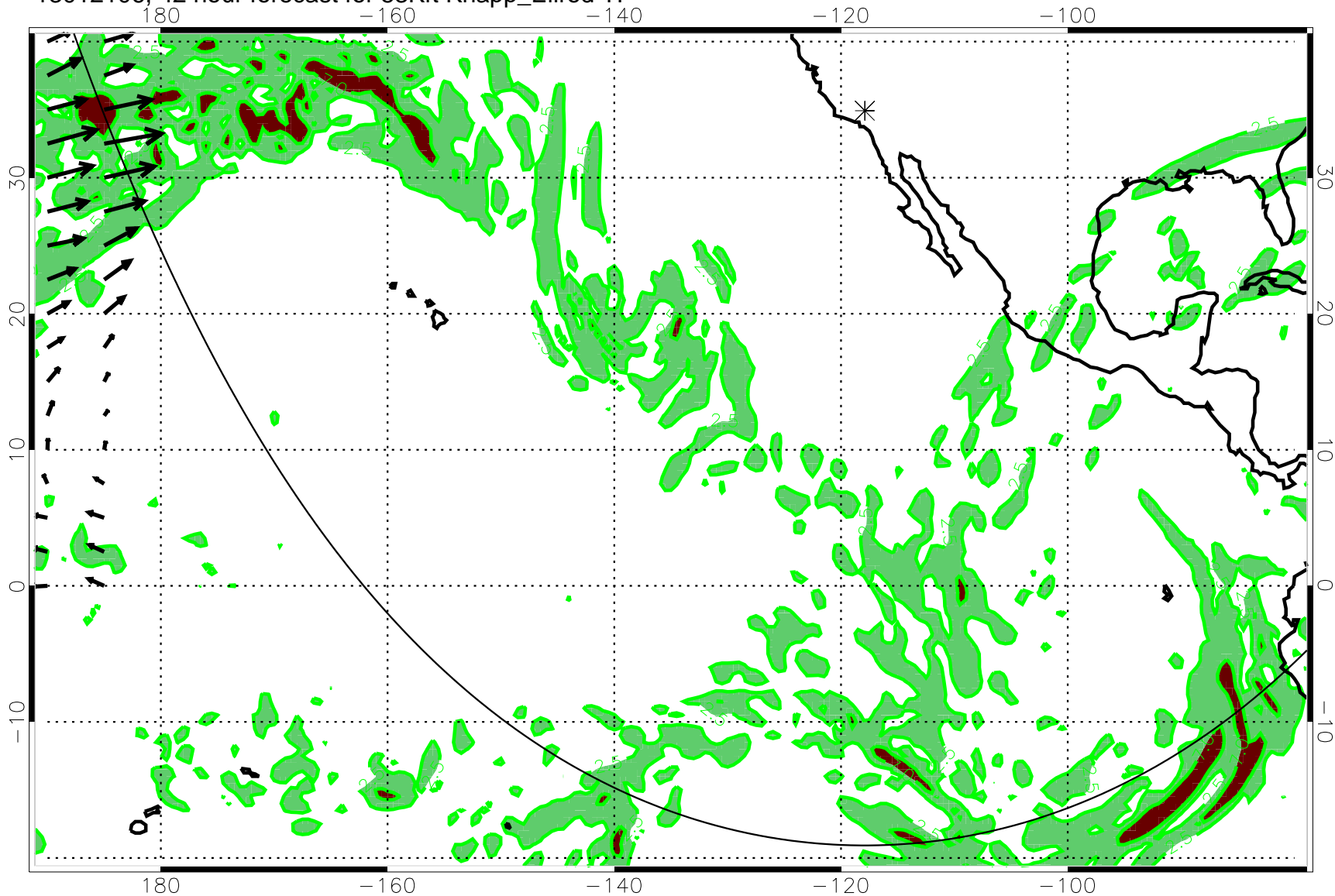
13012106, 42 hour forecast for 53Kft Knapp_Ellrod TI
