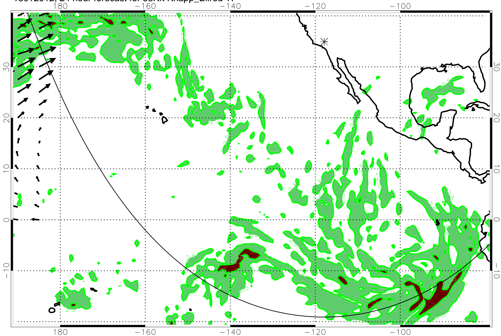
13012012, 24 hour forecast for 53Kft Knapp_Ellrod TI
