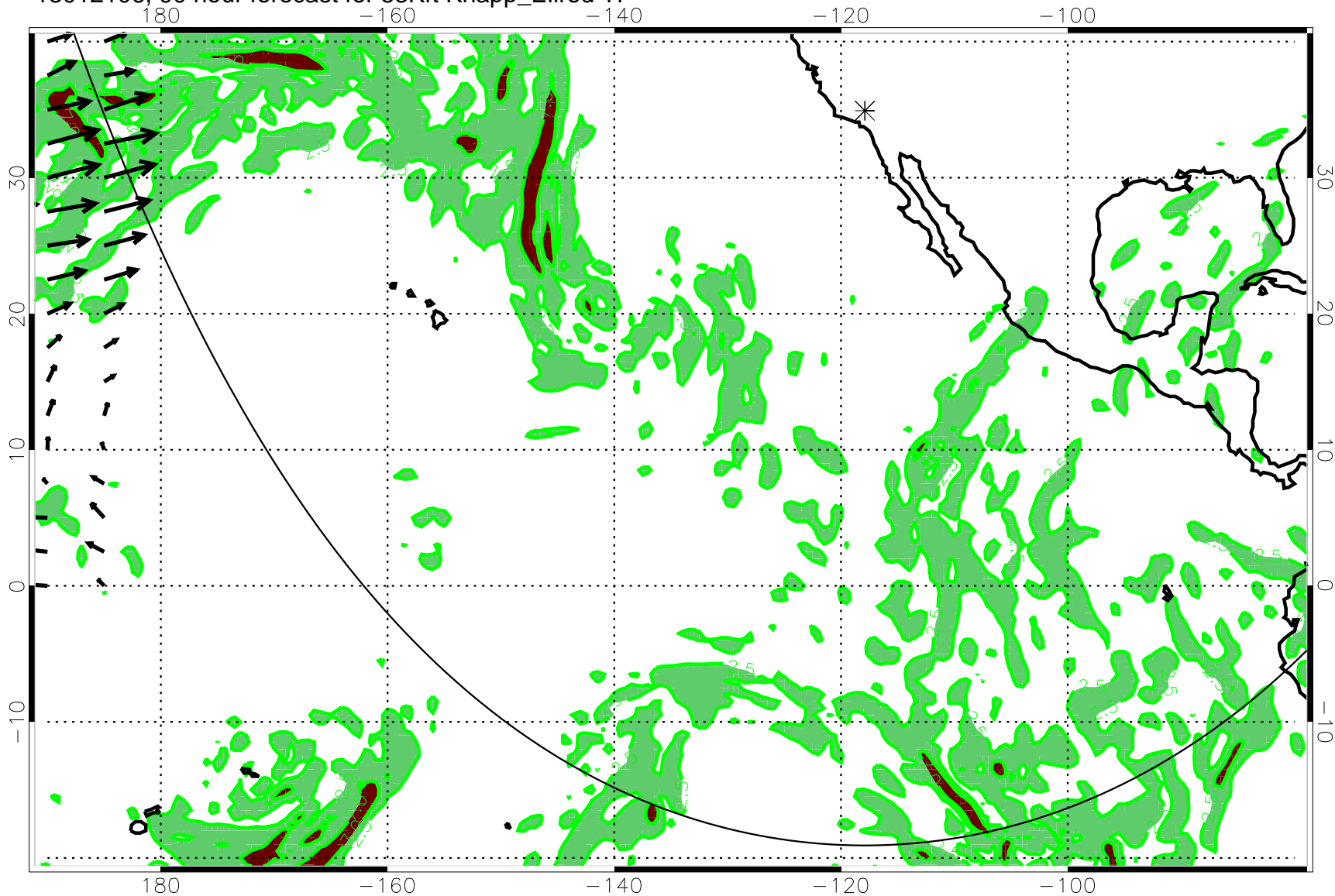
13012106, 90 hour forecast for 53Kft Knapp_Ellrod TI
