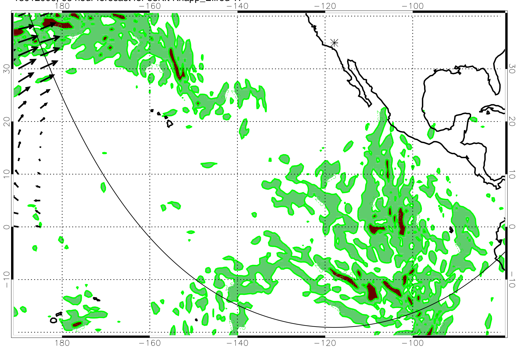
13012006, 66 hour forecast for 53Kft Knapp_Ellrod TI
