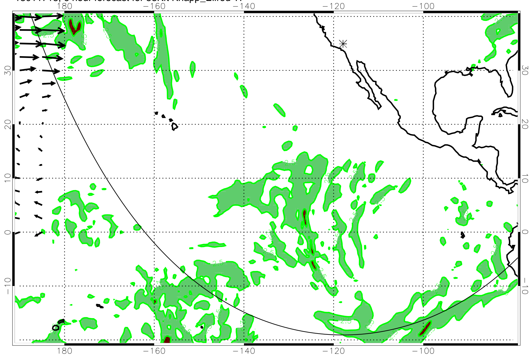
13011718, 6 hour forecast for 53Kft Knapp_Ellrod TI
