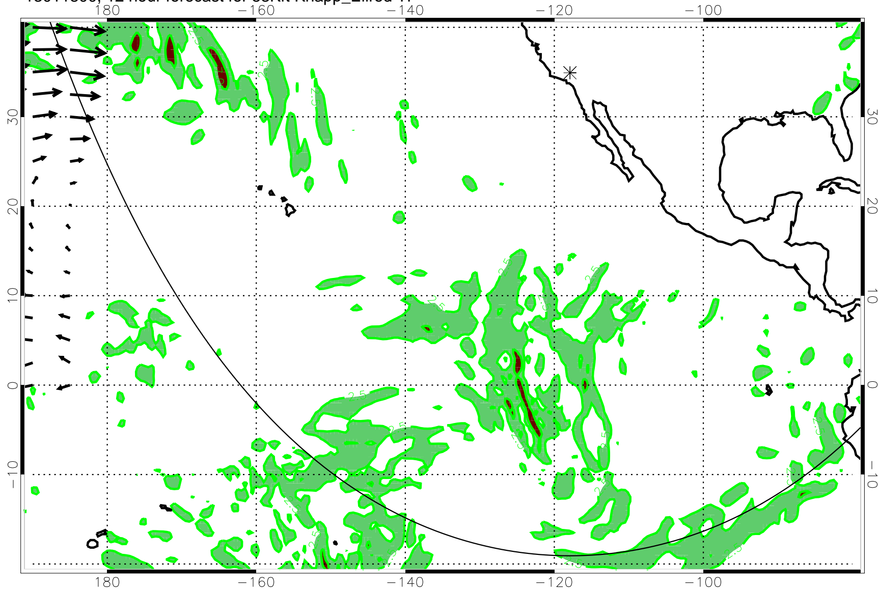
13011800, 12 hour forecast for 53Kft Knapp_Ellrod TI
