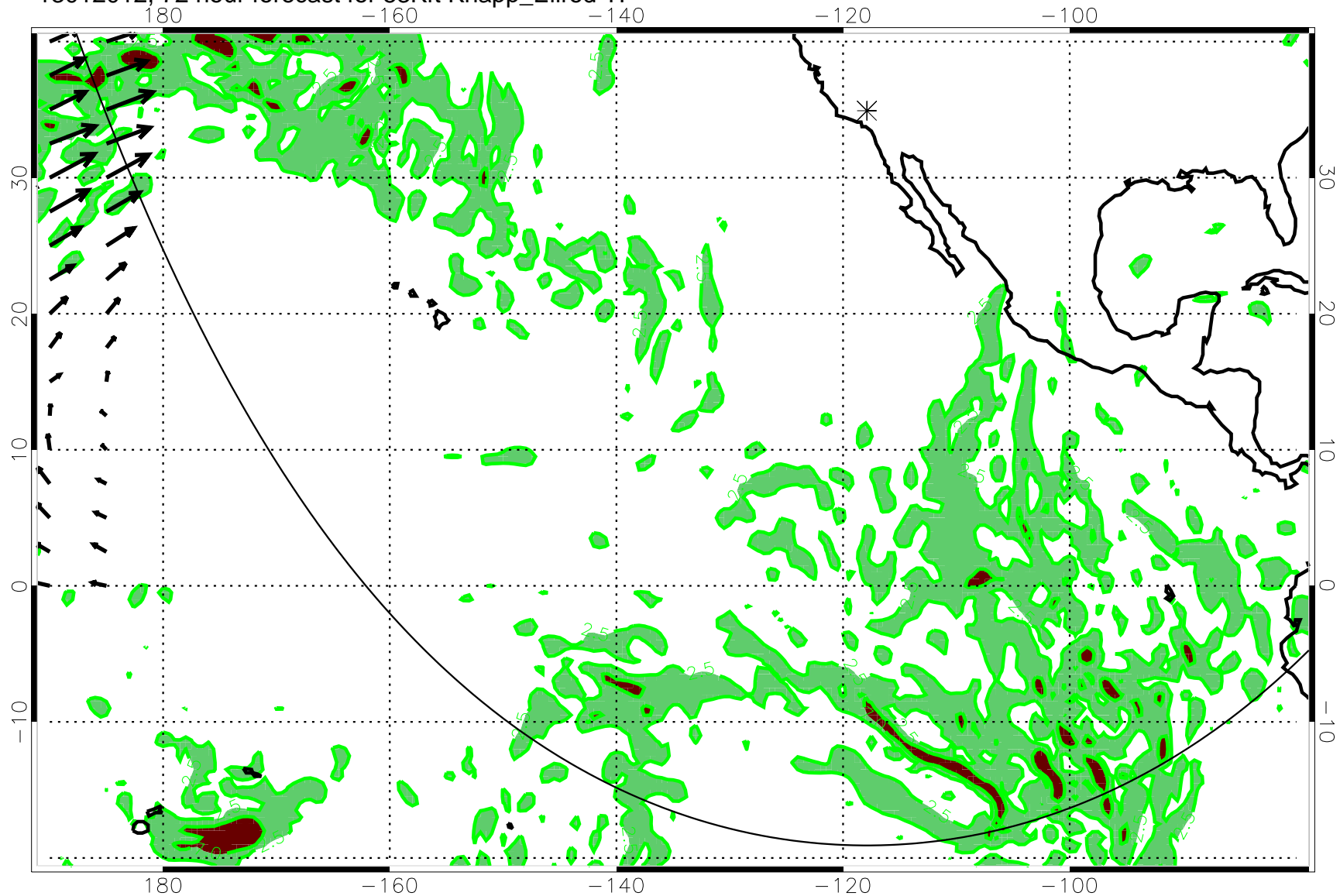
13012012, 72 hour forecast for 53Kft Knapp_Ellrod TI
