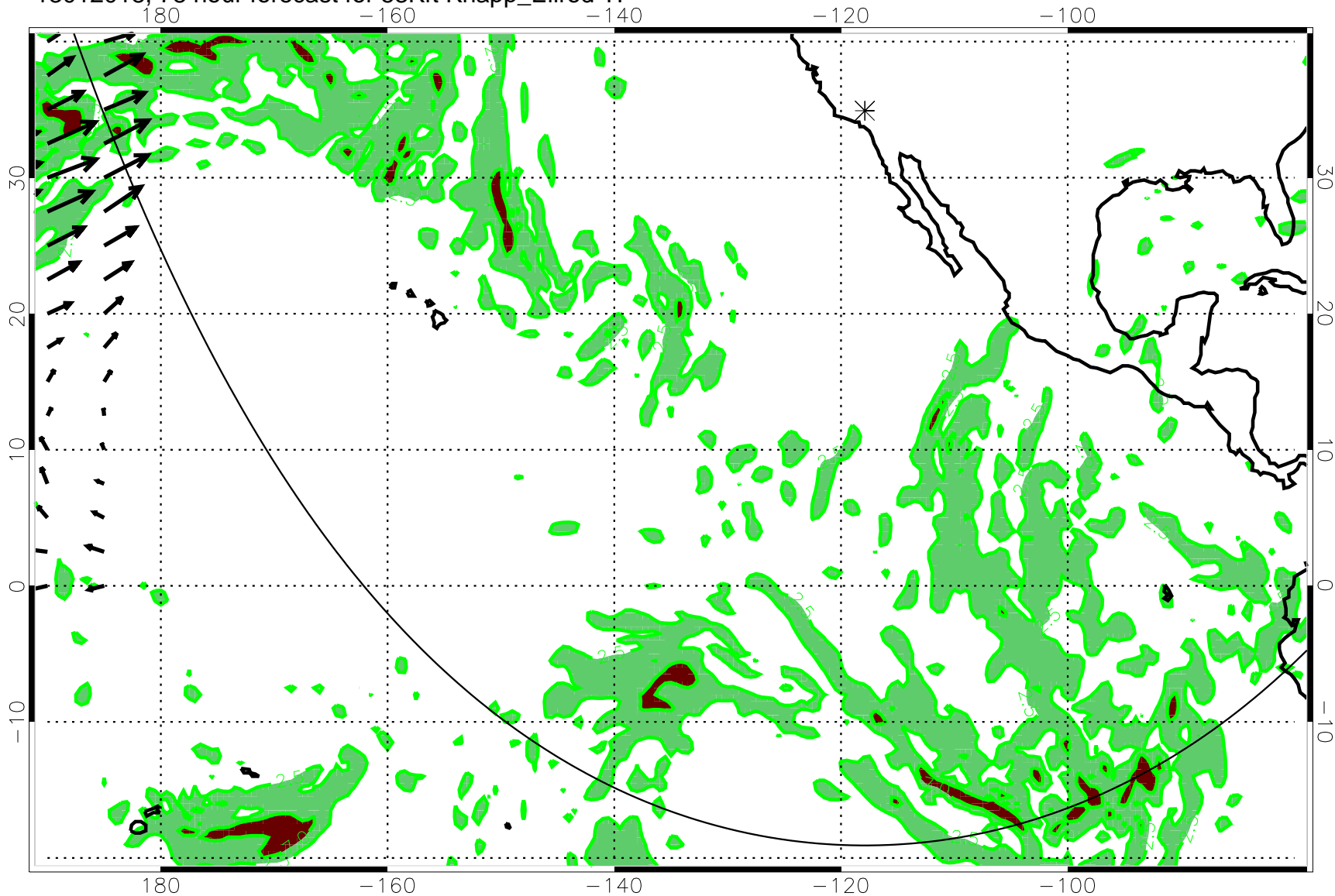
13012018, 78 hour forecast for 53Kft Knapp_Ellrod TI
