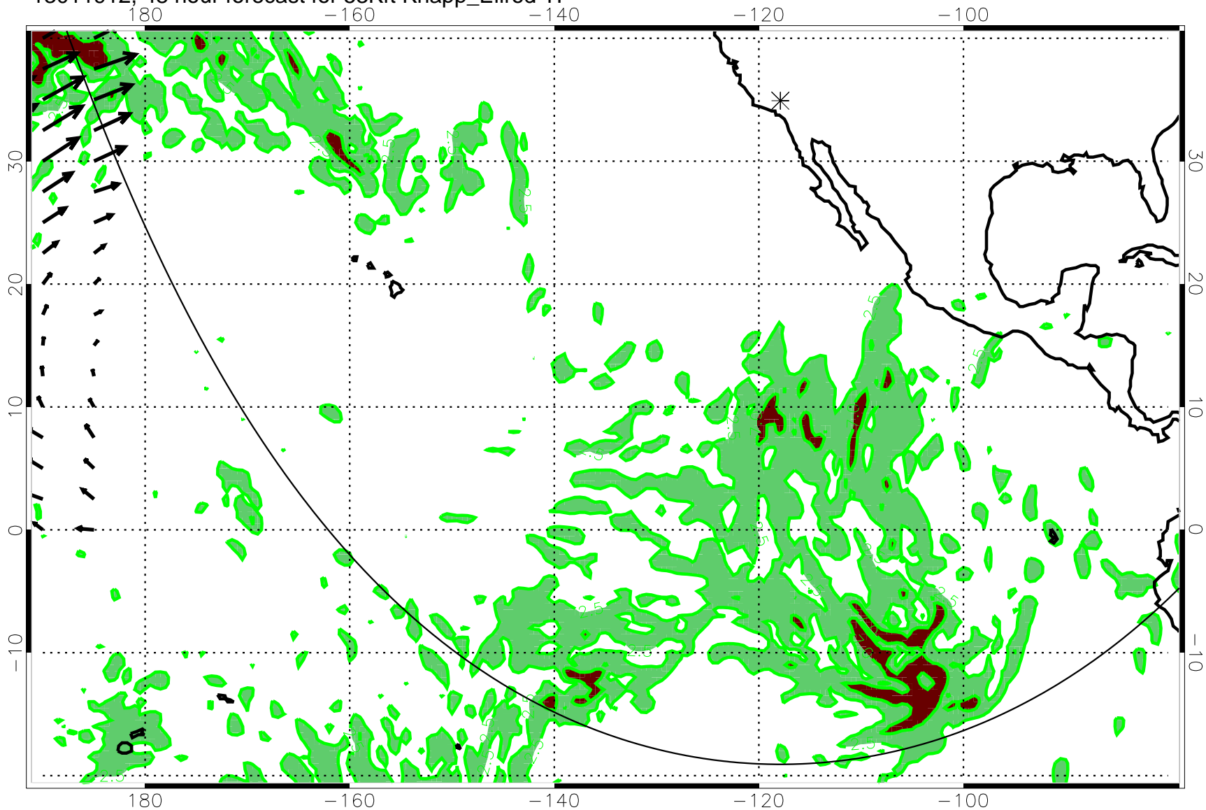
13011912, 48 hour forecast for 53Kft Knapp_Ellrod TI
