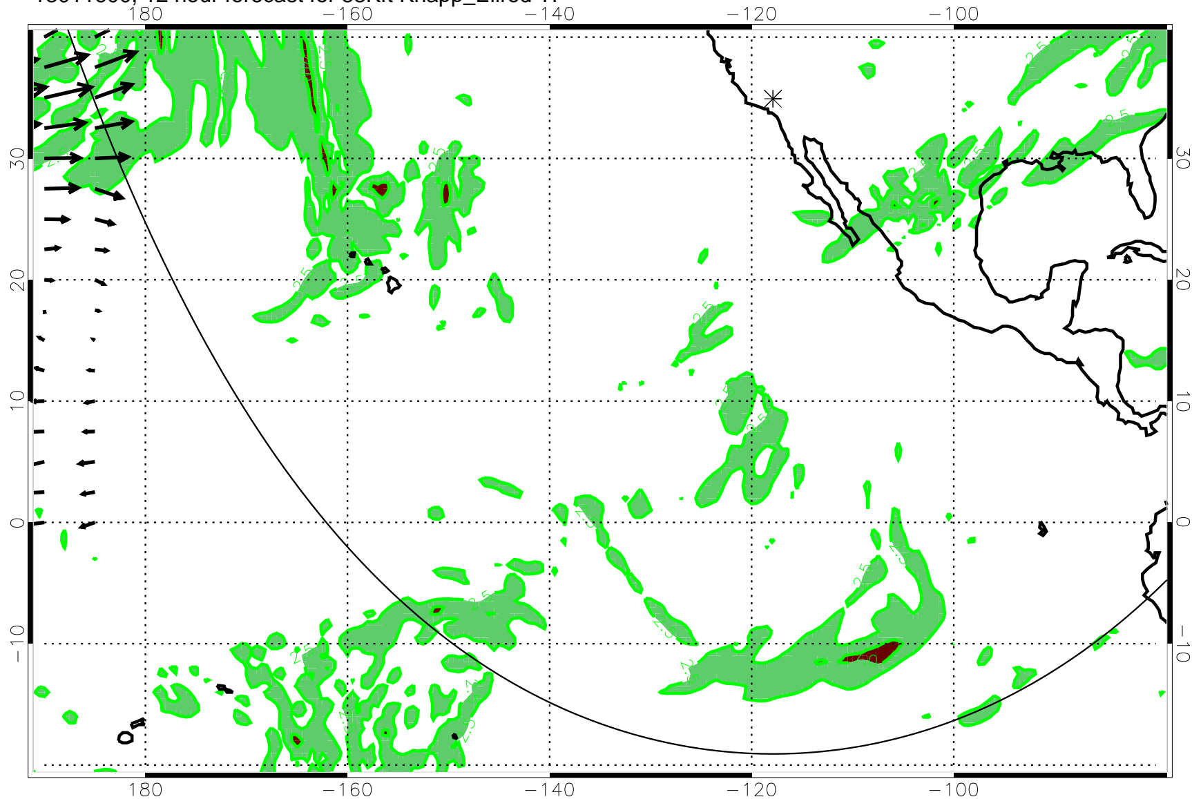
13011600, 12 hour forecast for 53Kft Knapp_Ellrod TI
