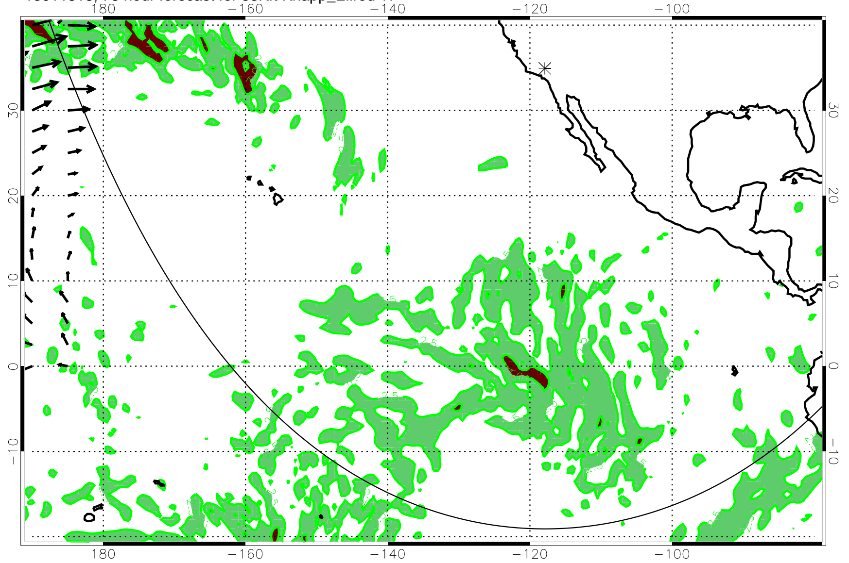
13011818, 78 hour forecast for 53Kft Knapp_Ellrod TI
