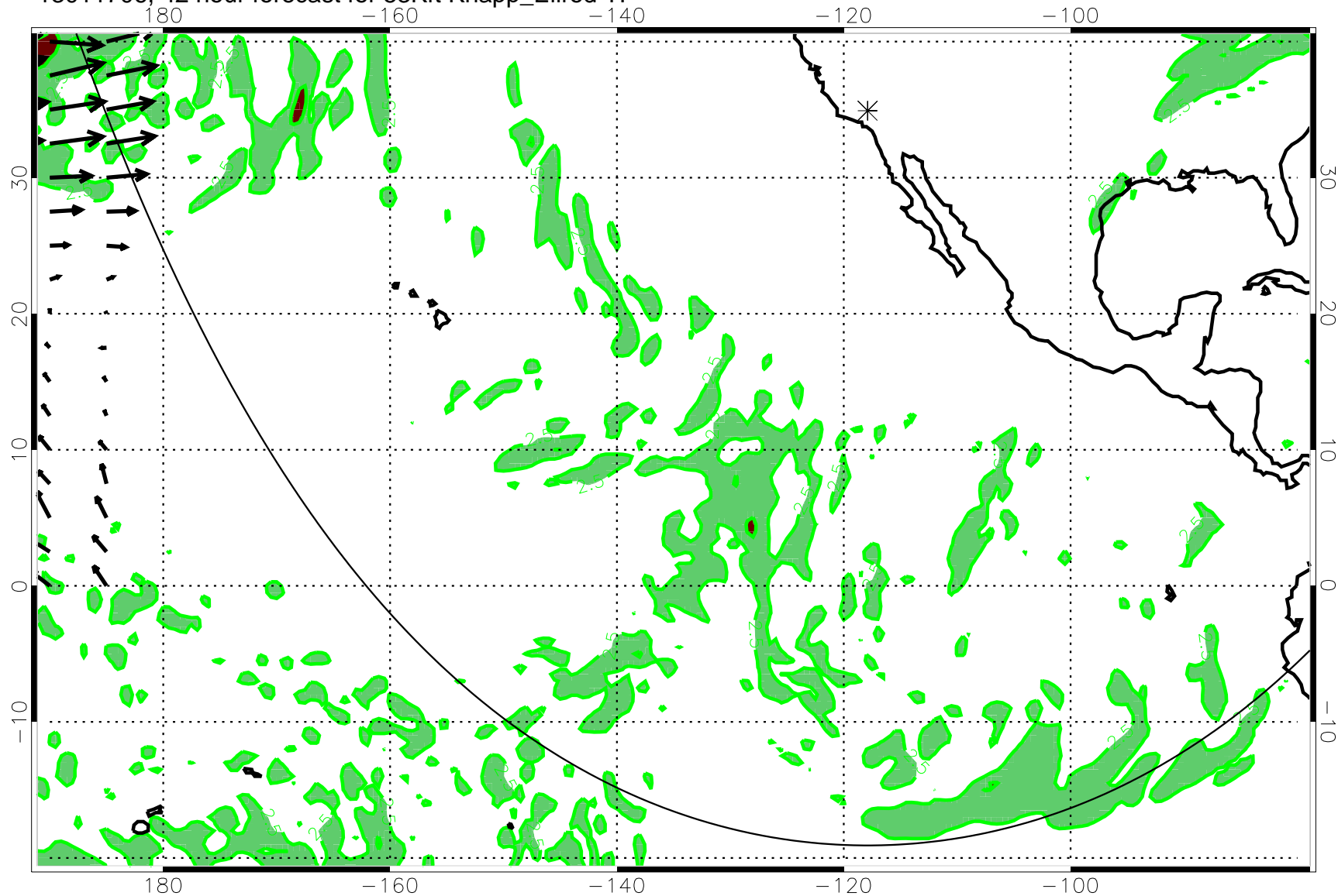
13011706, 42 hour forecast for 53Kft Knapp_Ellrod TI
