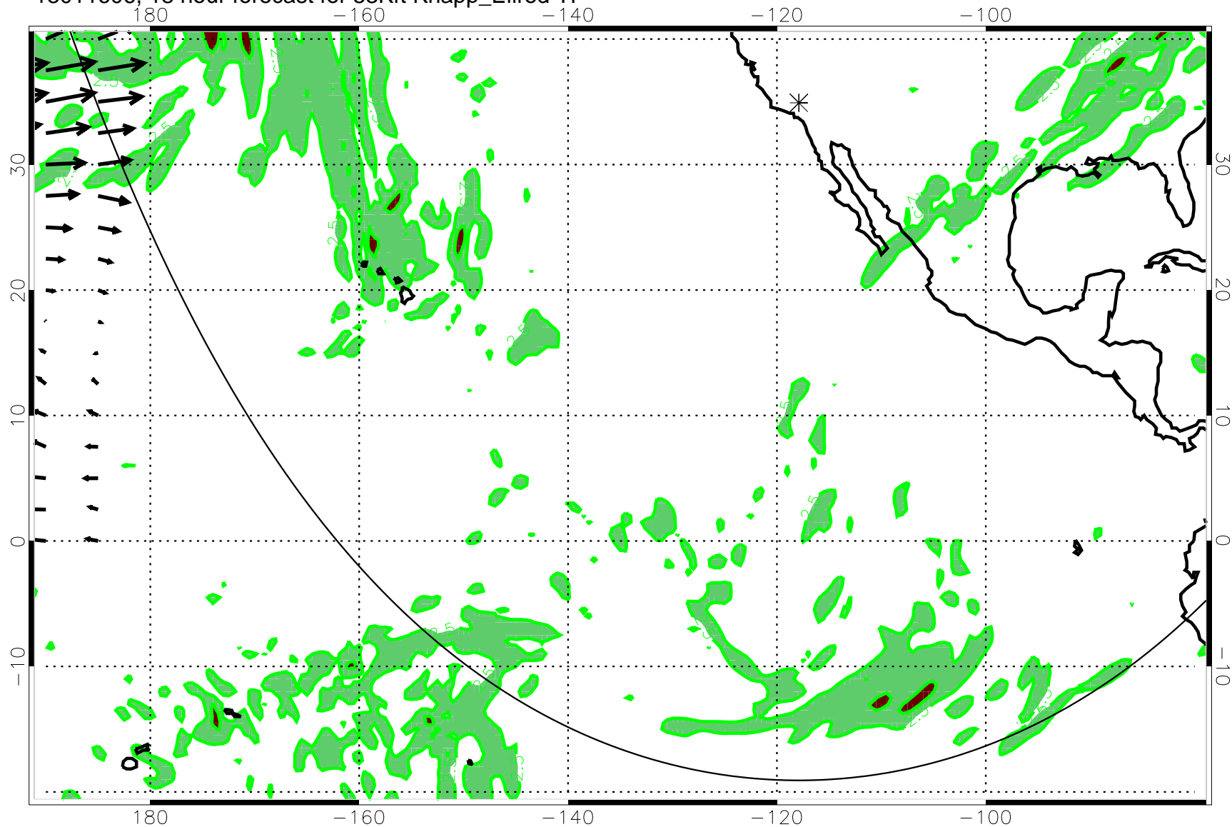
13011606, 18 hour forecast for 53Kft Knapp_Ellrod TI
