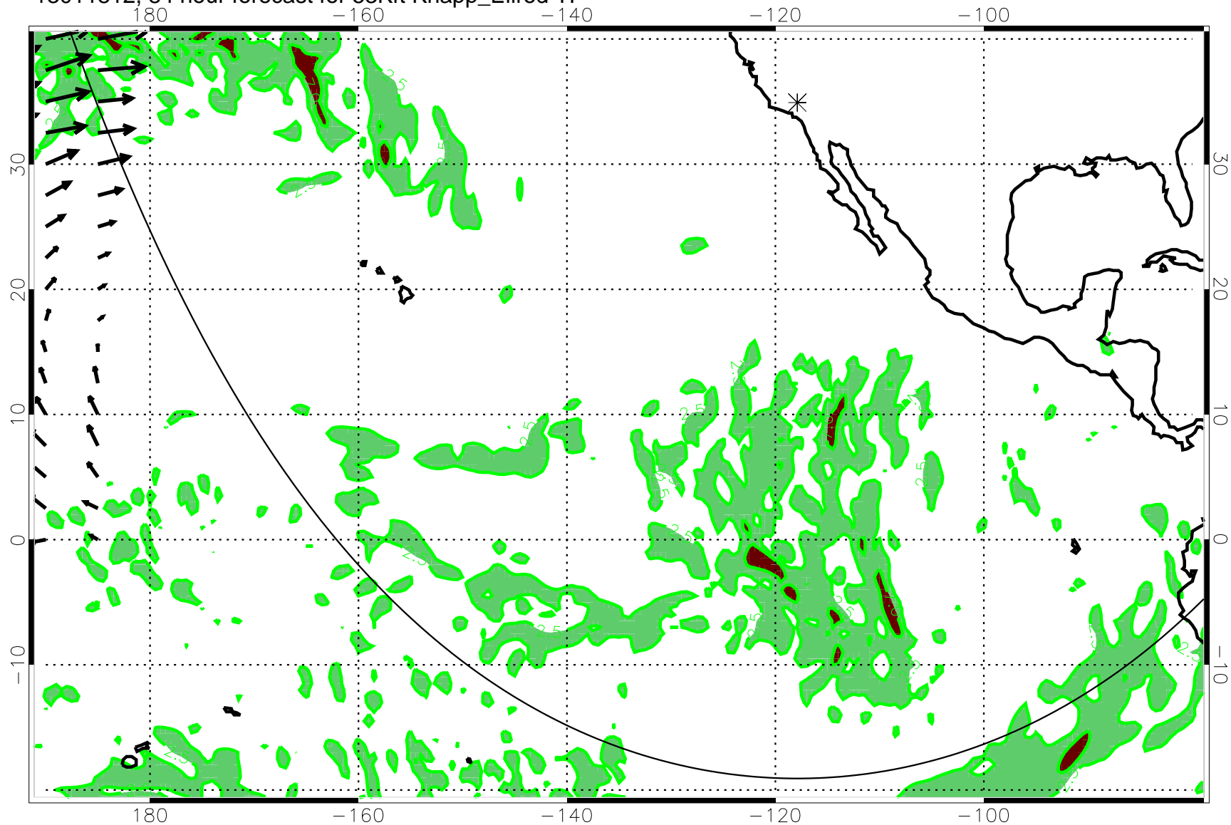
13011812, 84 hour forecast for 53Kft Knapp_Ellrod TI
