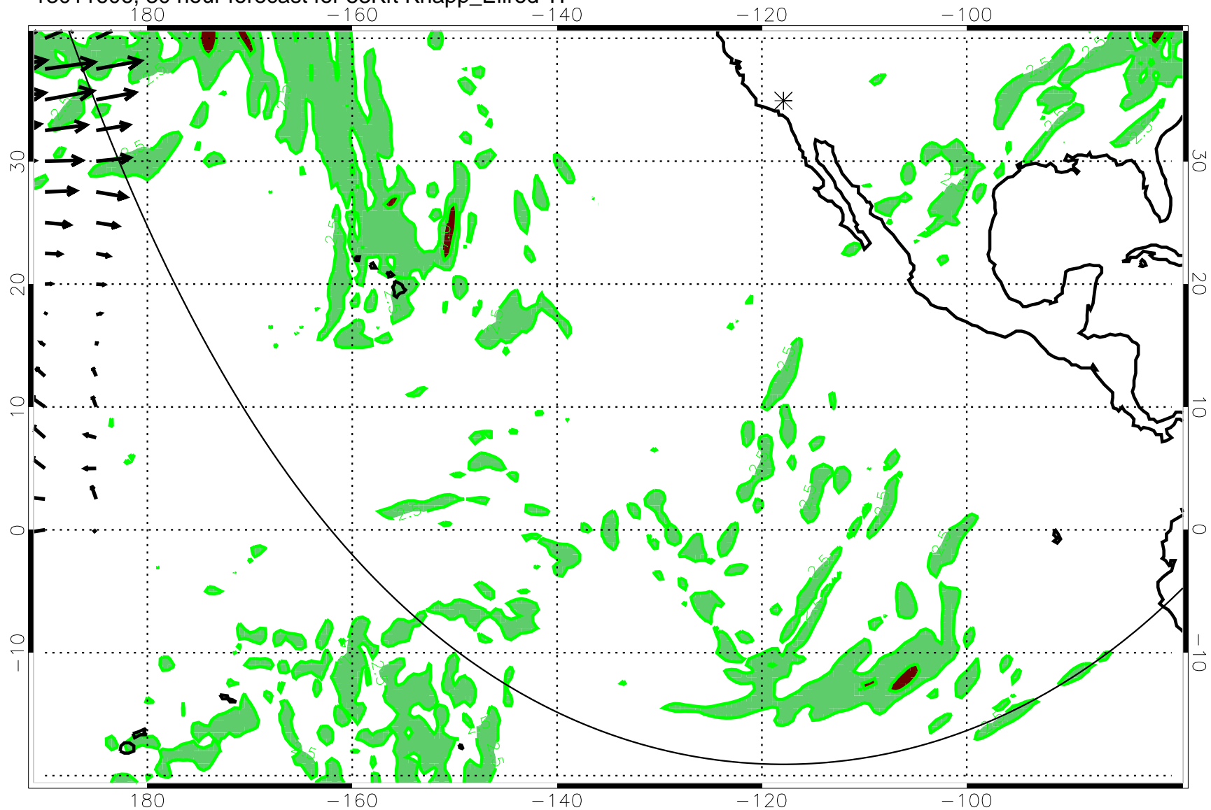
13011606, 30 hour forecast for 53Kft Knapp_Ellrod TI
