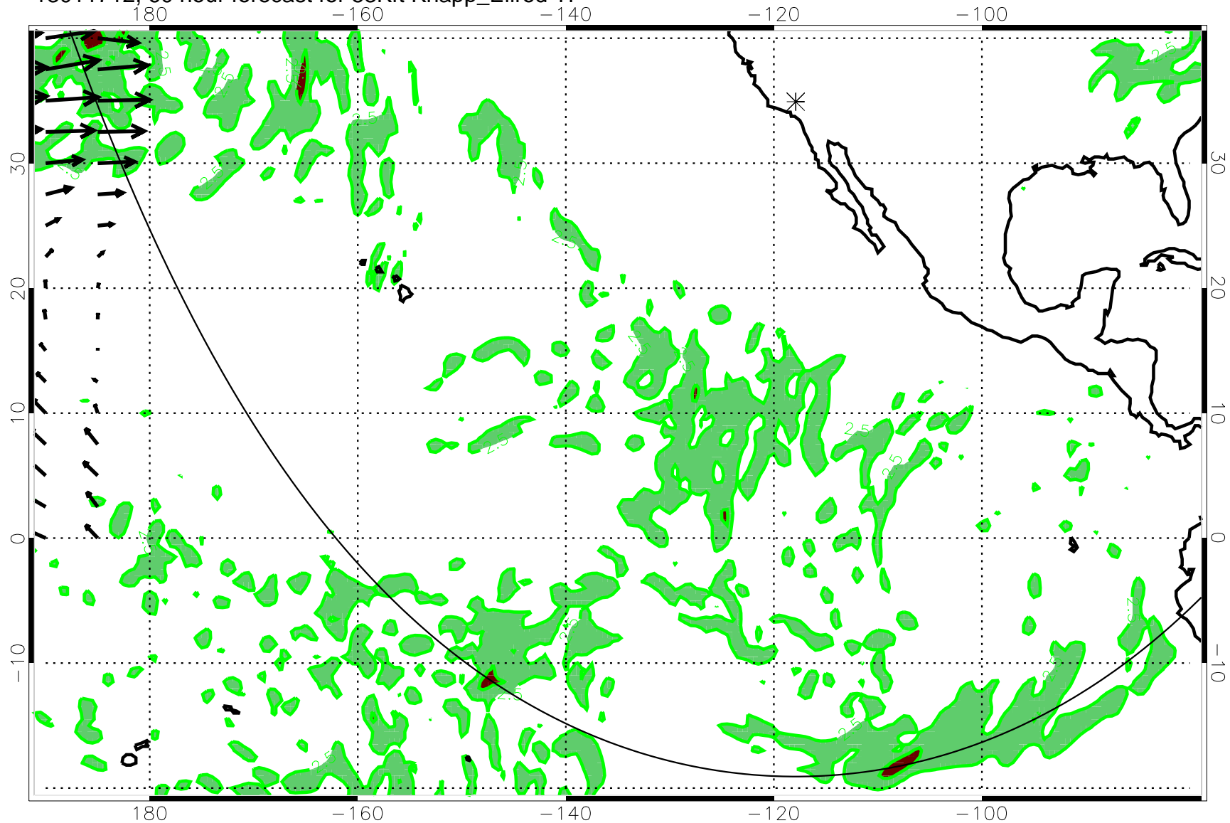
13011712, 60 hour forecast for 53Kft Knapp_Ellrod TI
