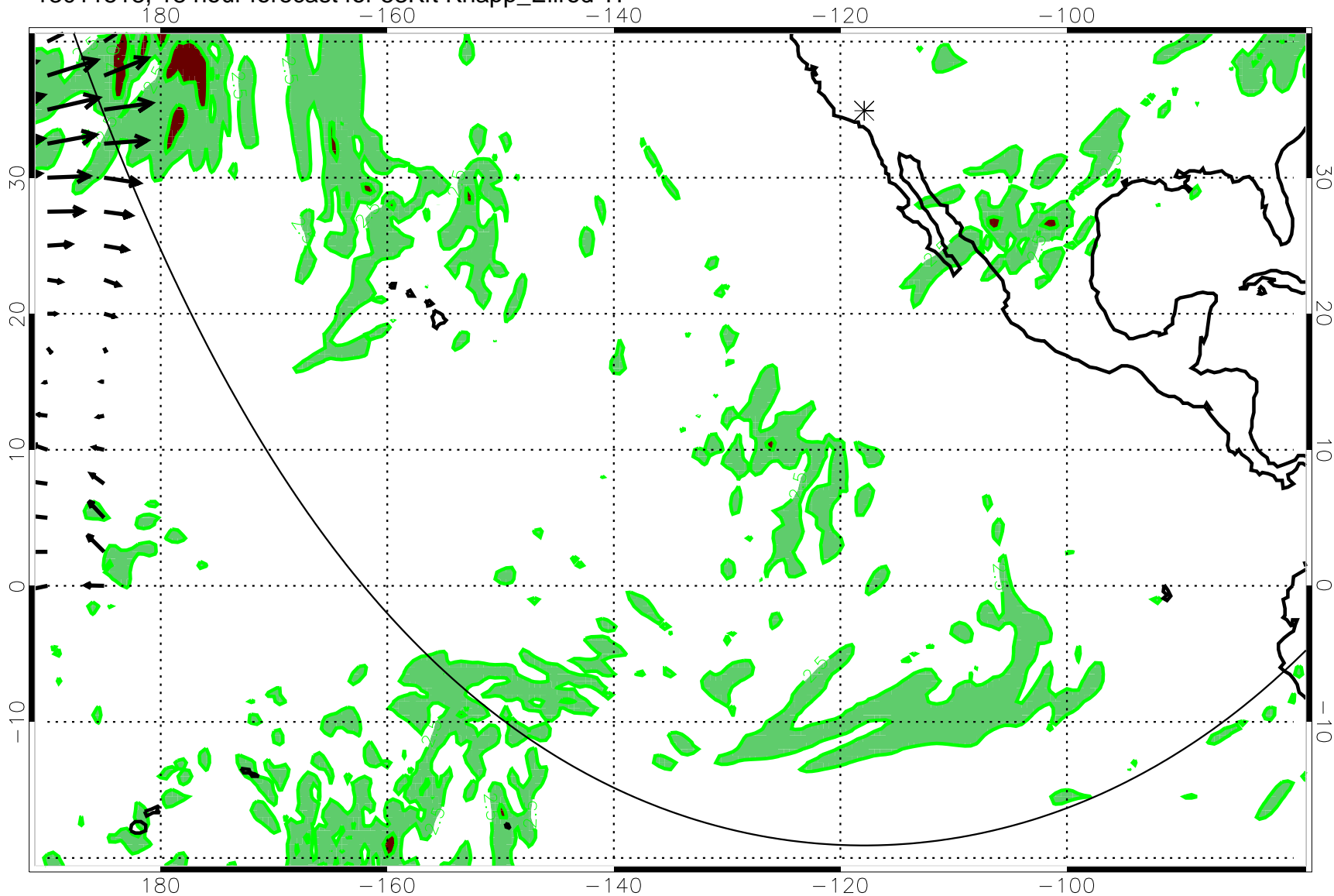
13011518, 18 hour forecast for 53Kft Knapp_Ellrod TI
