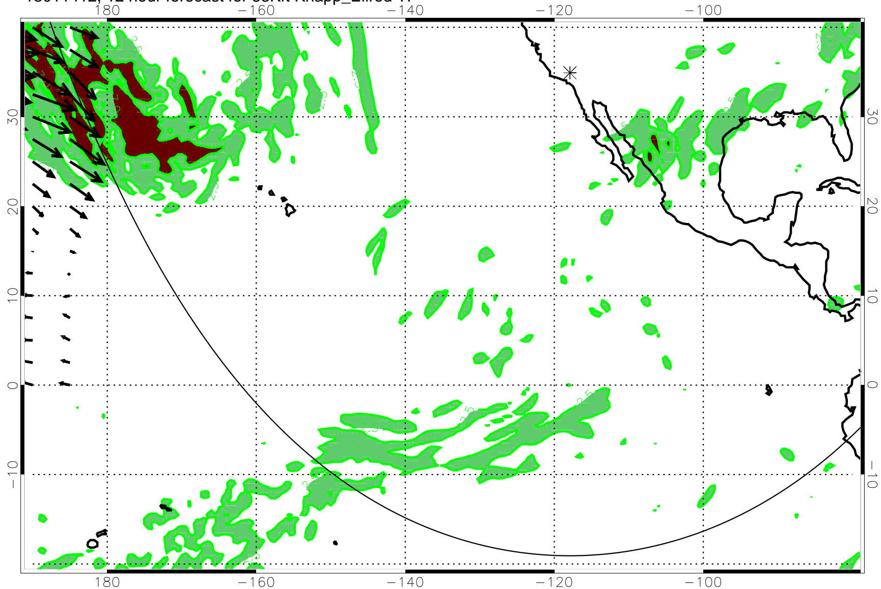
13011412, 12 hour forecast for 53Kft Knapp_Ellrod TI
