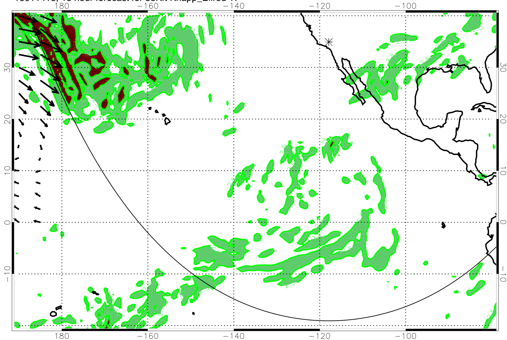
13011418, 18 hour forecast for 53Kft Knapp_Ellrod TI
