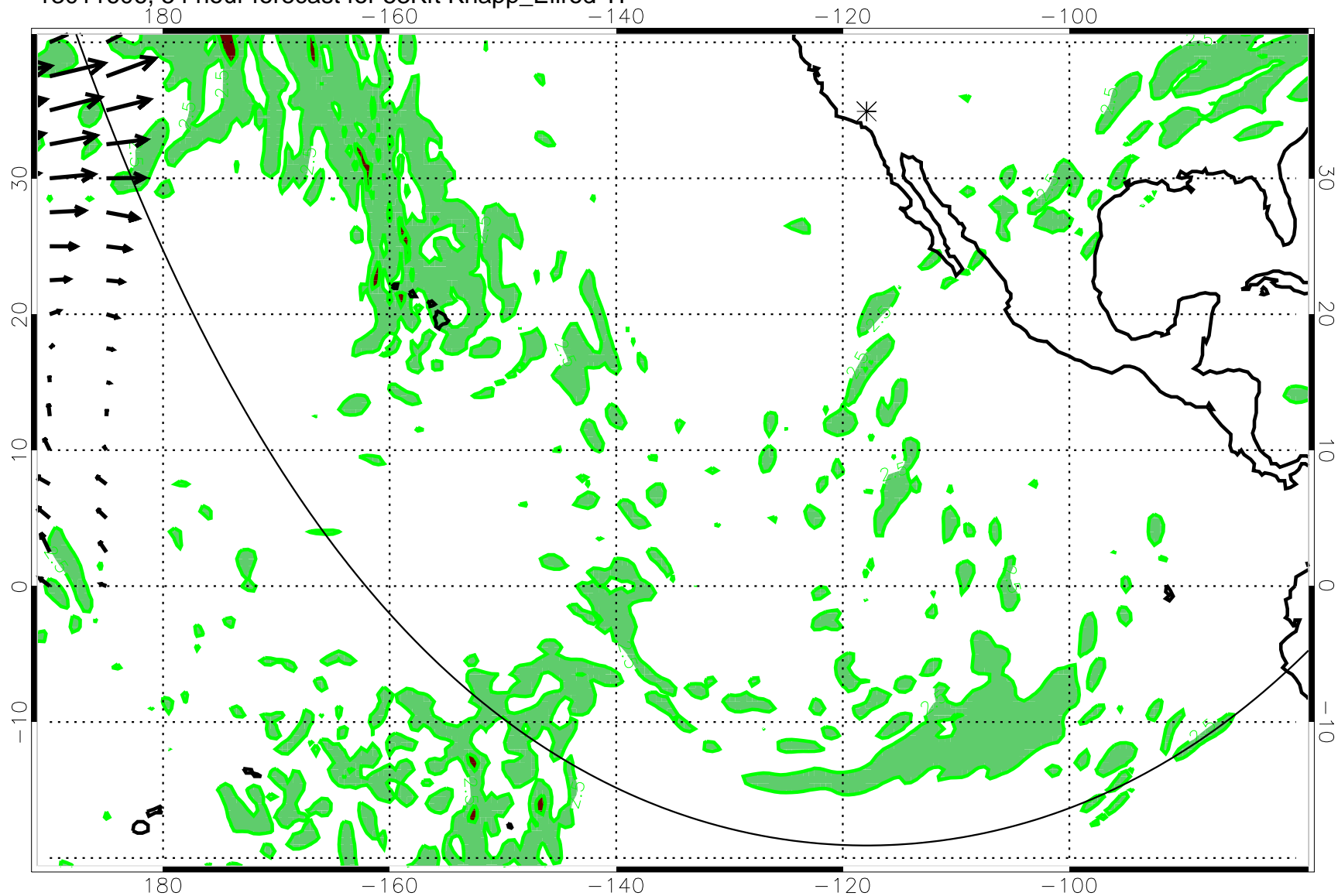
13011606, 54 hour forecast for 53Kft Knapp_Ellrod TI
