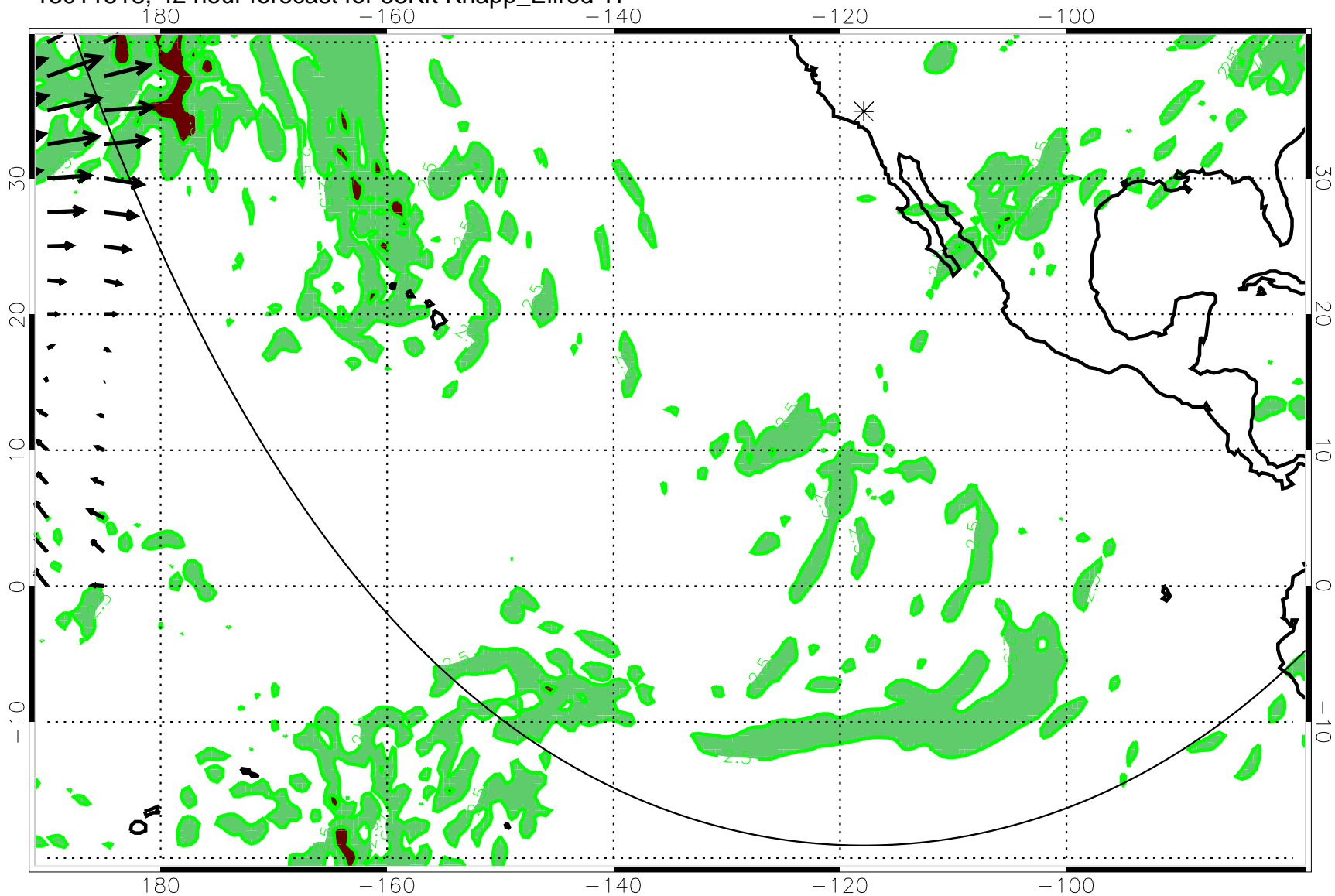
13011518, 42 hour forecast for 53Kft Knapp_Ellrod TI
