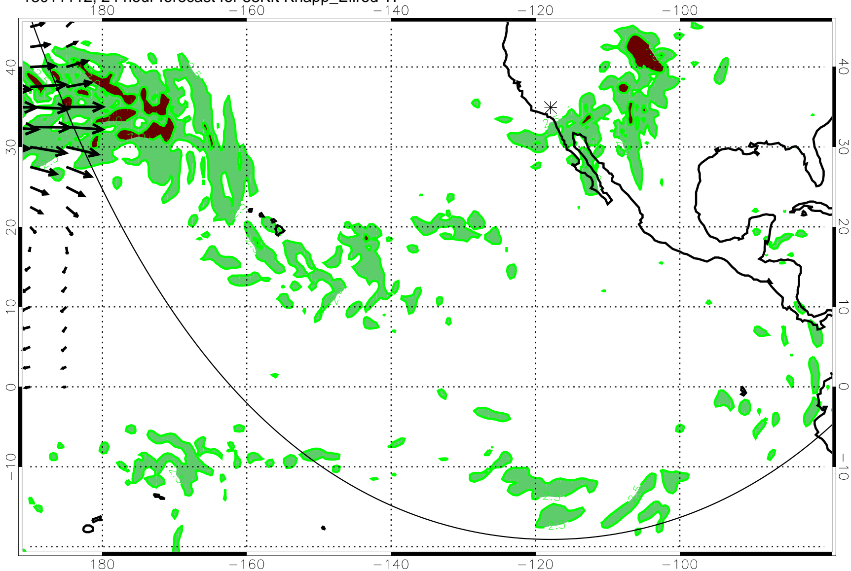
13011112, 24 hour forecast for 53Kft Knapp_Ellrod TI
