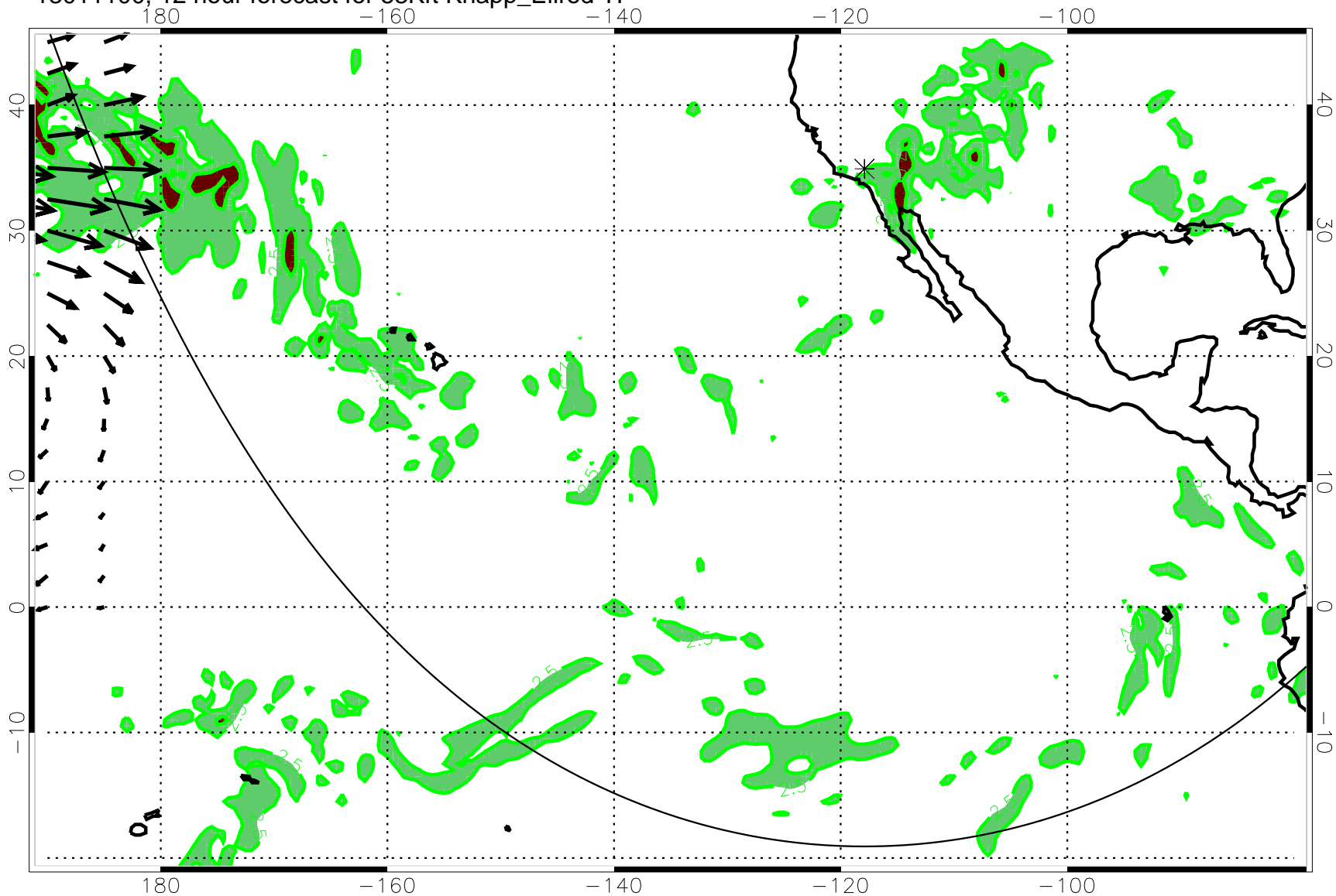
13011100, 12 hour forecast for 53Kft Knapp_Ellrod TI
