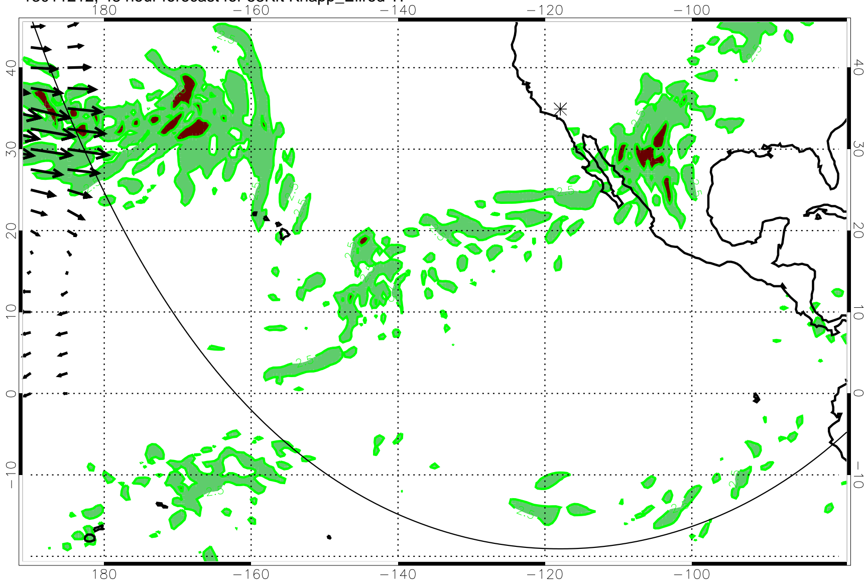
13011212, 48 hour forecast for 53Kft Knapp_Ellrod TI
