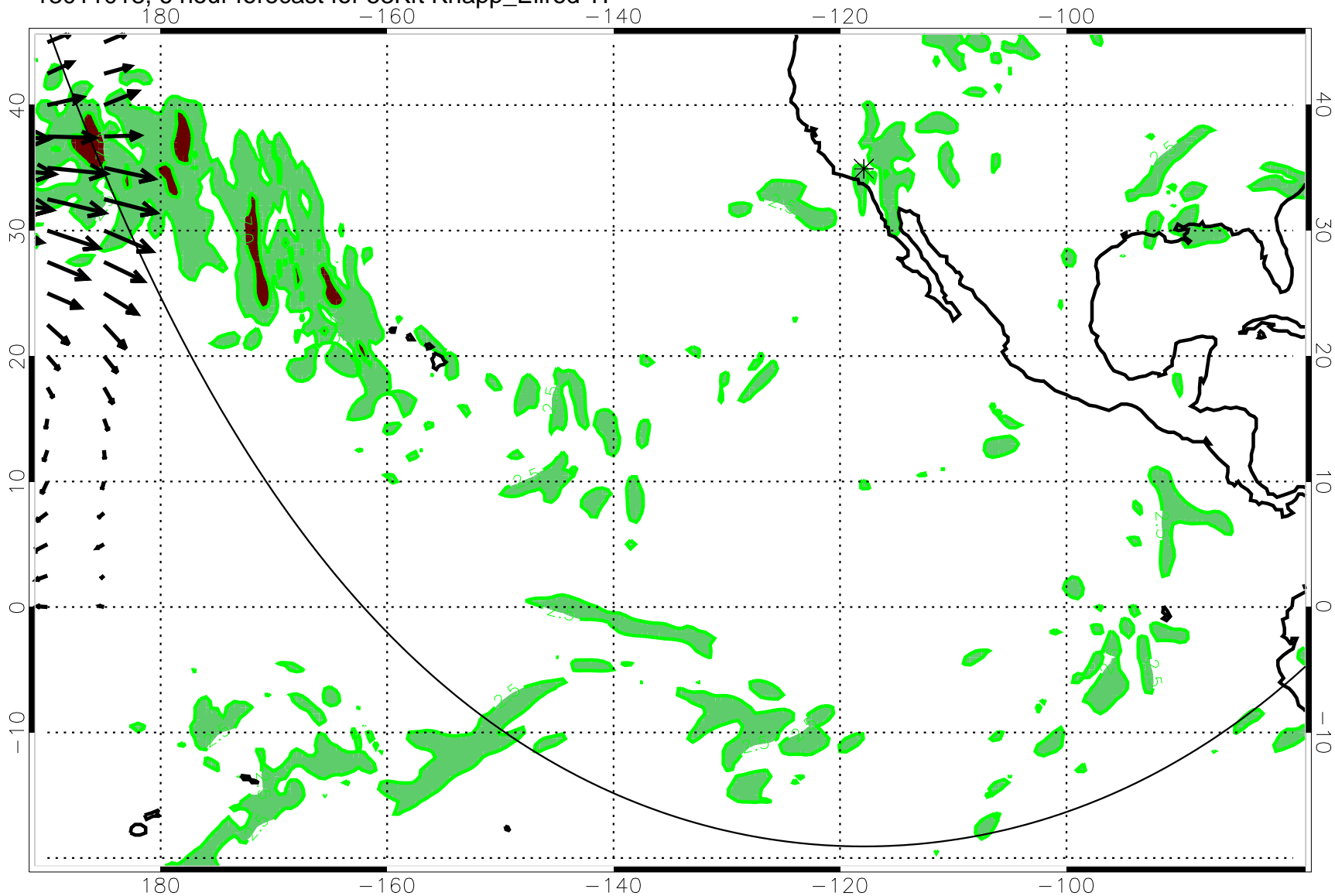
13011018, 6 hour forecast for 53Kft Knapp_Ellrod TI
