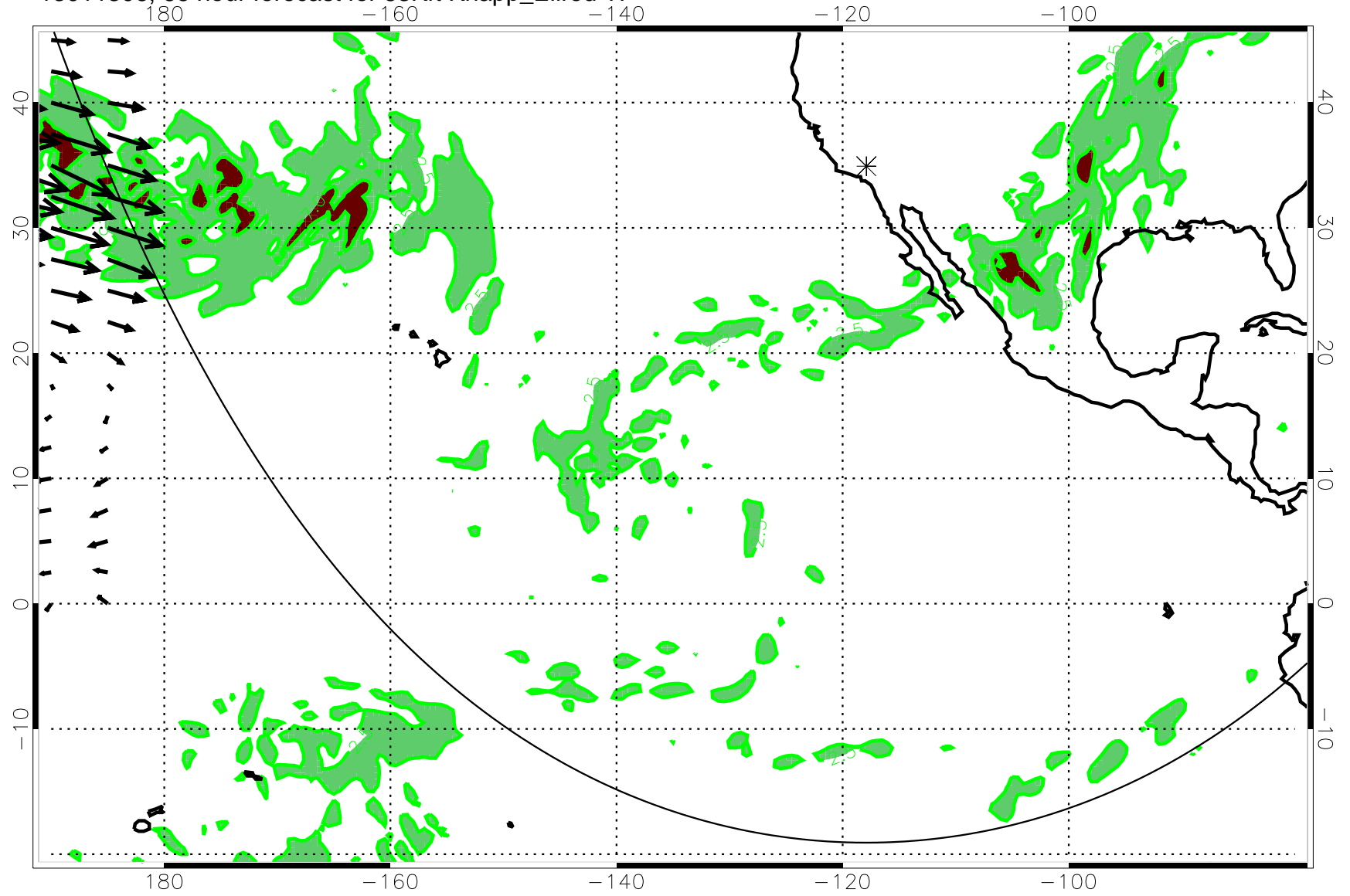
13011306, 66 hour forecast for 53Kft Knapp_Ellrod TI
