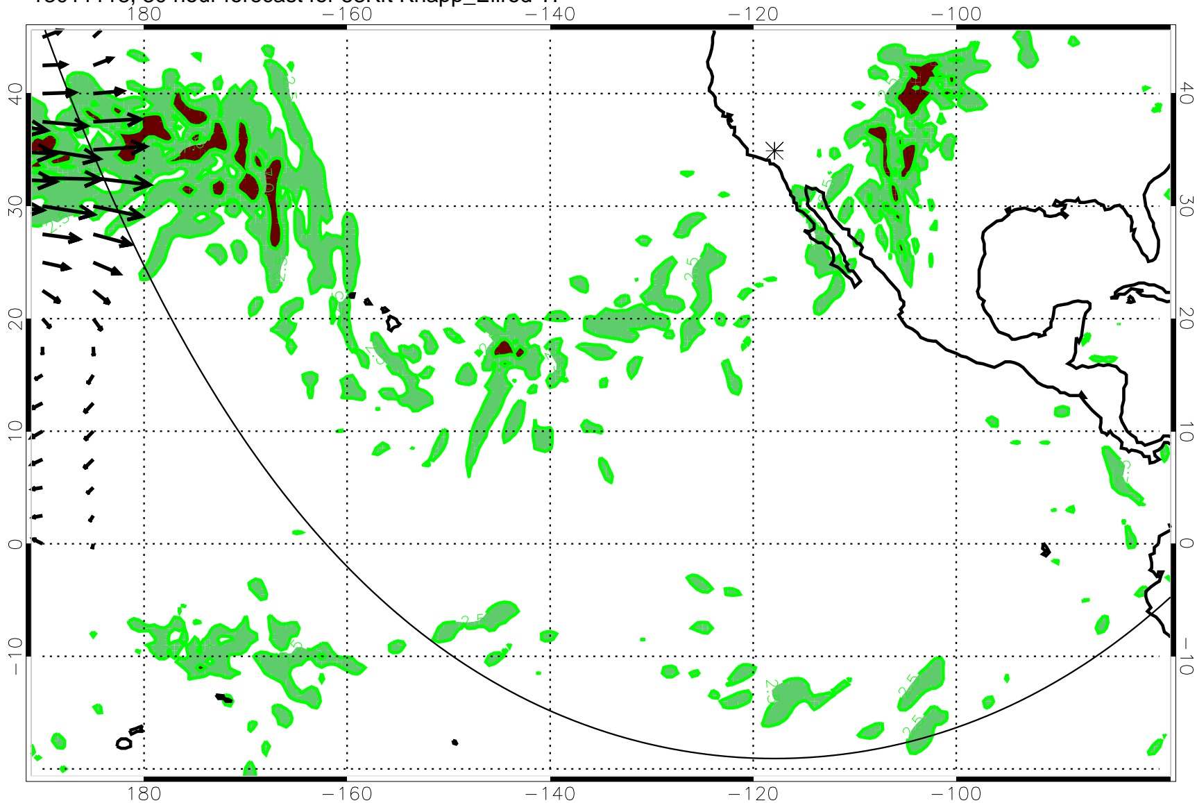
13011118, 30 hour forecast for 53Kft Knapp_Ellrod TI
