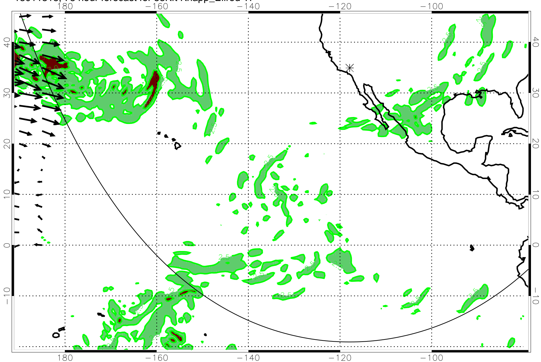
13011318, 78 hour forecast for 53Kft Knapp_Ellrod TI
