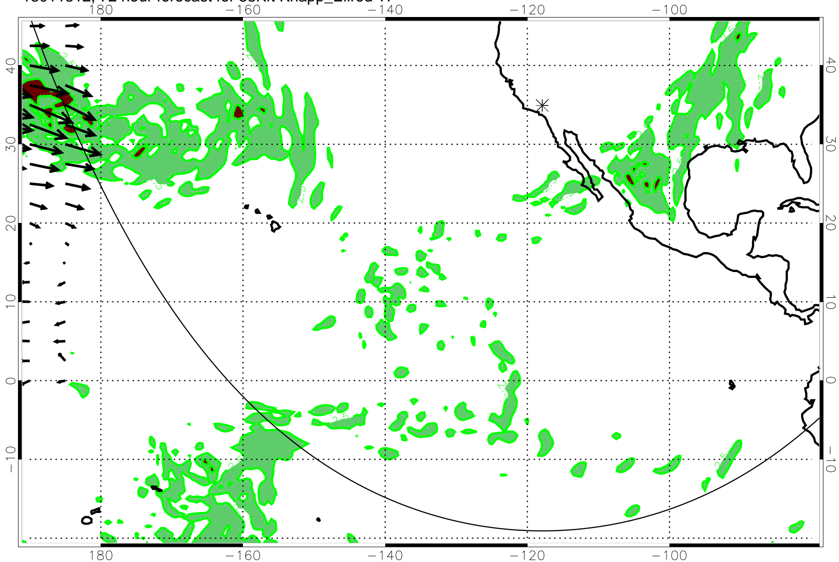
13011312, 72 hour forecast for 53Kft Knapp_Ellrod TI
