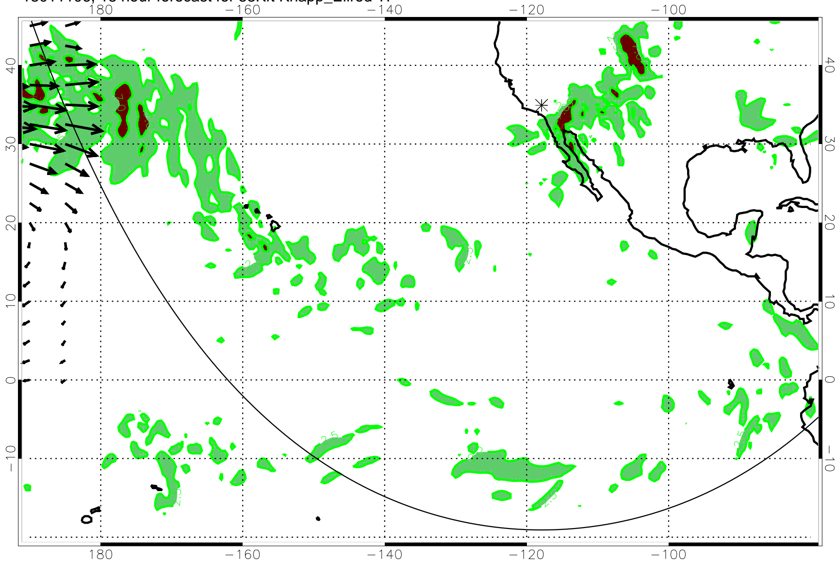
13011106, 18 hour forecast for 53Kft Knapp_Ellrod TI
