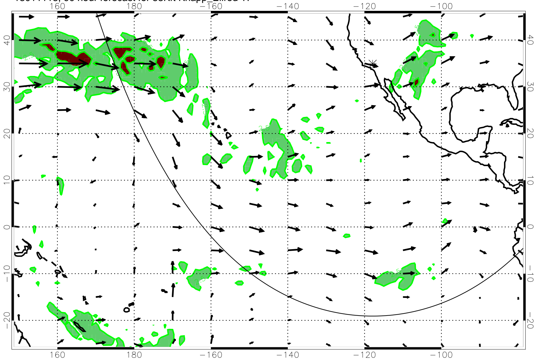
13011118, 90 hour forecast for 53Kft Knapp_Ellrod T1
