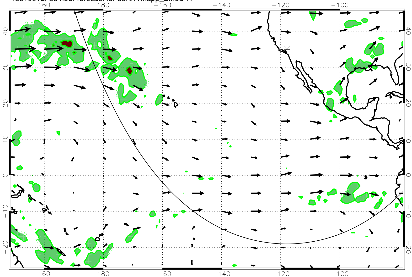
13010912, 36 hour forecast for 53Kft Knapp_Ellrod T1
