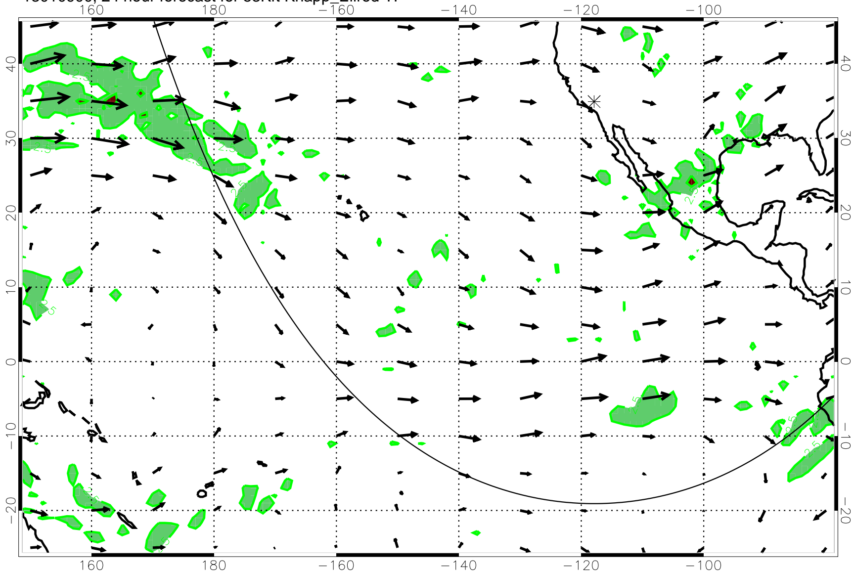
13010900, 24 hour forecast for 53Kft Knapp_Ellrod T1
