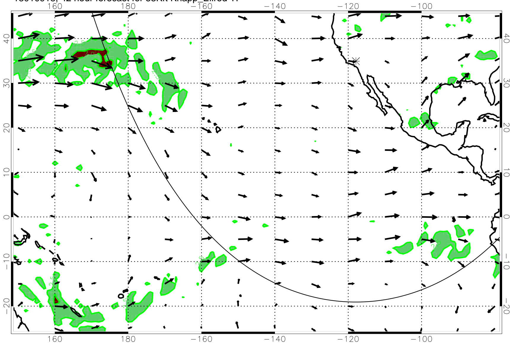
13010918, 42 hour forecast for 53Kft Knapp_Ellrod T1
