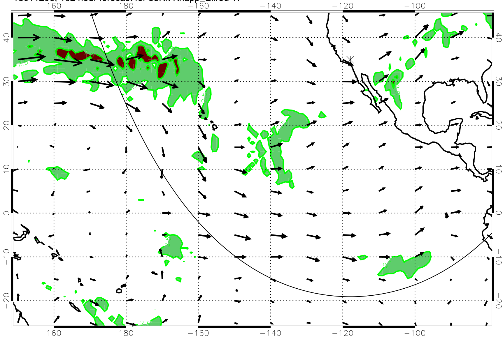
13011206, 102 hour forecast for 53Kft Knapp_Ellrod T1
