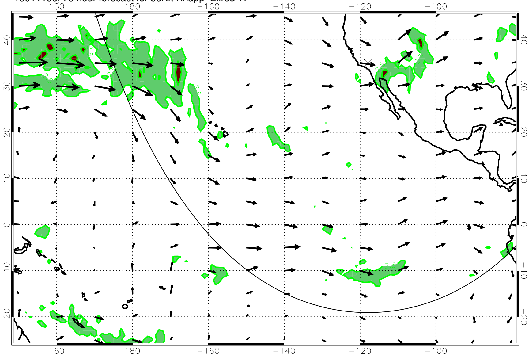
13011106, 78 hour forecast for 53Kft Knapp_Ellrod T1
