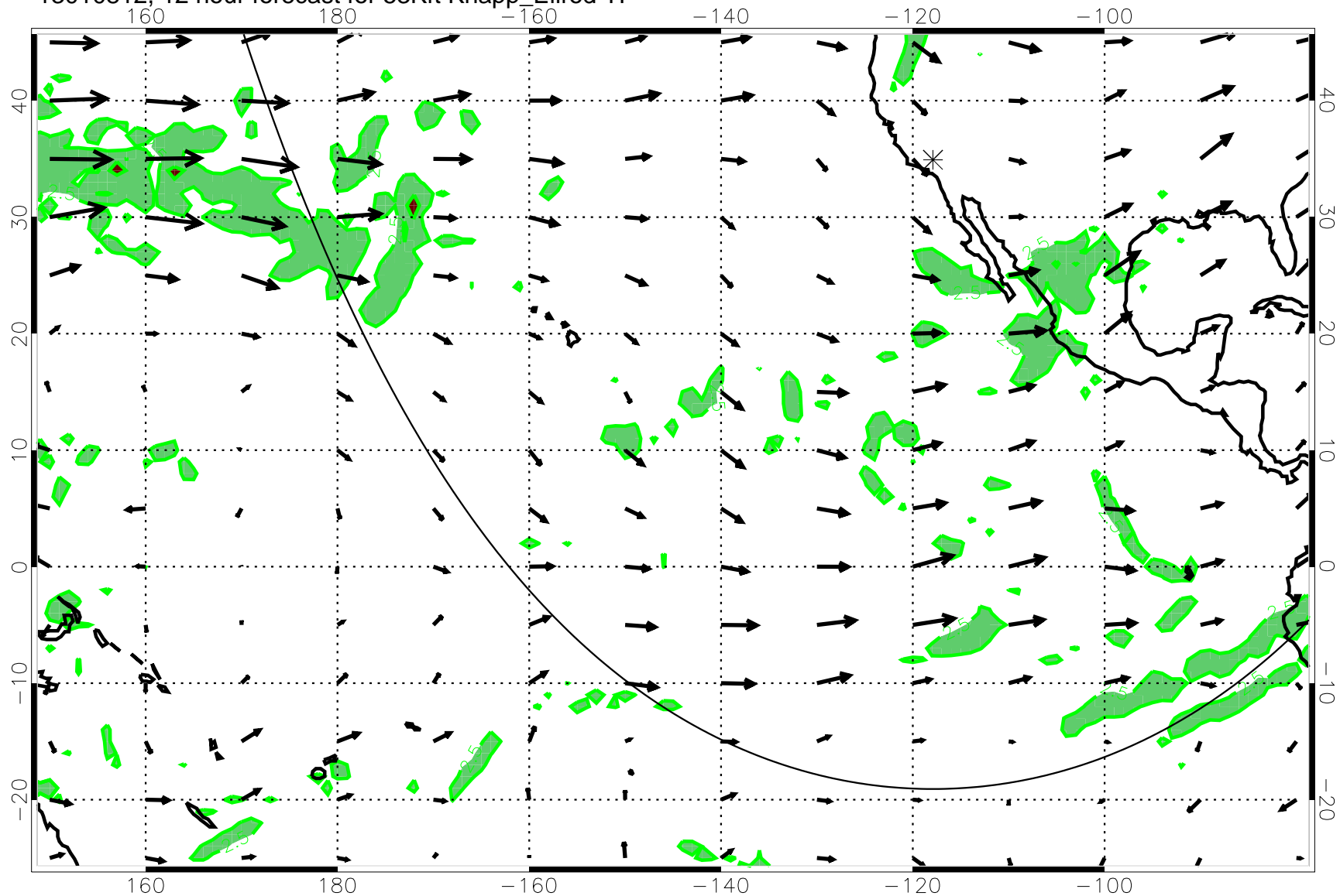
13010812, 12 hour forecast for 53Kft Knapp_Ellrod T1
