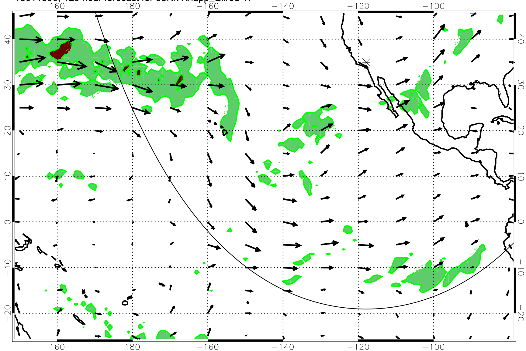
13011300, 120 hour forecast for 53Kft Knapp_Ellrod T1
