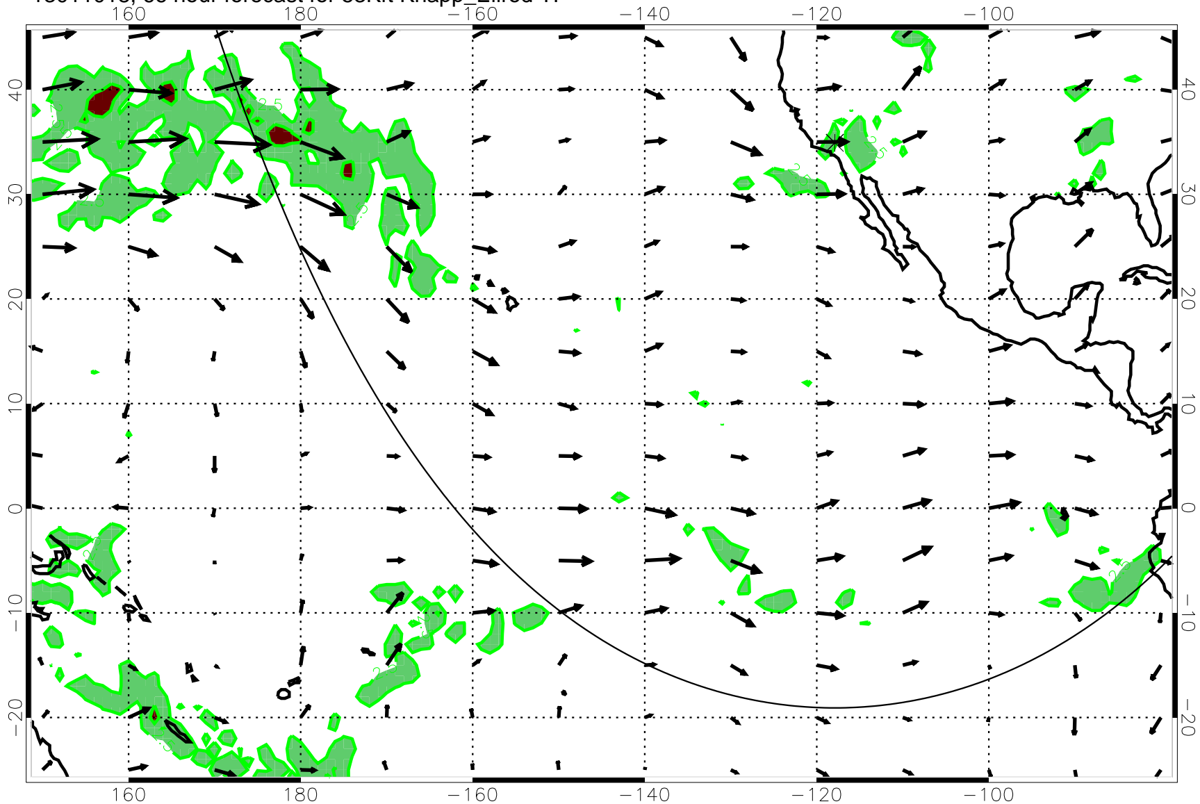
13011018, 66 hour forecast for 53Kft Knapp_Ellrod T1
