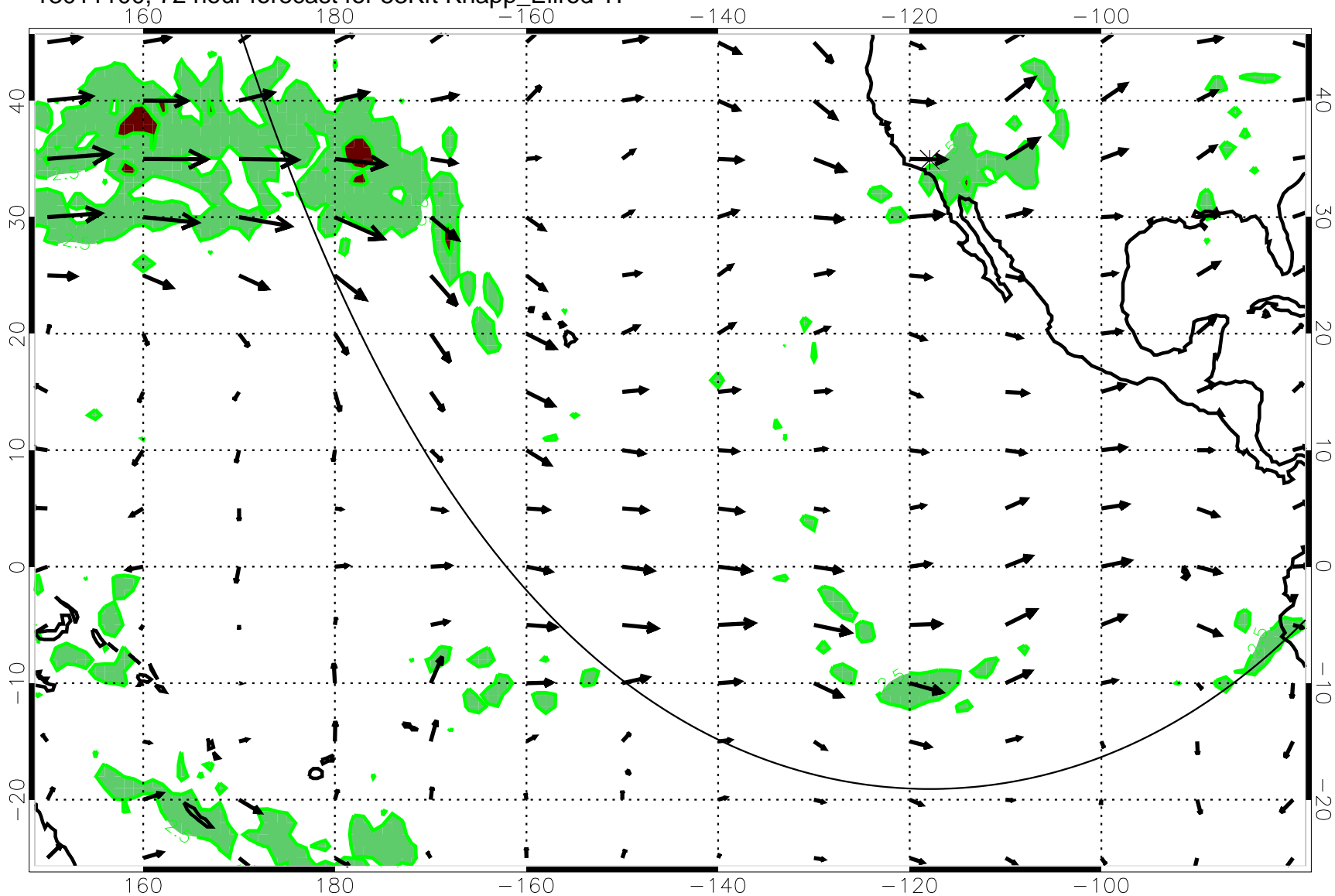
13011100, 72 hour forecast for 53Kft Knapp_Ellrod T1
