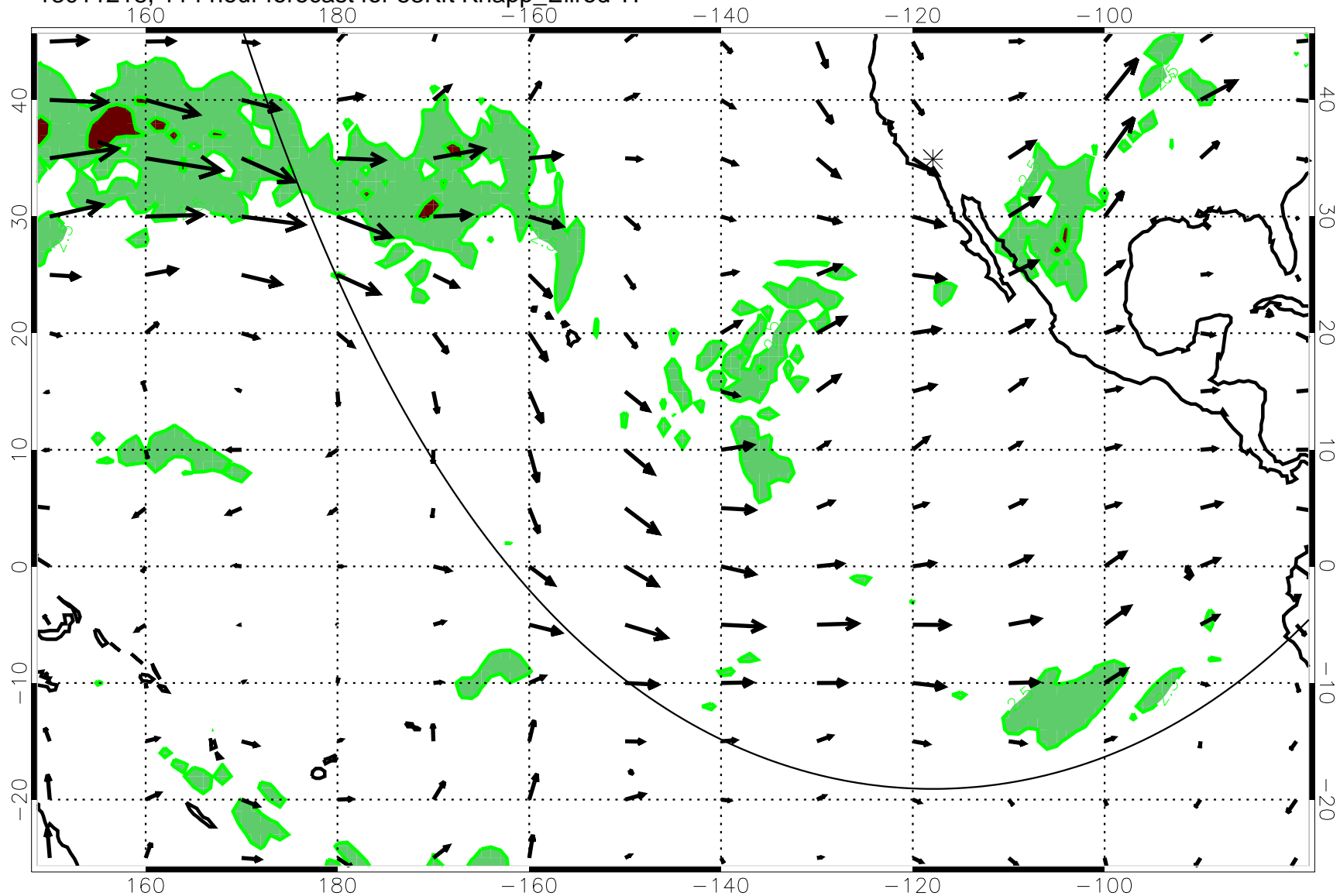
13011218, 114 hour forecast for 53Kft Knapp_Ellrod T1
