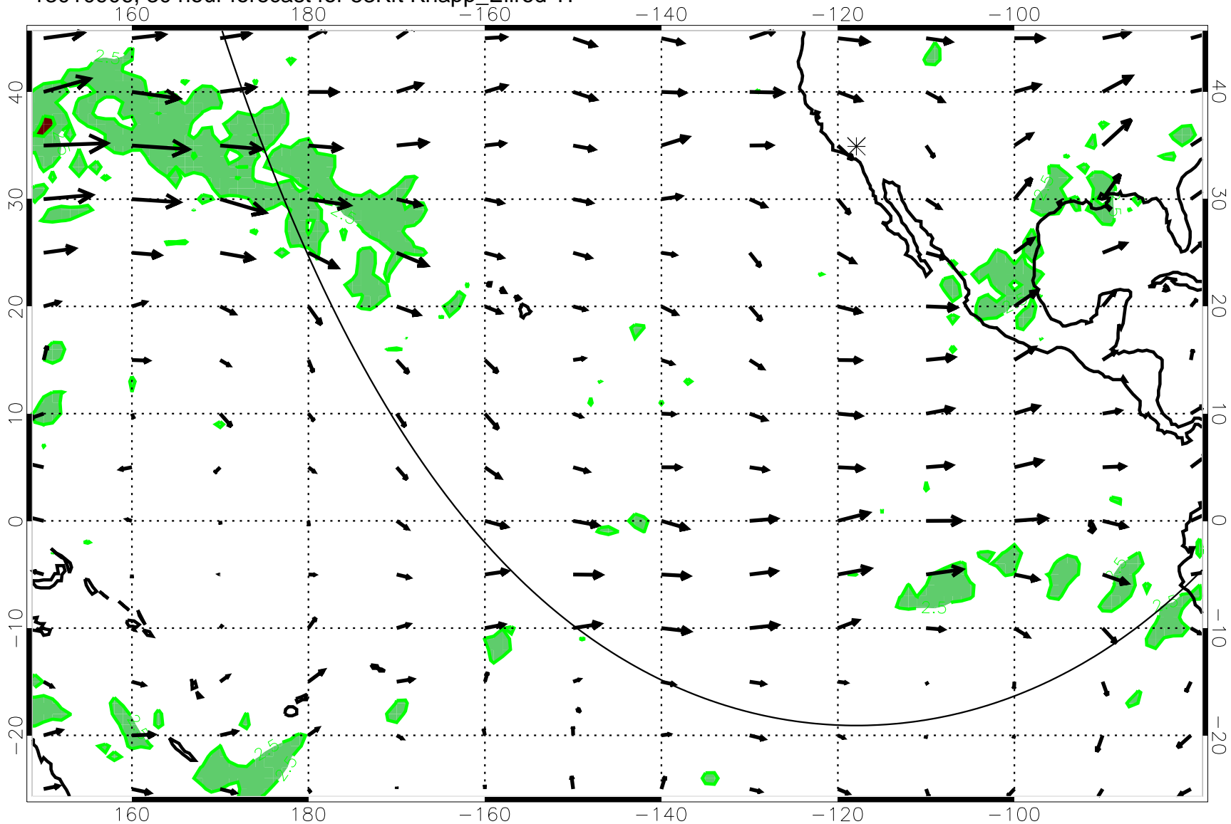
13010906, 30 hour forecast for 53Kft Knapp_Ellrod TI
