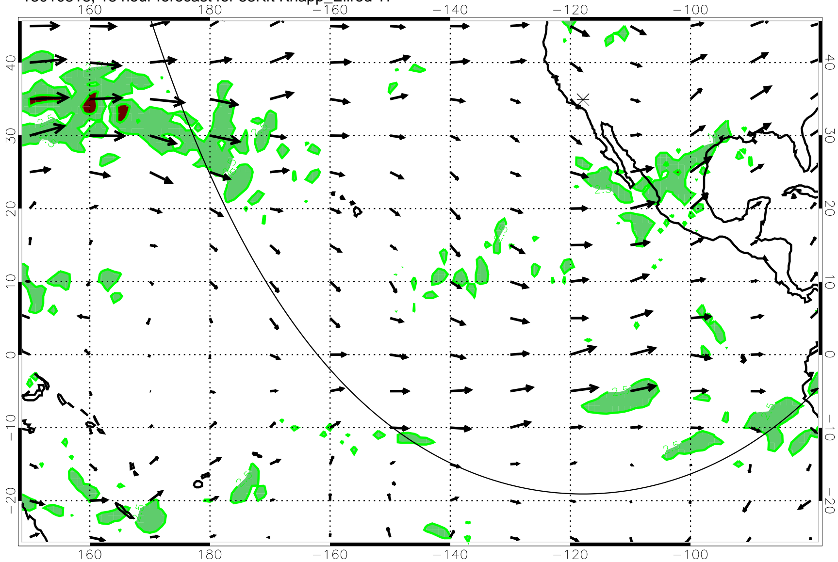
13010818, 18 hour forecast for 53Kft Knapp_Ellrod T1
