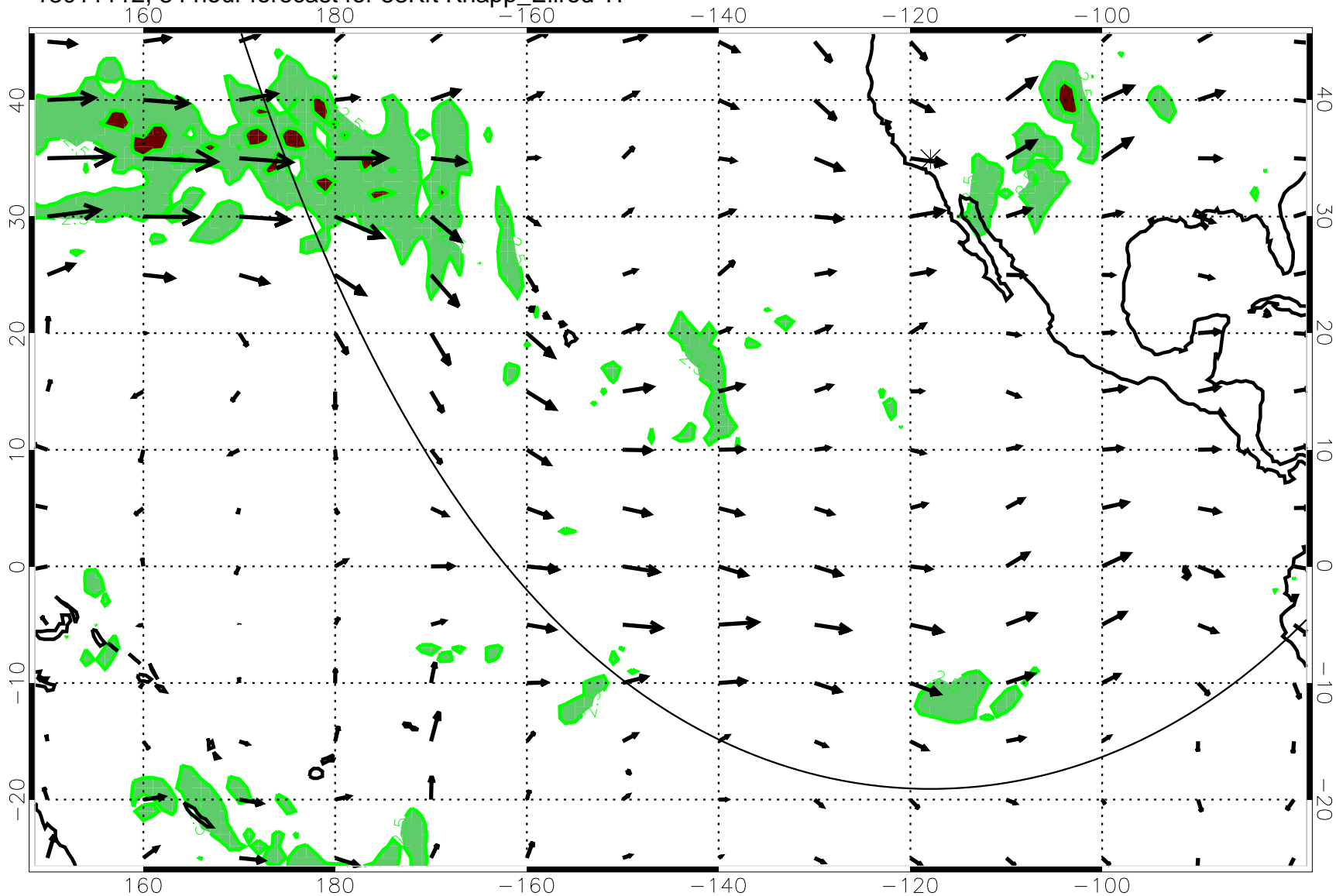
13011112, 84 hour forecast for 53Kft Knapp_Ellrod TI
