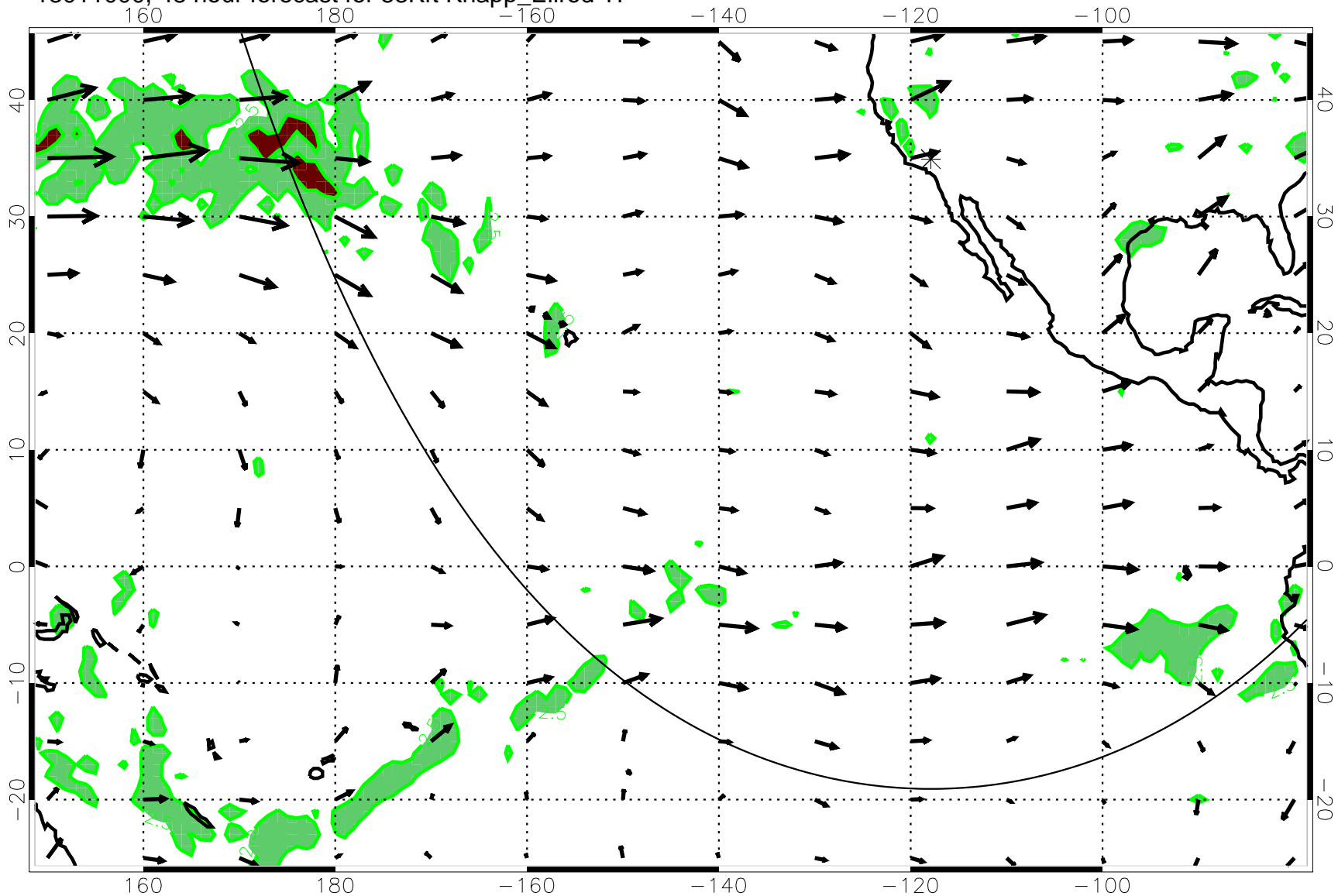
13011000, 48 hour forecast for 53Kft Knapp_Ellrod T1
