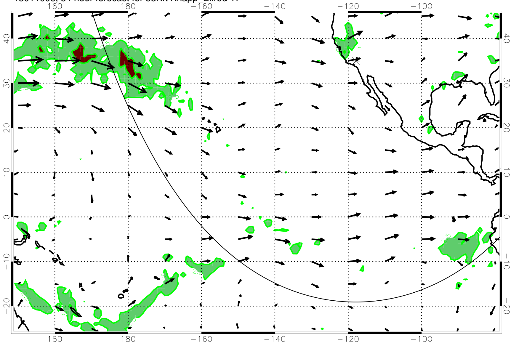
13011006, 54 hour forecast for 53Kft Knapp_Ellrod T1
