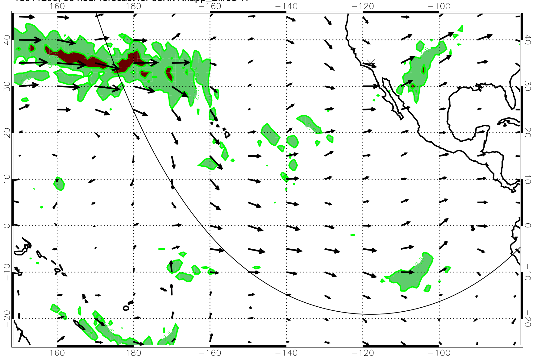
13011200, 96 hour forecast for 53Kft Knapp_Ellrod T1
