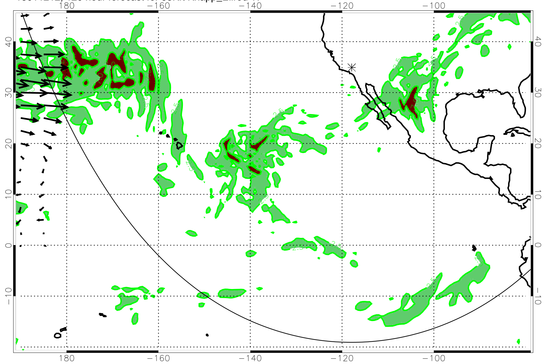
13011212, 120 hour forecast for 53Kft Knapp_Ellrod T1
