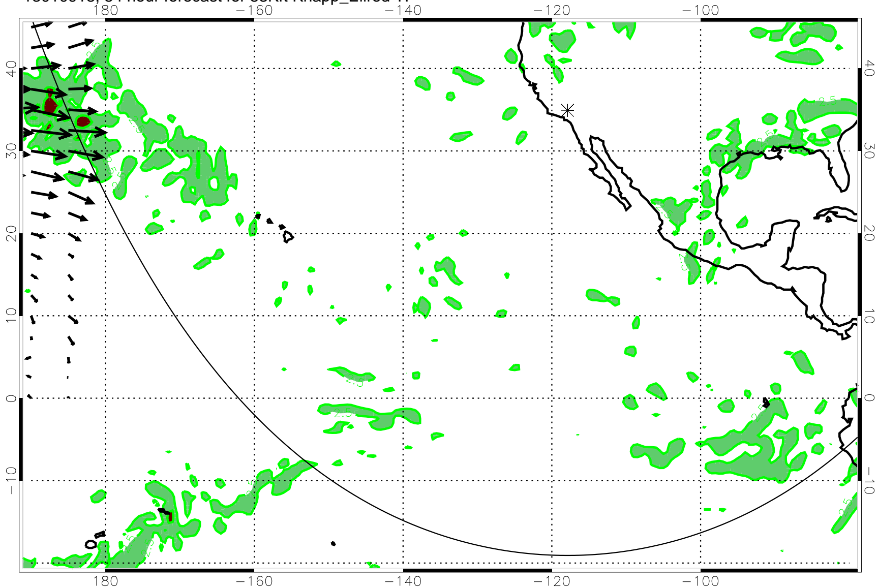
13010918, 54 hour forecast for 53Kft Knapp_Ellrod TI
