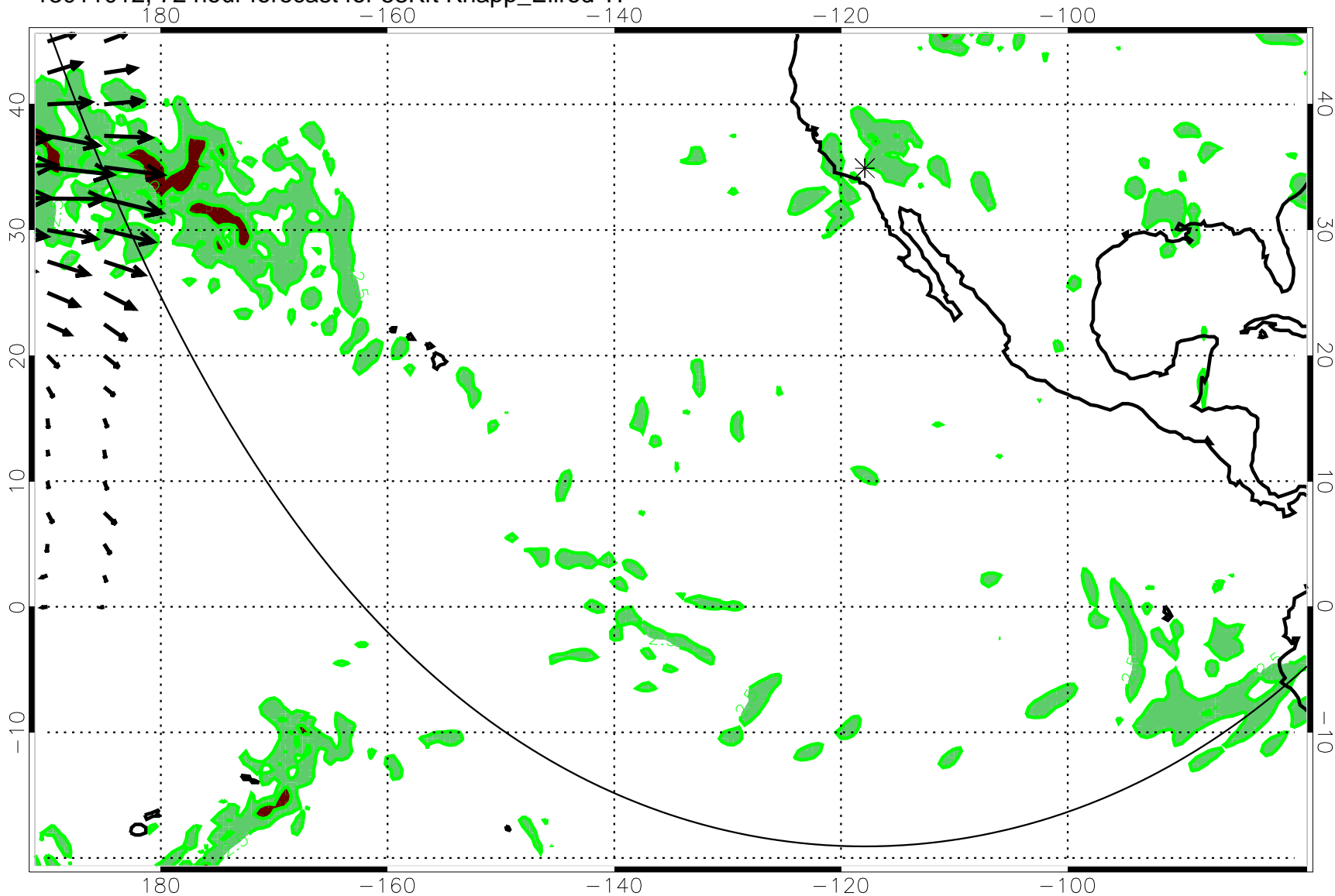
13011012, 72 hour forecast for 53Kft Knapp_Ellrod TI
