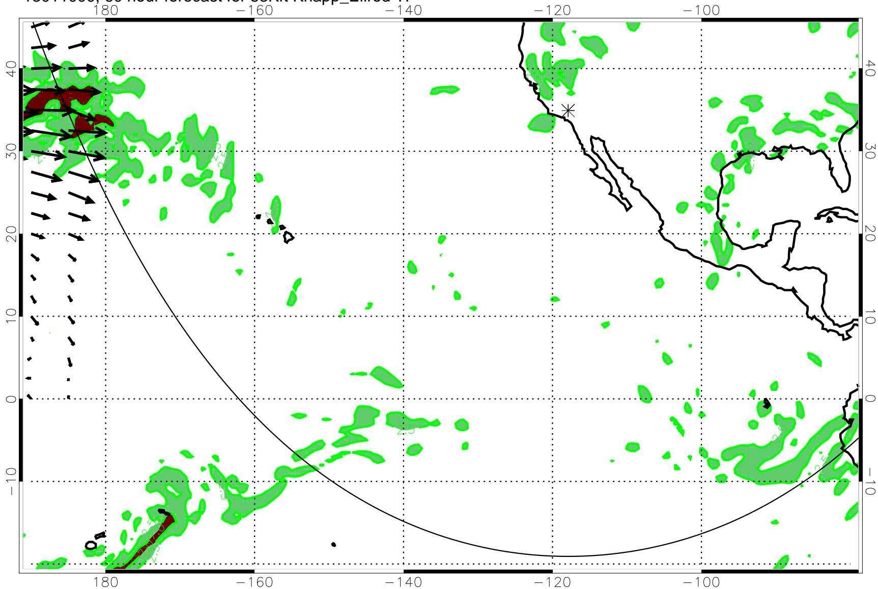
13011000, 60 hour forecast for 53Kft Knapp_Ellrod TI
