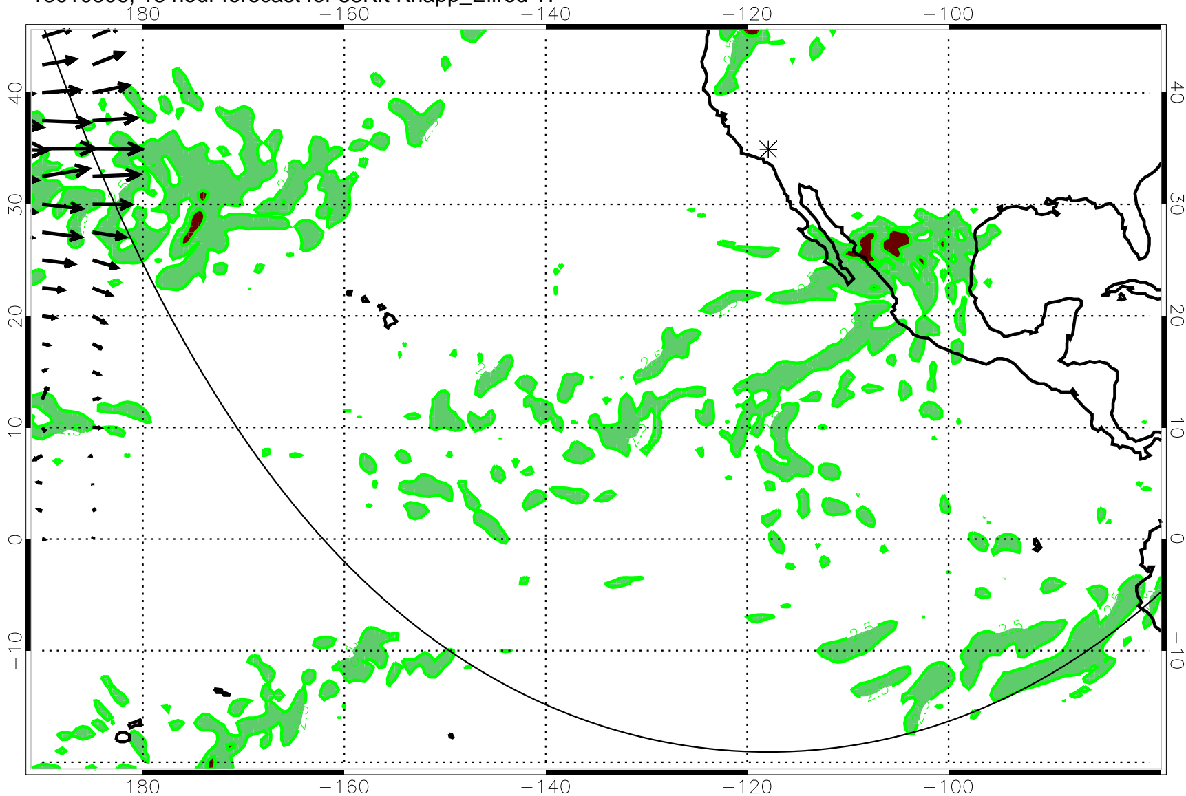
13010806, 18 hour forecast for 53Kft Knapp_Ellrod TI
