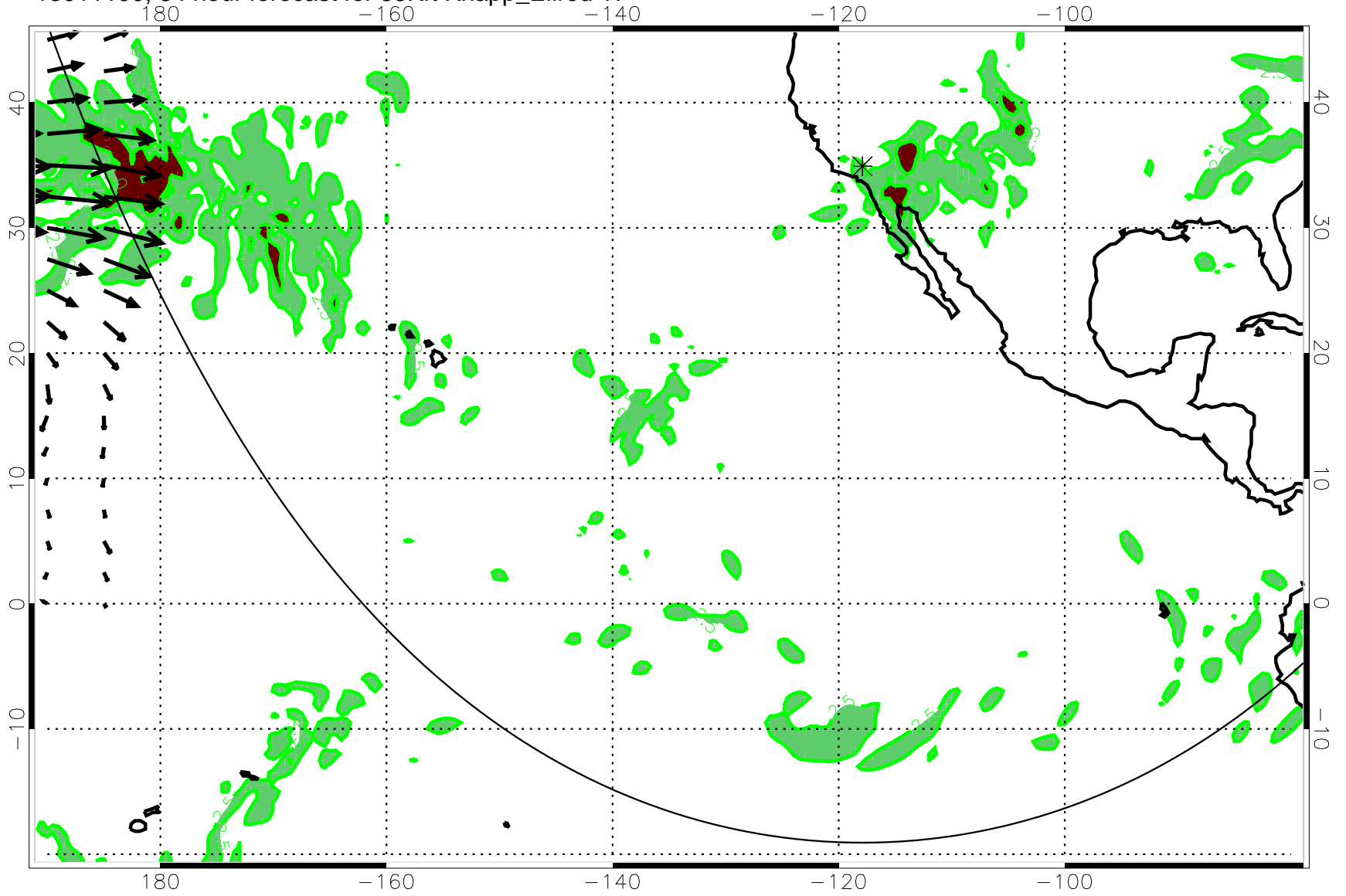
13011100, 84 hour forecast for 53Kft Knapp_Ellrod TI
