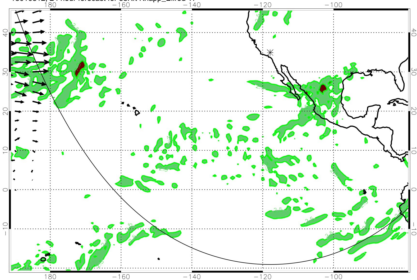
13010812, 24 hour forecast for 53Kft Knapp_Ellrod TI
