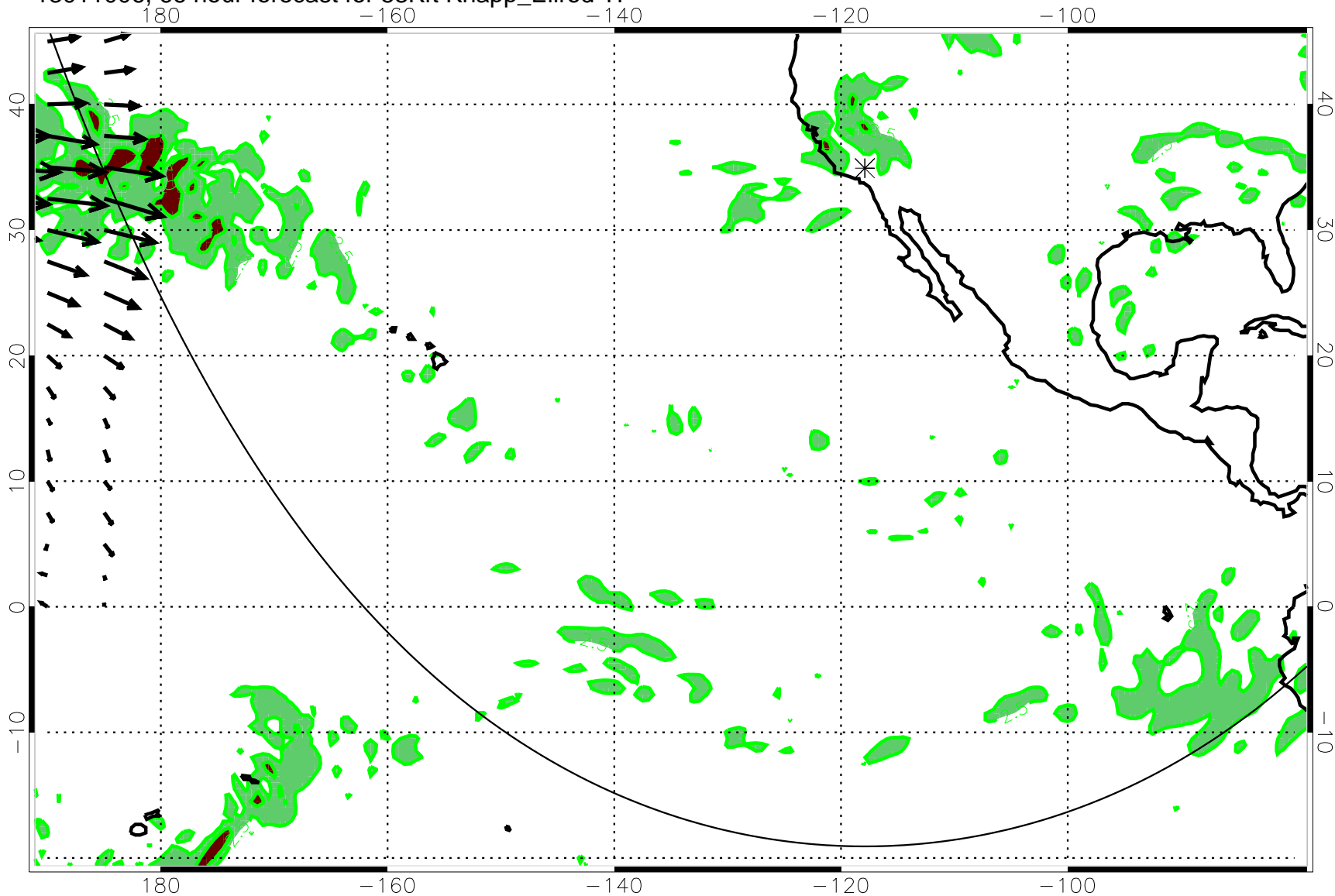
13011006, 66 hour forecast for 53Kft Knapp_Ellrod TI
