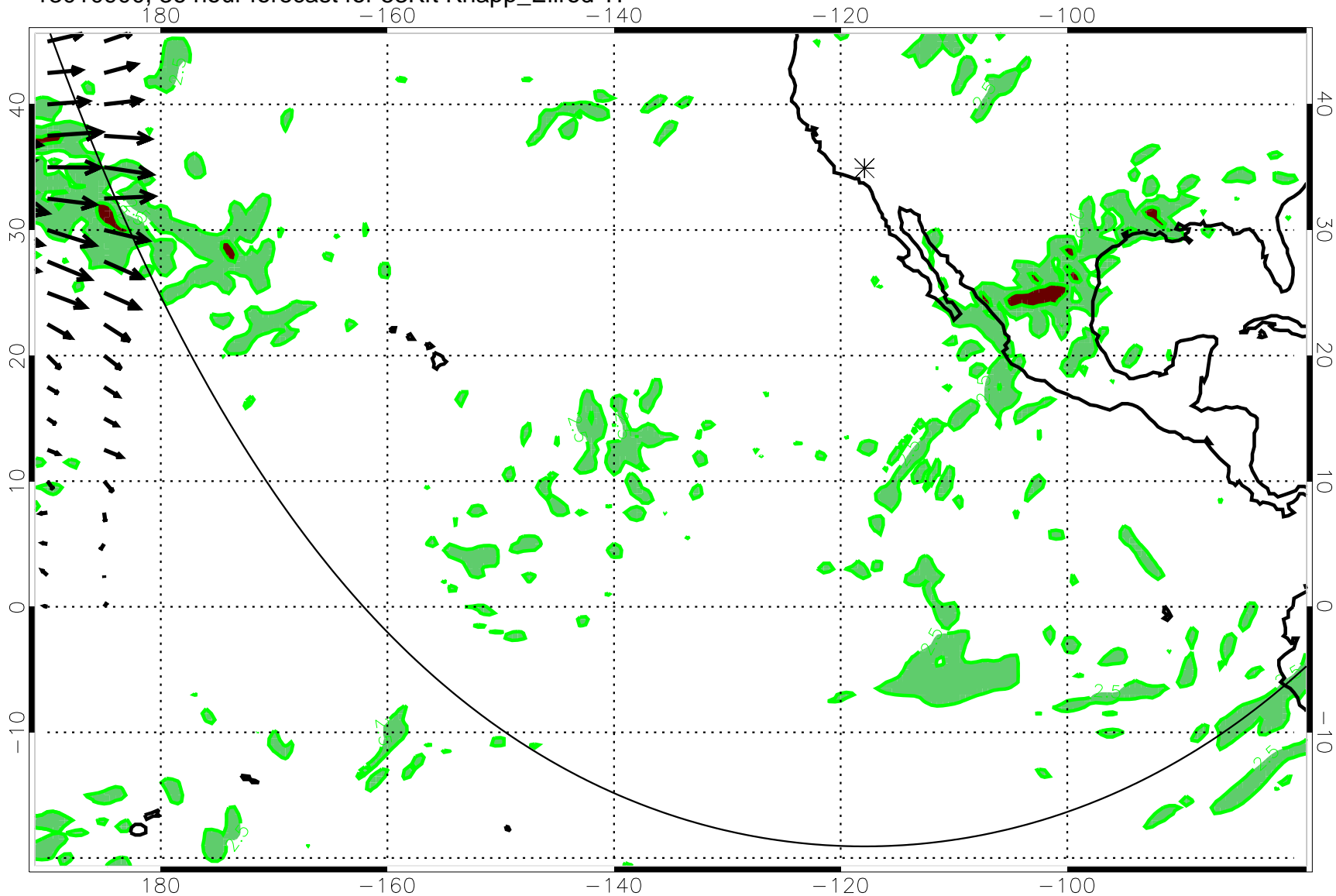
13010900, 36 hour forecast for 53Kft Knapp_Ellrod TI
