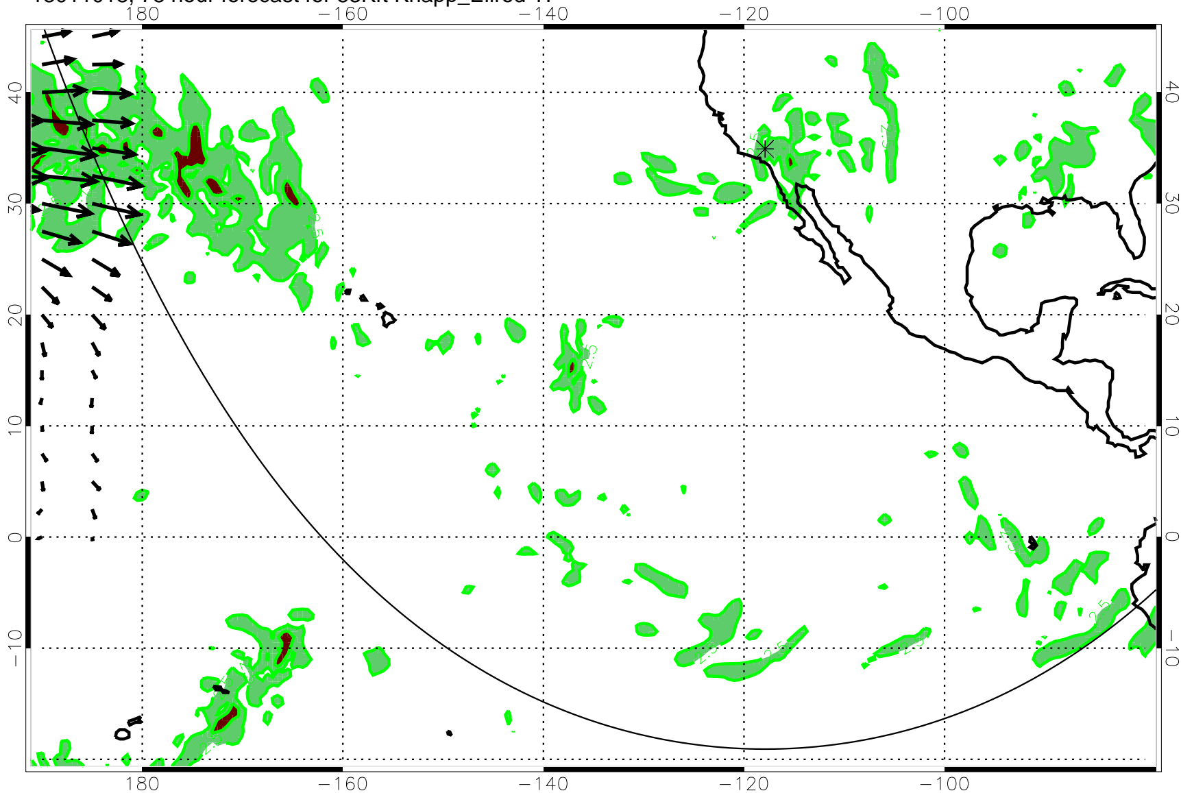
13011018, 78 hour forecast for 53Kft Knapp_Ellrod TI
