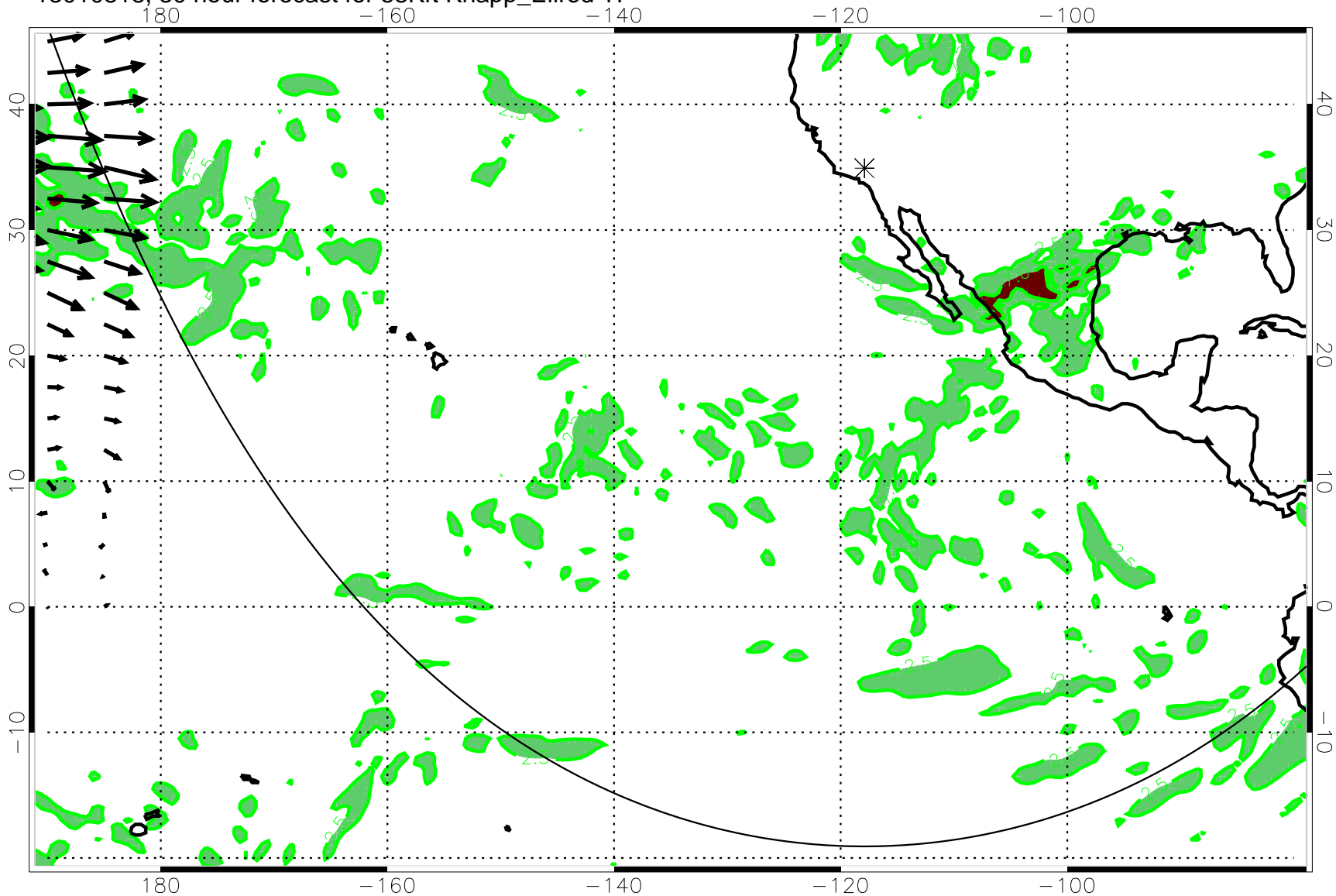
13010818, 30 hour forecast for 53Kft Knapp_Ellrod TI
