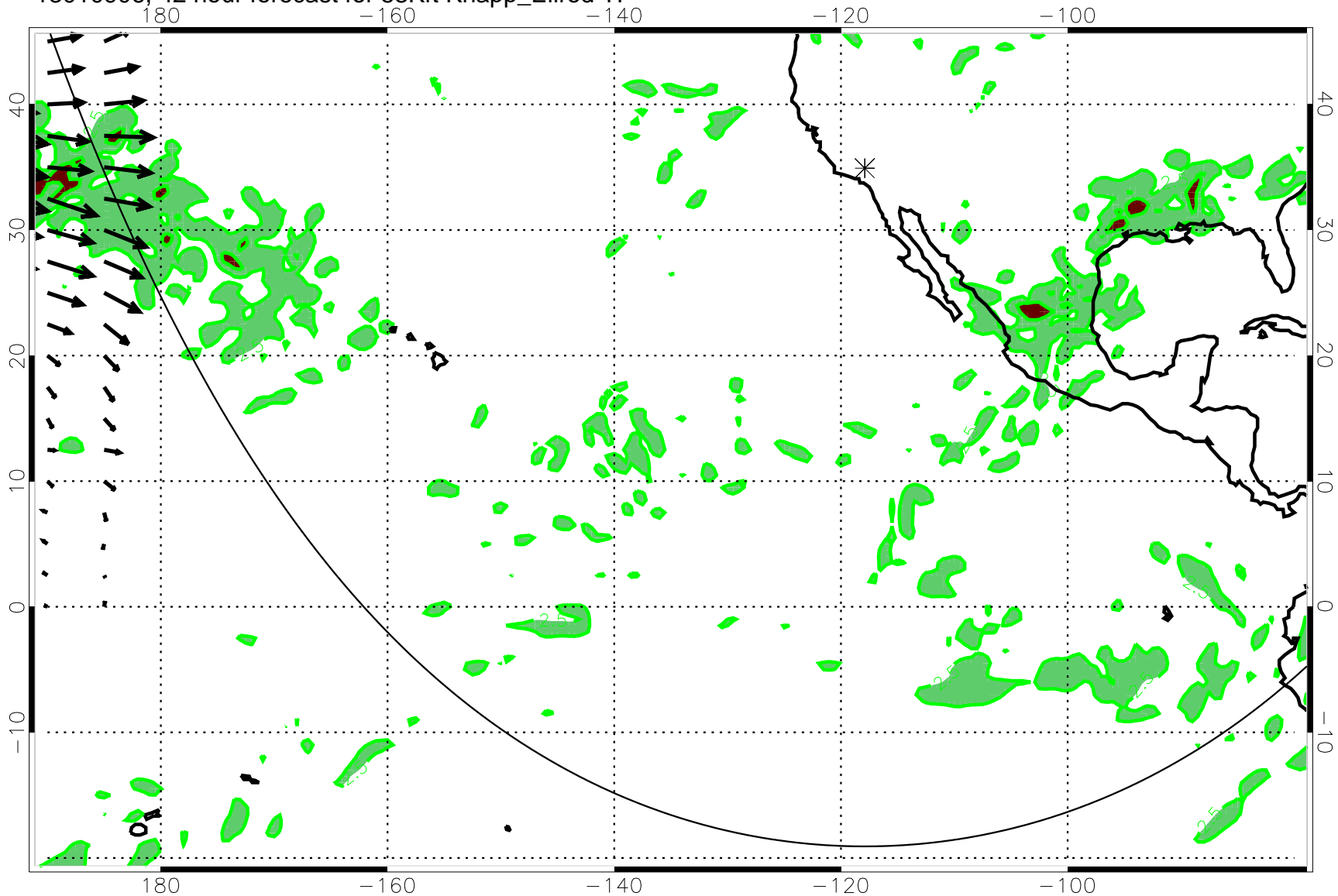
13010906, 42 hour forecast for 53Kft Knapp_Ellrod TI
