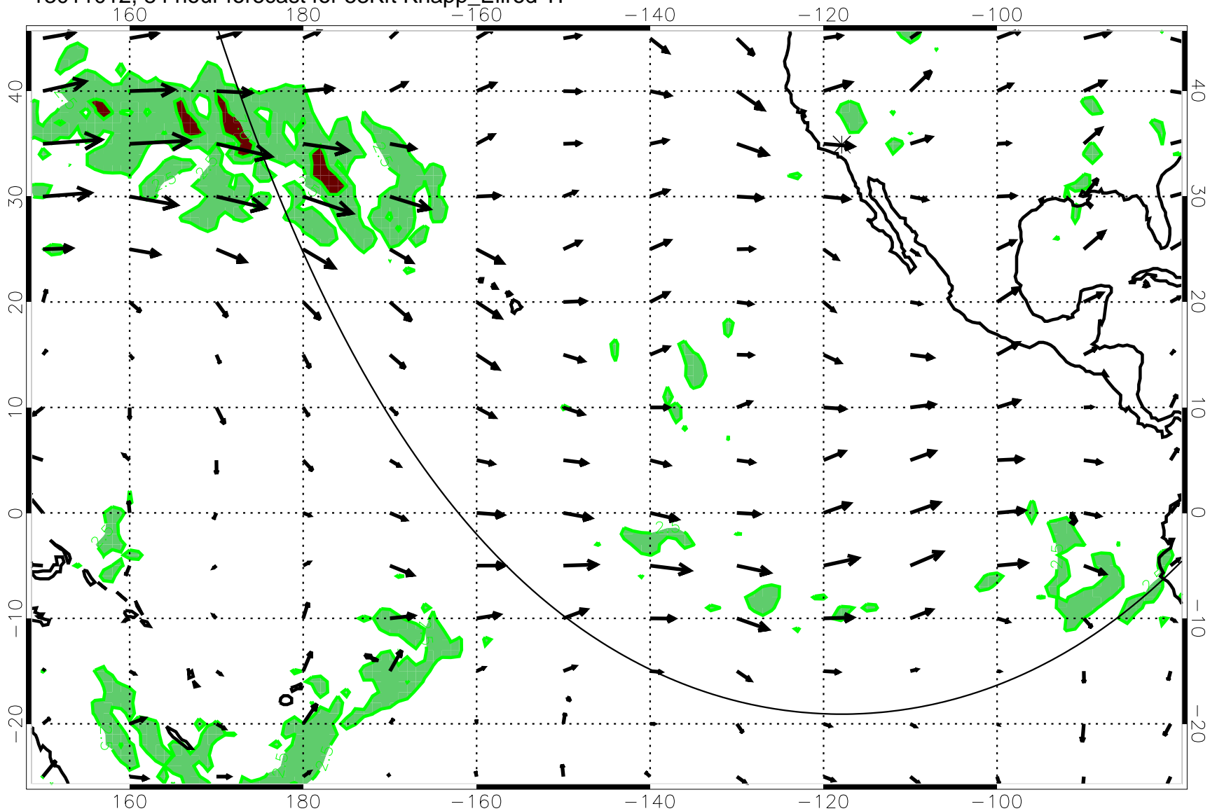
13011012, 84 hour forecast for 53Kft Knapp_Ellrod Tl
