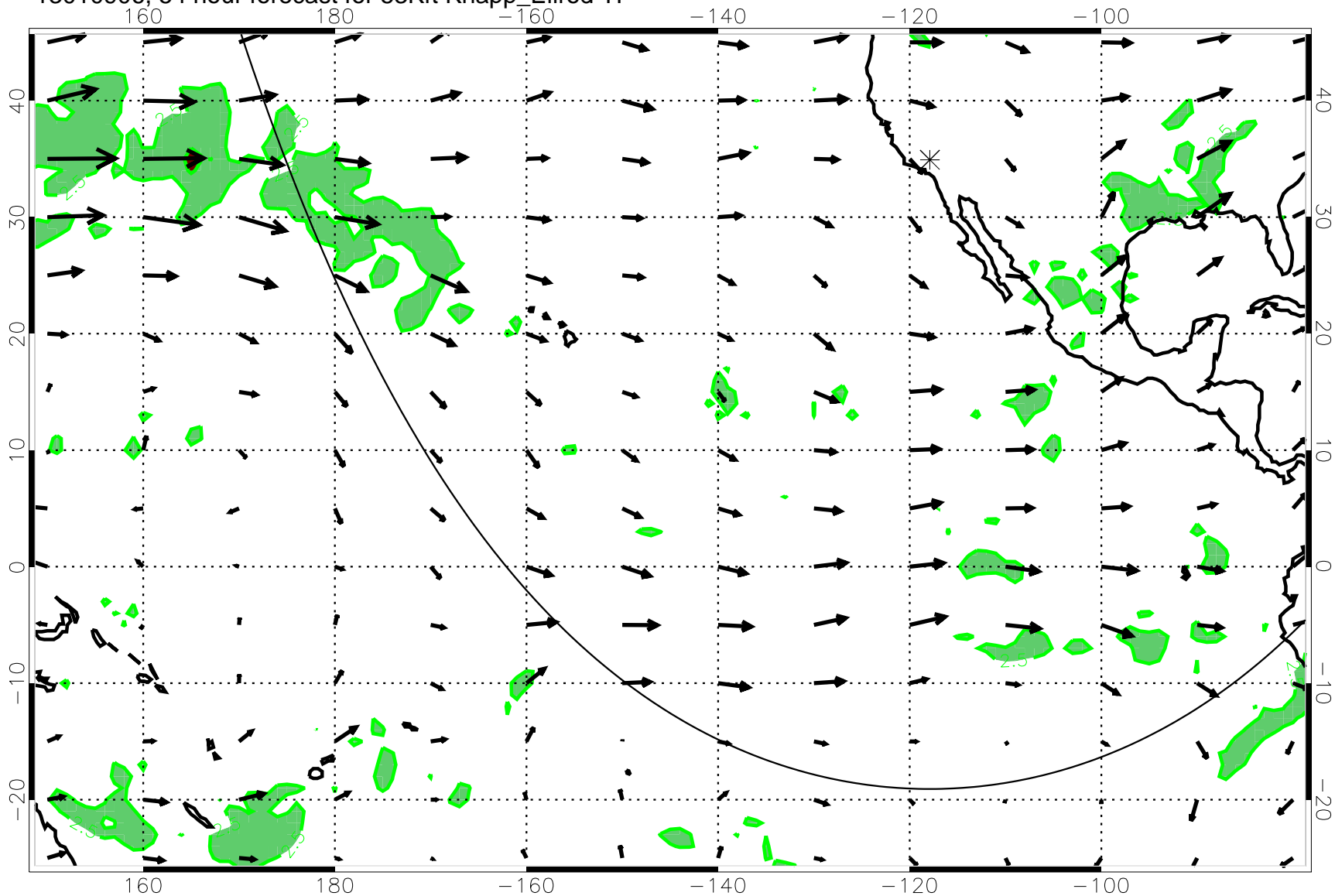
13010906, 54 hour forecast for 53Kft Knapp_Ellrod T1
