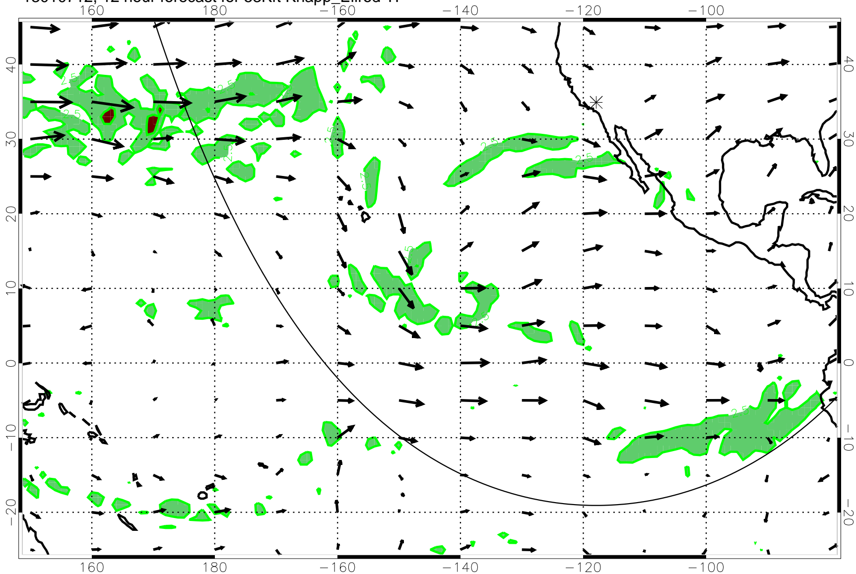
13010712, 12 hour forecast for 53Kft Knapp_Ellrod T1
