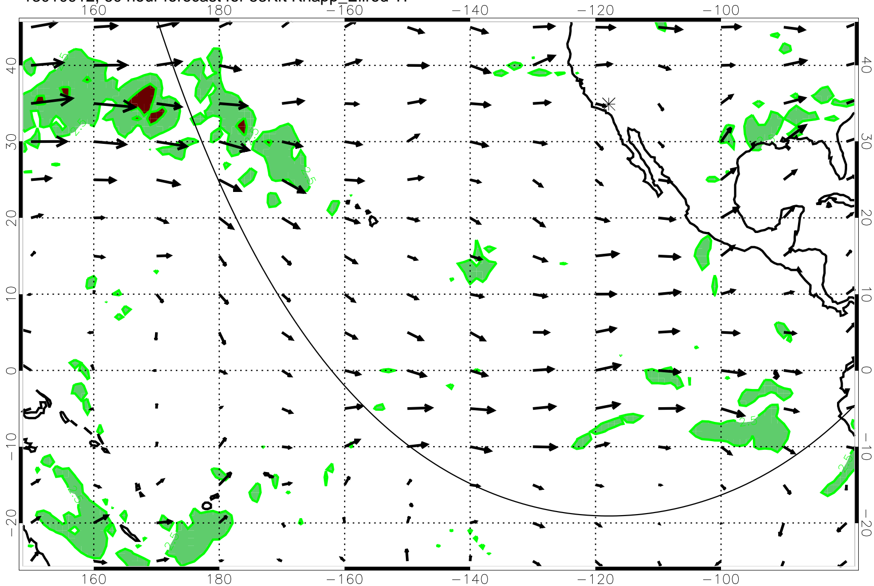
13010912, 60 hour forecast for 53Kft Knapp_Ellrod T1
