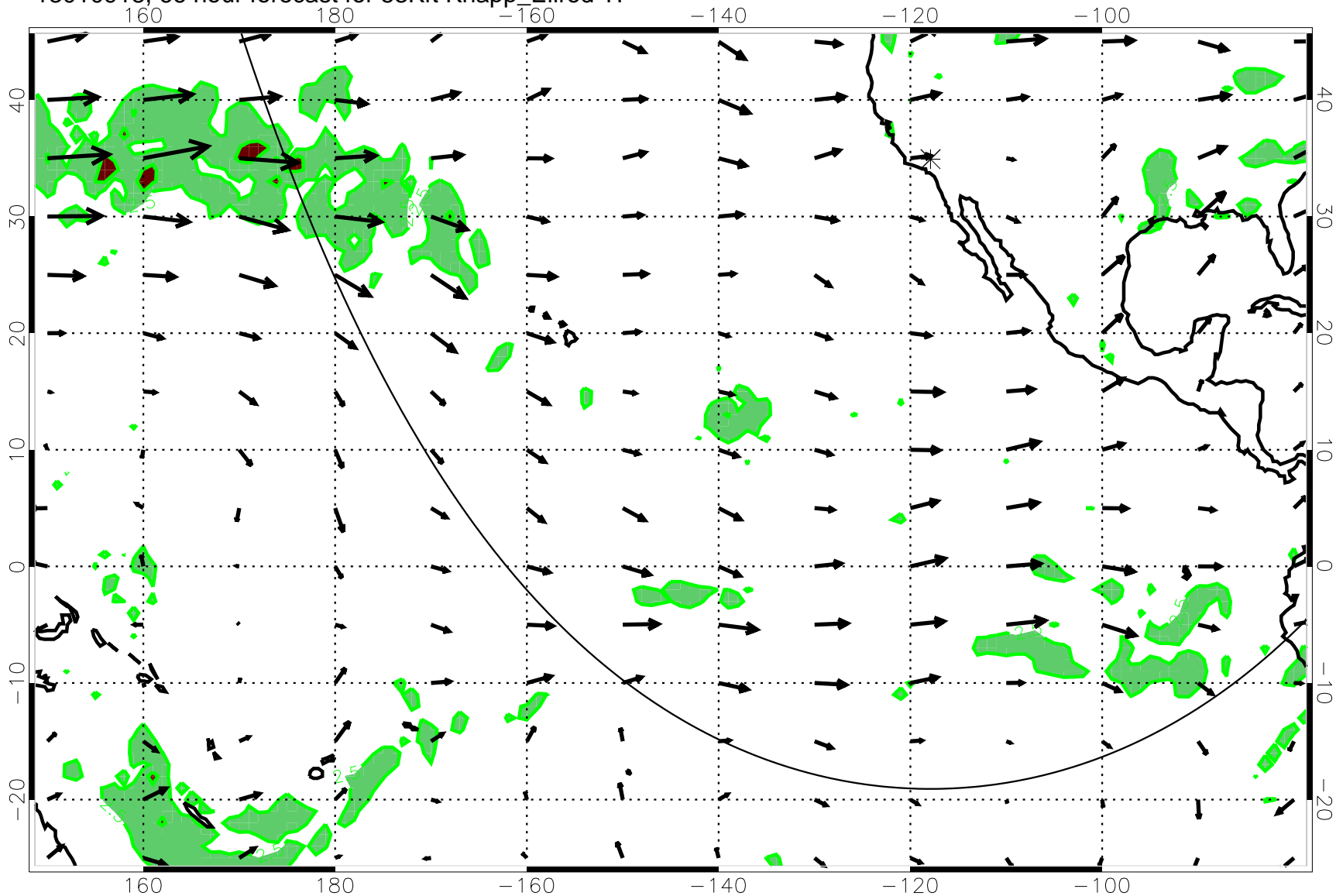
13010918, 66 hour forecast for 53Kft Knapp_Ellrod T1
