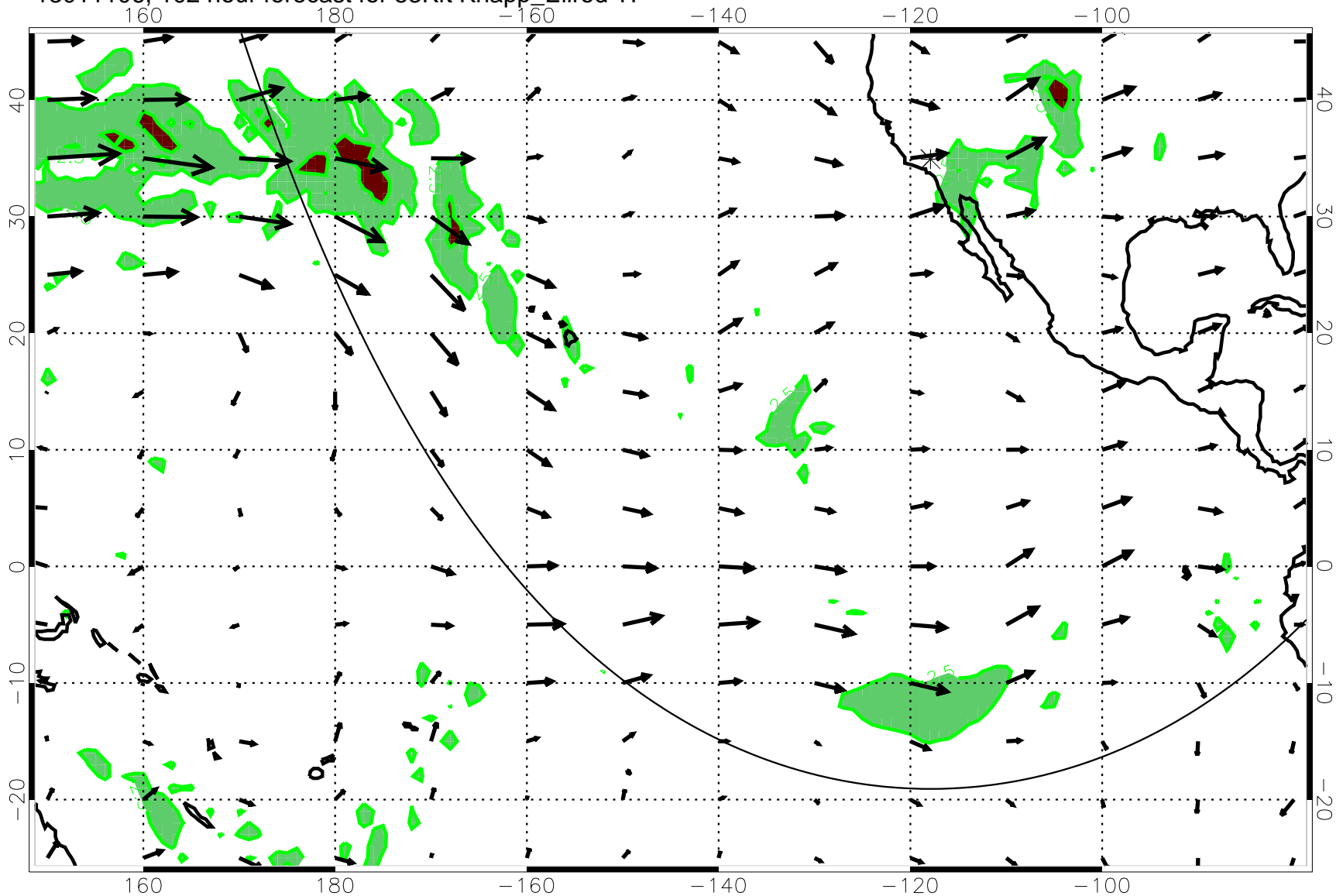
13011106, 102 hour forecast for 53Kft Knapp_Ellrod T1
