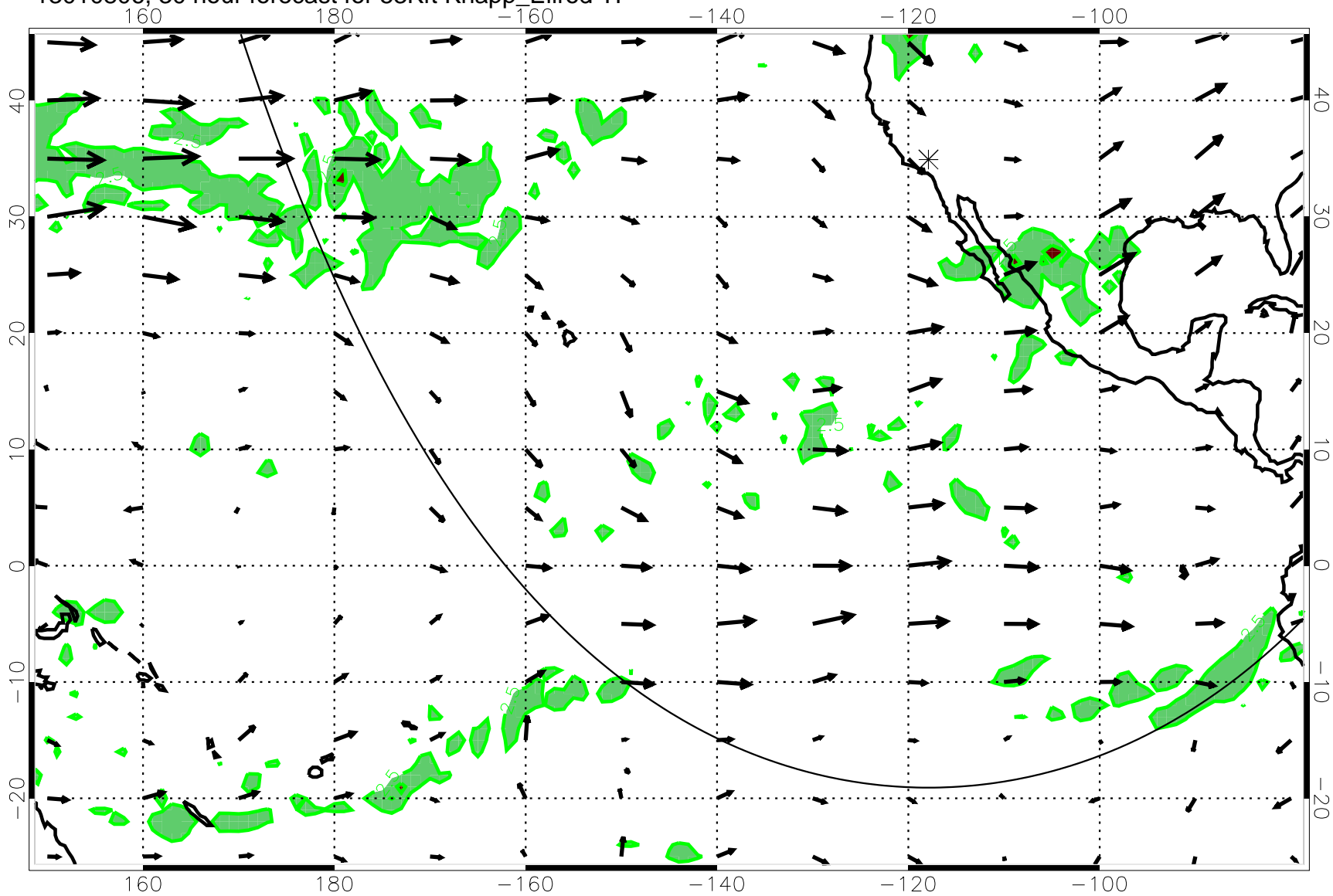
13010806, 30 hour forecast for 53Kft Knapp_Ellrod TI
