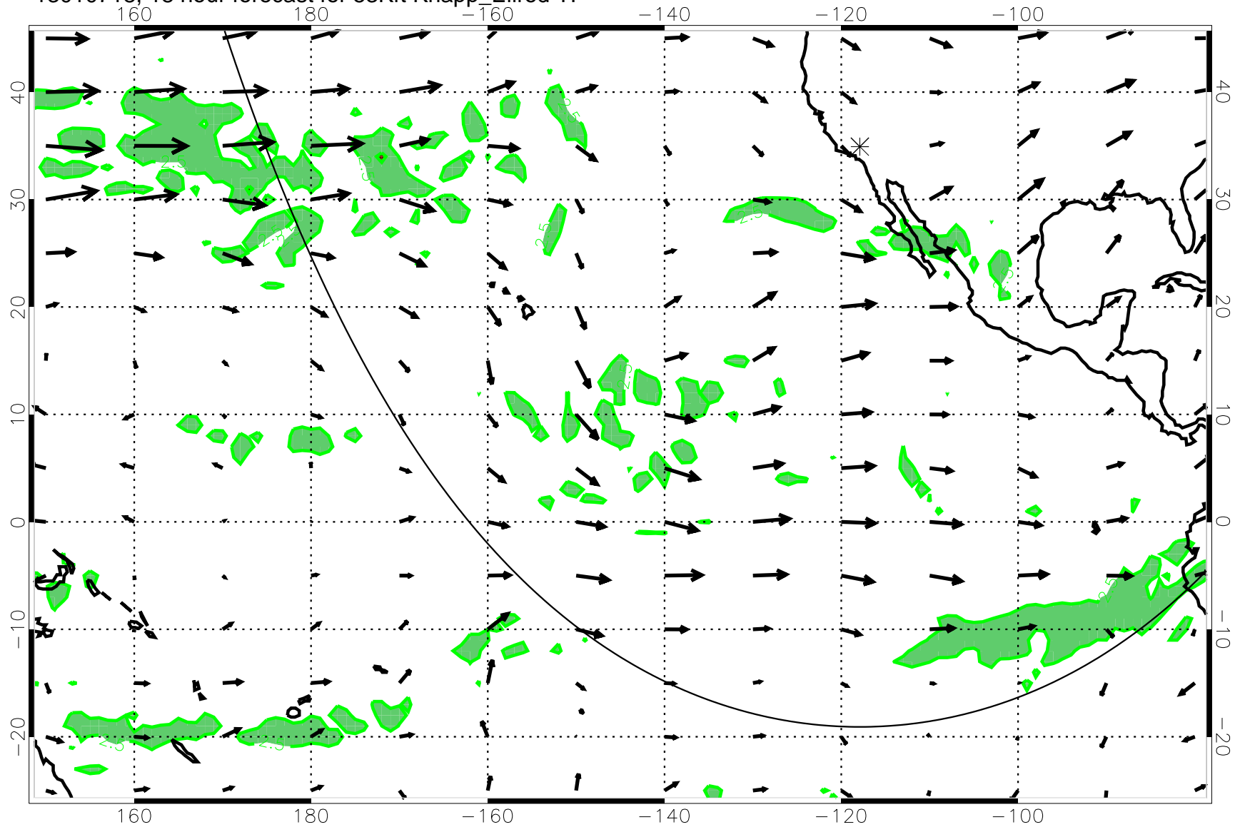
13010718, 18 hour forecast for 53Kft Knapp_Ellrod TI
