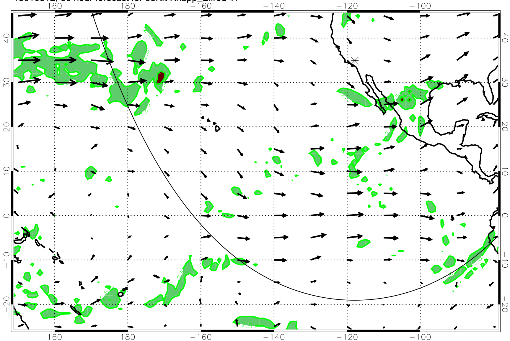
13010812, 36 hour forecast for 53Kft Knapp_Ellrod TI
