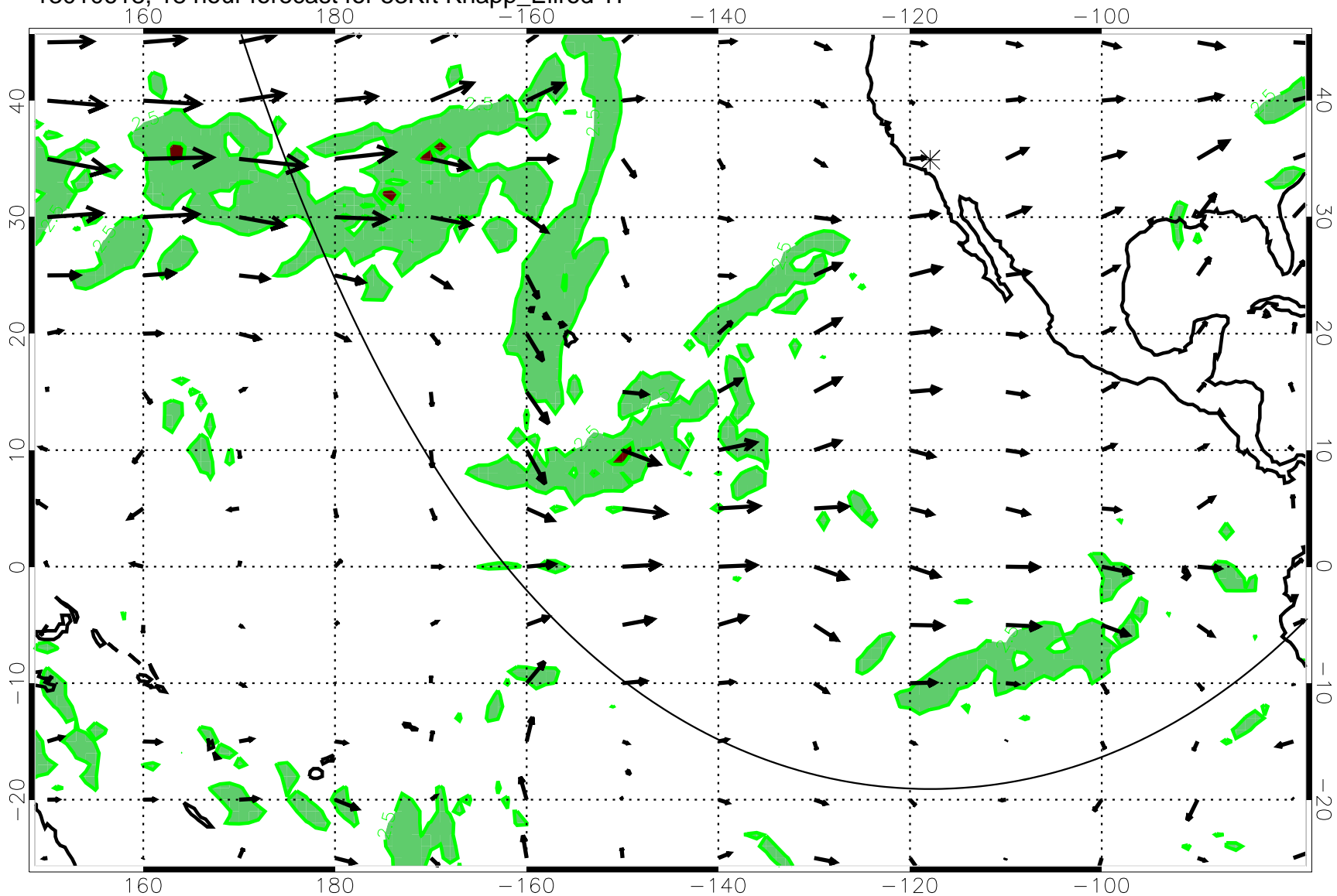
13010618, 18 hour forecast for 53Kft Knapp_Ellrod T1
