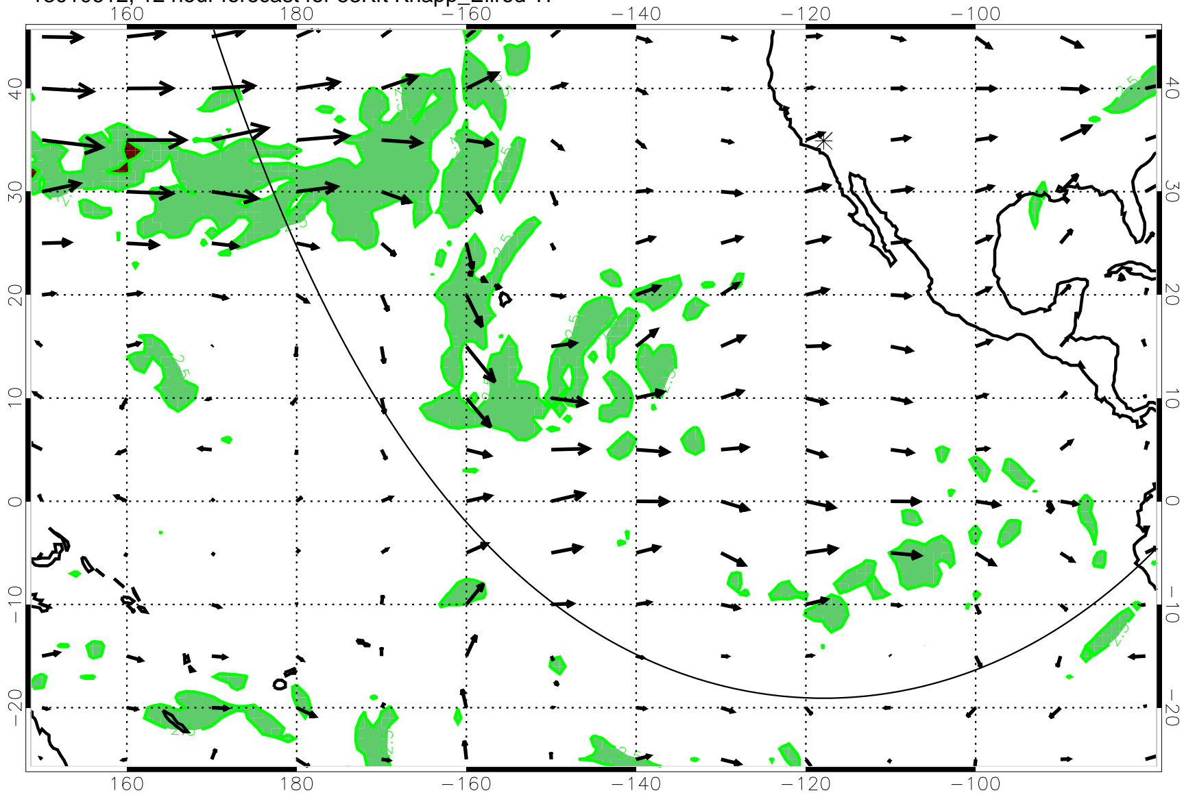
13010612, 12 hour forecast for 53Kft Knapp_Ellrod T1
