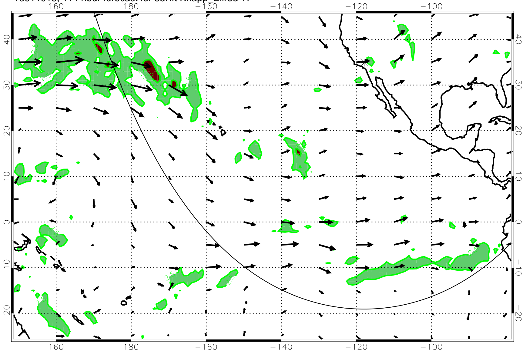
13011018, 114 hour forecast for 53Kft Knapp_Ellrod T1
