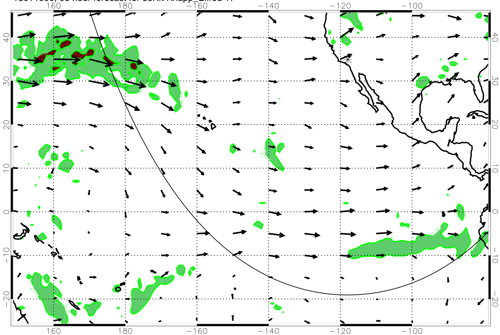
13011000, 96 hour forecast for 53Kft Knapp_Ellrod T1
