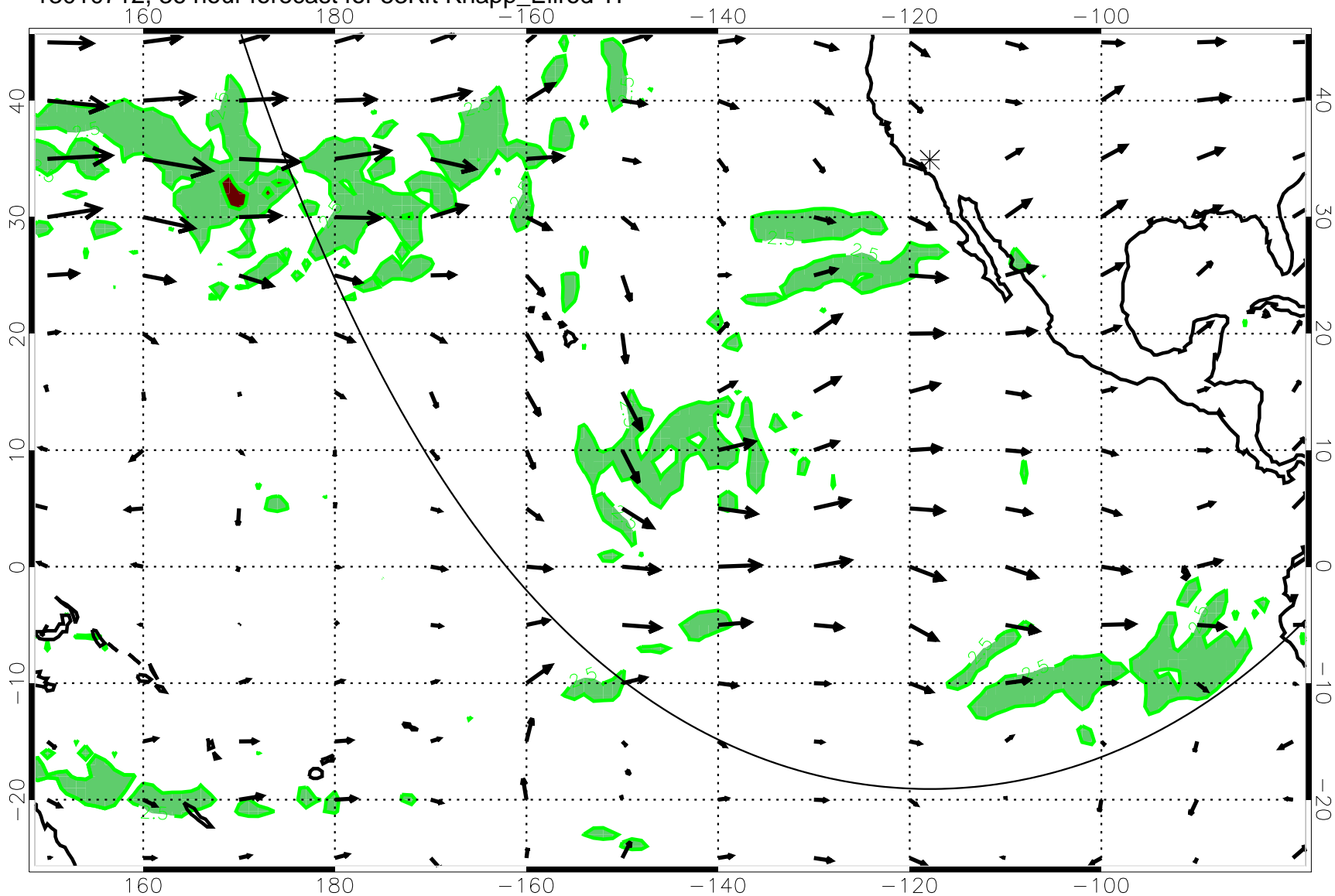
13010712, 36 hour forecast for 53Kft Knapp_Ellrod Tl
