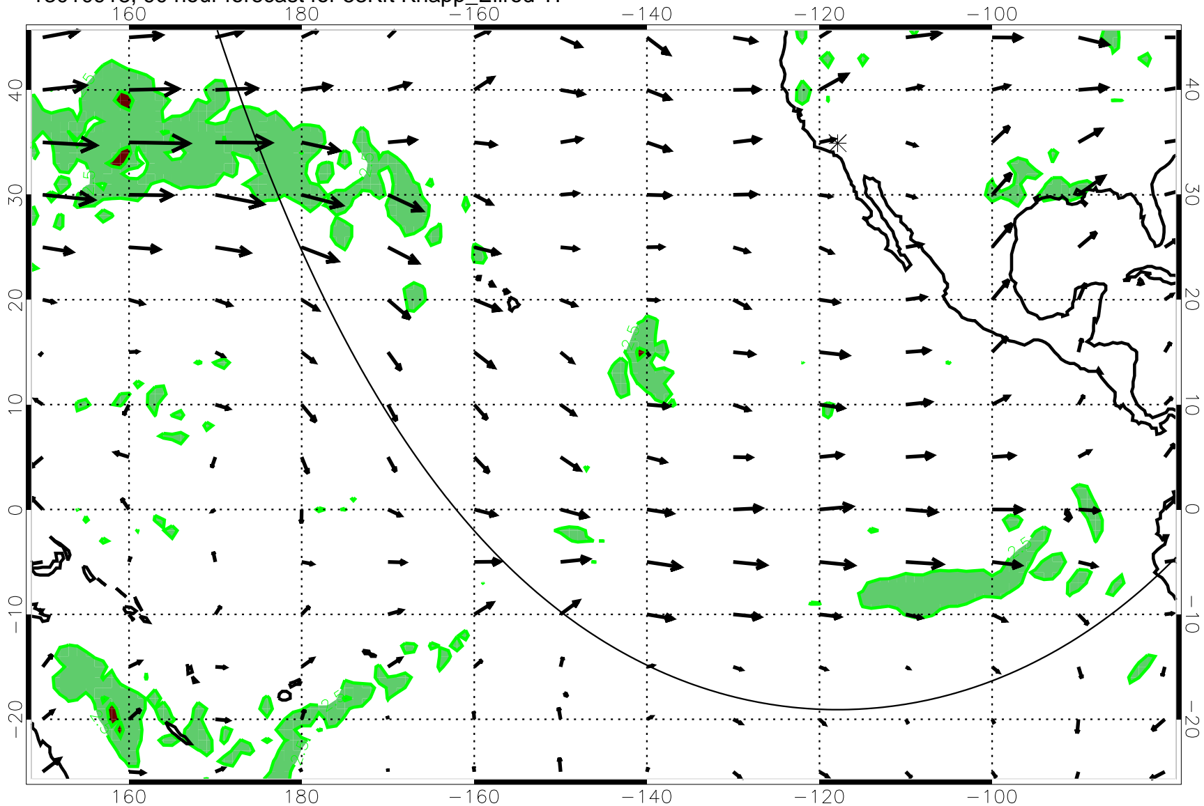
13010918, 90 hour forecast for 53Kft Knapp_Ellrod T1
