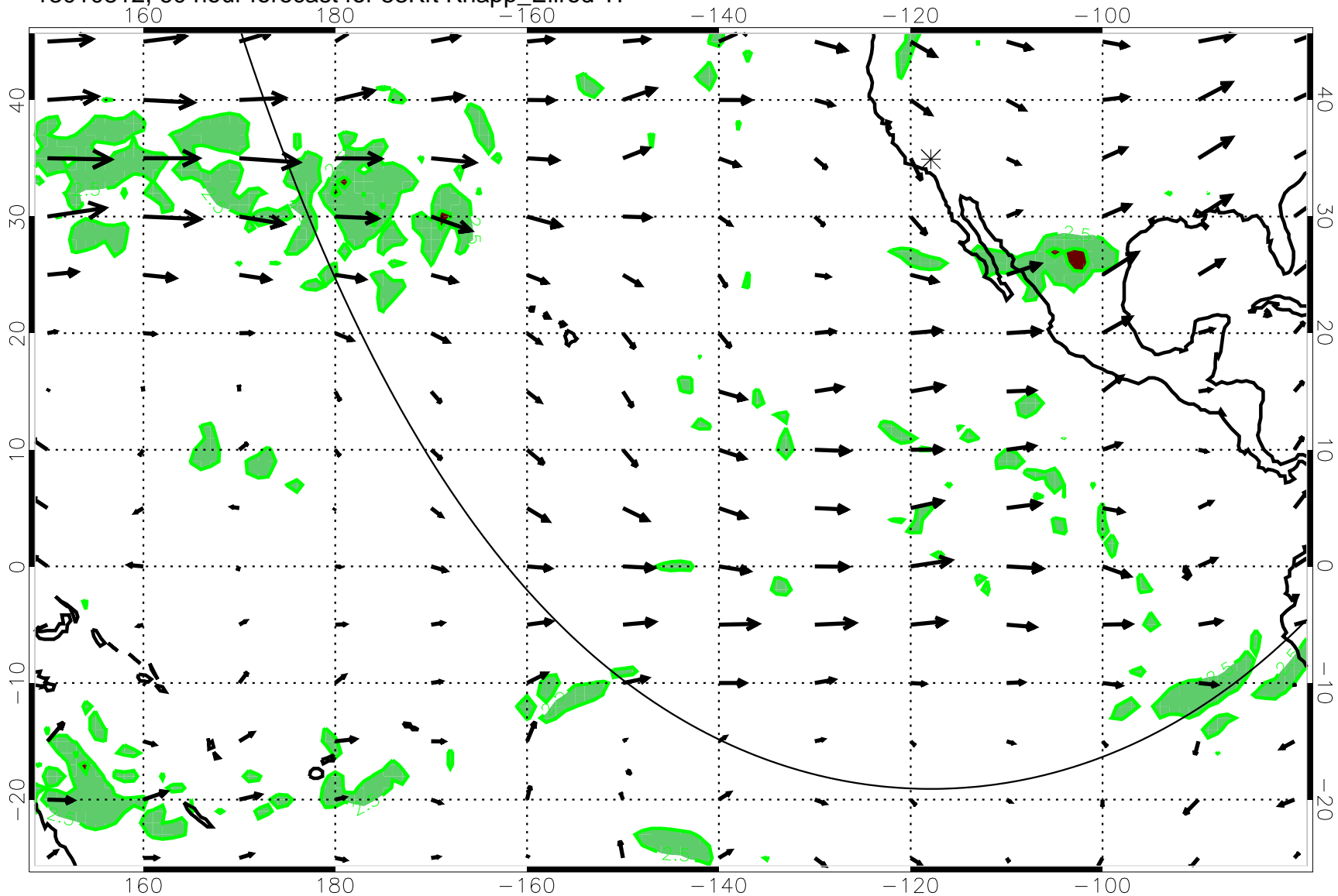
13010812, 60 hour forecast for 53Kft Knapp_Ellrod T1
