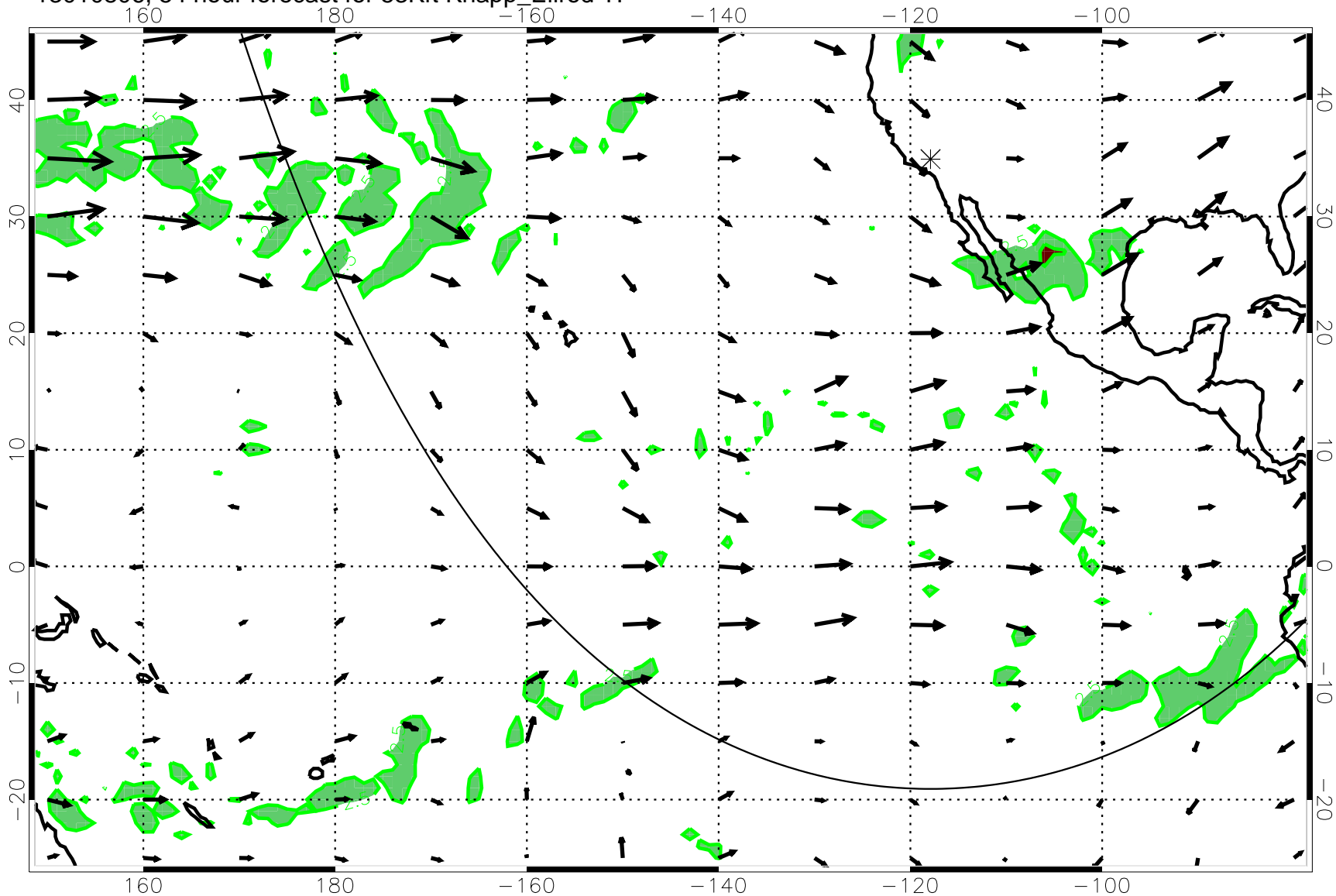
13010806, 54 hour forecast for 53Kft Knapp_Ellrod Tl
