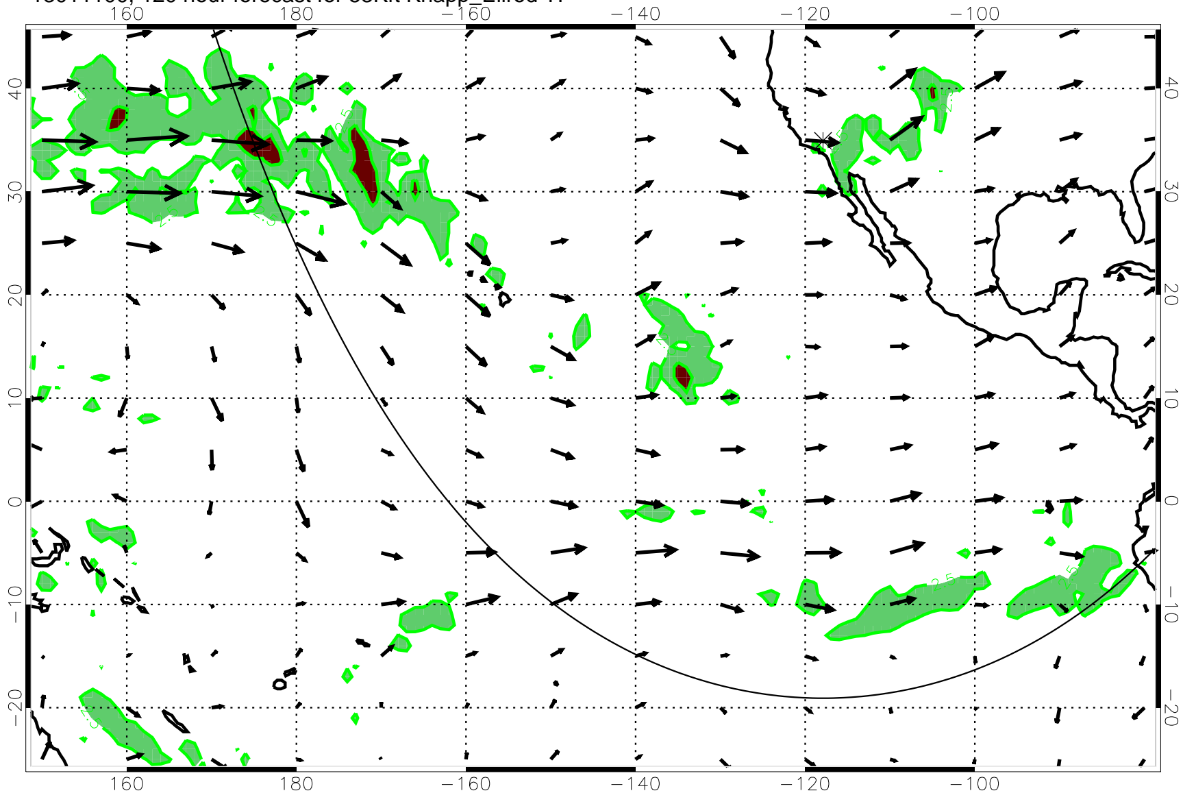
13011100, 120 hour forecast for 53Kft Knapp_Ellrod T1
