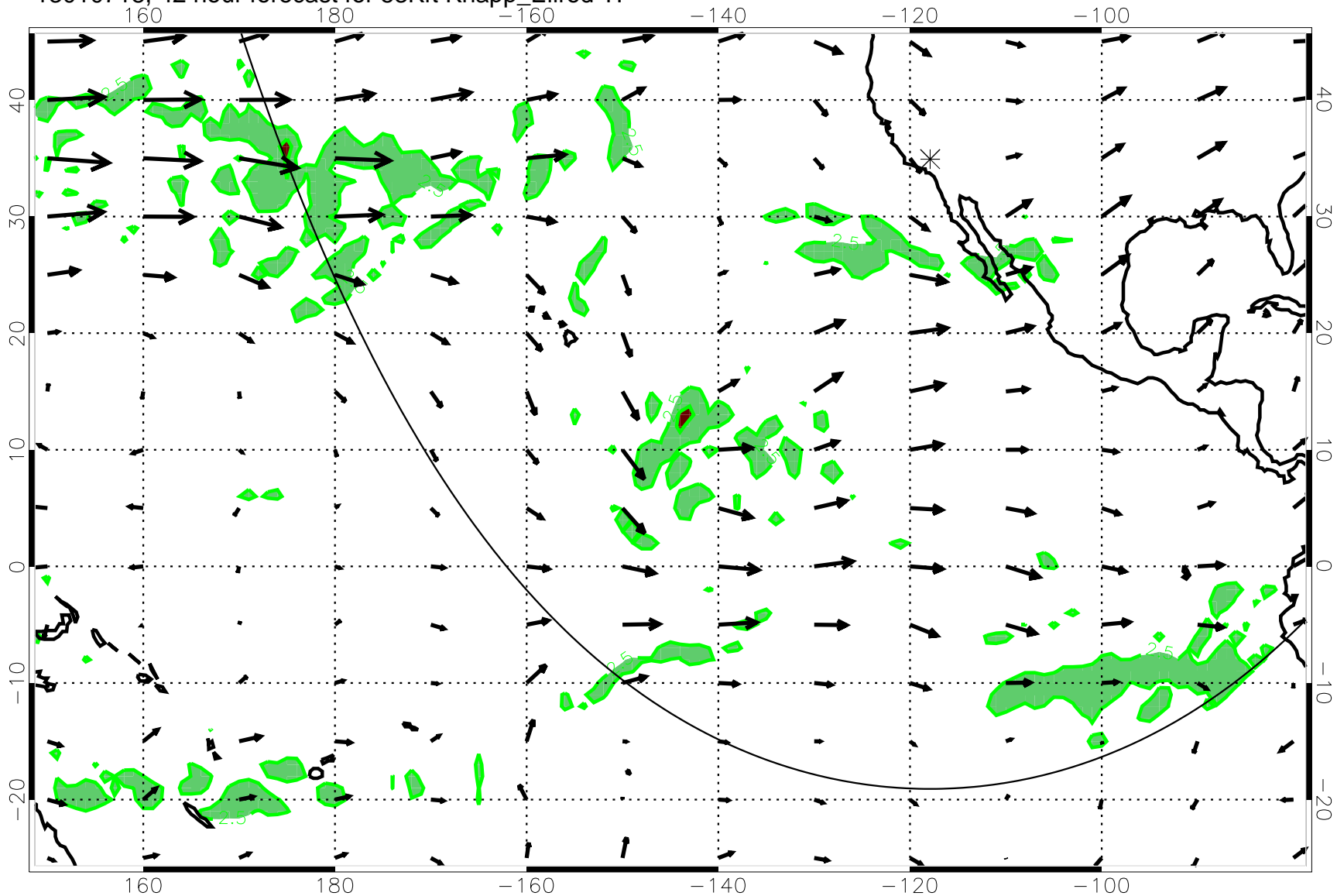
13010718, 42 hour forecast for 53Kft Knapp_Ellrod TI
