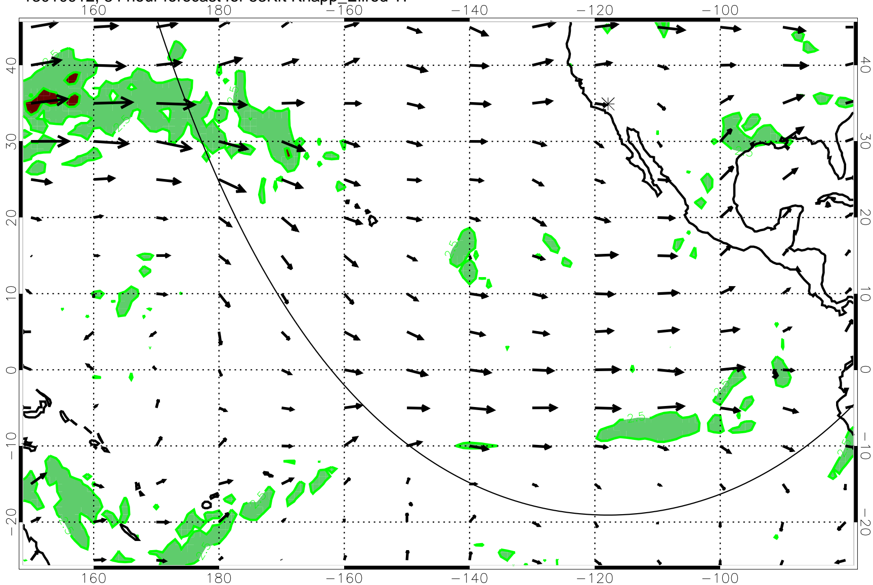
13010912, 84 hour forecast for 53Kft Knapp_Ellrod T1
