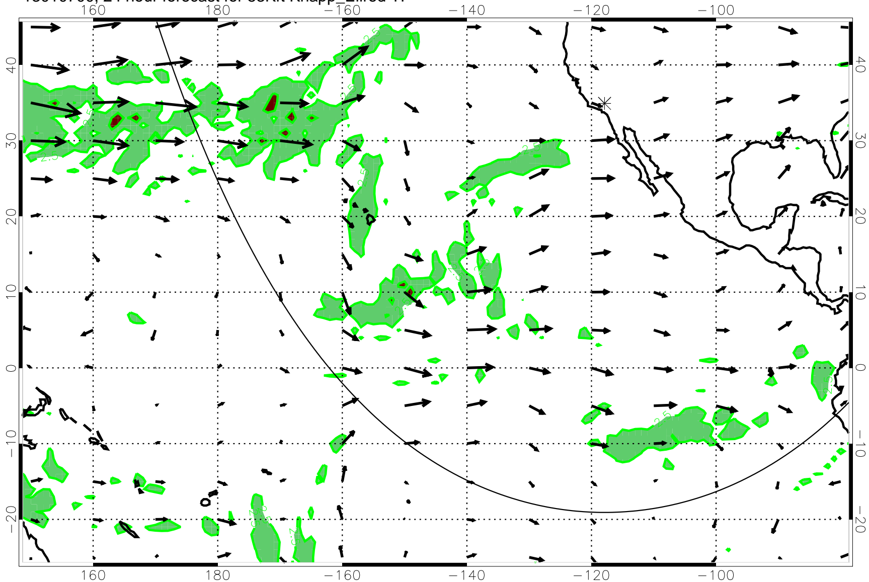
13010700, 24 hour forecast for 53Kft Knapp_Ellrod TI
