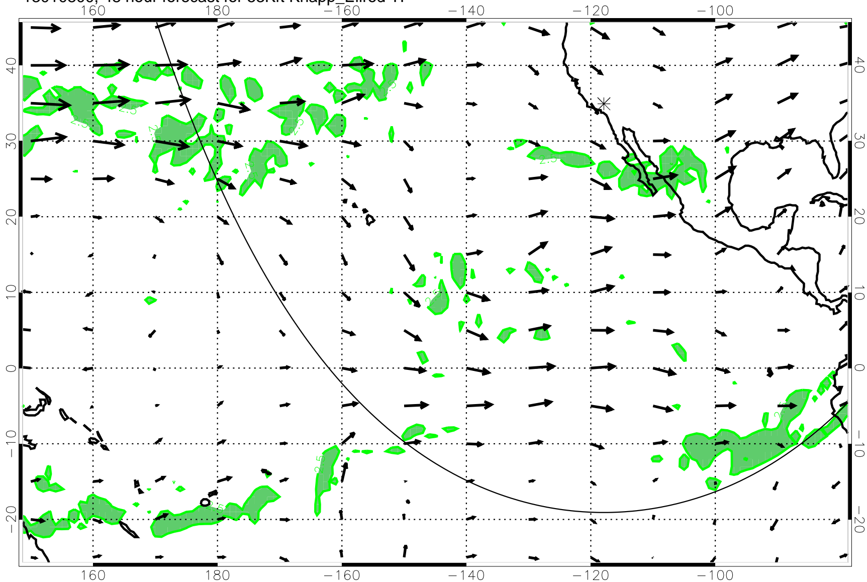
13010800, 48 hour forecast for 53Kft Knapp_Ellrod T1
