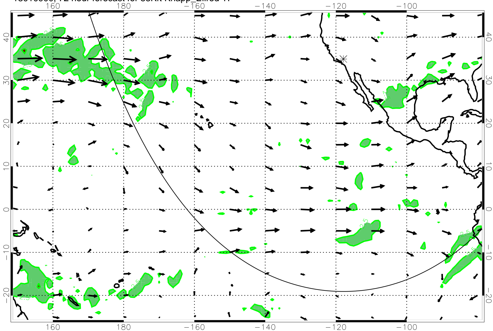
13010900, 72 hour forecast for 53Kft Knapp_Ellrod T1
