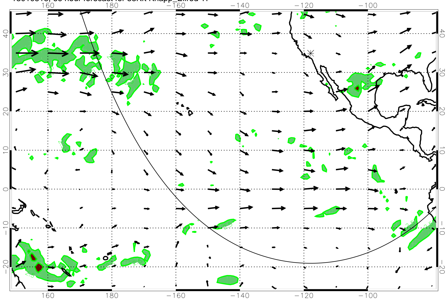
13010818, 66 hour forecast for 53Kft Knapp_Ellrod T1
