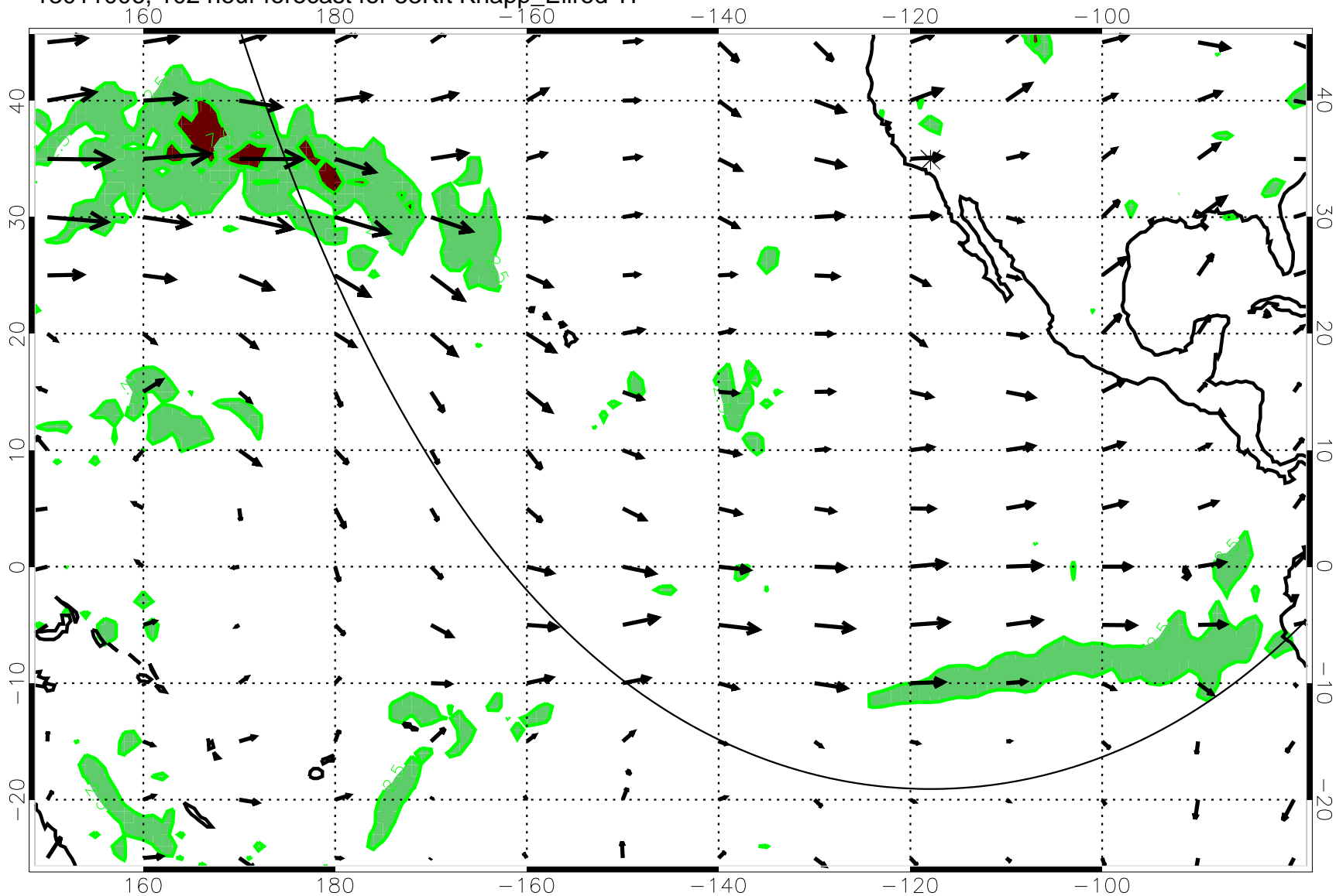
13011006, 102 hour forecast for 53Kft Knapp_Ellrod T1
