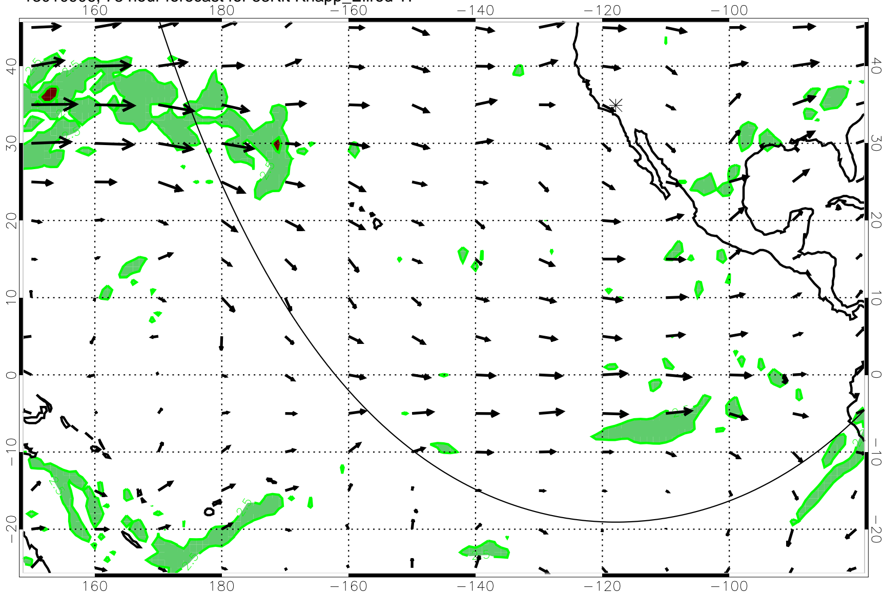
13010906, 78 hour forecast for 53Kft Knapp_Ellrod T1
