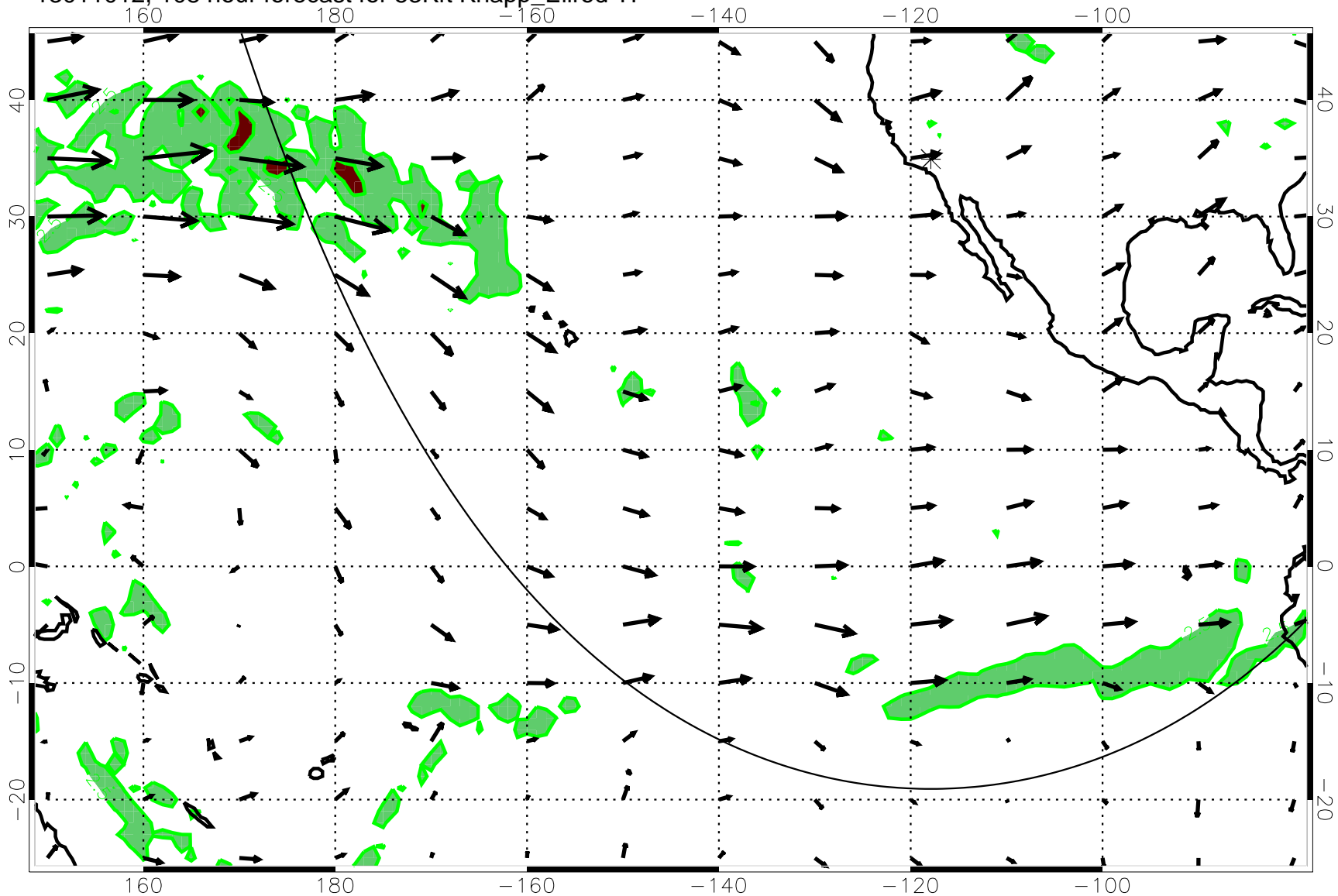
13011012, 108 hour forecast for 53Kft Knapp_Ellrod T1
