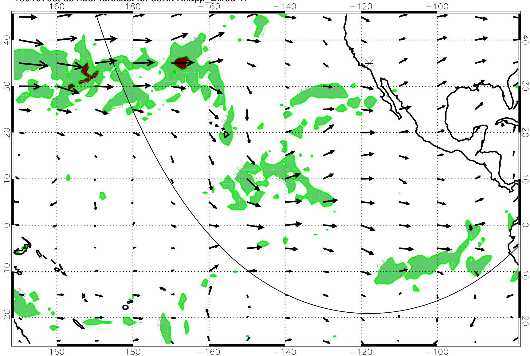
13010706, 30 hour forecast for 53Kft Knapp_Ellrod T1
