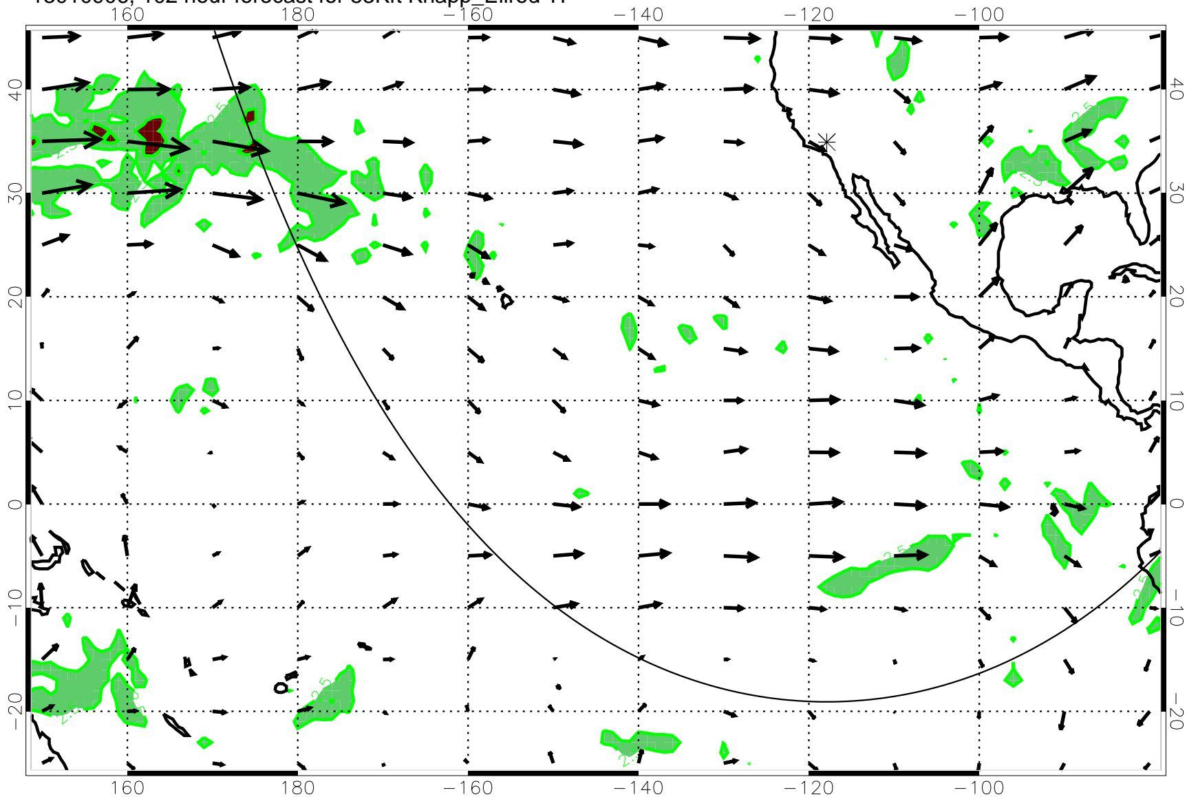
13010906, 102 hour forecast for 53Kft Knapp_Ellrod T1
