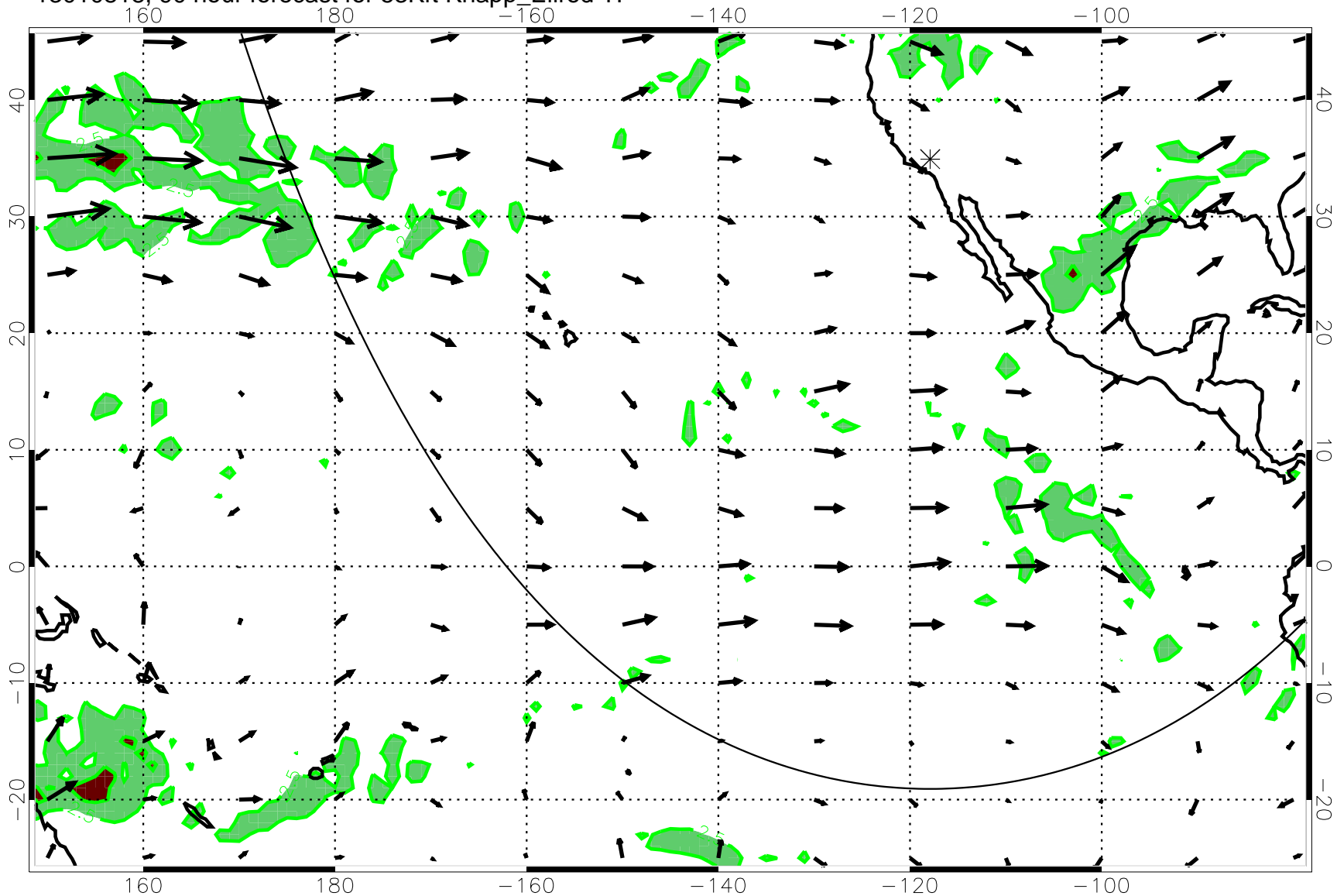
13010818, 90 hour forecast for 53Kft Knapp_Ellrod T1
