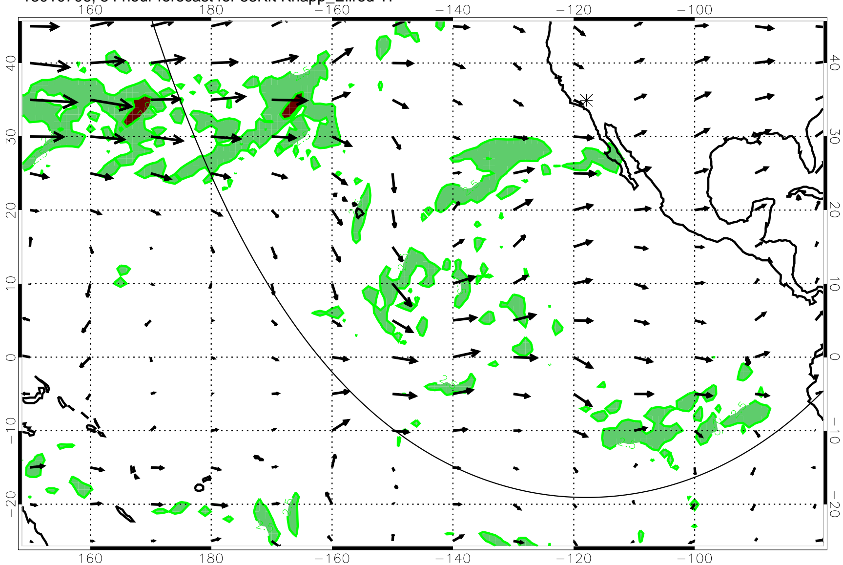
13010706, 54 hour forecast for 53Kft Knapp_Ellrod T1
