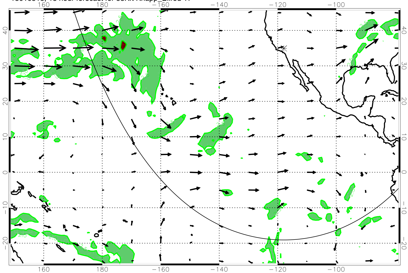
13010518, 18 hour forecast for 53Kft Knapp_Ellrod T1
