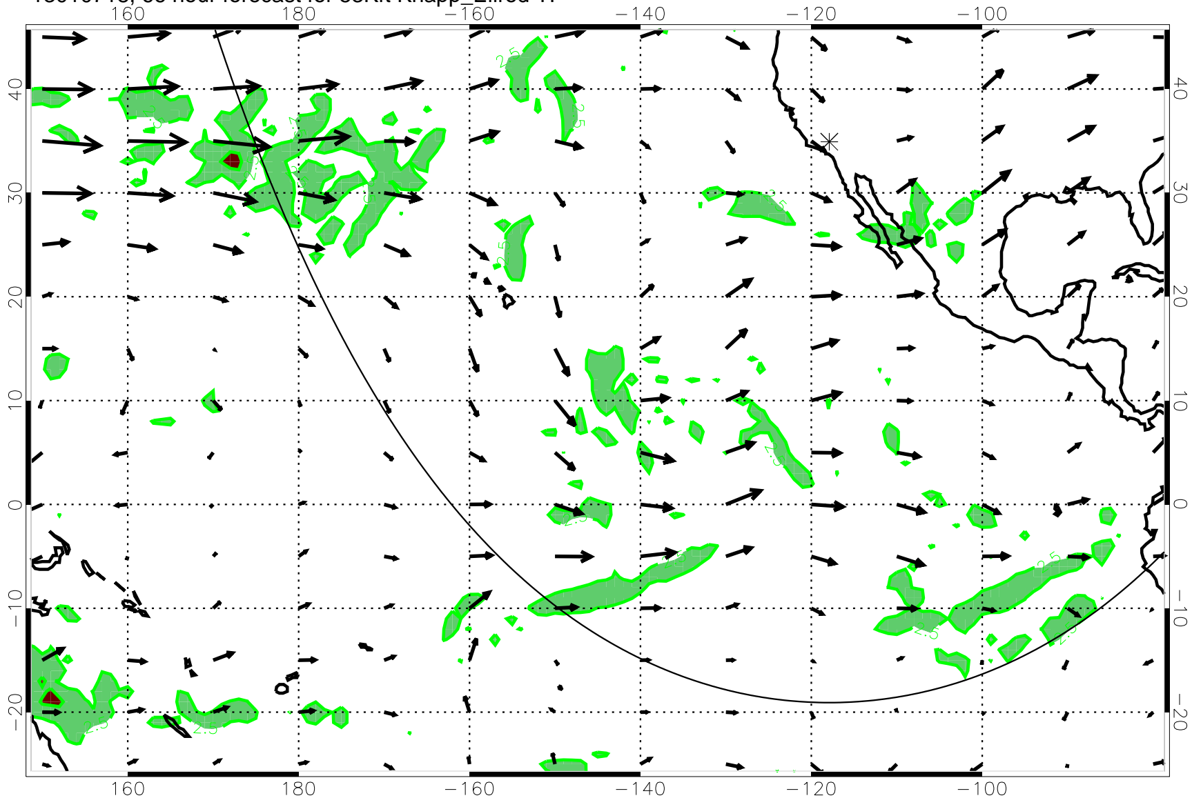
13010718, 66 hour forecast for 53Kft Knapp_Ellrod Tl
