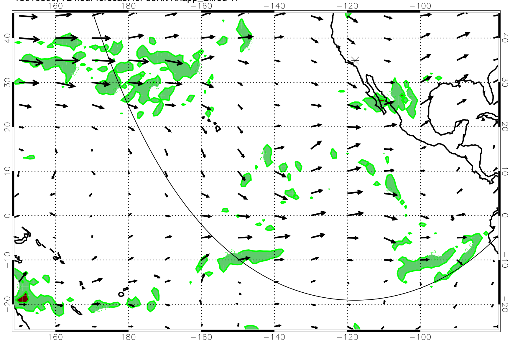
13010800, 72 hour forecast for 53Kft Knapp_Ellrod T1
