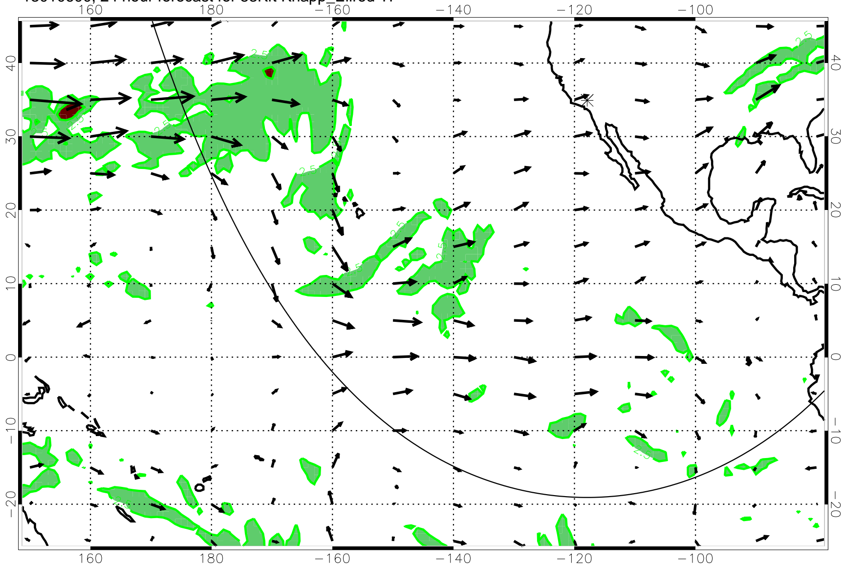
13010600, 24 hour forecast for 53Kft Knapp_Ellrod T1
