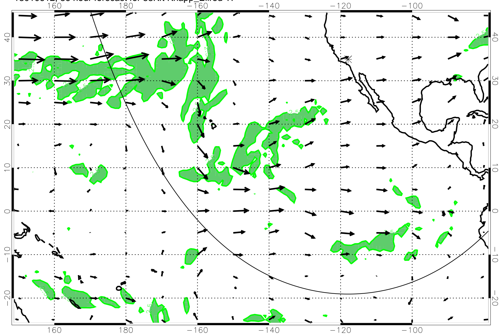
13010612, 36 hour forecast for 53Kft Knapp_Ellrod T1
