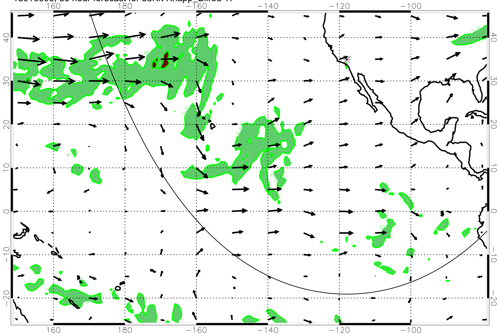
13010606, 30 hour forecast for 53Kft Knapp_Ellrod T1
