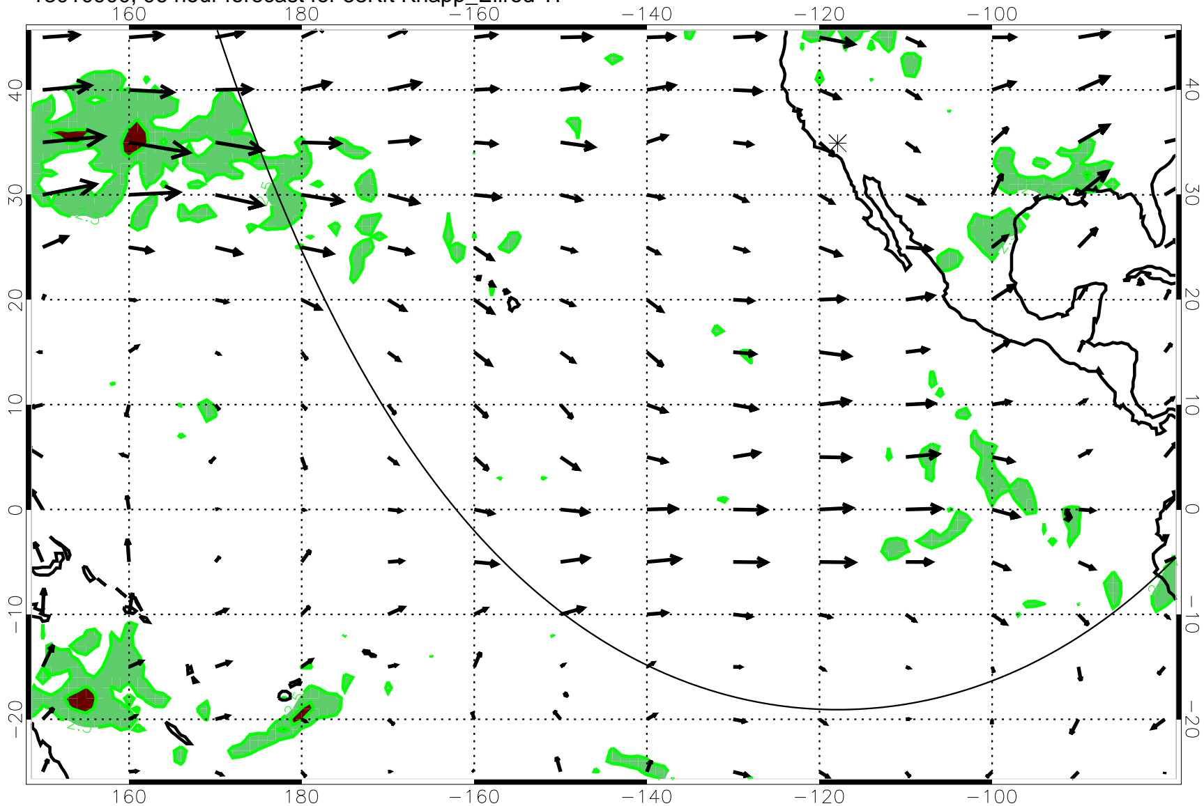
13010900, 96 hour forecast for 53Kft Knapp_Ellrod T1
