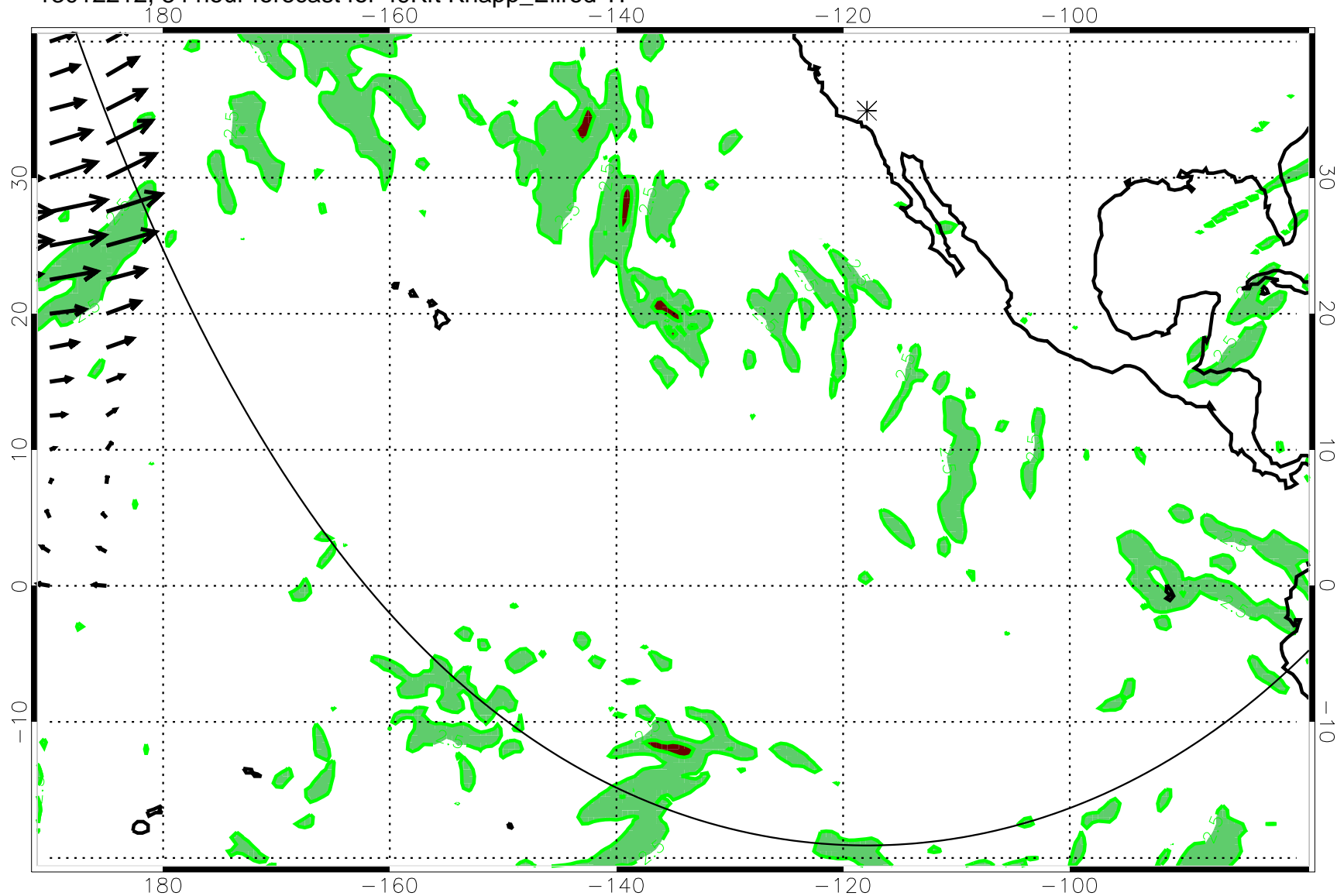
13012212, 84 hour forecast for 49Kft Knapp_Ellrod TI
