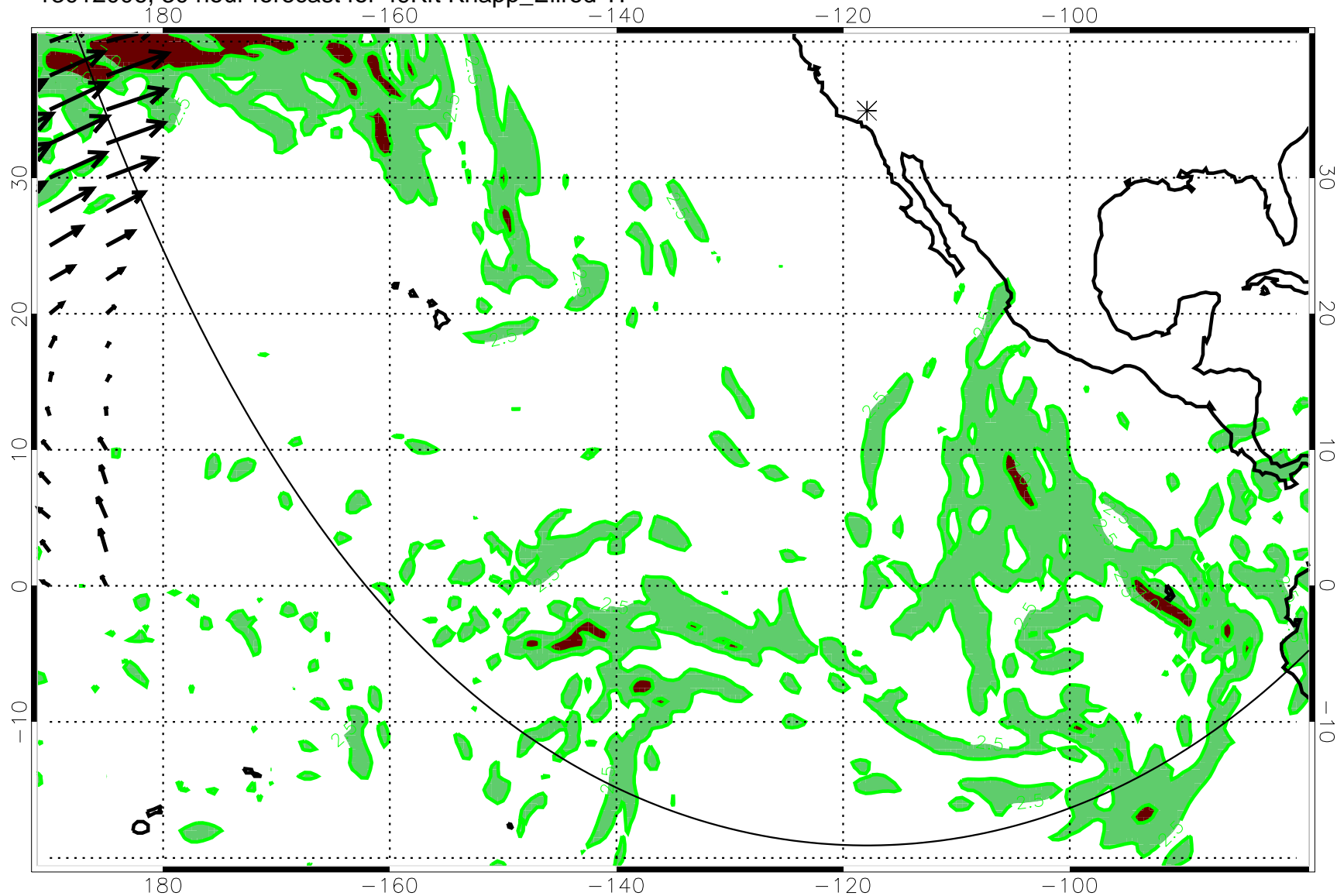
13012006, 30 hour forecast for 49Kft Knapp_Ellrod TI
