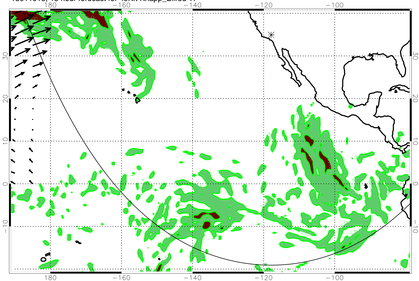
13011918, 18 hour forecast for 49Kft Knapp_Ellrod TI
