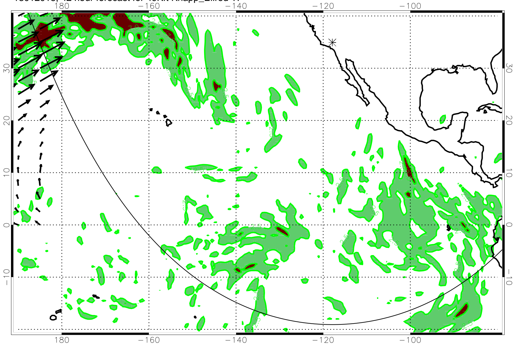
13012018, 42 hour forecast for 49Kft Knapp_Ellrod TI
