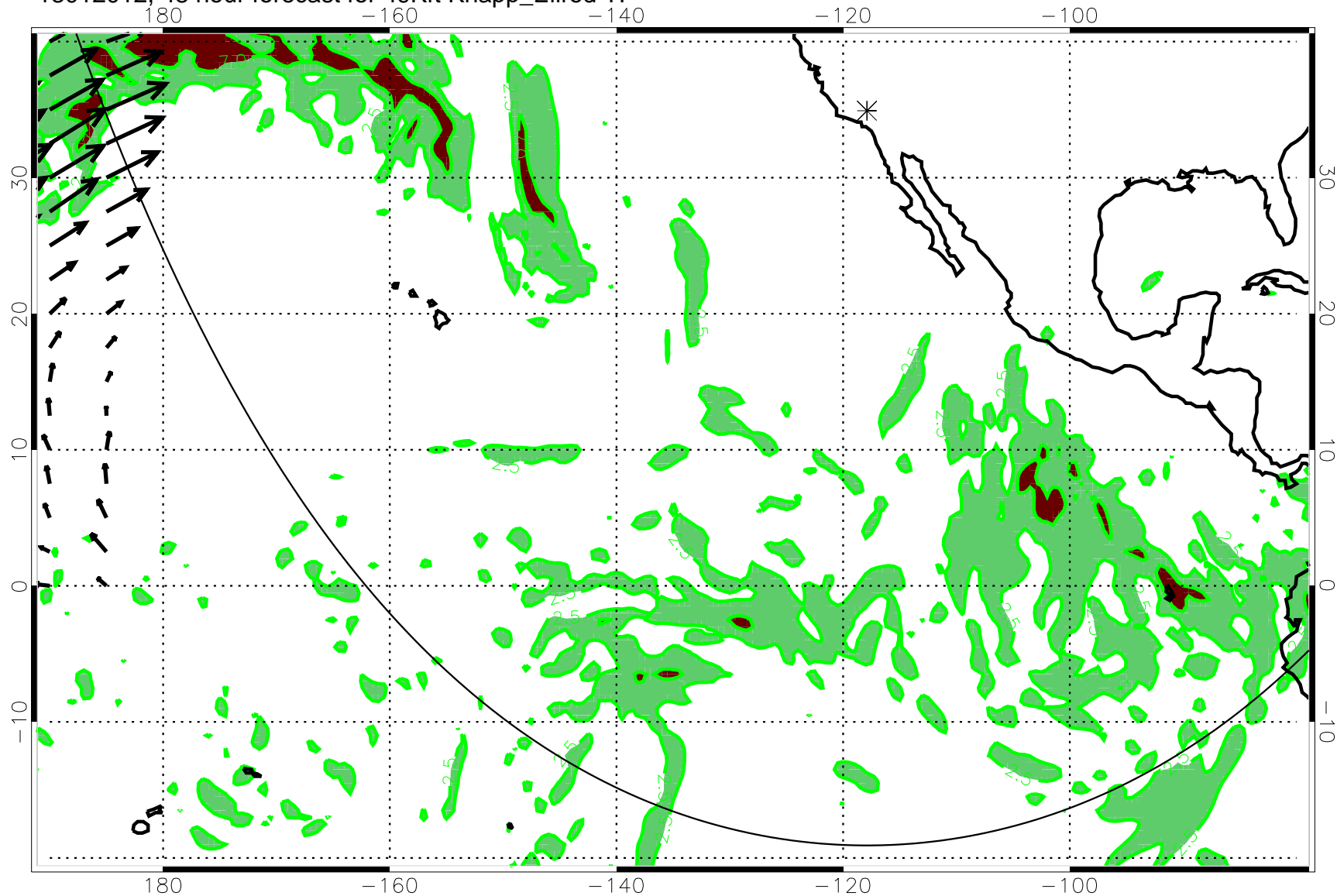
13012012, 48 hour forecast for 49Kft Knapp_Ellrod TI
