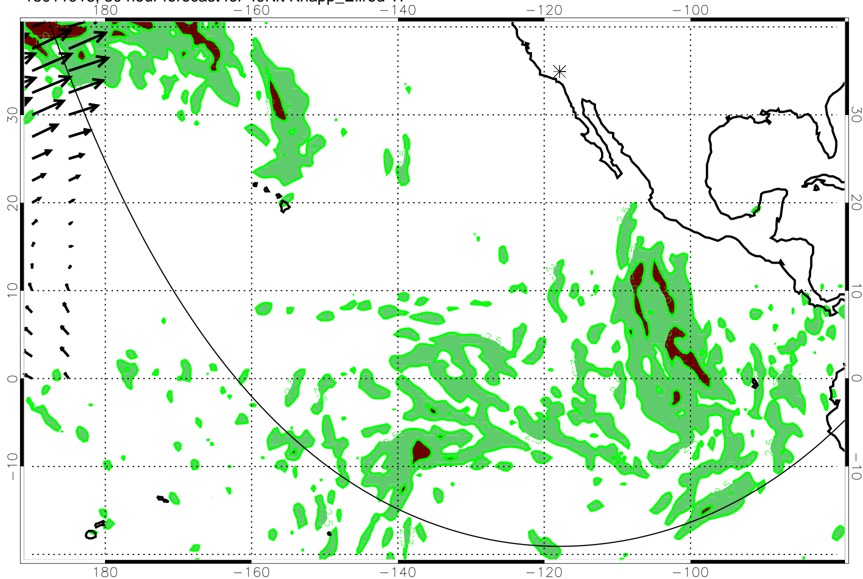
13011918, 30 hour forecast for 49Kft Knapp_Ellrod TI
