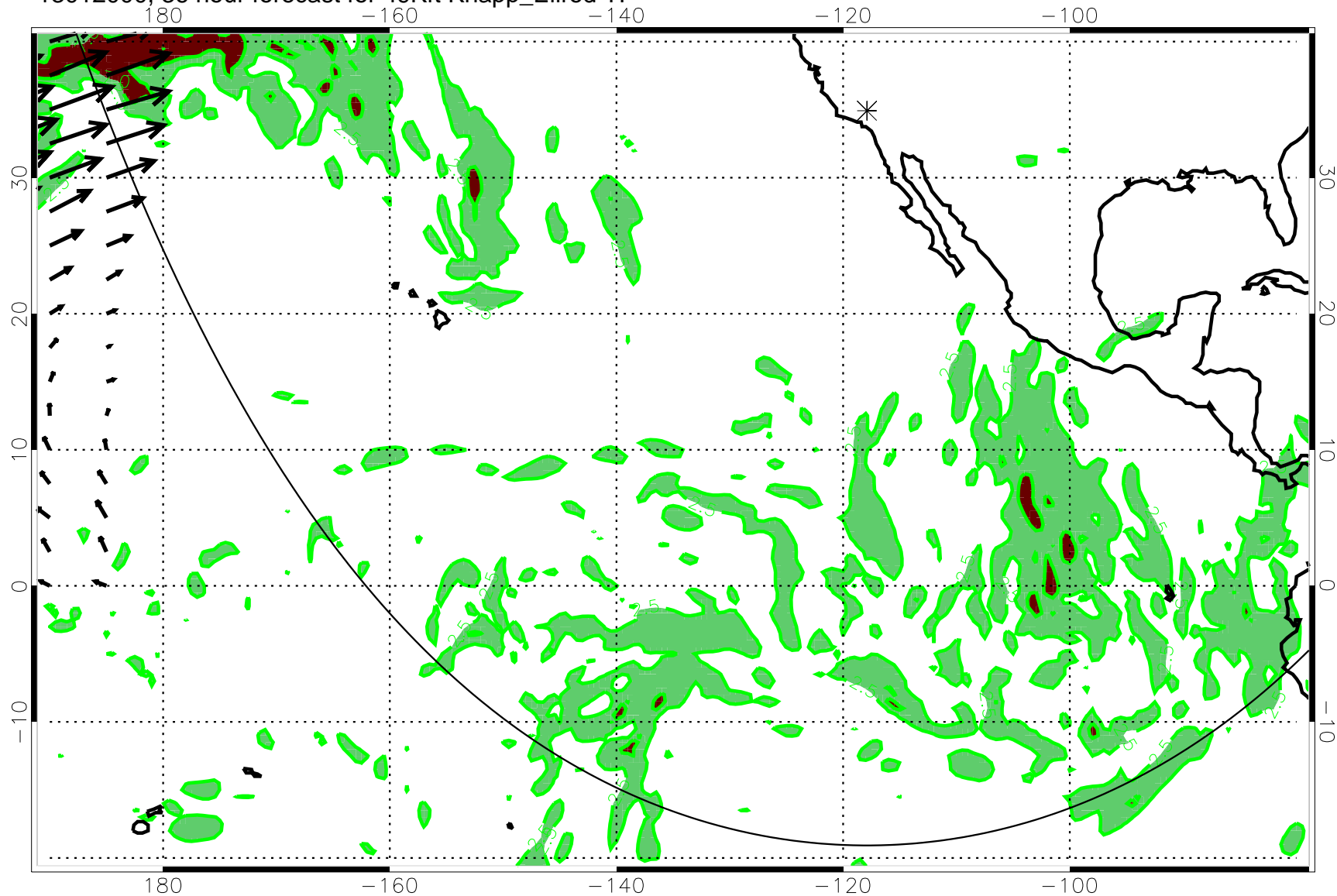
13012000, 36 hour forecast for 49Kft Knapp_Ellrod TI
