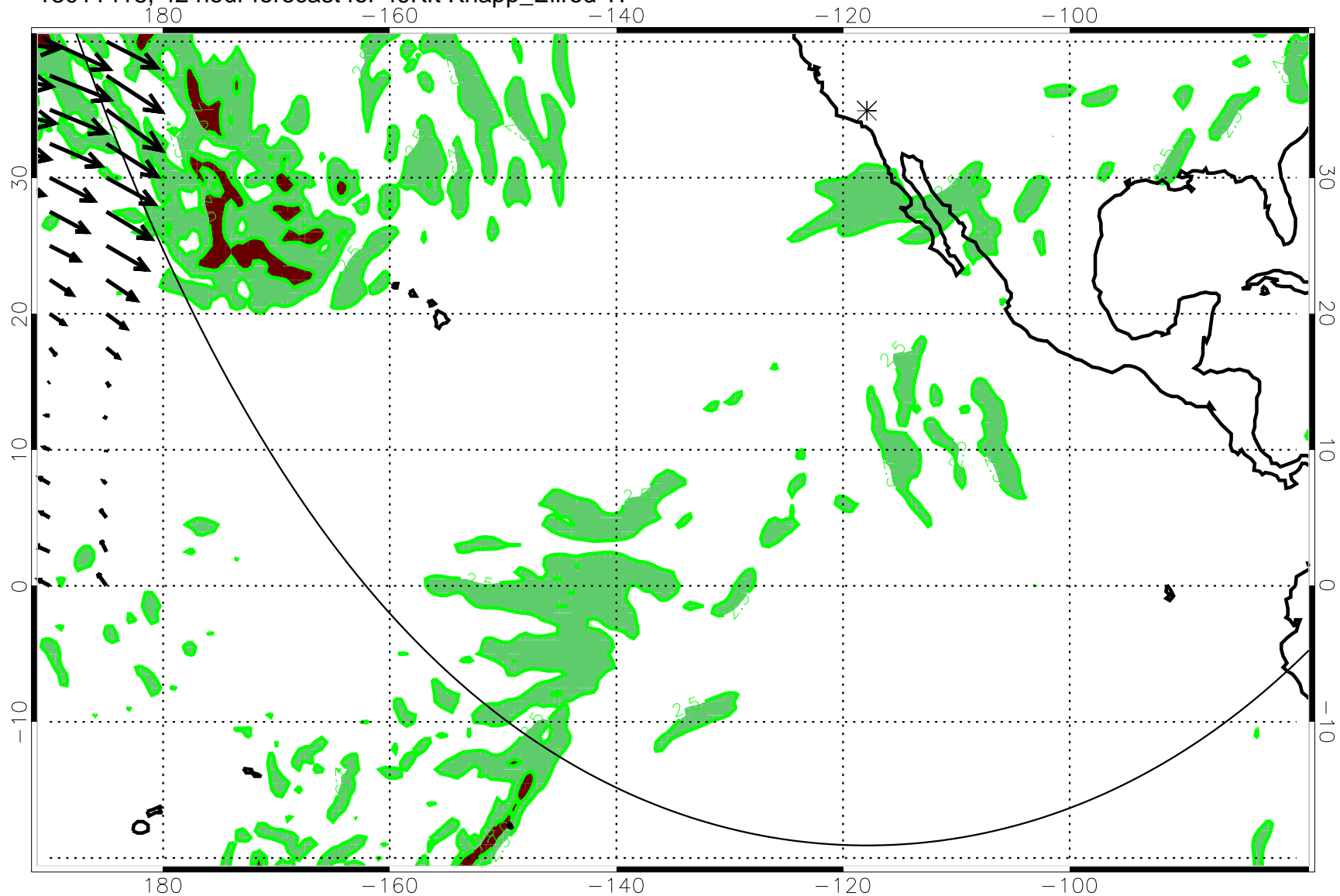
13011418, 42 hour forecast for 49Kft Knapp_Ellrod TI
