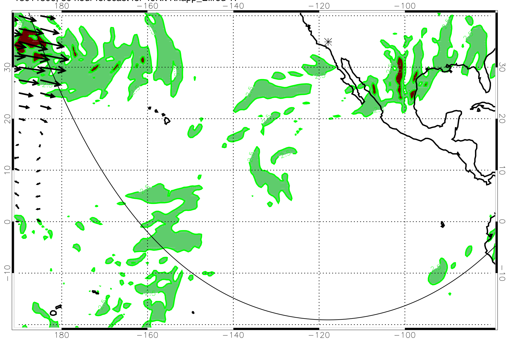
13011306, 30 hour forecast for 49Kft Knapp_Ellrod TI
