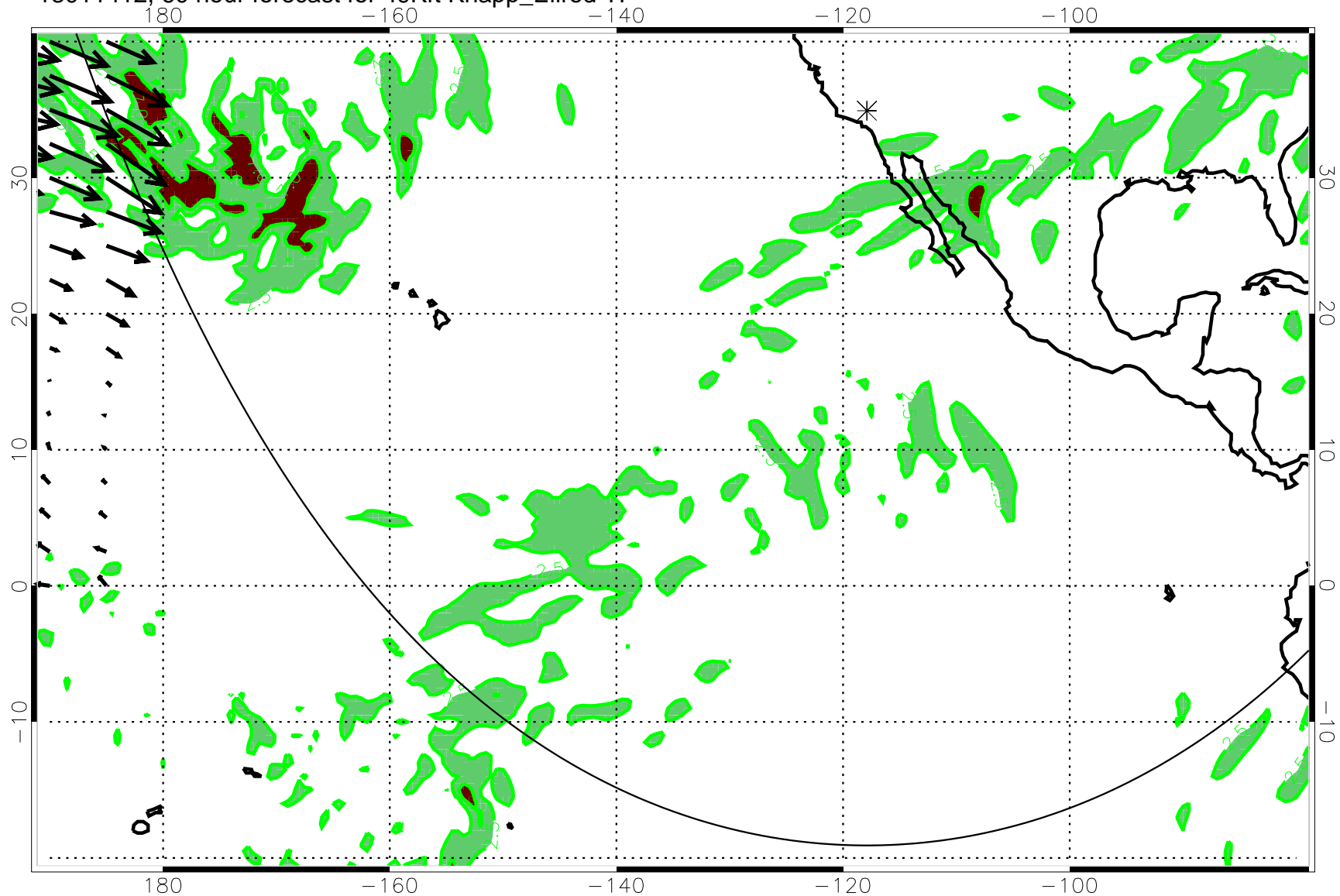
13011412, 60 hour forecast for 49Kft Knapp_Ellrod TI
