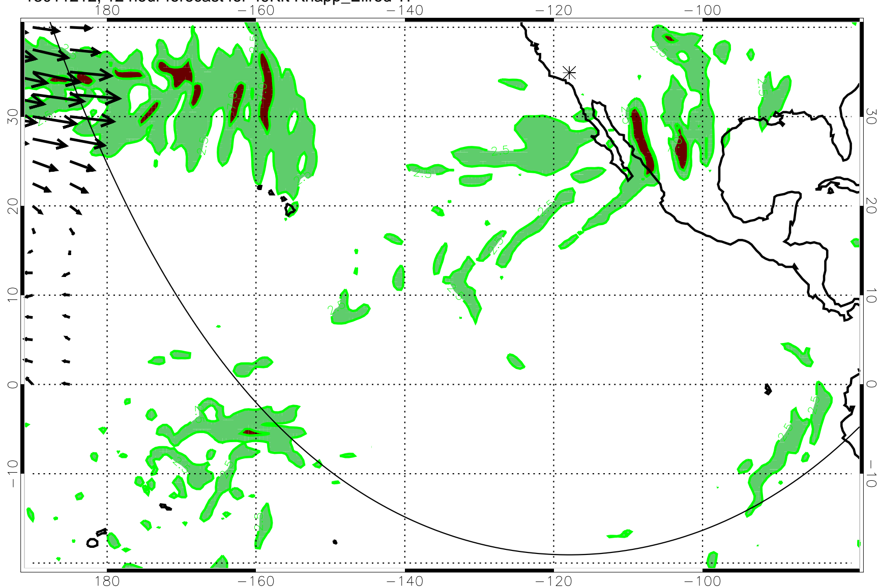
13011212, 12 hour forecast for 49Kft Knapp_Ellrod TI
