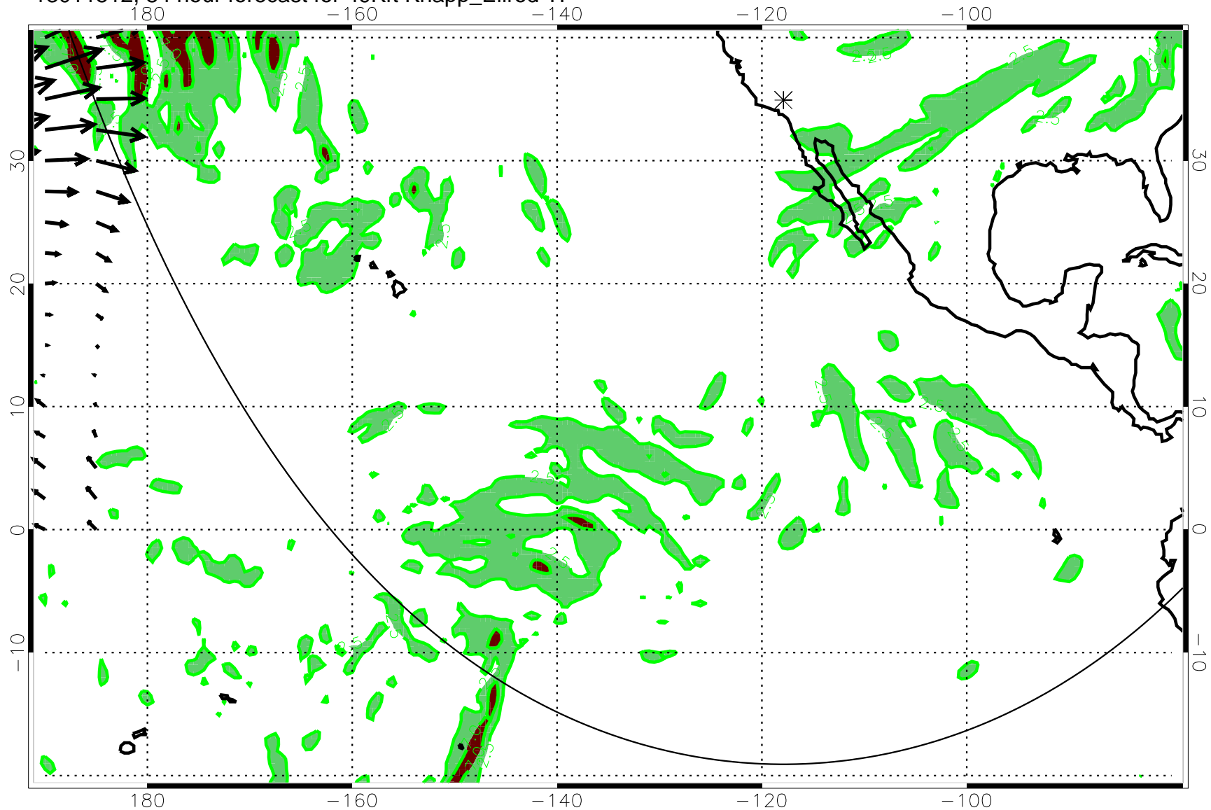
13011512, 84 hour forecast for 49Kft Knapp_Ellrod TI
