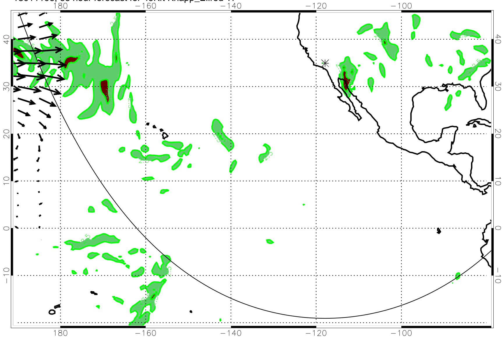
13011106, 66 hour forecast for 49Kft Knapp_Ellrod TI
