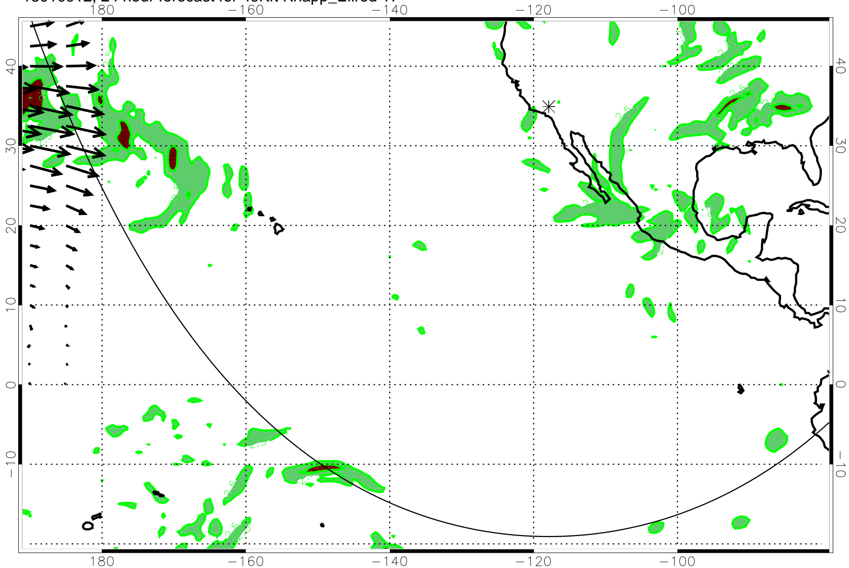
13010912, 24 hour forecast for 49Kft Knapp_Ellrod TI
