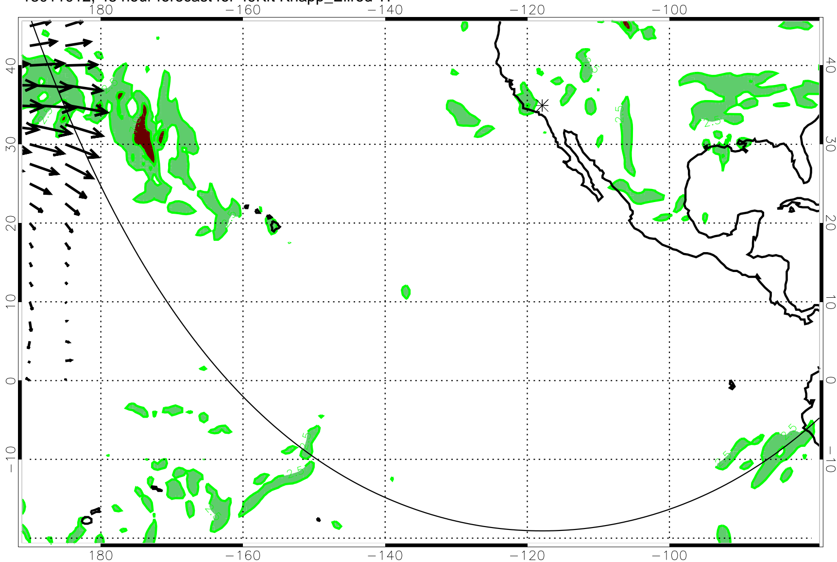
13011012, 48 hour forecast for 49Kft Knapp_Ellrod TI
