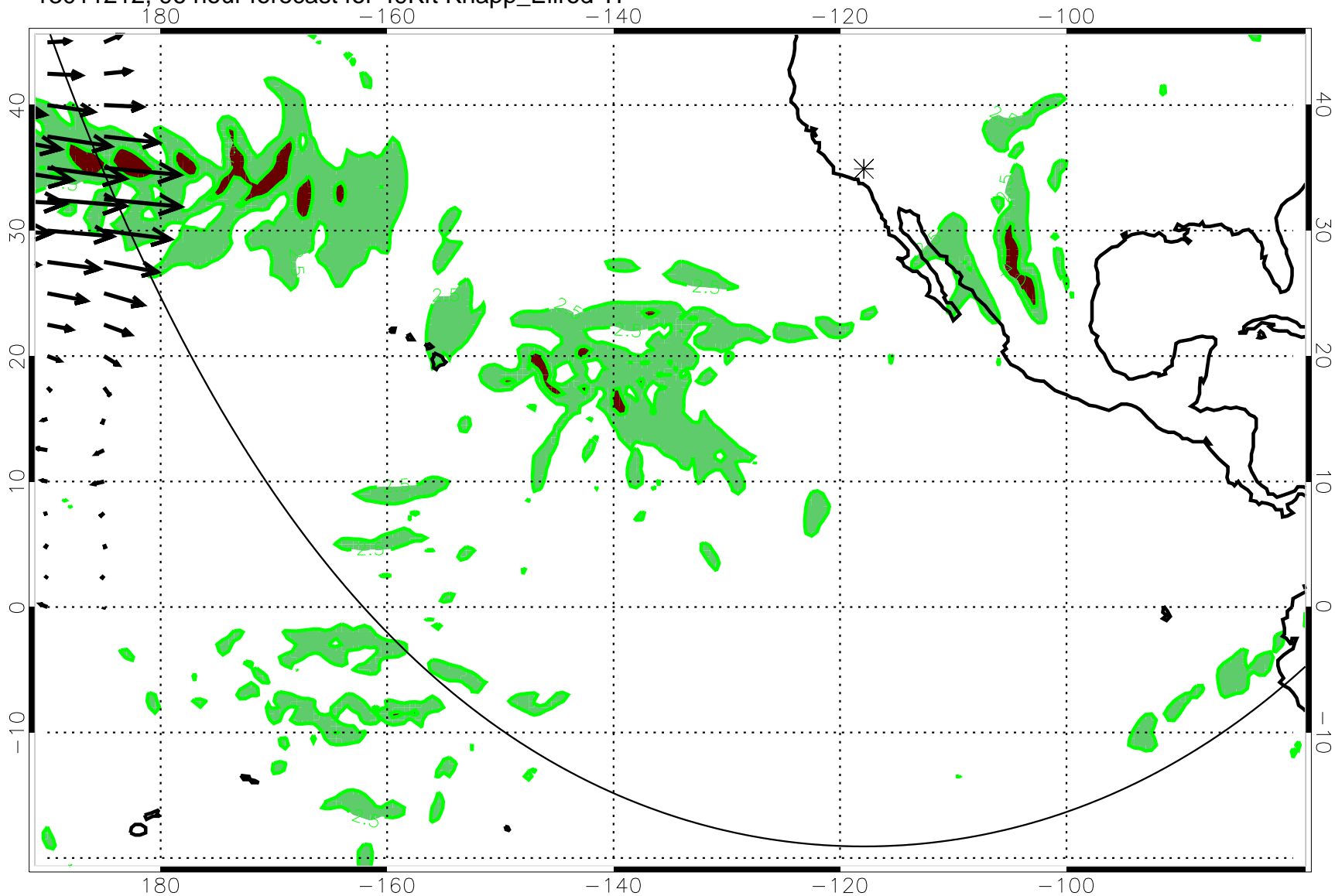
13011212, 96 hour forecast for 49Kft Knapp_Ellrod TI
