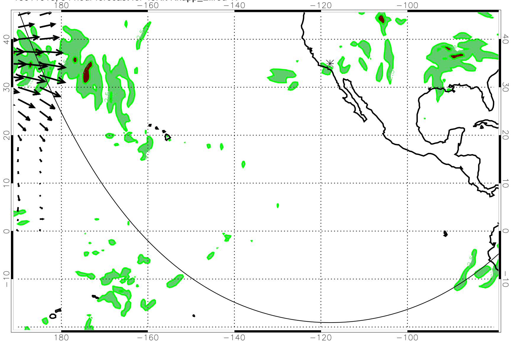
13011018, 54 hour forecast for 49Kft Knapp_Ellrod TI
