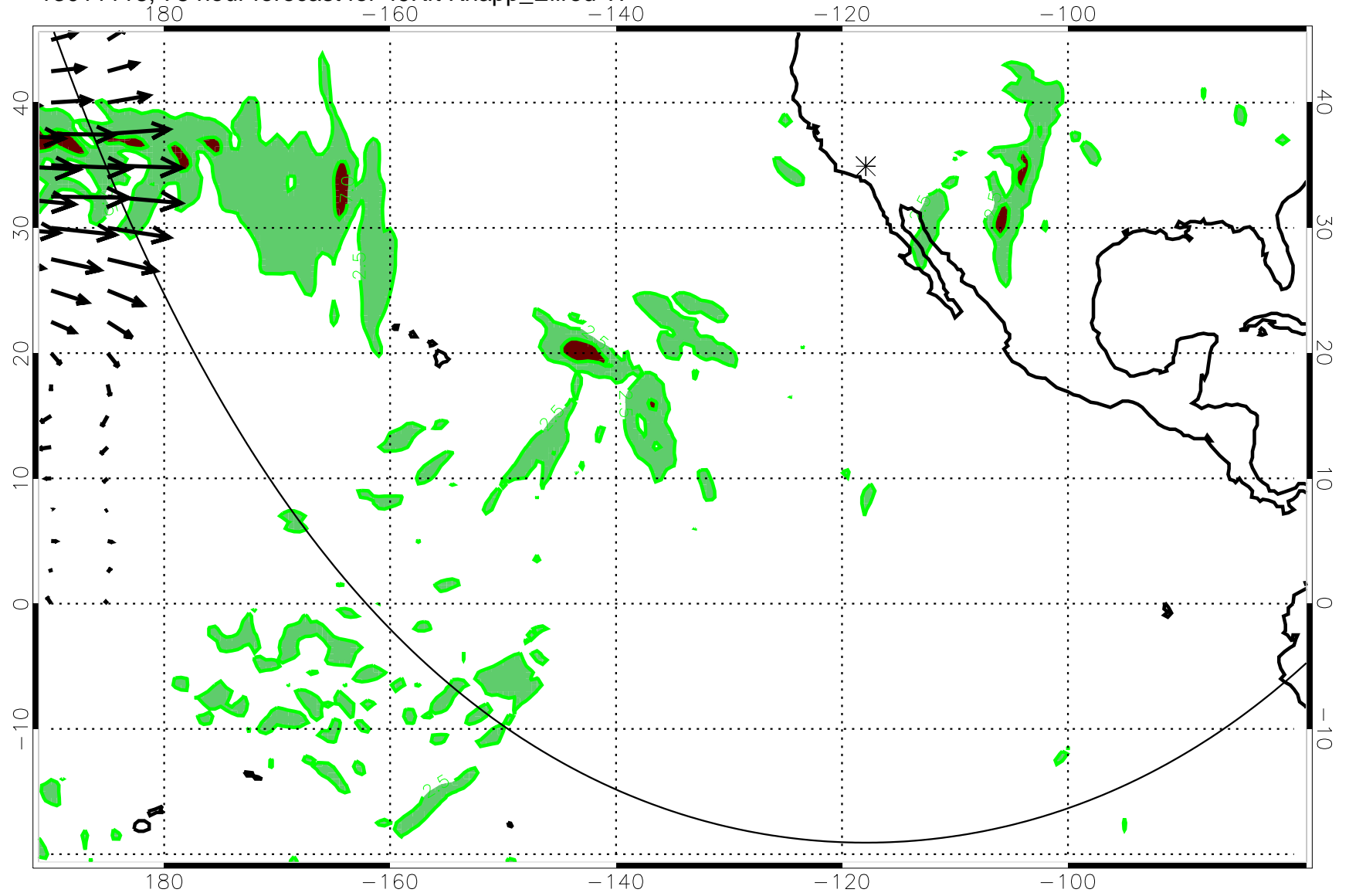
13011118, 78 hour forecast for 49Kft Knapp_Ellrod TI
