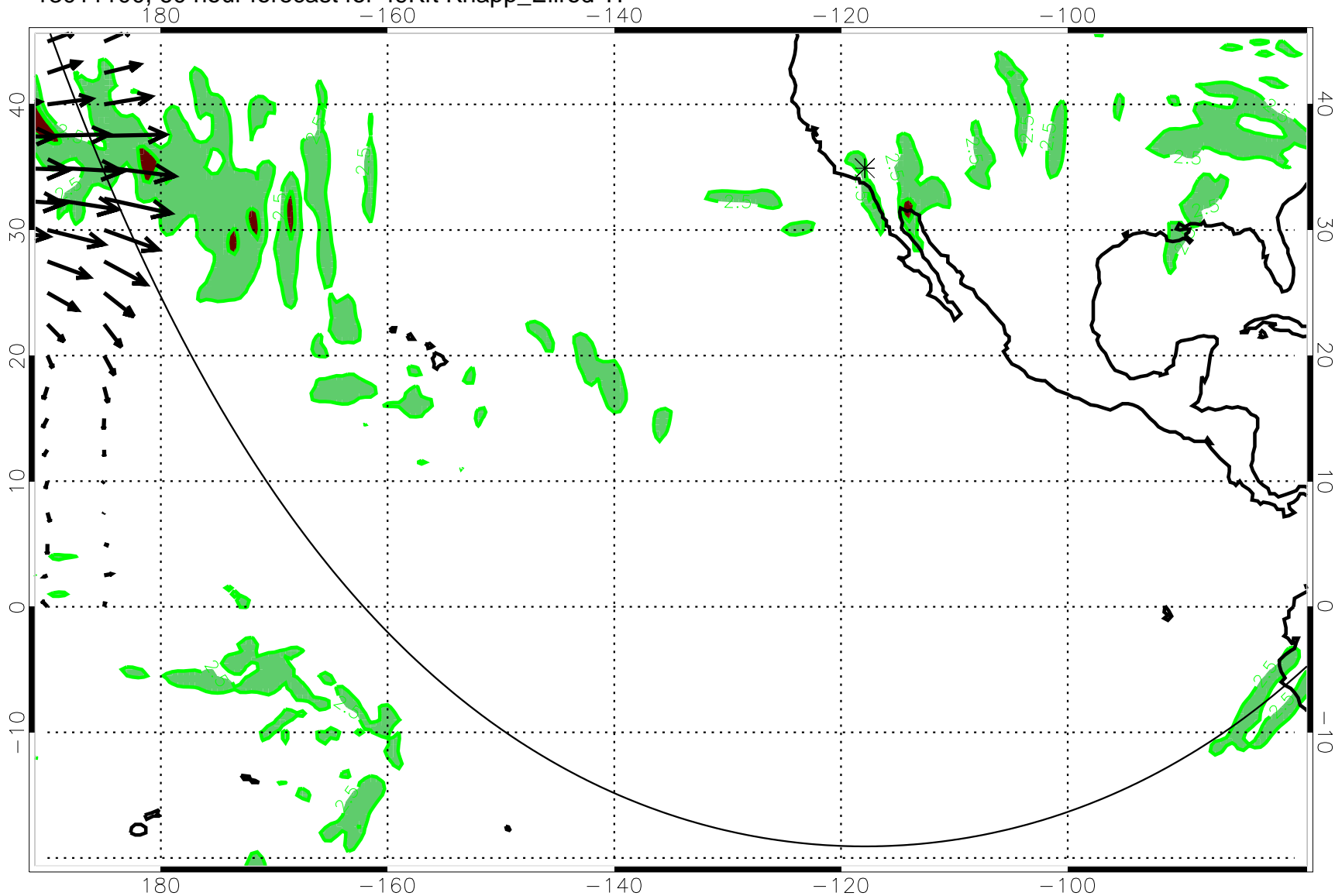
13011100, 60 hour forecast for 49Kft Knapp_Ellrod TI
