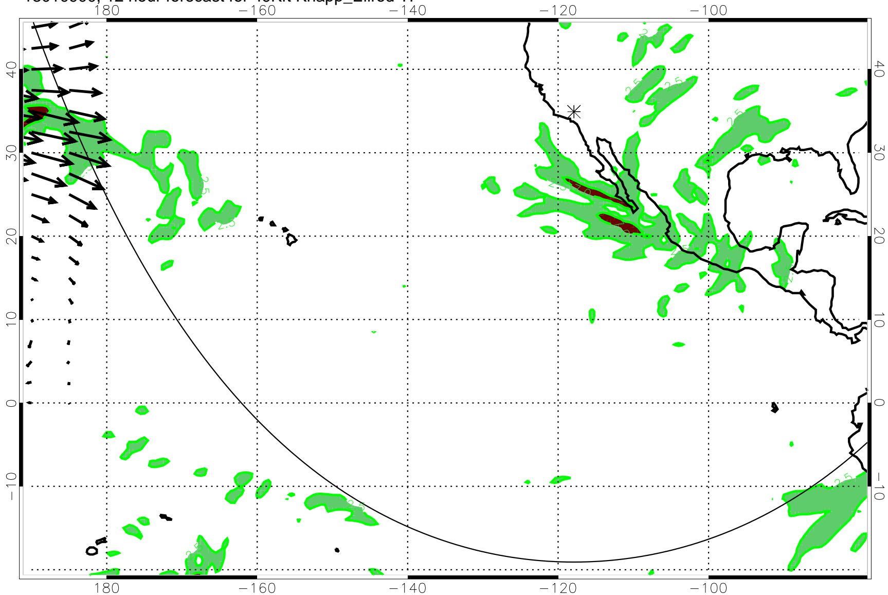
13010900, 12 hour forecast for 49Kft Knapp_Ellrod TI
