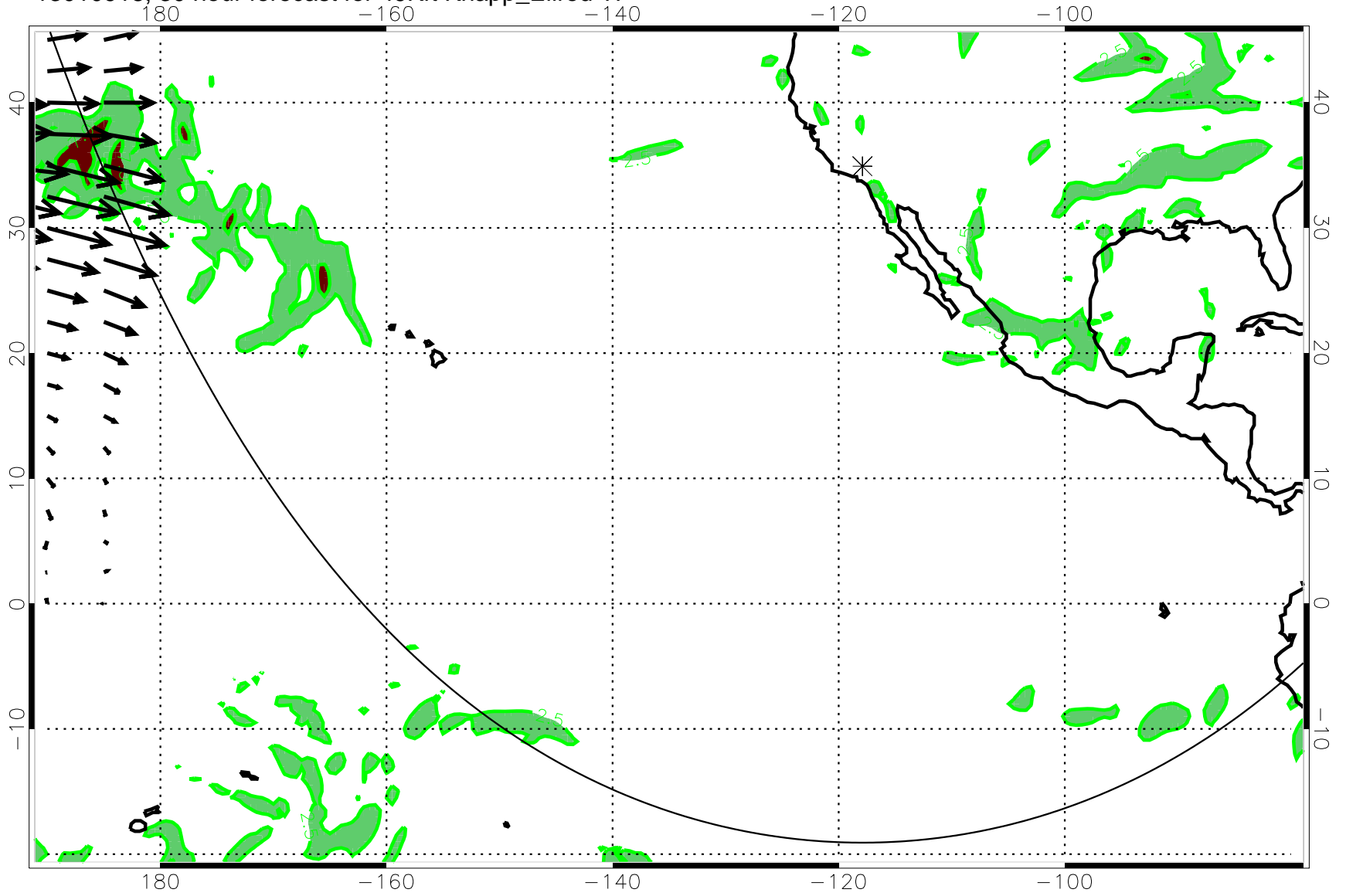
13010918, 30 hour forecast for 49Kft Knapp_Ellrod TI
