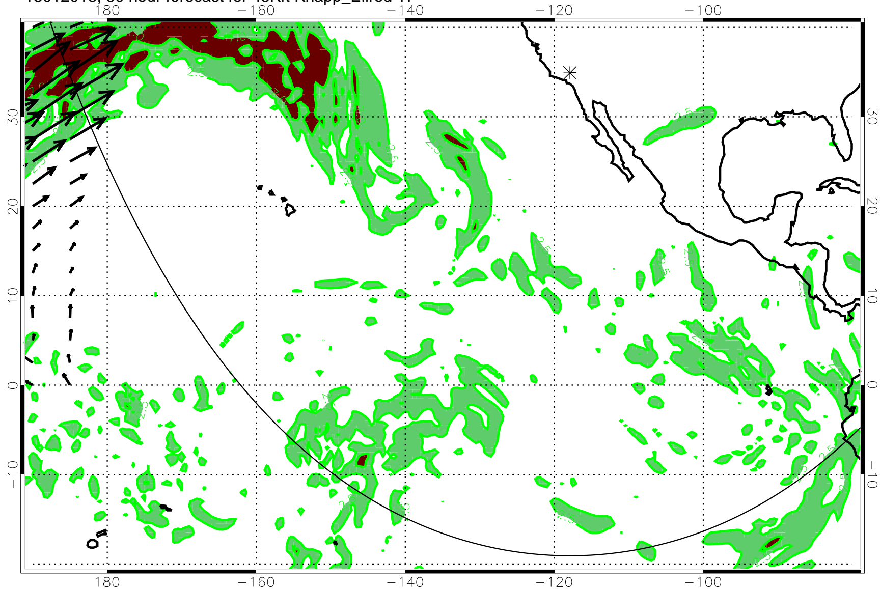
13012018, 30 hour forecast for 45Kft Knapp_Ellrod TI
