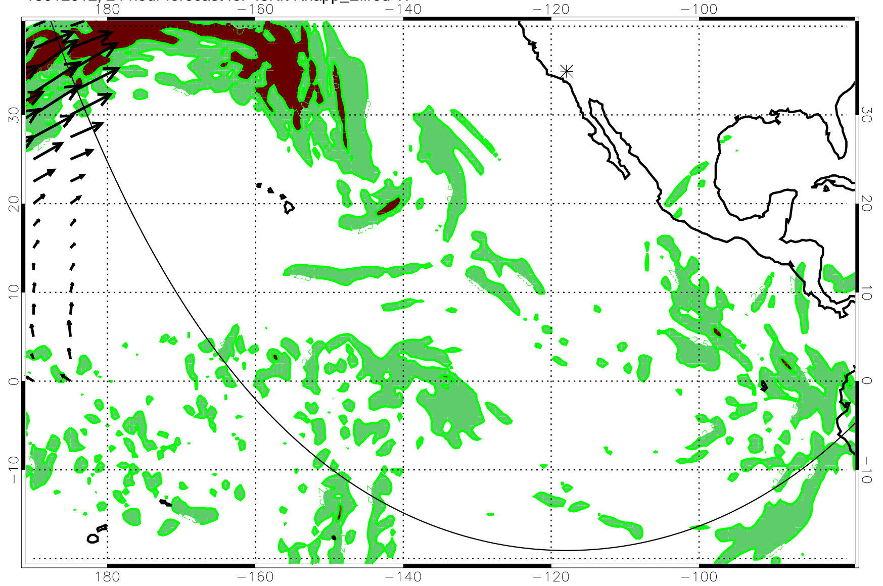
13012012, 24 hour forecast for 45Kft Knapp_Ellrod TI
