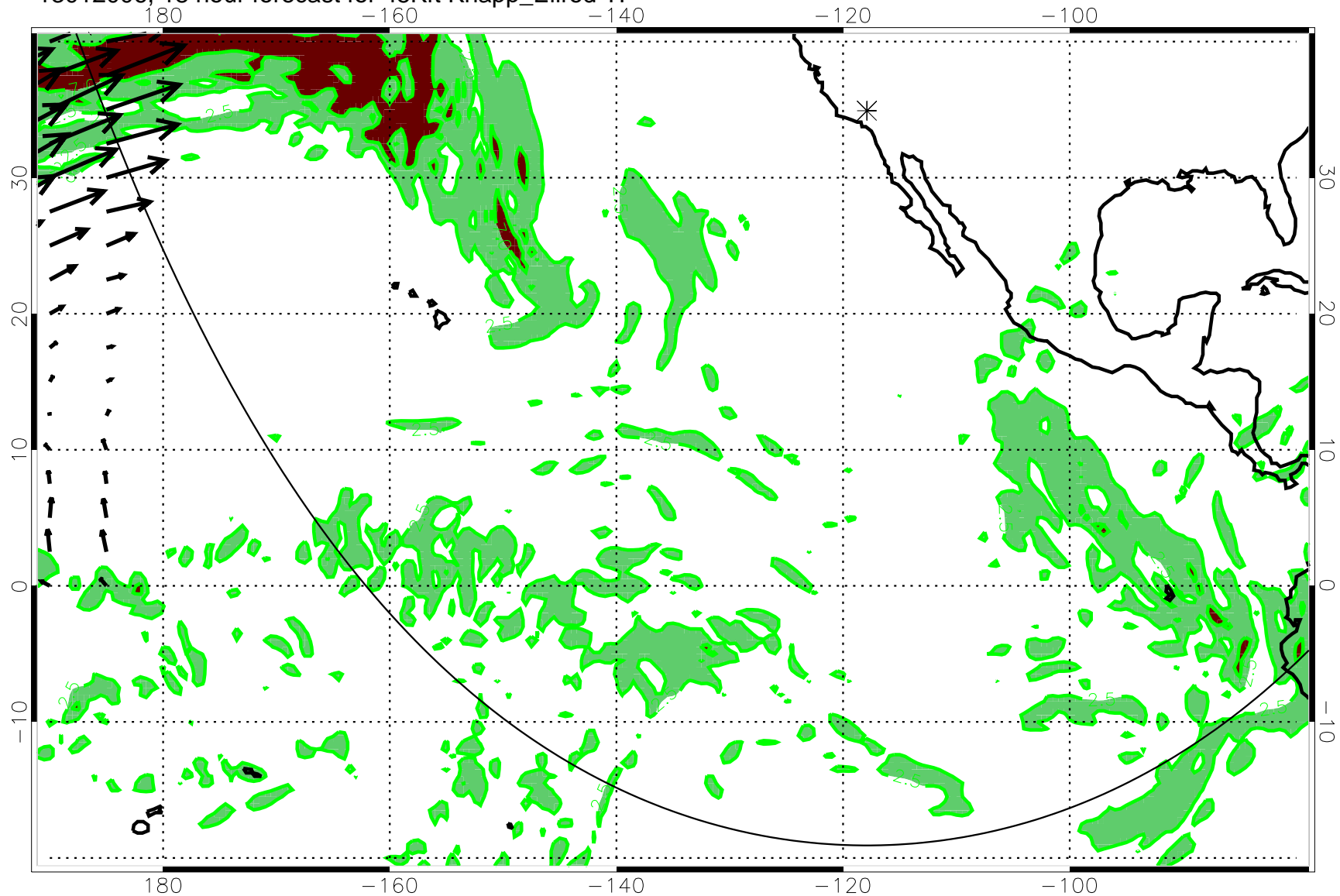
13012006, 18 hour forecast for 45Kft Knapp_Ellrod TI
