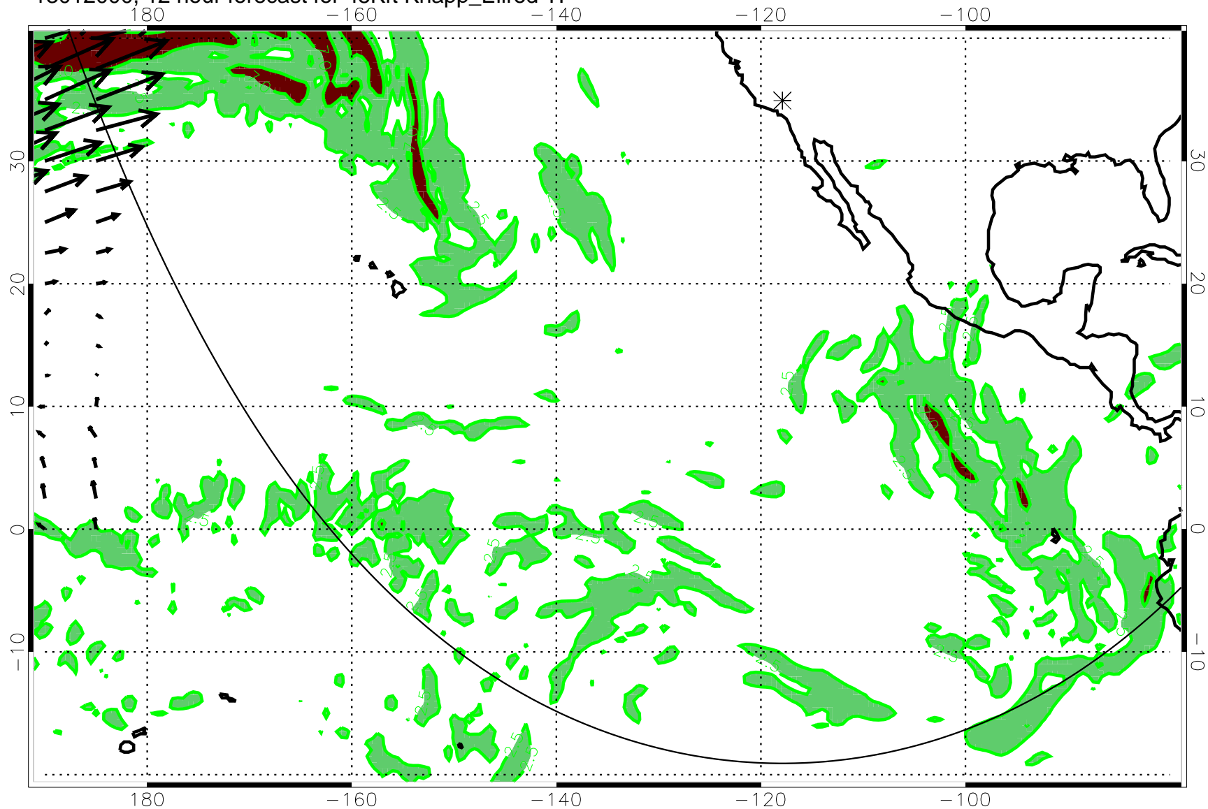
13012000, 12 hour forecast for 45Kft Knapp_Ellrod TI
