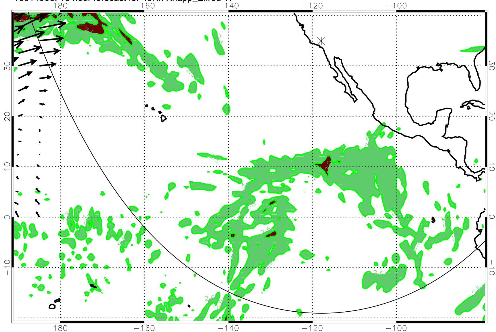
13011906, 18 hour forecast for 45Kft Knapp_Ellrod T1
