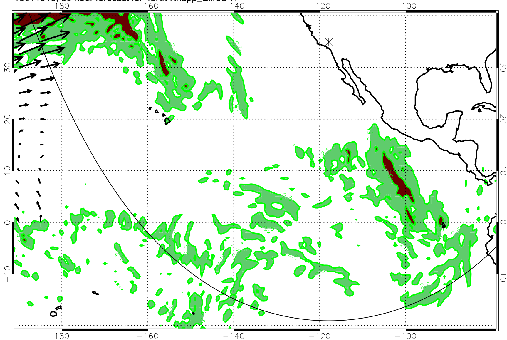
13011918, 30 hour forecast for 45Kft Knapp_Ellrod TI
