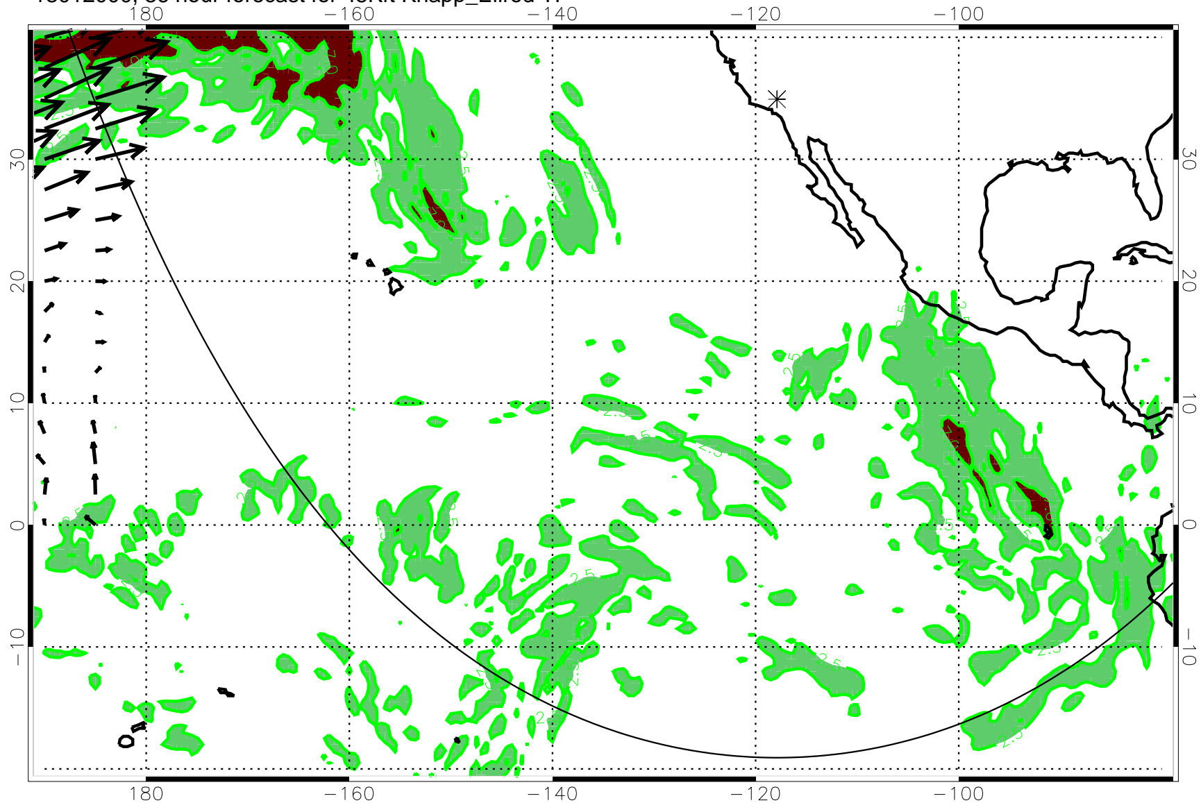
13012000, 36 hour forecast for 45Kft Knapp_Ellrod TI
