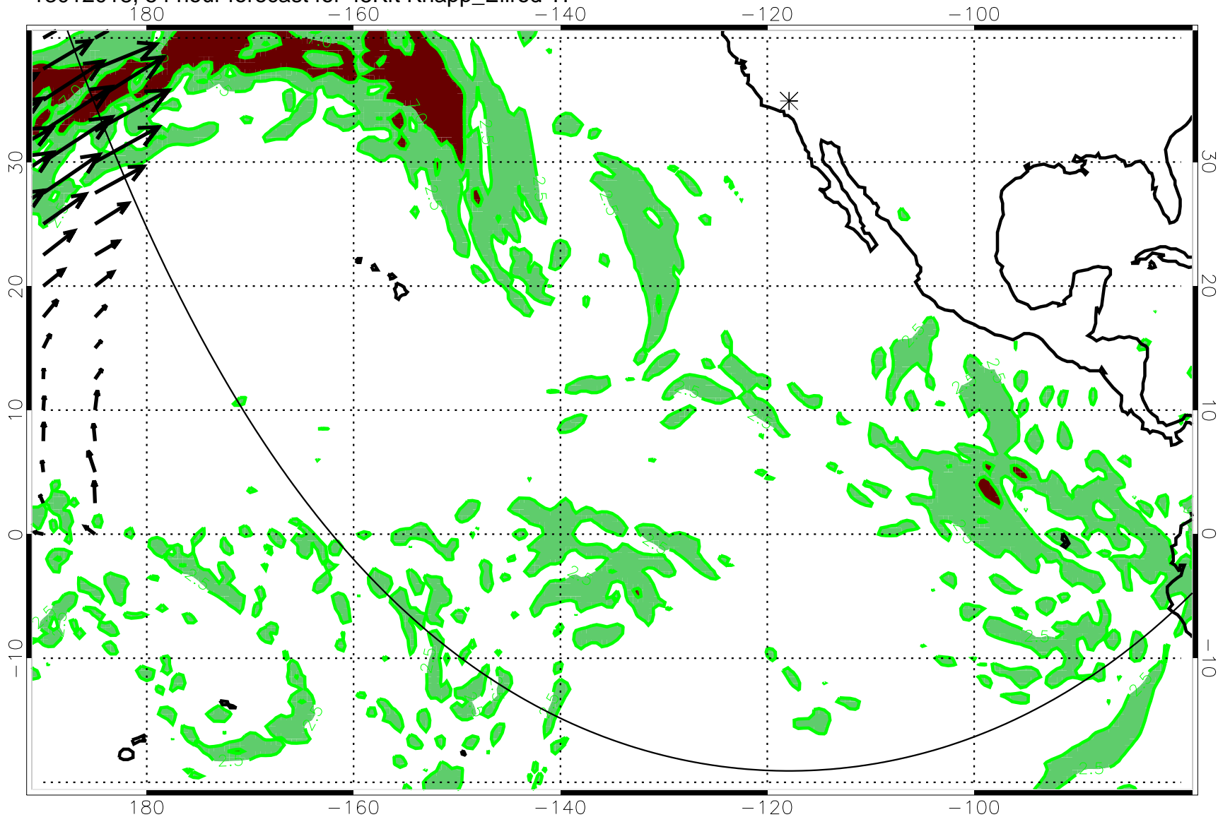
13012018, 54 hour forecast for 45Kft Knapp_Ellrod TI
