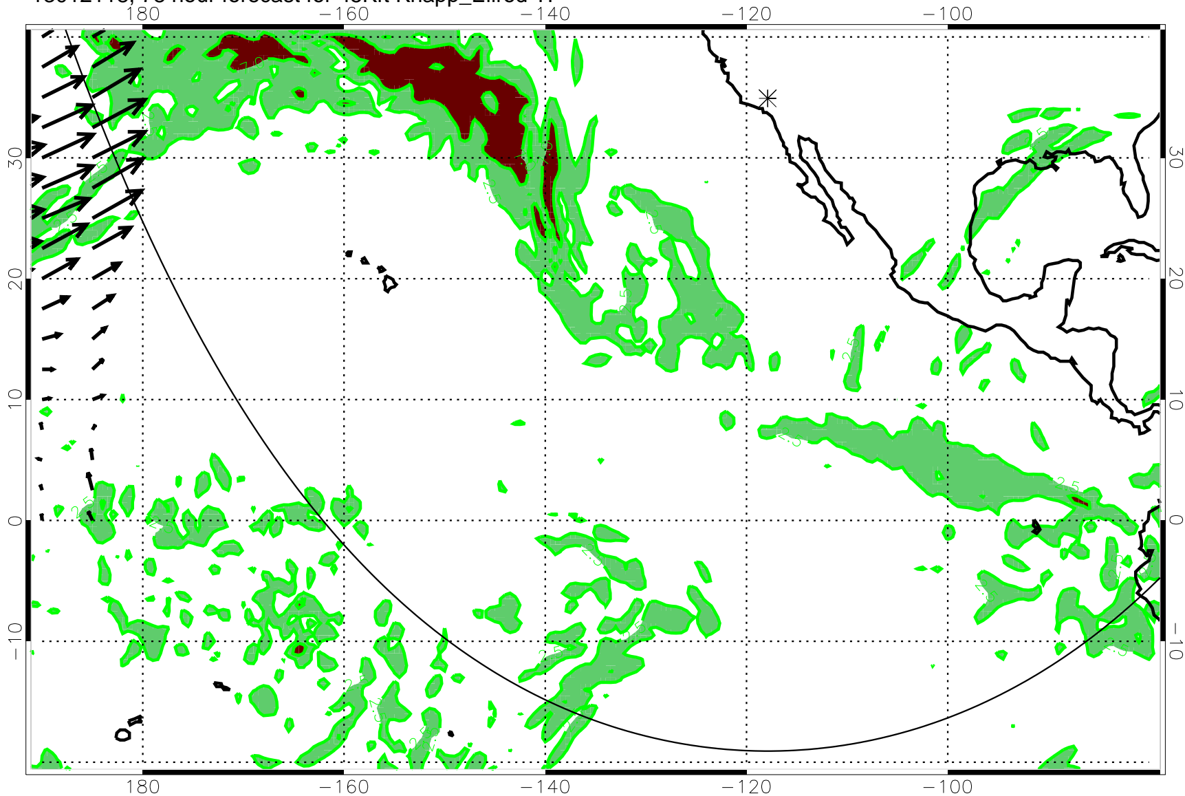
13012118, 78 hour forecast for 45Kft Knapp_Ellrod TI
