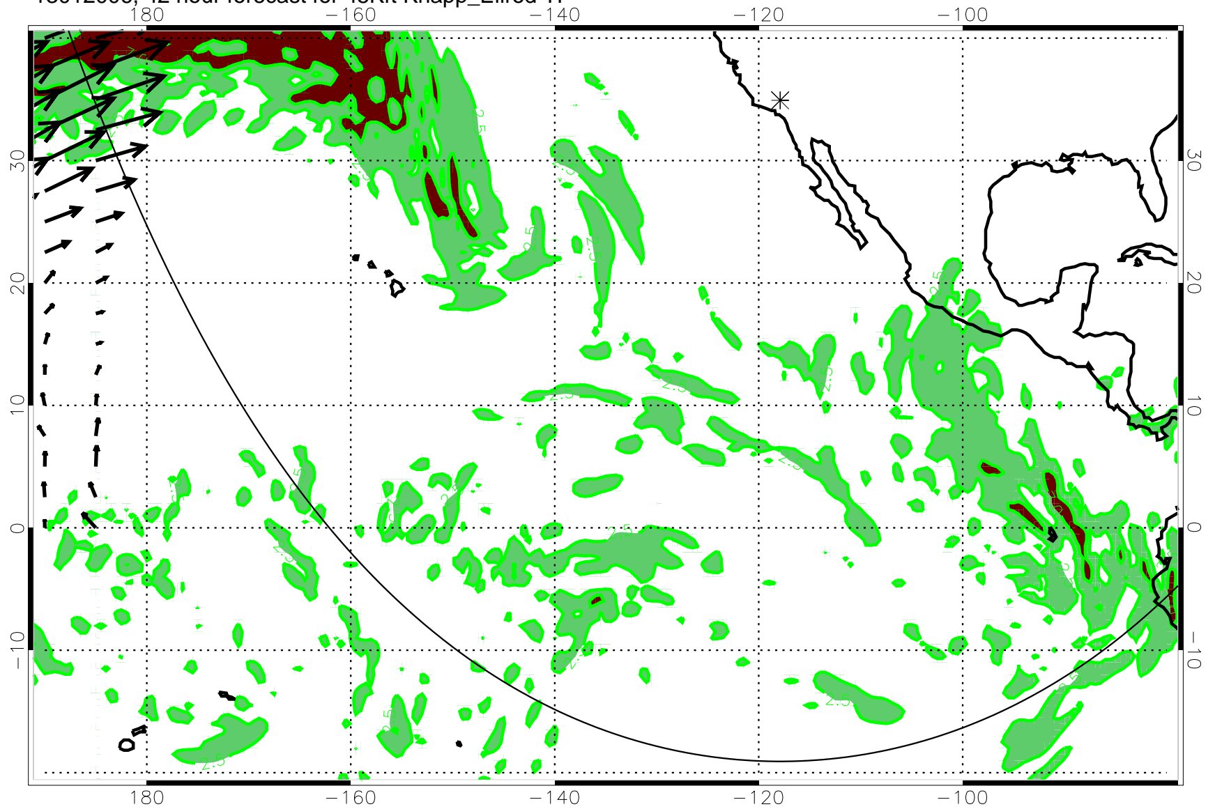
13012006, 42 hour forecast for 45Kft Knapp_Ellrod TI
