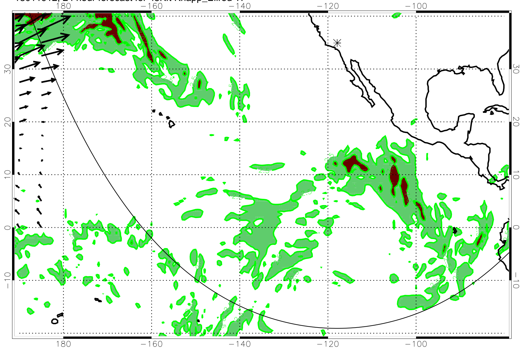
13011912, 24 hour forecast for 45Kft Knapp_Ellrod TI
