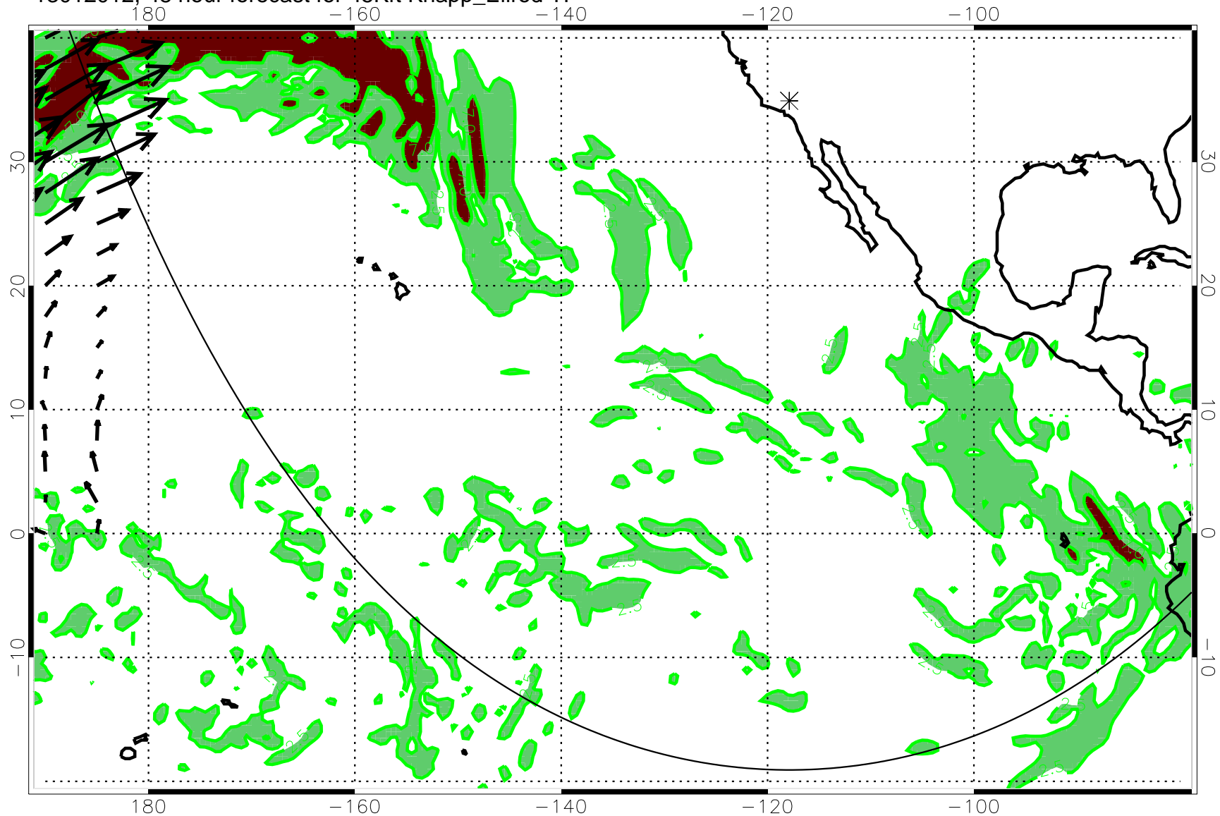
13012012, 48 hour forecast for 45Kft Knapp_Ellrod TI
