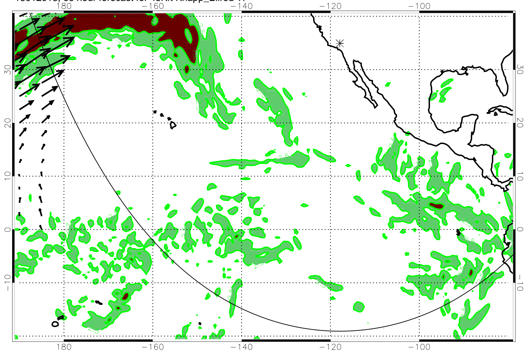
13012018, 66 hour forecast for 45Kft Knapp_Ellrod TI
