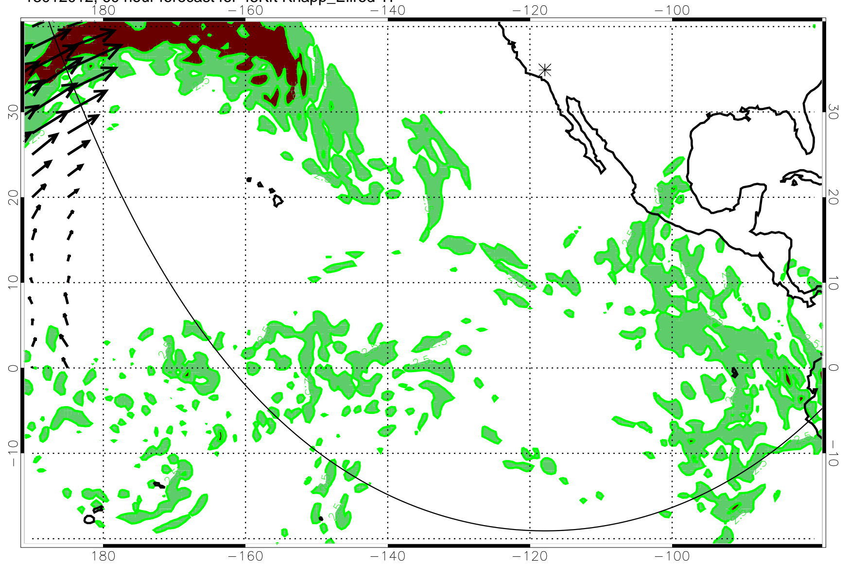
13012012, 60 hour forecast for 45Kft Knapp_Ellrod TI
