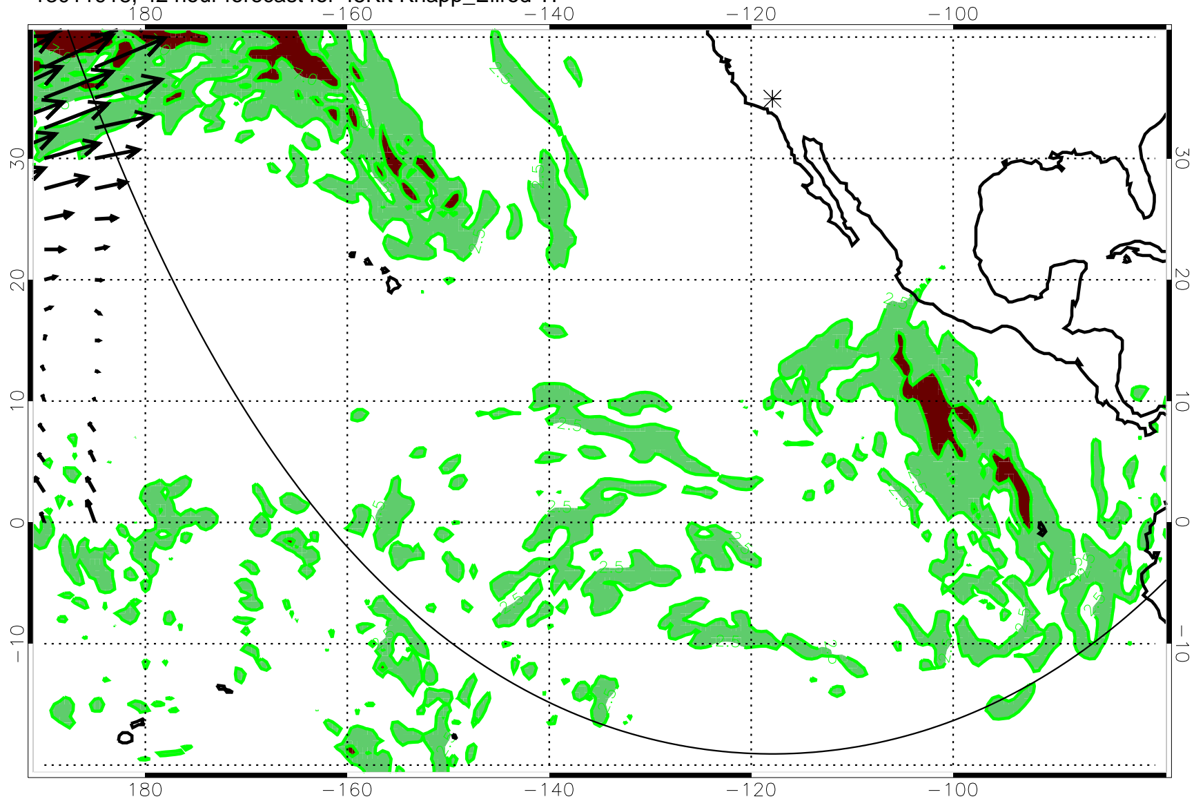
13011918, 42 hour forecast for 45Kft Knapp_Ellrod TI
