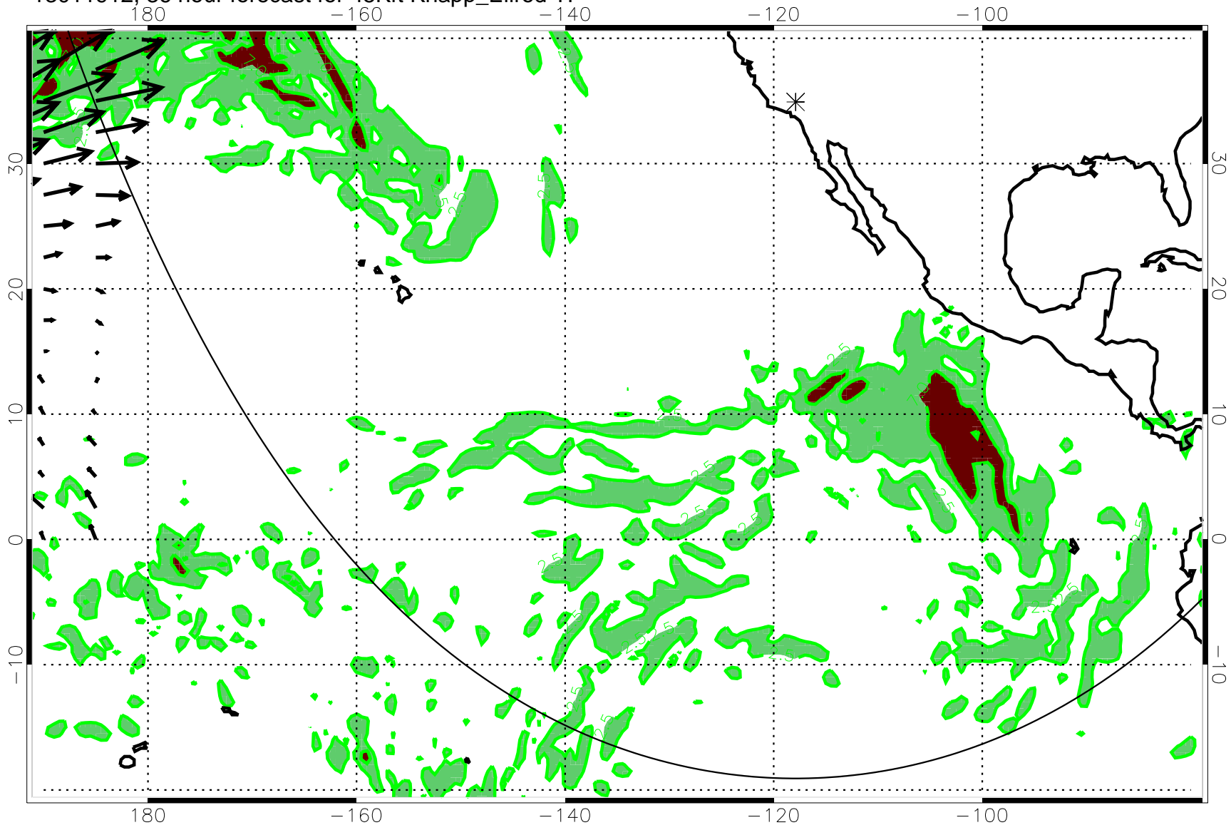
13011912, 36 hour forecast for 45Kft Knapp_Ellrod TI
