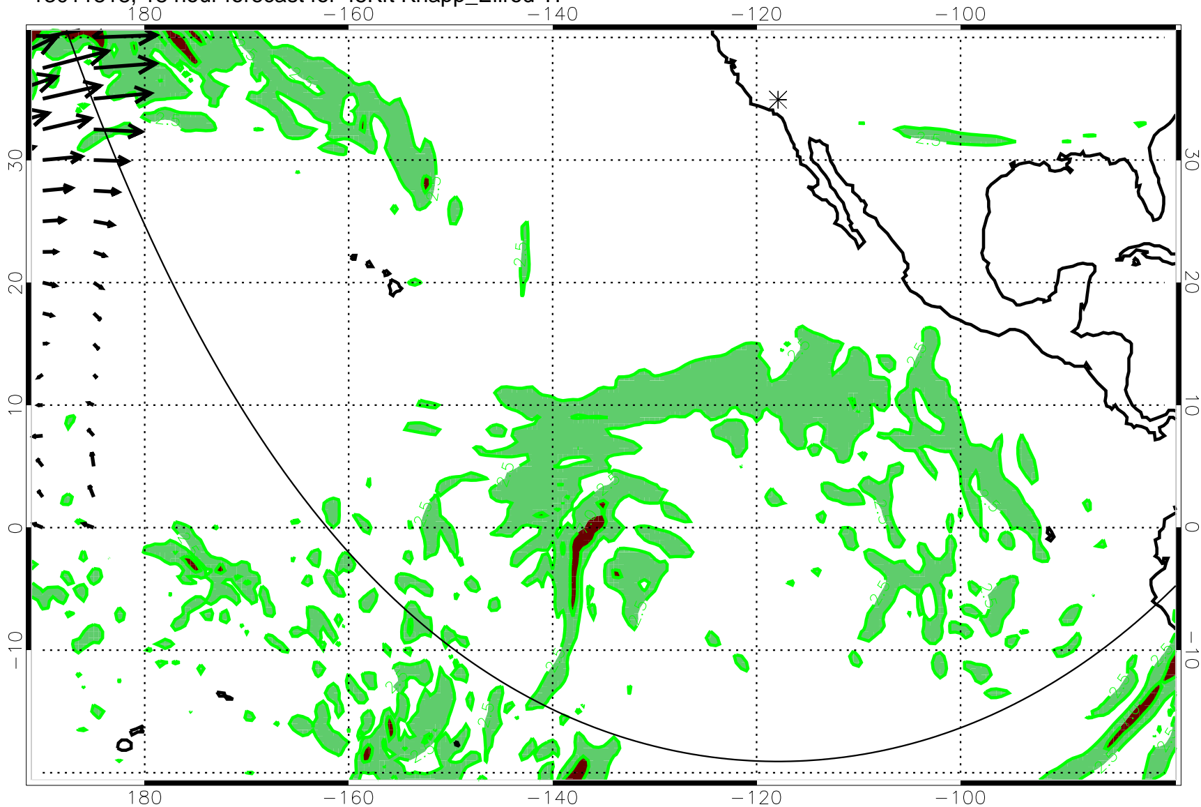
13011818, 18 hour forecast for 45Kft Knapp_Ellrod TI
