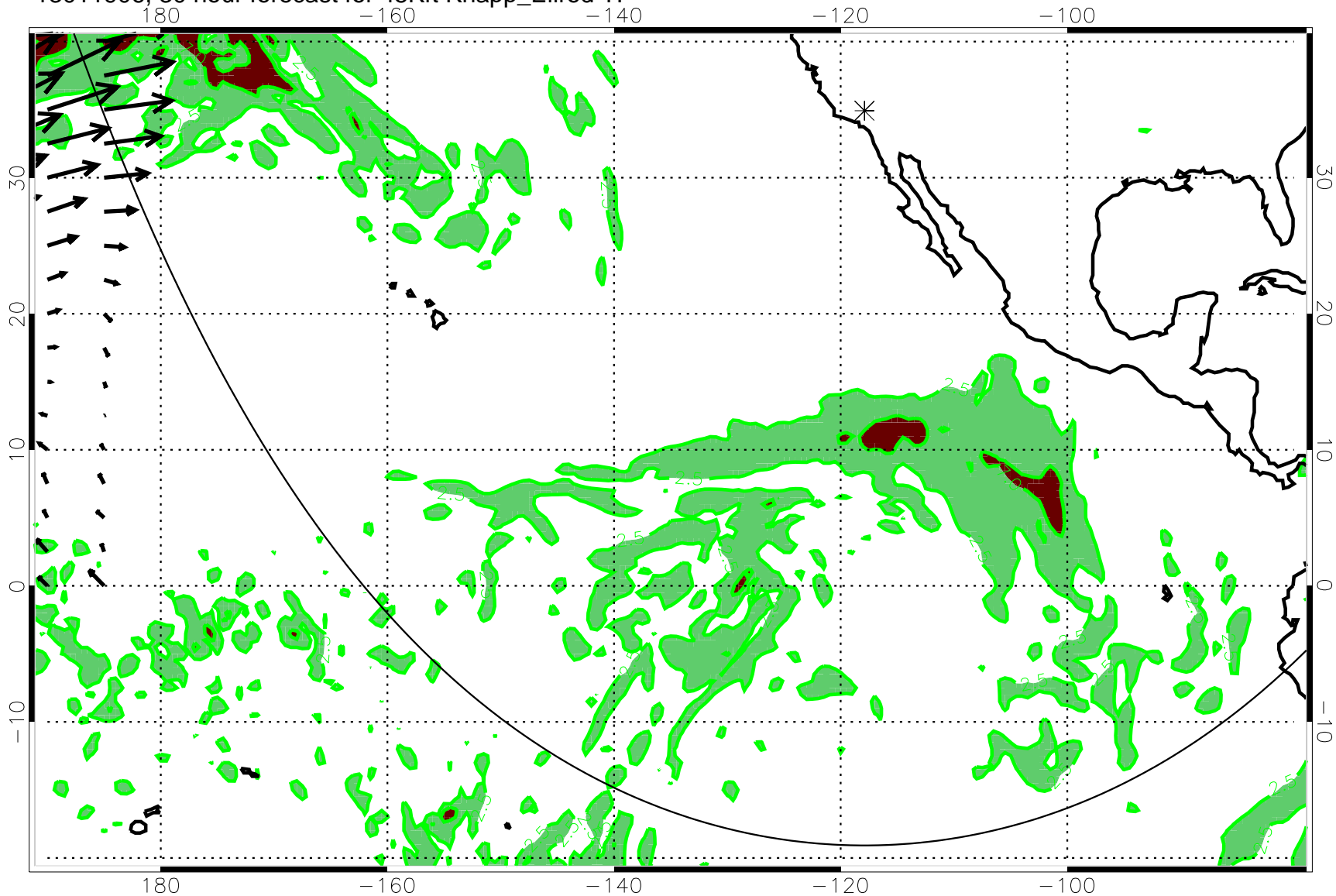
13011906, 30 hour forecast for 45Kft Knapp_Ellrod TI
