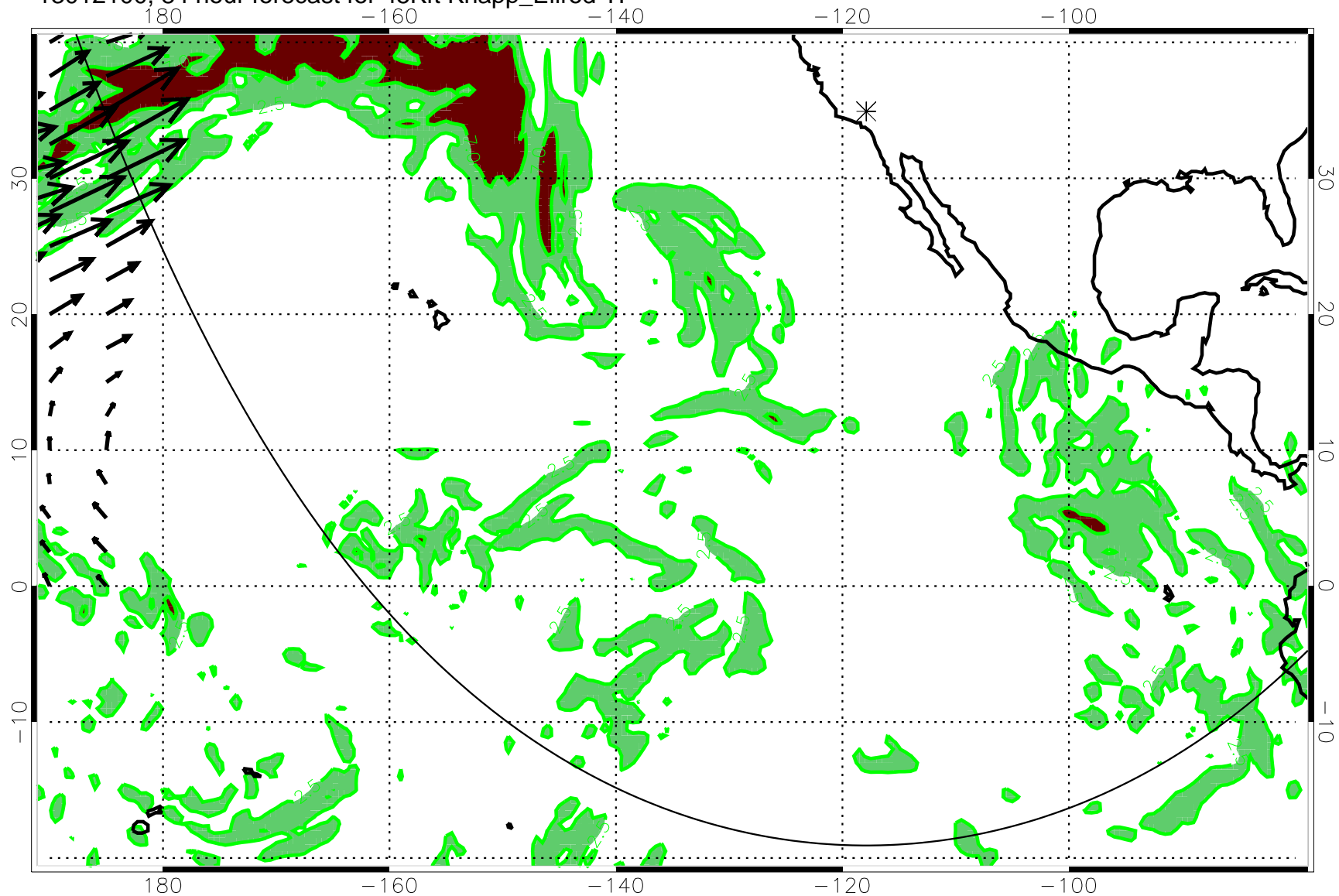
13012100, 84 hour forecast for 45Kft Knapp_Ellrod TI
