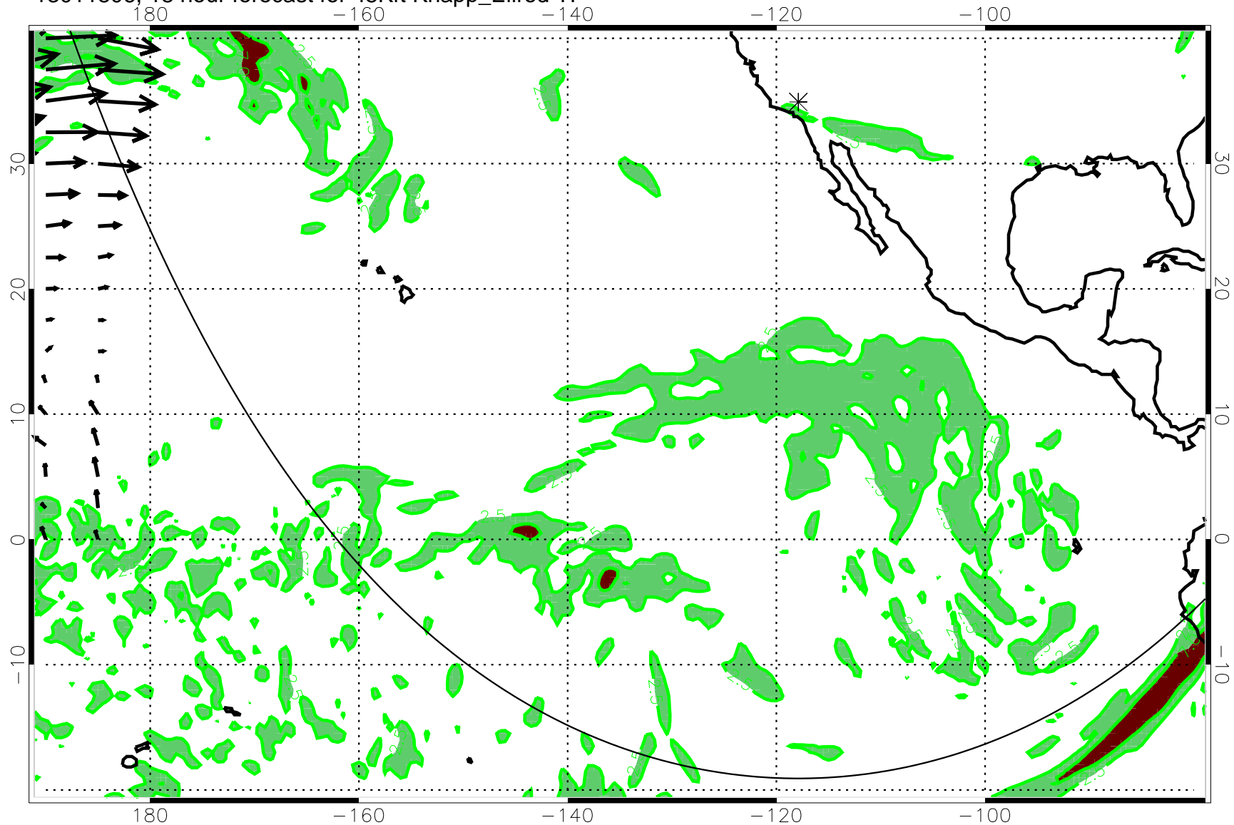
13011806, 18 hour forecast for 45Kft Knapp_Ellrod TI
