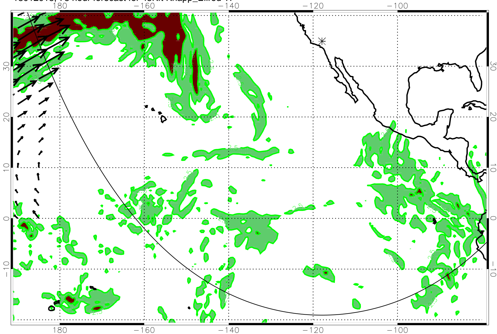
13012018, 78 hour forecast for 45Kft Knapp_Ellrod TI
