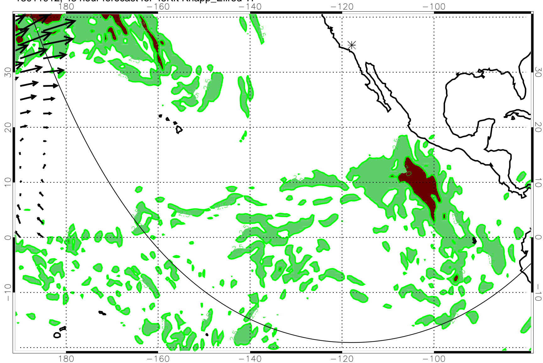
13011912, 48 hour forecast for 45Kft Knapp_Ellrod TI
