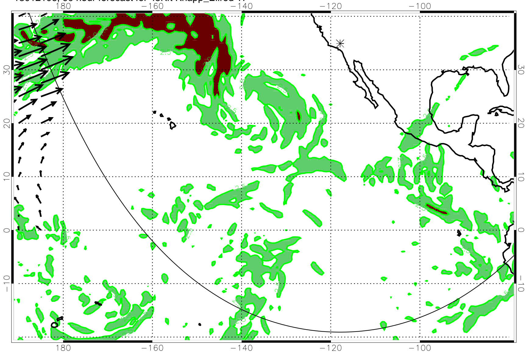
13012106, 90 hour forecast for 45Kft Knapp_Ellrod TI
