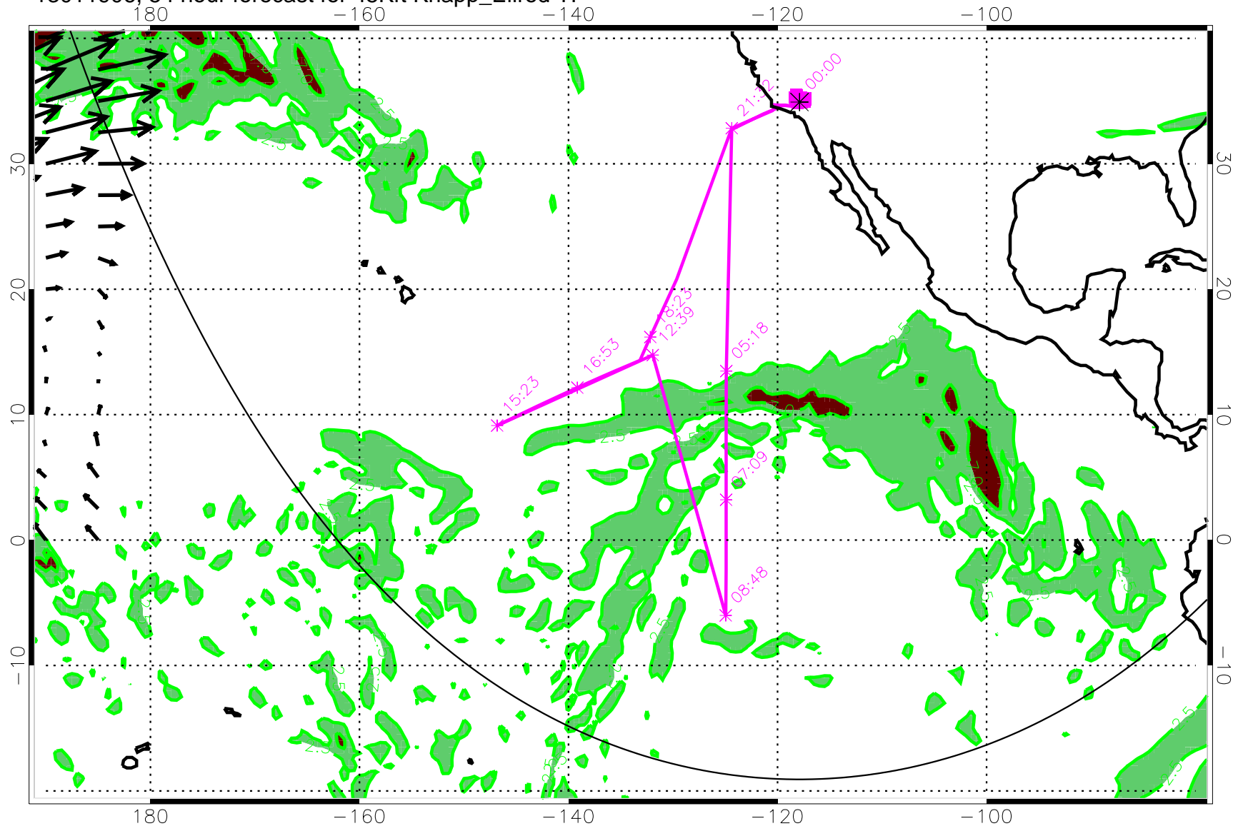
13011906, 54 hour forecast for 45Kft Knapp_Ellrod TI
