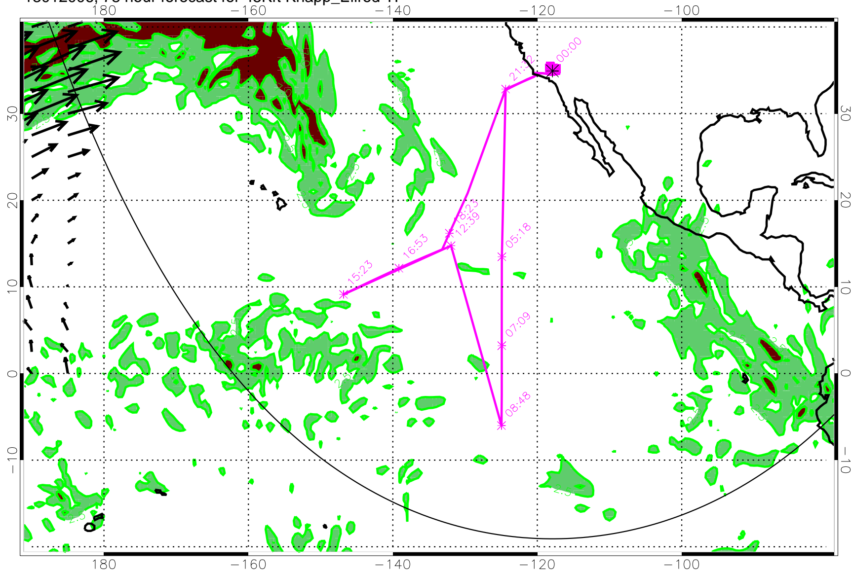
13012006, 78 hour forecast for 45Kft Knapp_Ellrod TI
