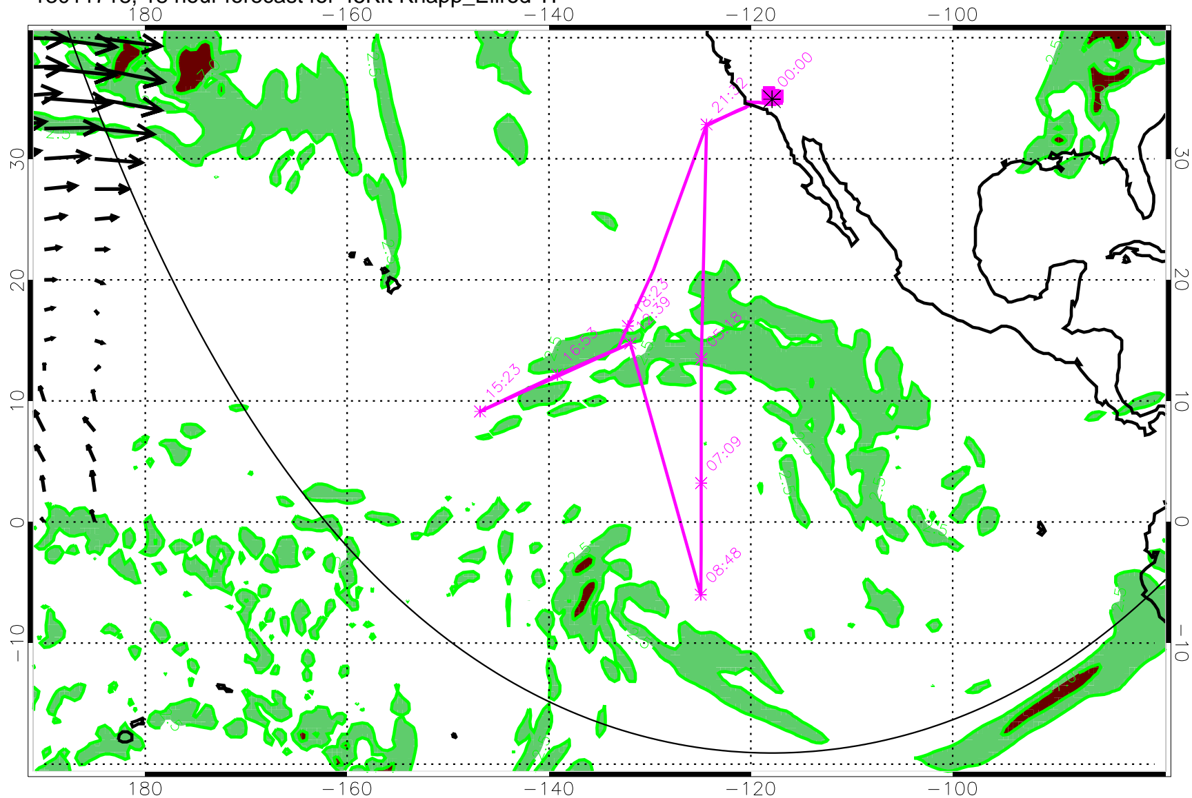
13011718, 18 hour forecast for 45Kft Knapp_Ellrod TI
