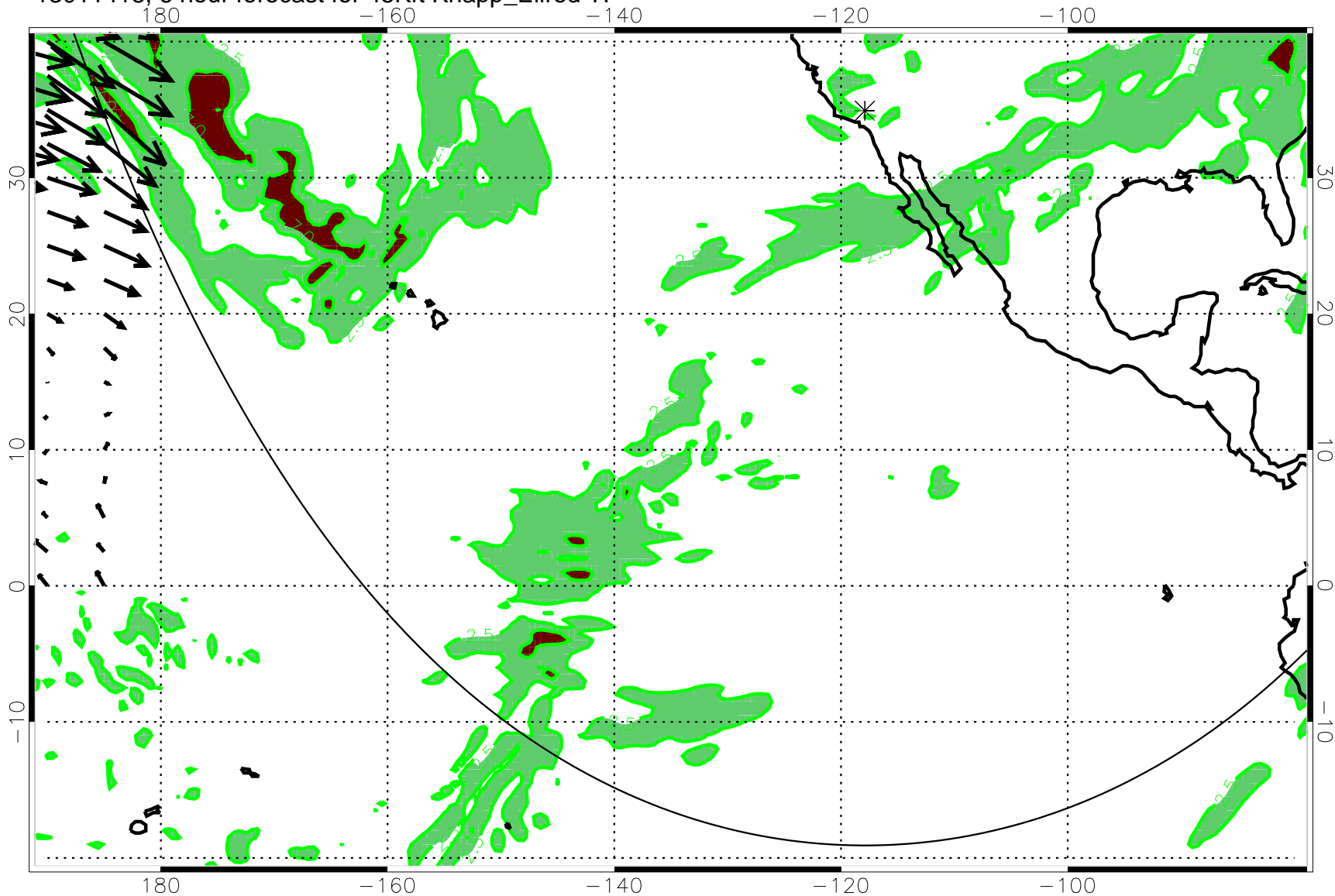
13011418, 6 hour forecast for 45Kft Knapp_Ellrod TI
