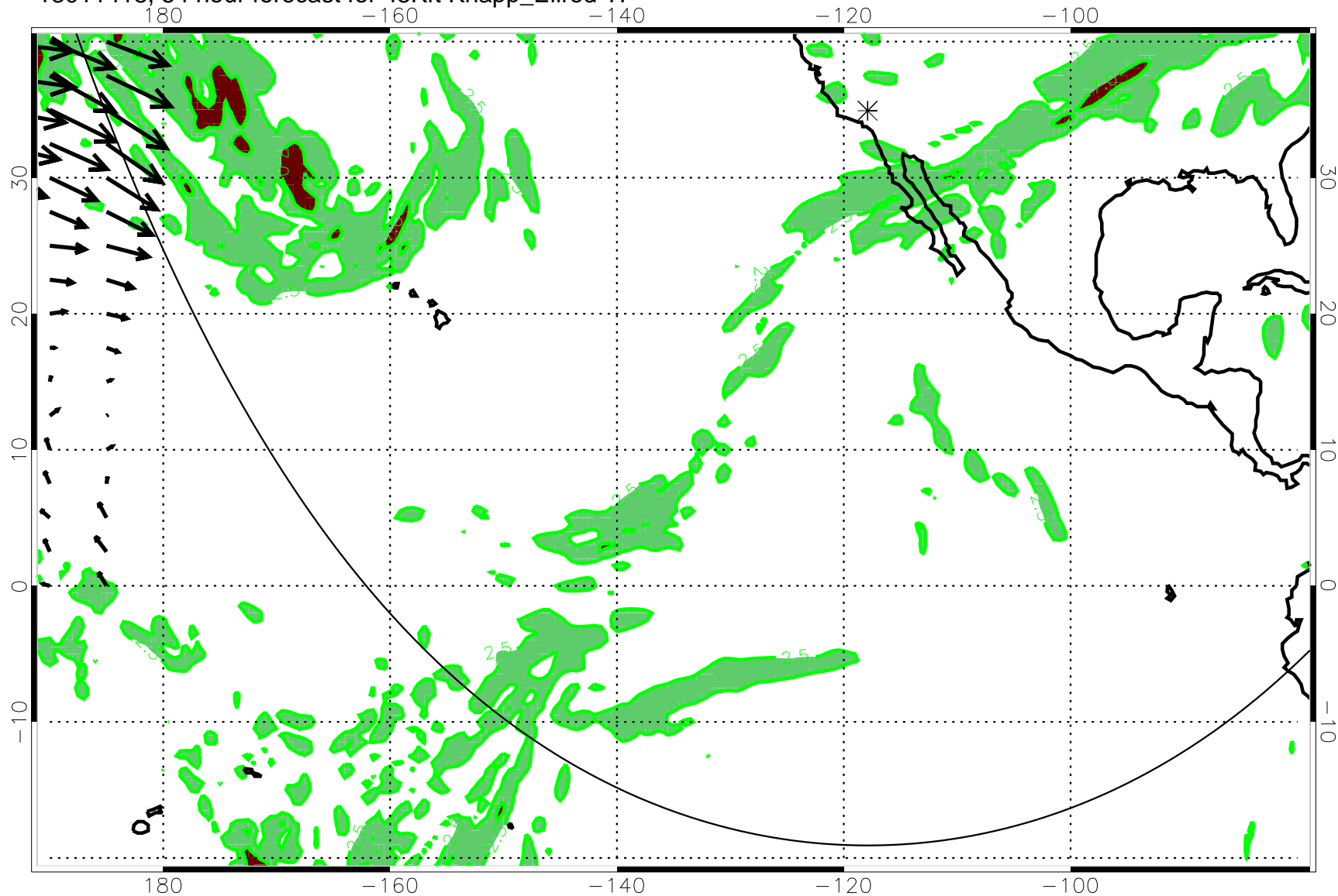
13011418, 54 hour forecast for 45Kft Knapp_Ellrod TI
