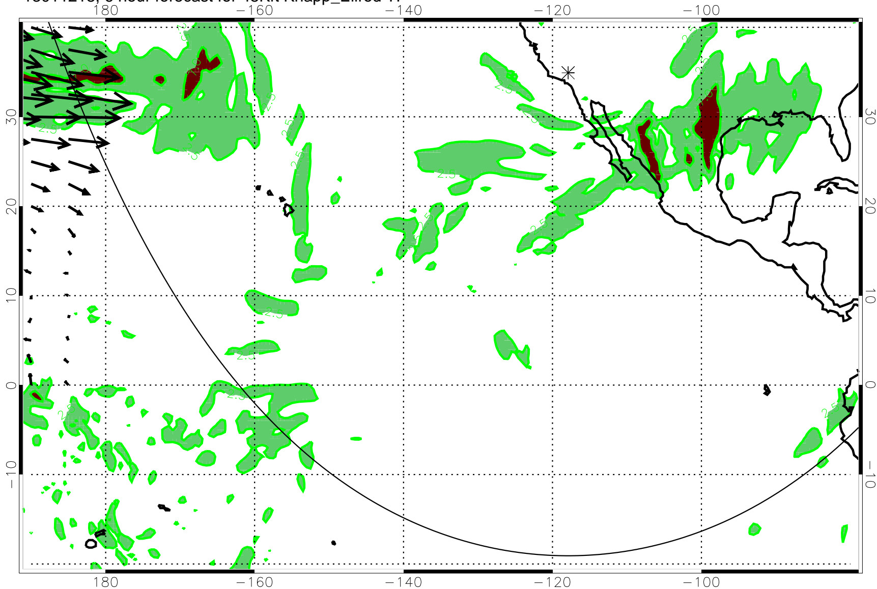
13011218, 6 hour forecast for 45Kft Knapp_Ellrod TI
