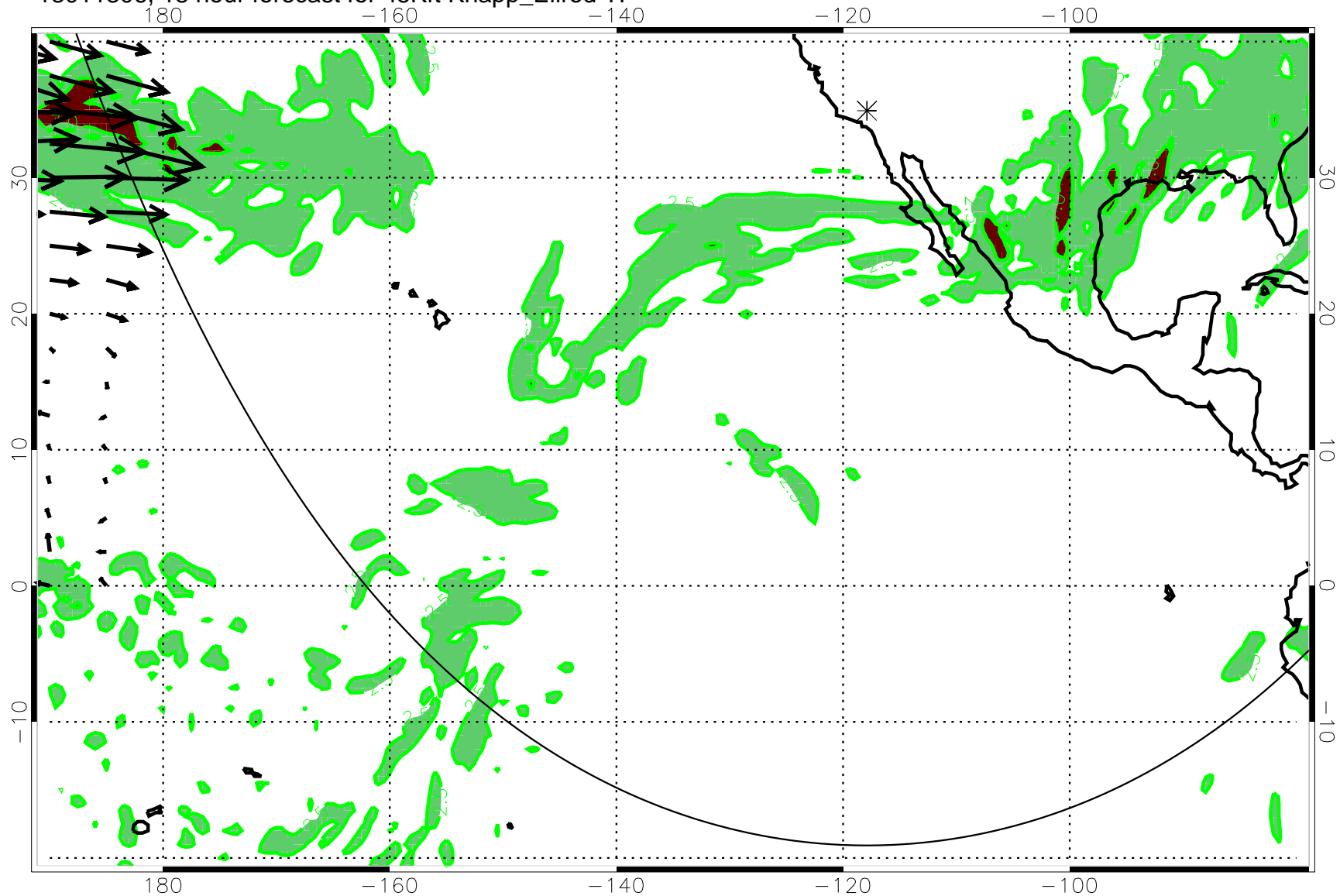
13011306, 18 hour forecast for 45Kft Knapp_Ellrod TI
