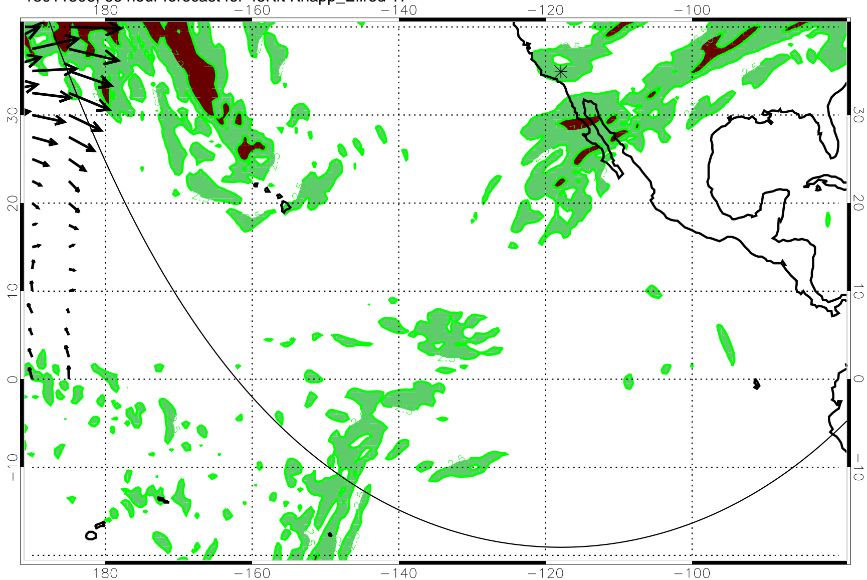
13011506, 66 hour forecast for 45Kft Knapp_Ellrod TI
