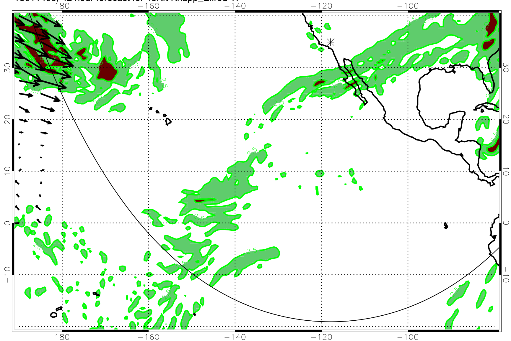
13011406, 42 hour forecast for 45Kft Knapp_Ellrod TI
