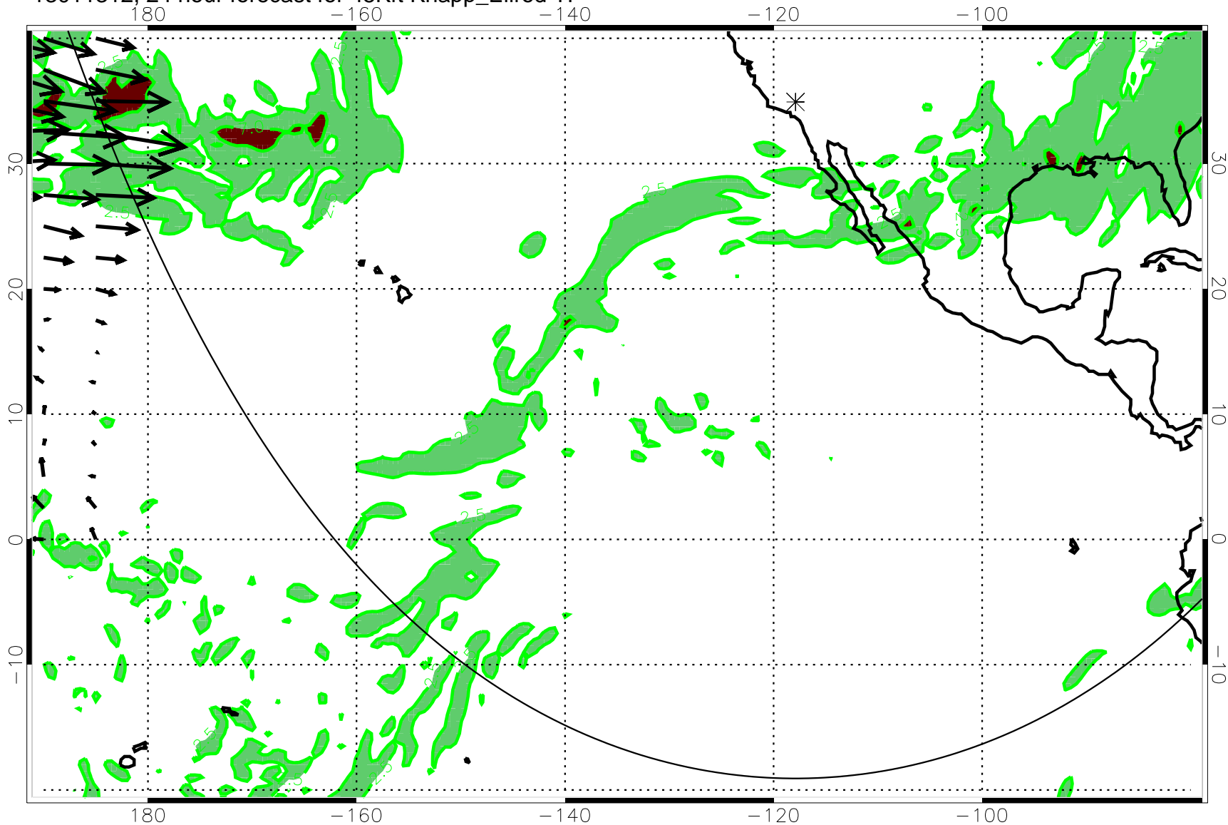
13011312, 24 hour forecast for 45Kft Knapp_Ellrod TI
