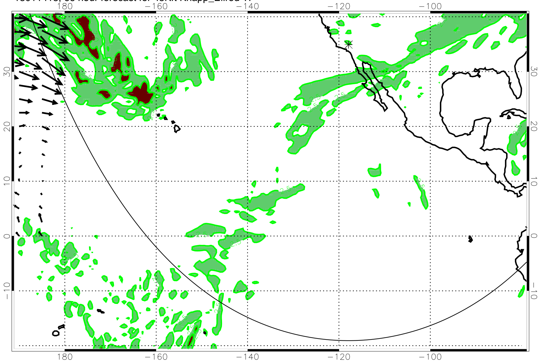
13011418, 66 hour forecast for 45Kft Knapp_Ellrod TI
