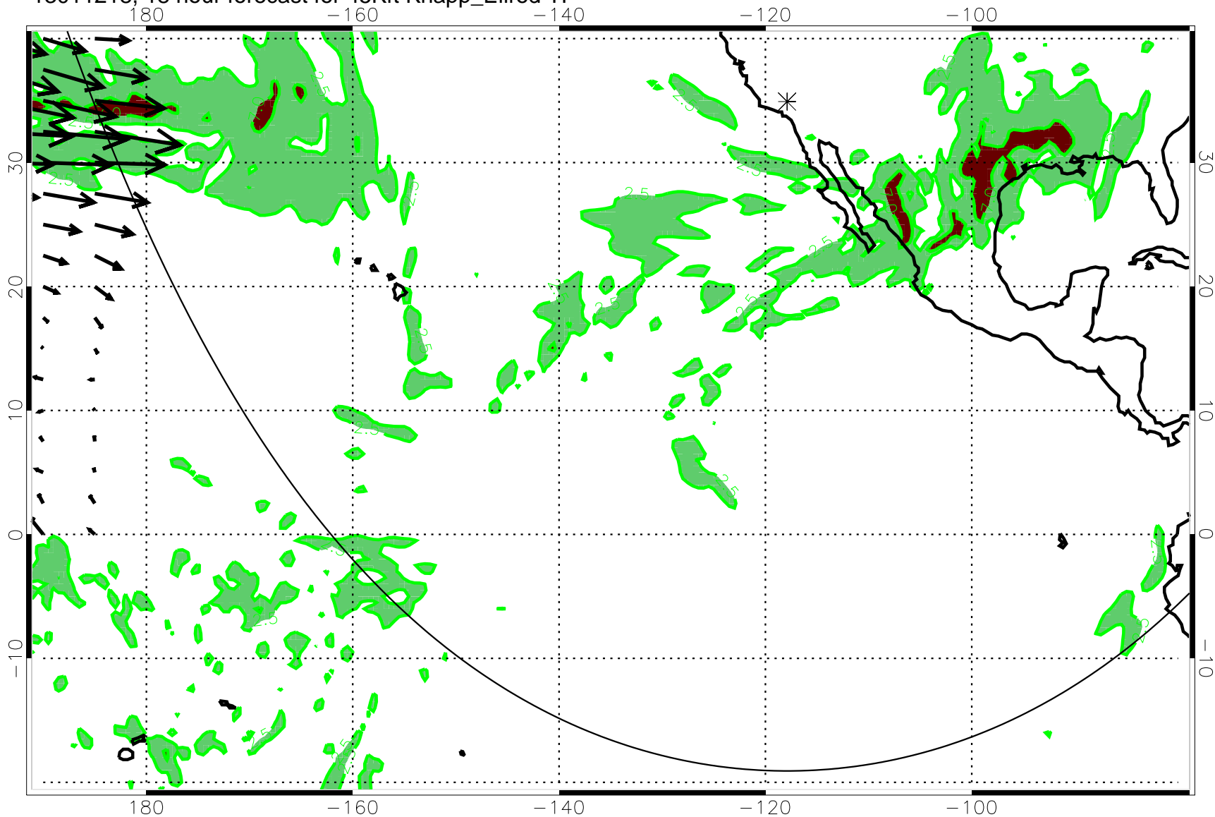
13011218, 18 hour forecast for 45Kft Knapp_Ellrod TI
