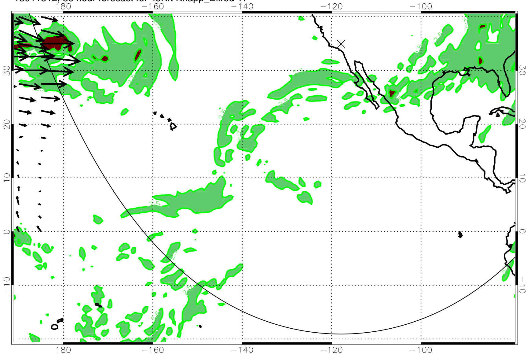
13011312, 36 hour forecast for 45Kft Knapp_Ellrod TI
