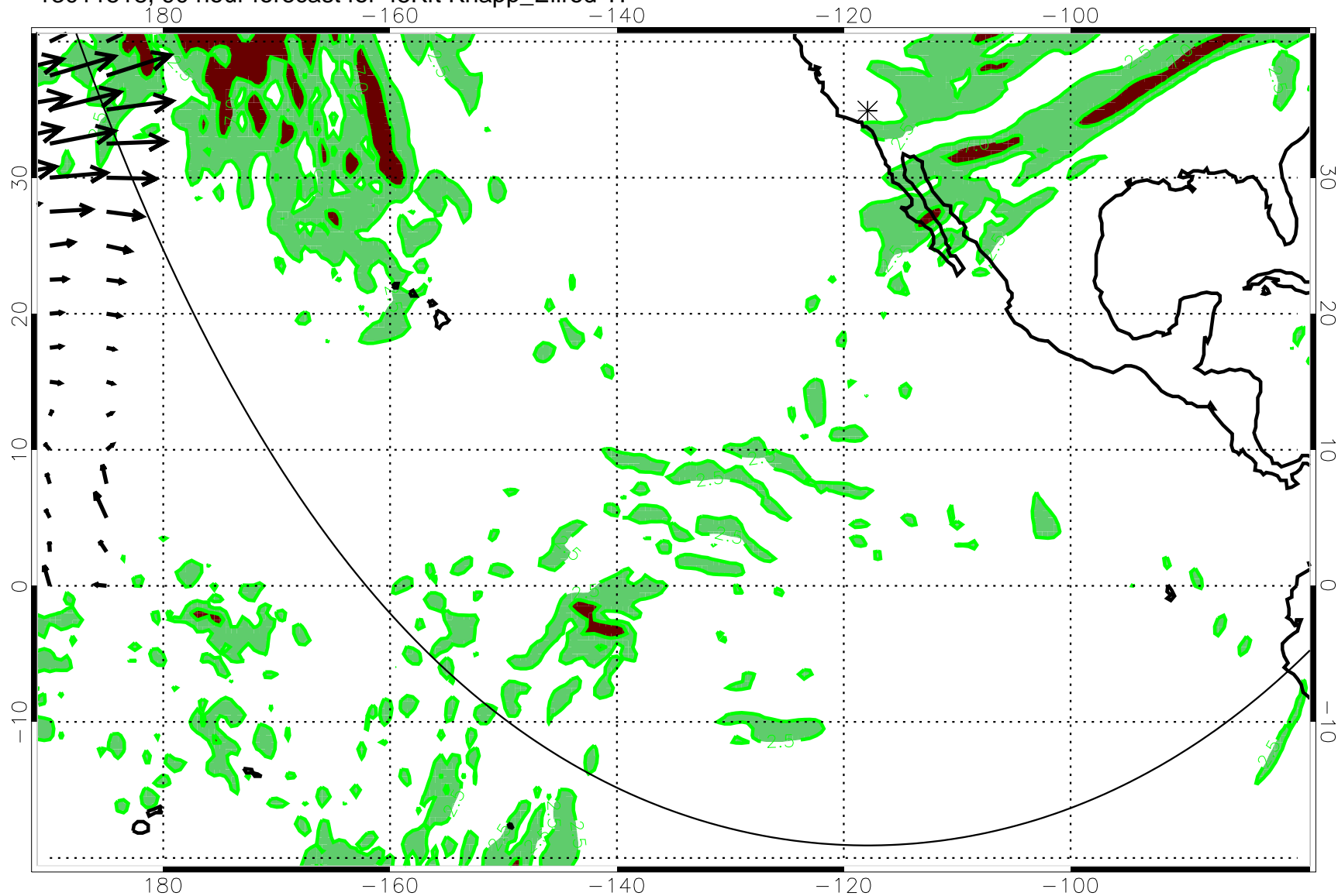
13011518, 90 hour forecast for 45Kft Knapp_Ellrod TI
