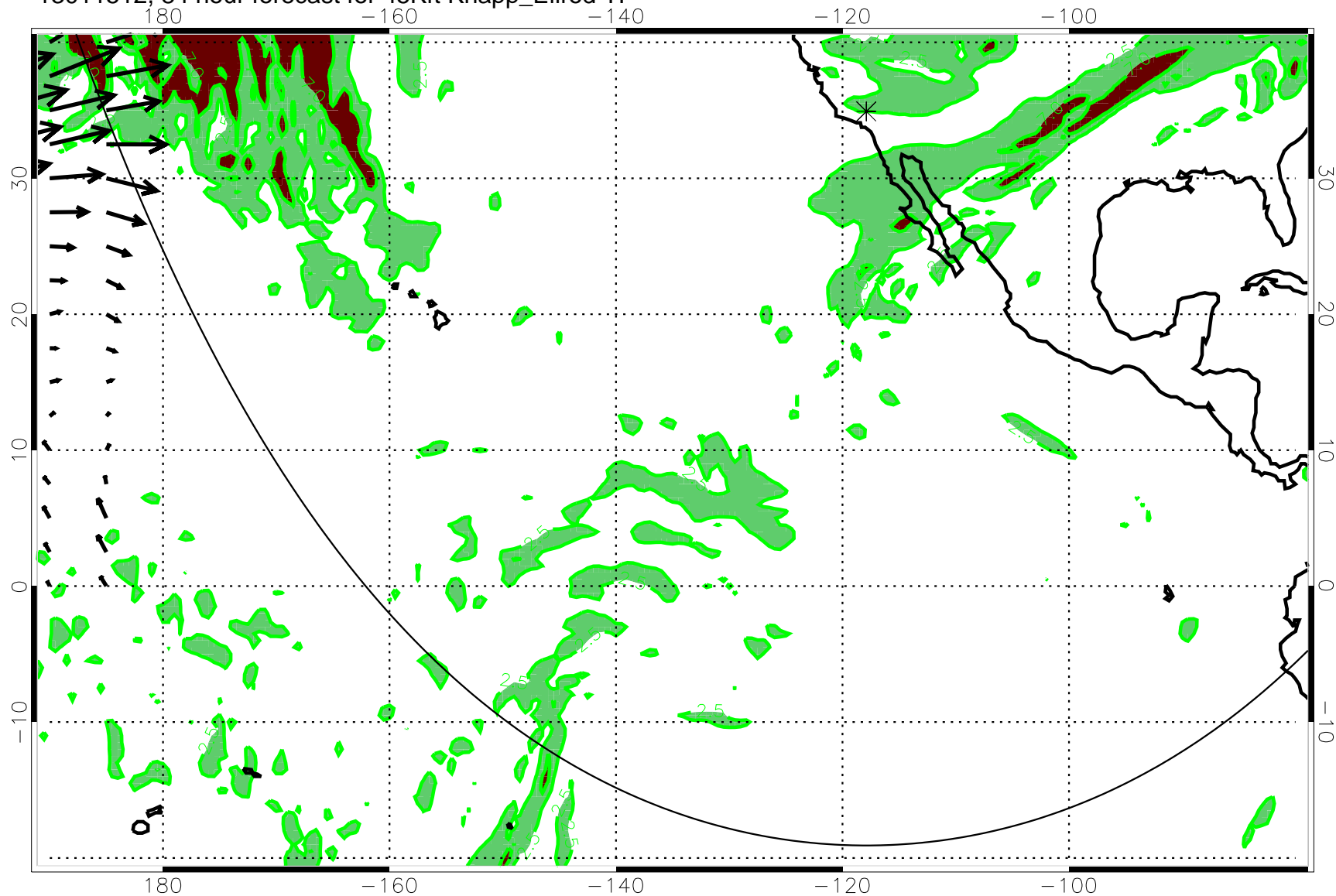
13011512, 84 hour forecast for 45Kft Knapp_Ellrod TI
