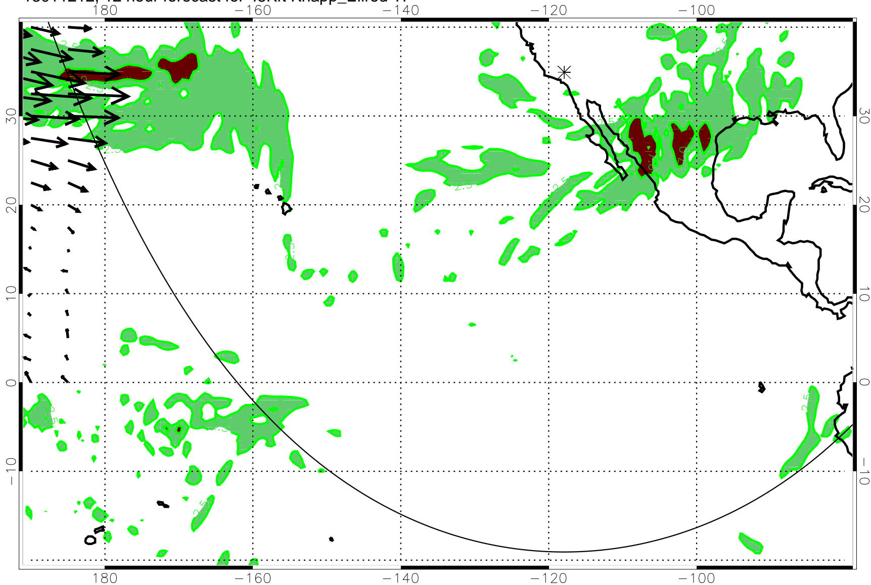
13011212, 12 hour forecast for 45Kft Knapp_Ellrod TI
