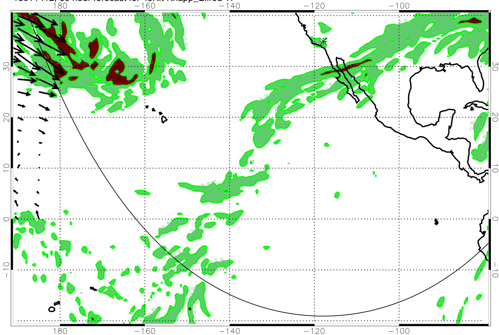
13011412, 60 hour forecast for 45Kft Knapp_Ellrod TI
