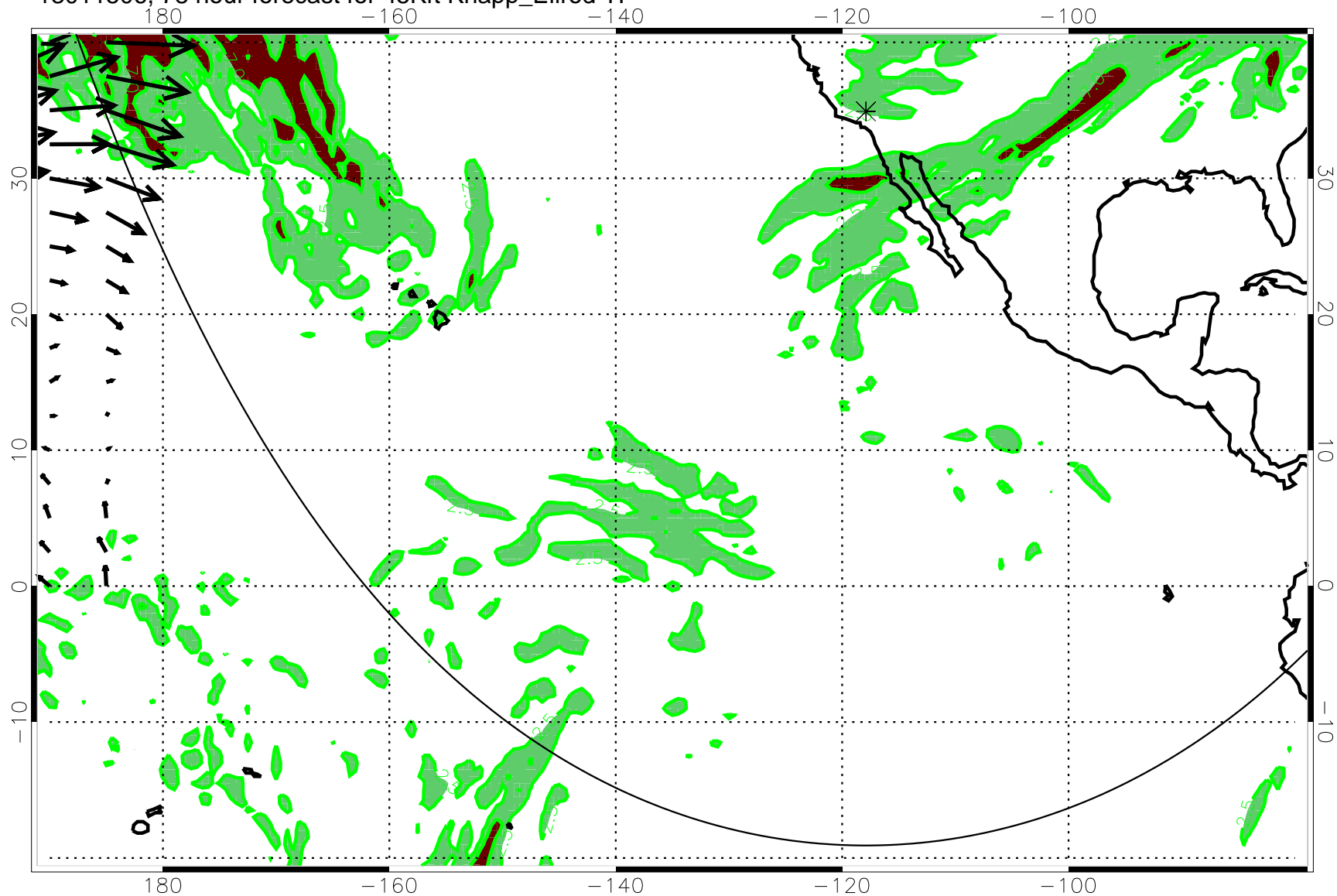
13011506, 78 hour forecast for 45Kft Knapp_Ellrod TI
