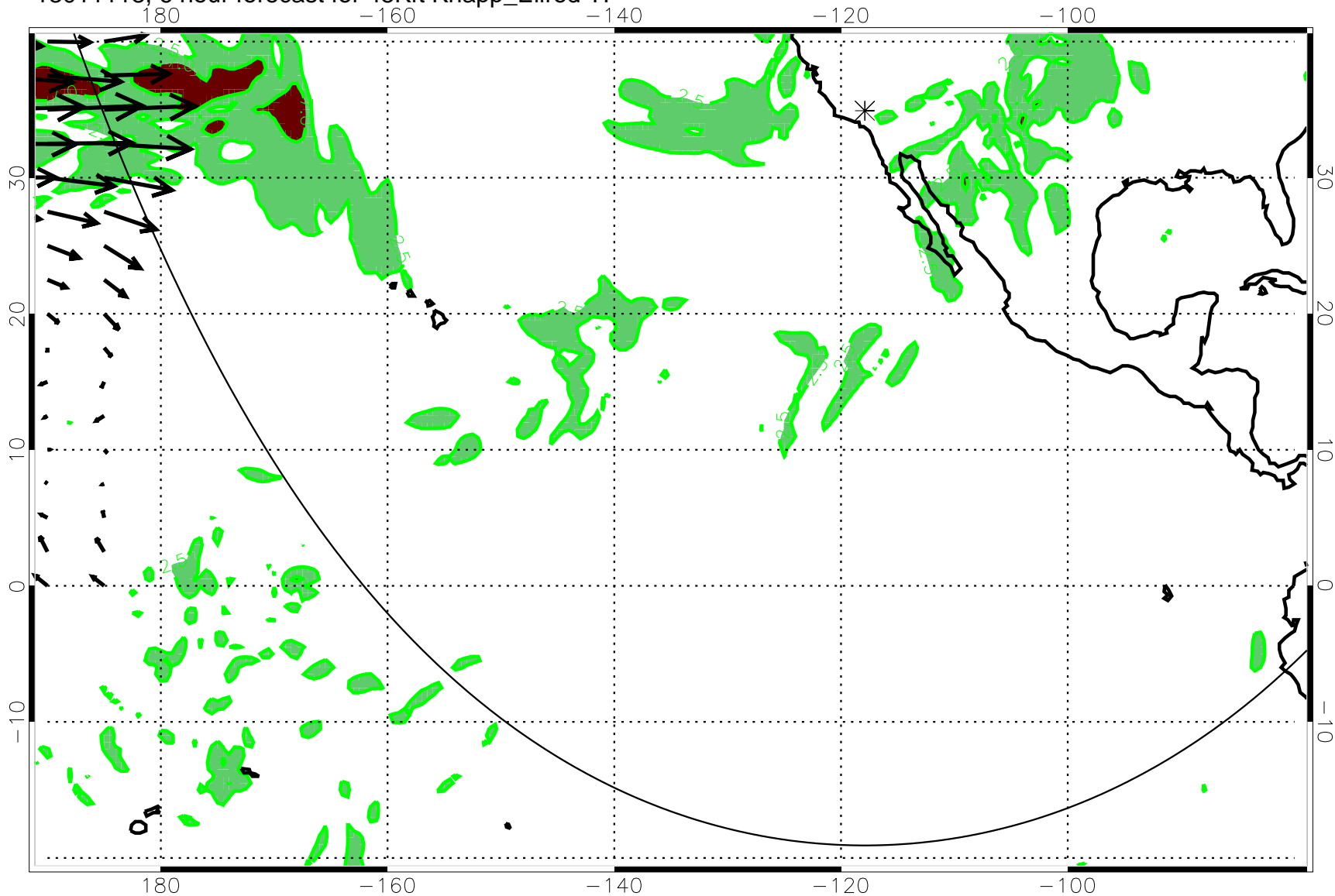
13011118, 6 hour forecast for 45Kft Knapp_Ellrod TI
