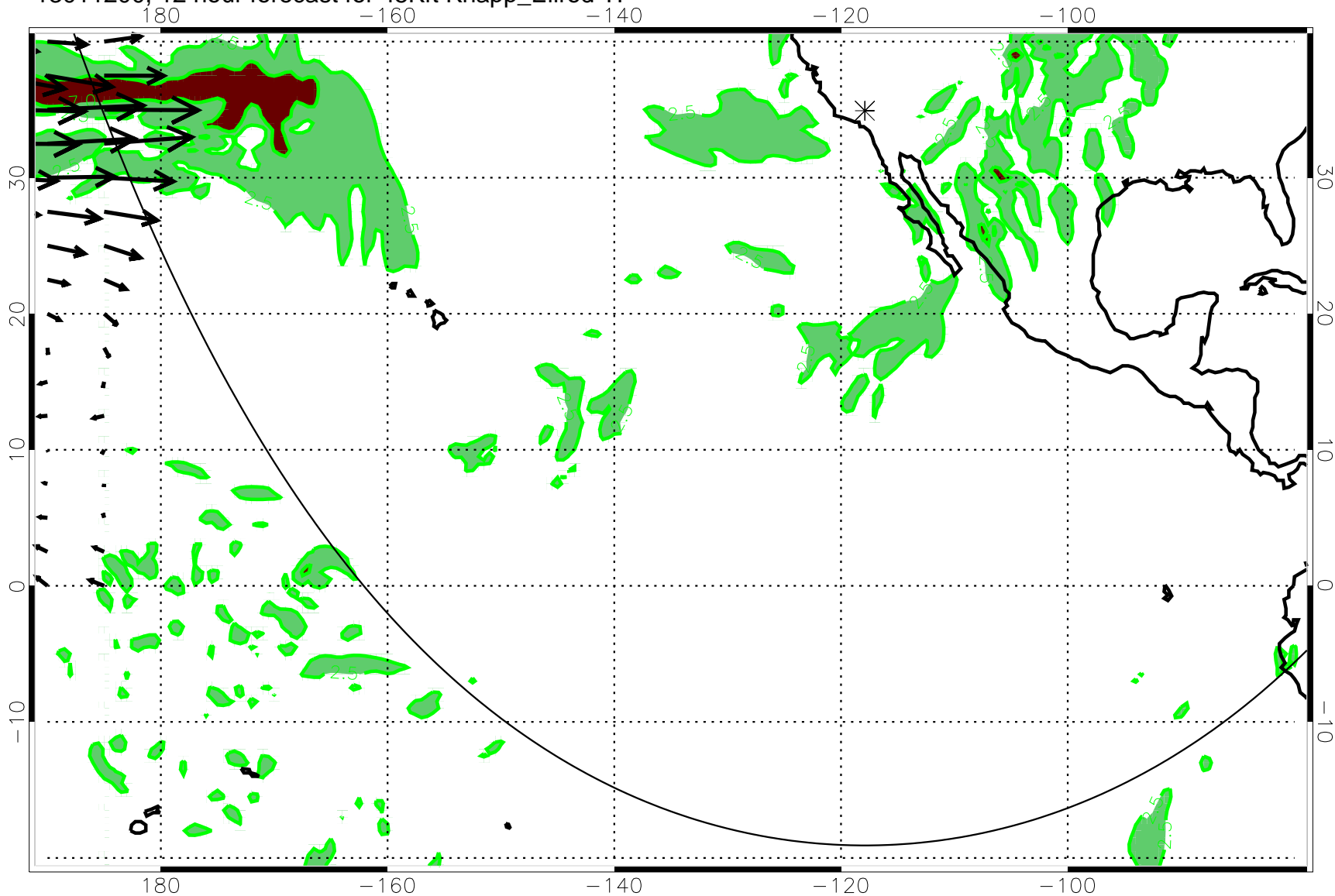
13011200, 12 hour forecast for 45Kft Knapp_Ellrod TI
