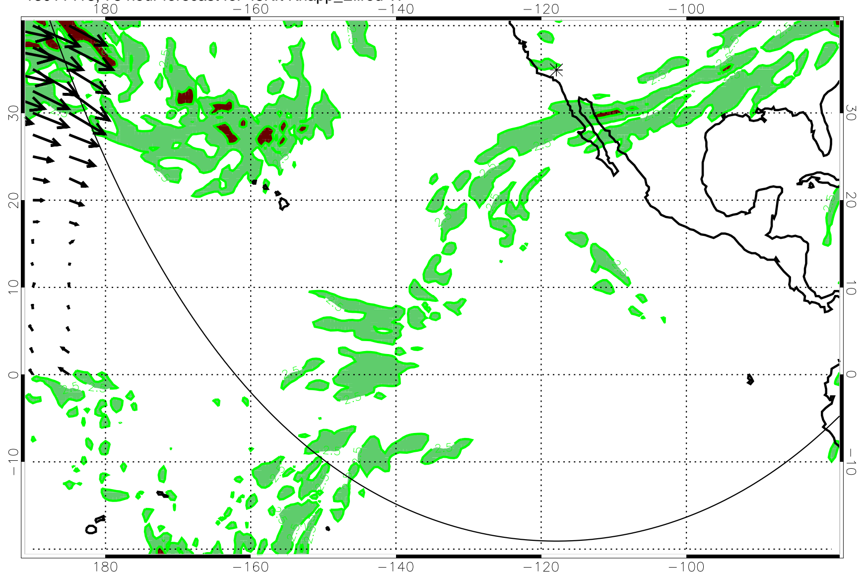
13011418, 78 hour forecast for 45Kft Knapp_Ellrod TI
