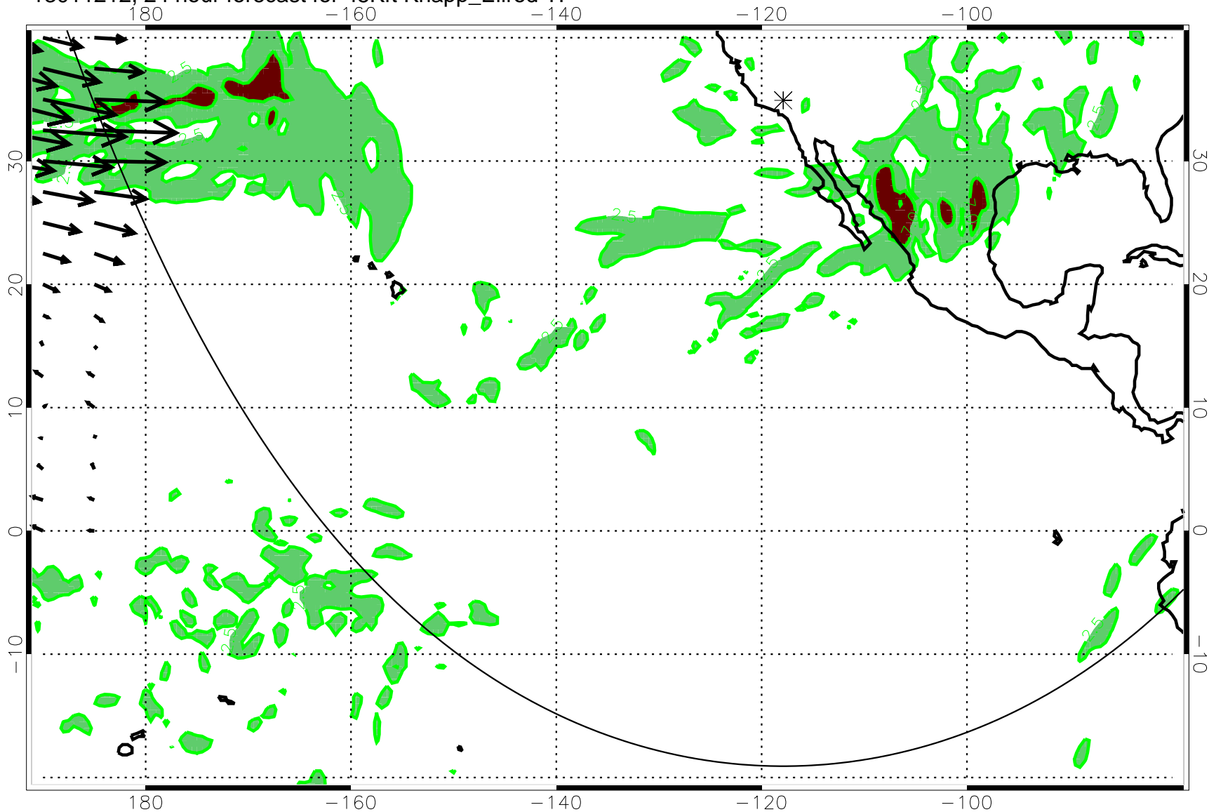
13011212, 24 hour forecast for 45Kft Knapp_Ellrod TI
