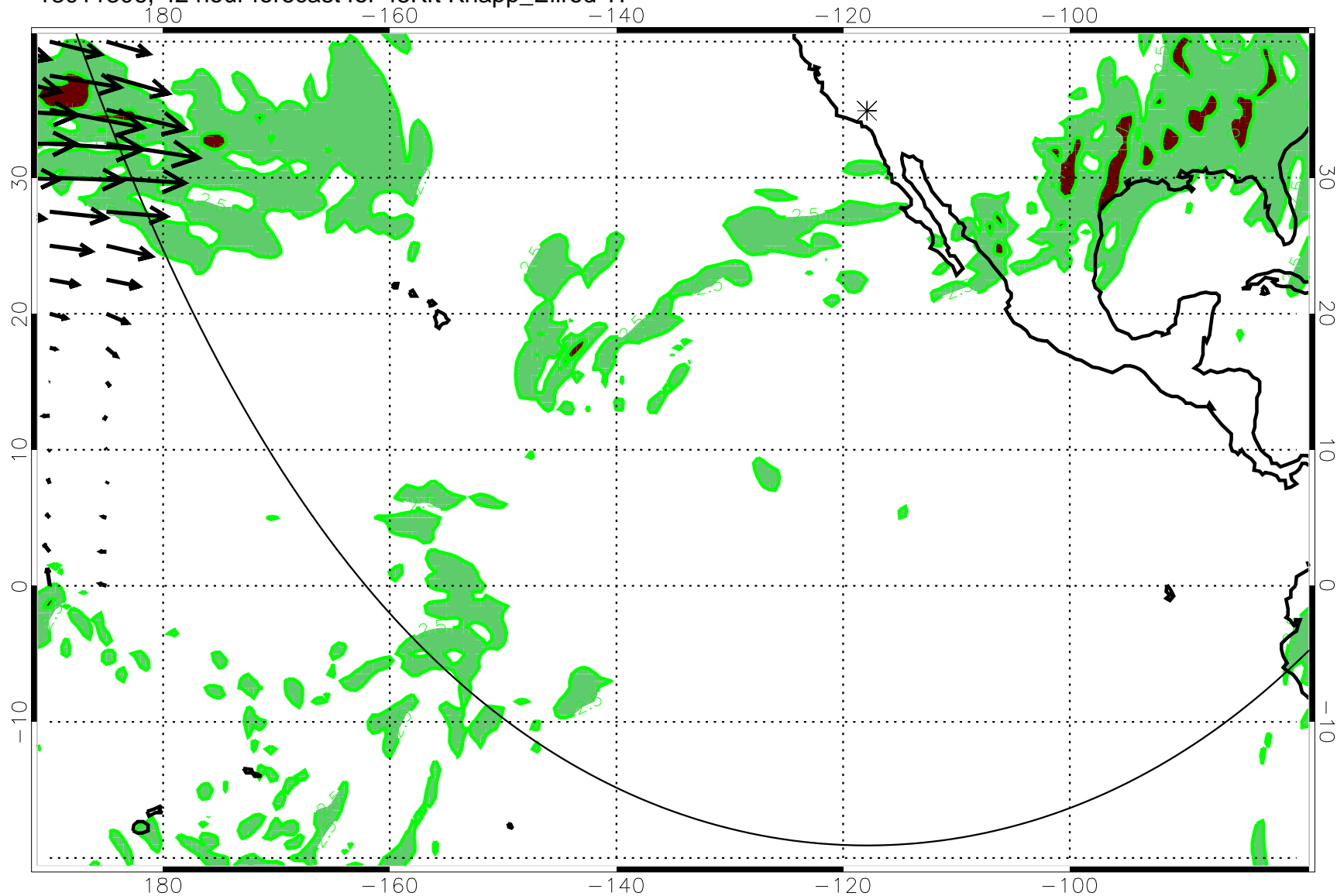
13011306, 42 hour forecast for 45Kft Knapp_Ellrod TI
