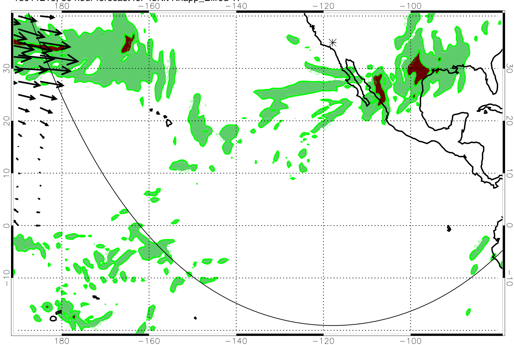
13011218, 30 hour forecast for 45Kft Knapp_Ellrod TI
