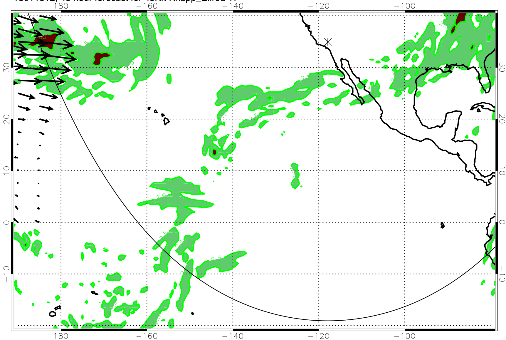
13011312, 48 hour forecast for 45Kft Knapp_Ellrod TI
