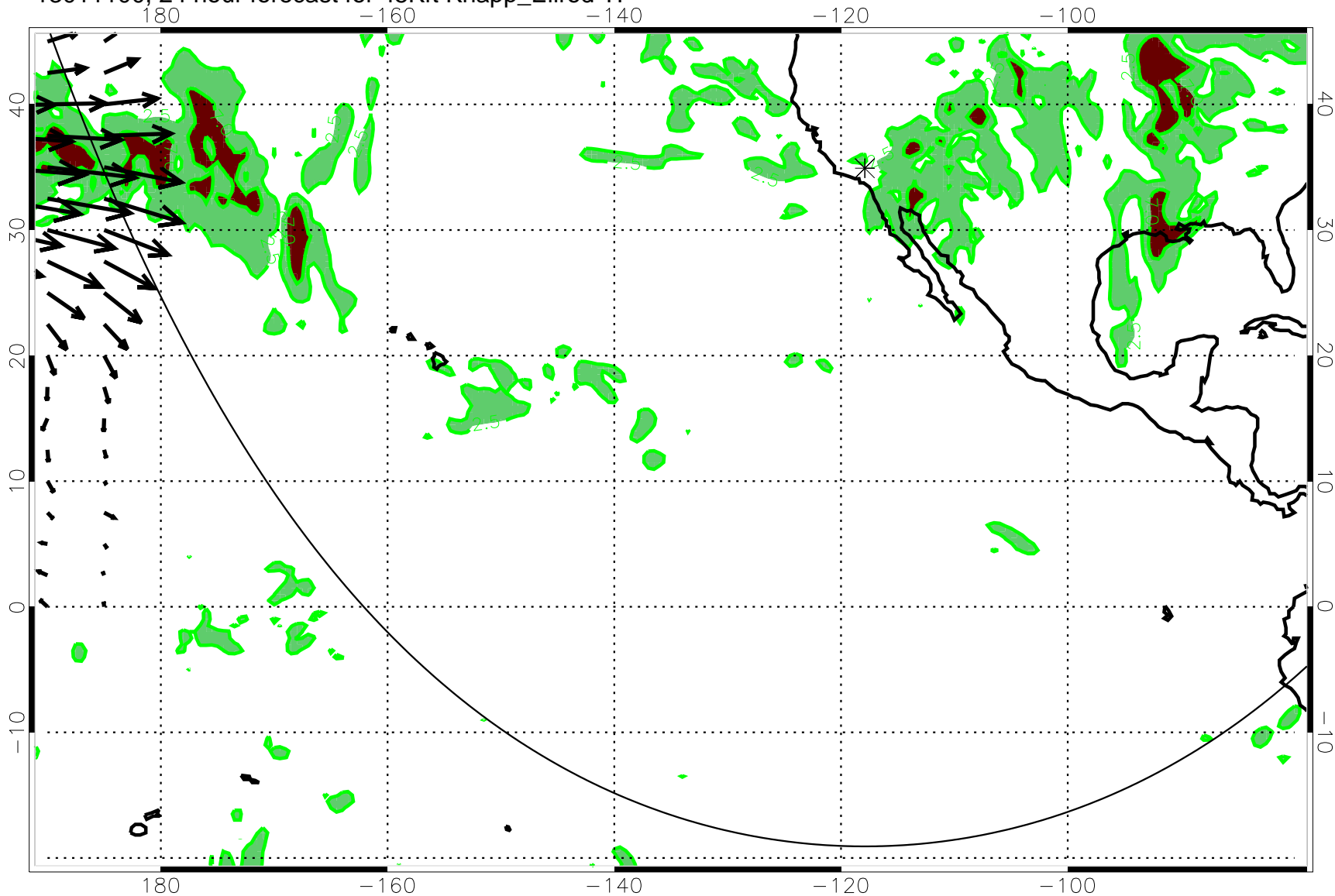
13011100, 24 hour forecast for 45Kft Knapp_Ellrod TI
