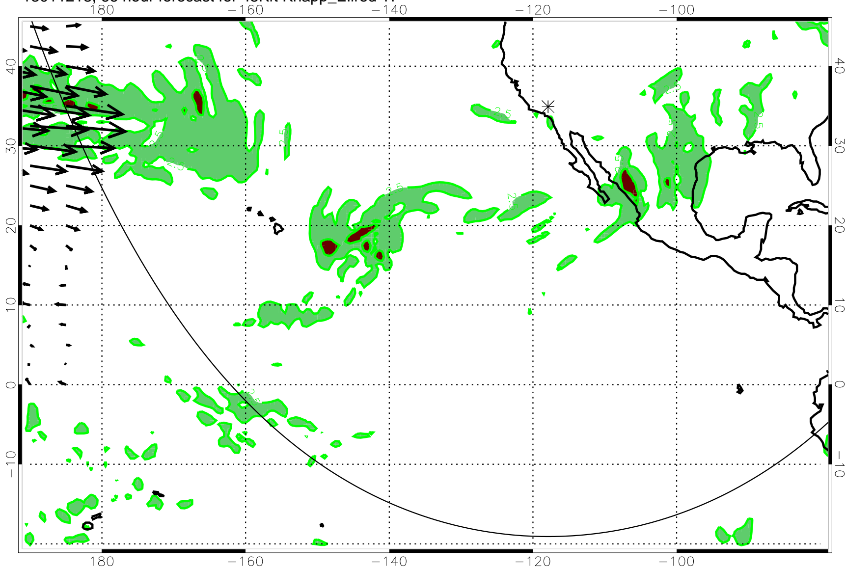
13011218, 66 hour forecast for 45Kft Knapp_Ellrod TI
