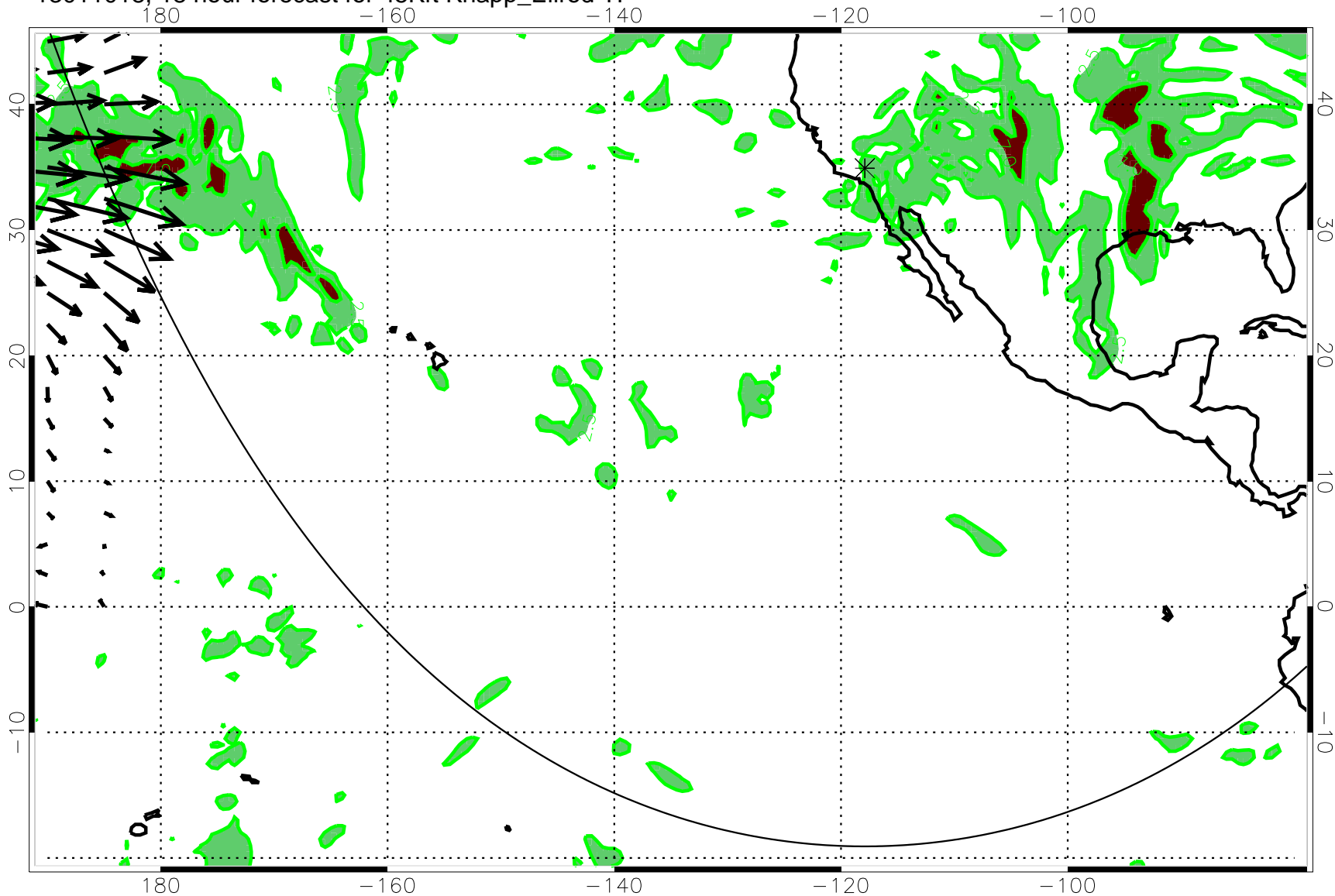
13011018, 18 hour forecast for 45Kft Knapp_Ellrod TI
