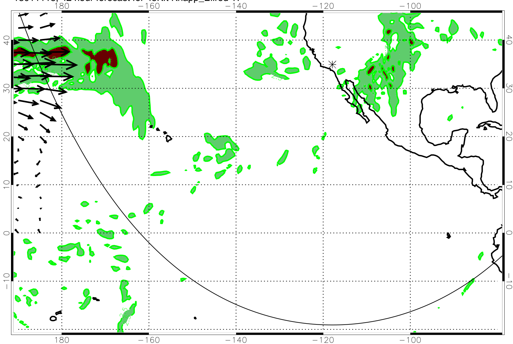
13011118, 42 hour forecast for 45Kft Knapp_Ellrod TI
