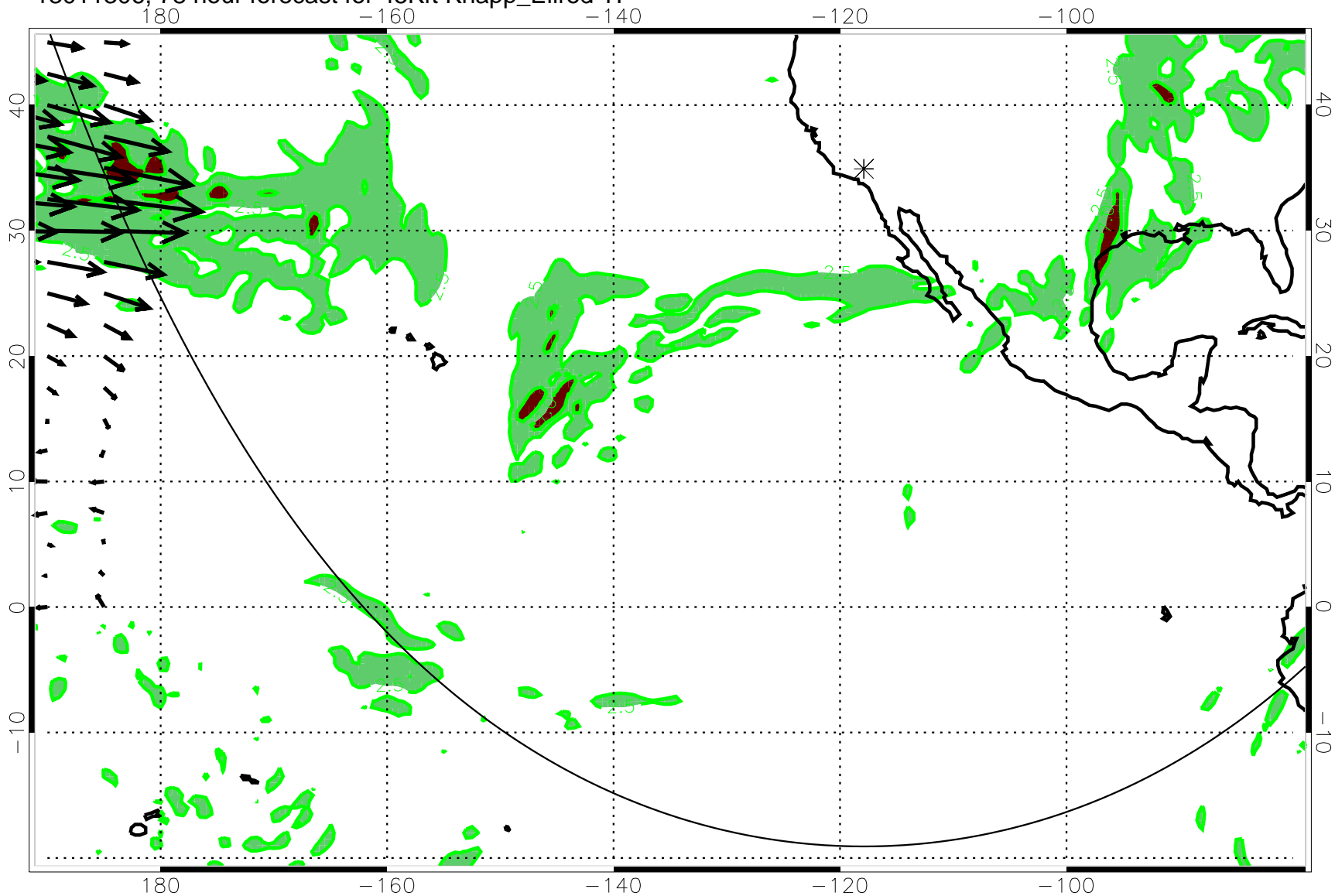
13011306, 78 hour forecast for 45Kft Knapp_Ellrod TI
