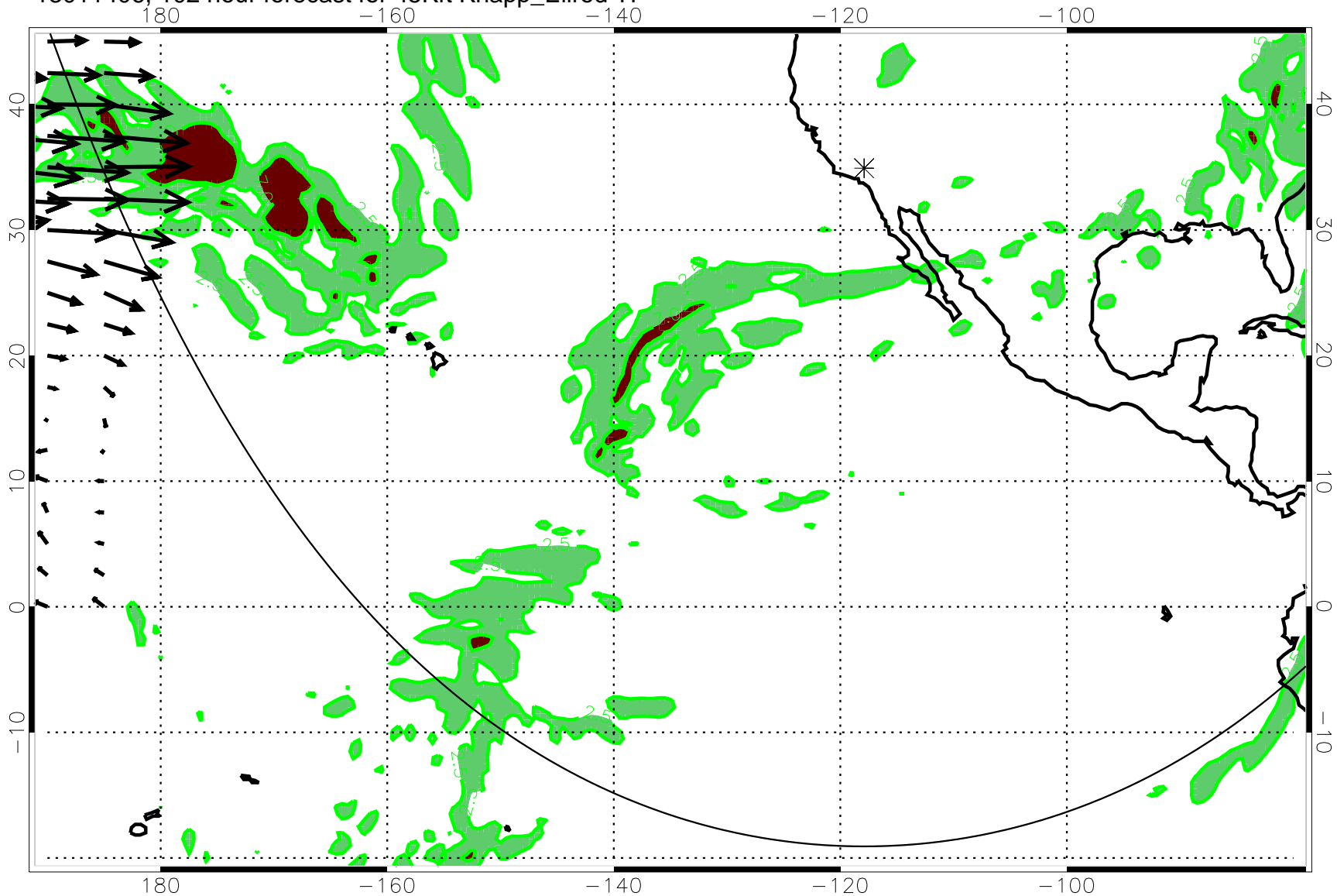
13011406, 102 hour forecast for 45Kft Knapp_Ellrod T1
