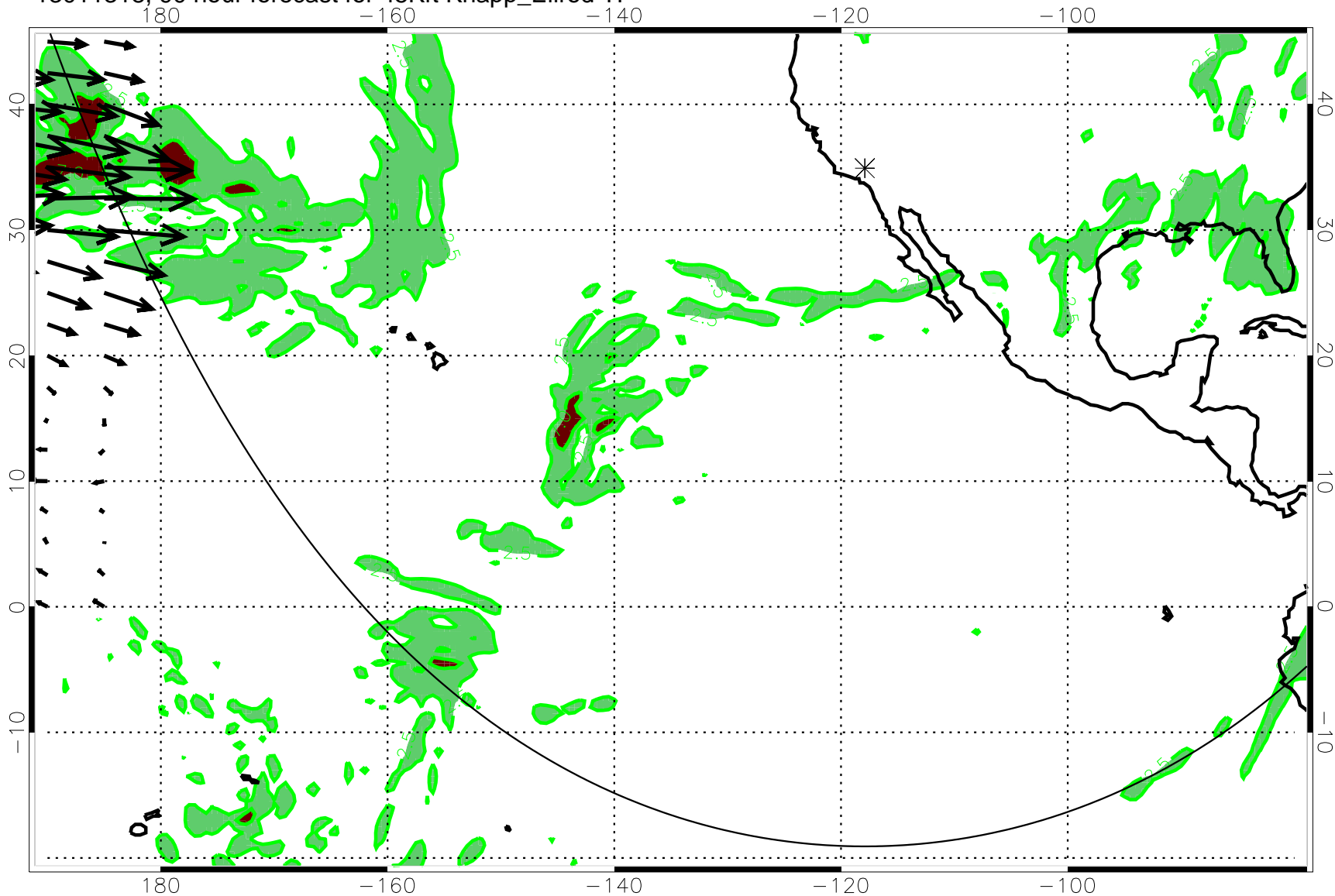
13011318, 90 hour forecast for 45Kft Knapp_Ellrod TI
