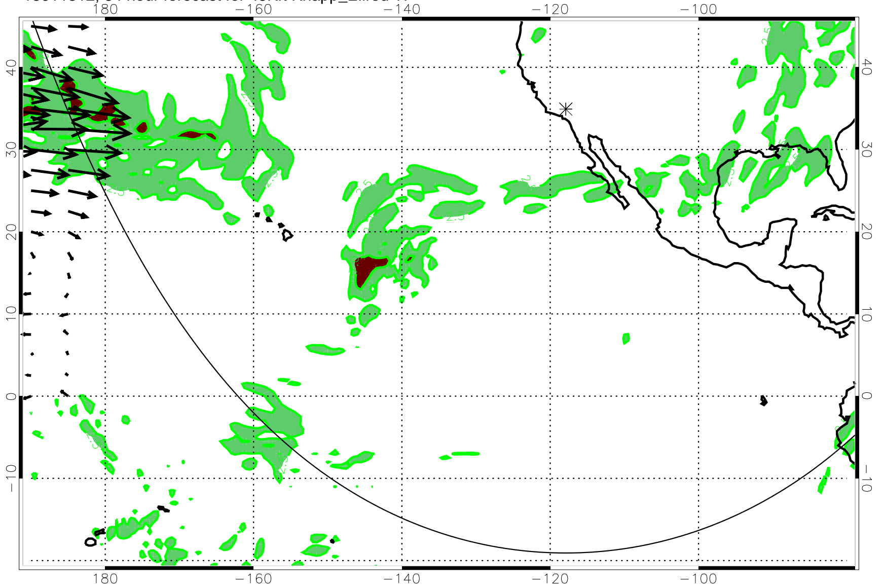
13011312, 84 hour forecast for 45Kft Knapp_Ellrod TI
