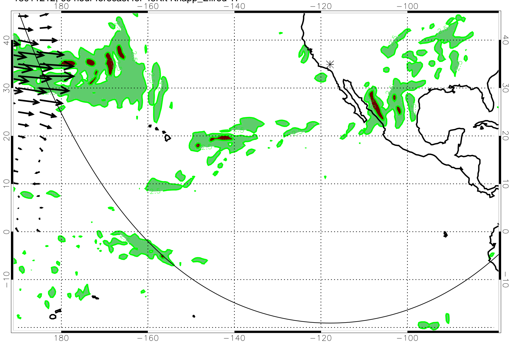
13011212, 60 hour forecast for 45Kft Knapp_Ellrod TI
