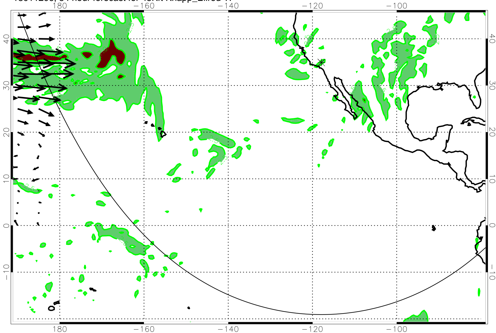
13011206, 54 hour forecast for 45Kft Knapp_Ellrod TI
