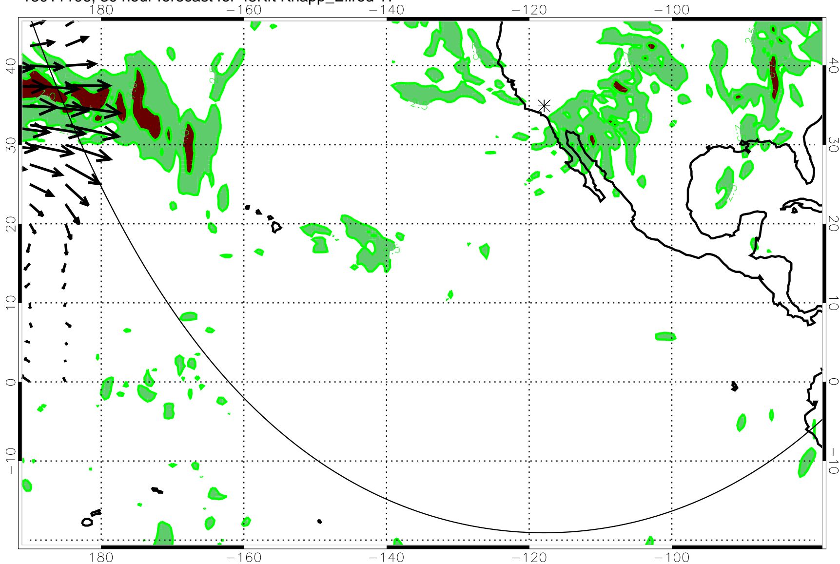
13011106, 30 hour forecast for 45Kft Knapp_Ellrod TI
