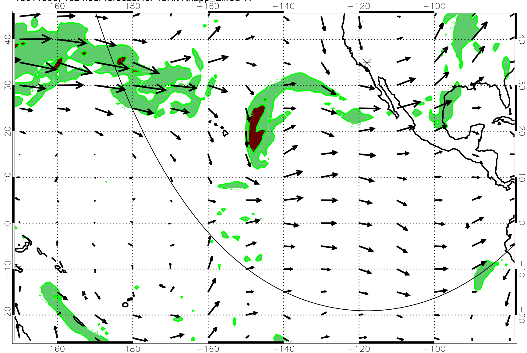
13011306, 102 hour forecast for 45Kft Knapp_Ellrod T1
