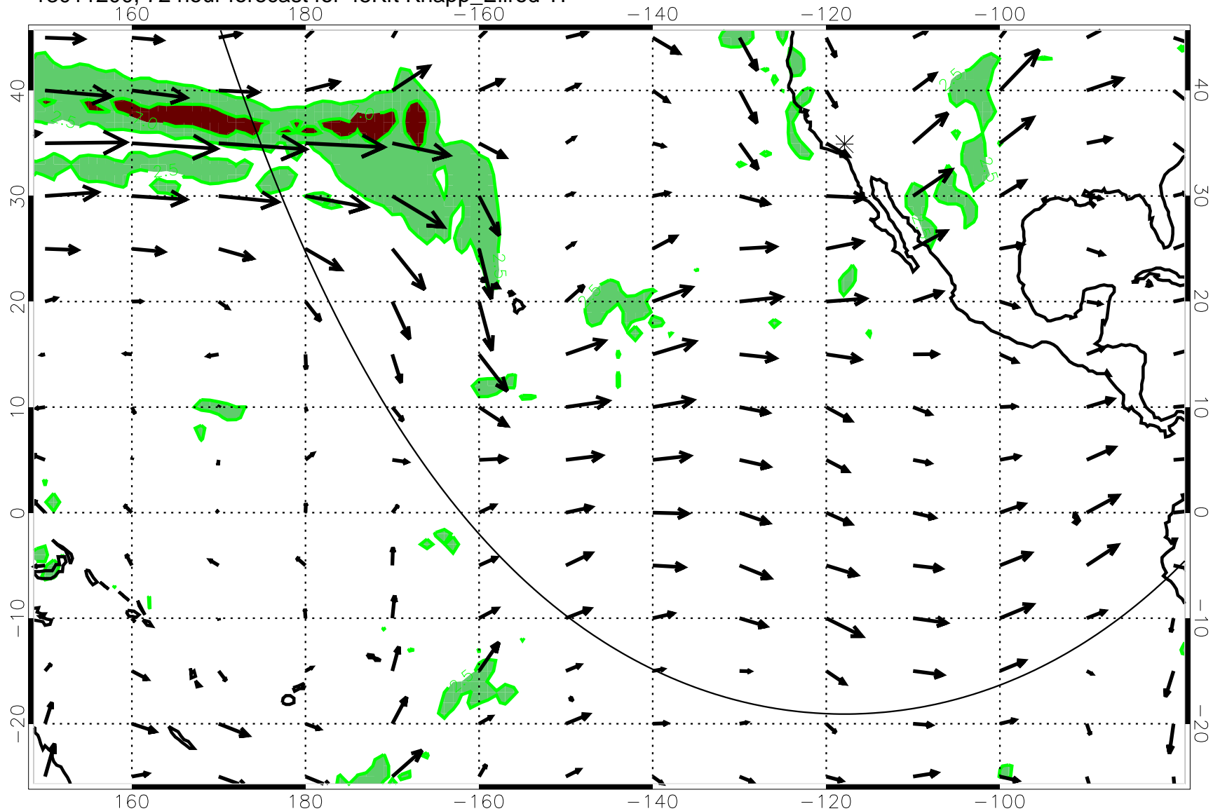
13011200, 72 hour forecast for 45Kft Knapp_Ellrod T1
