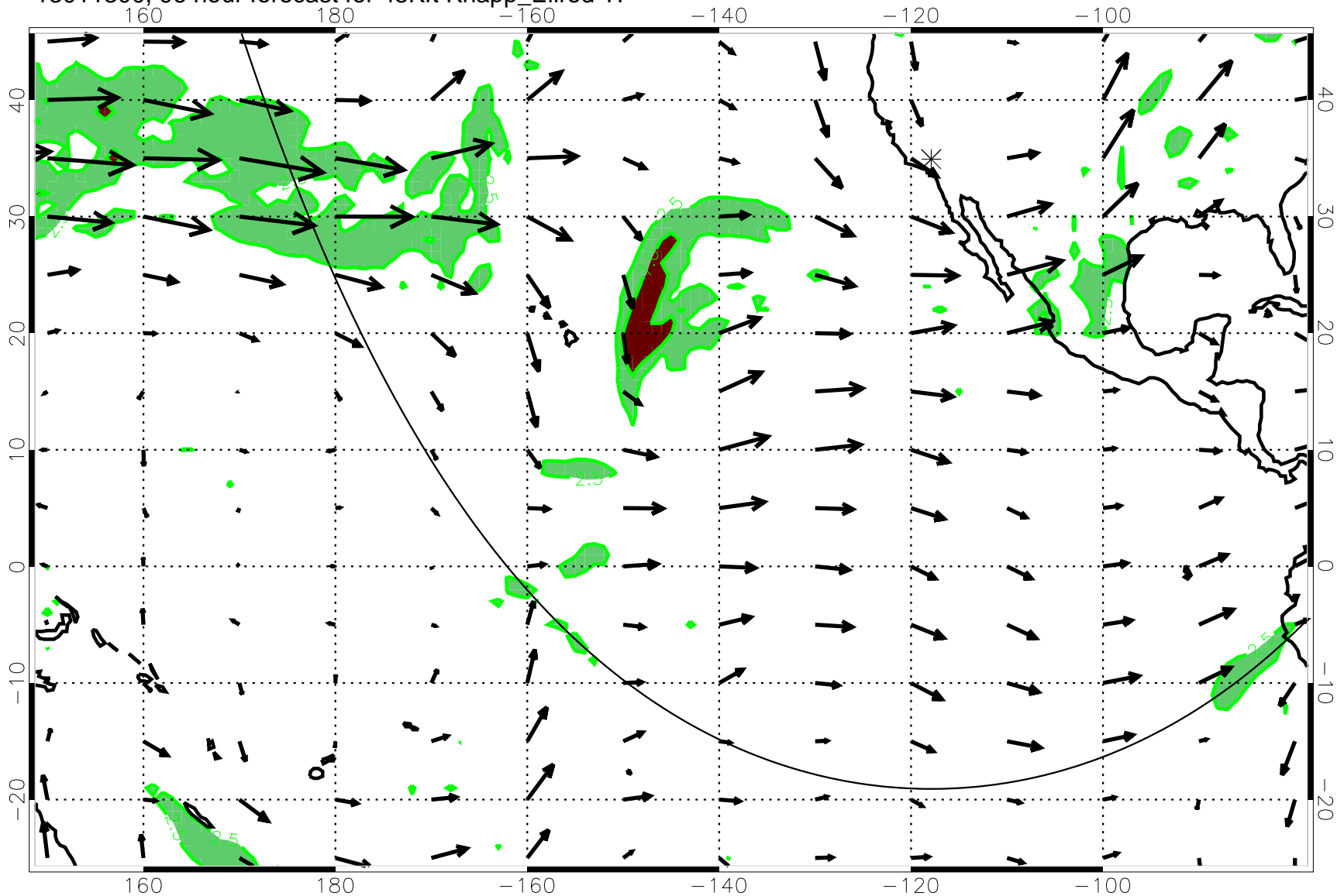
13011300, 96 hour forecast for 45Kft Knapp_Ellrod T1
