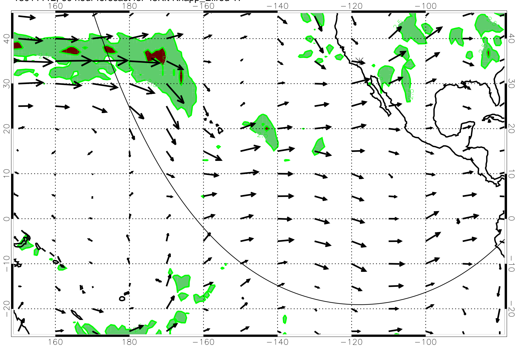
13011112, 60 hour forecast for 45Kft Knapp_Ellrod T1
