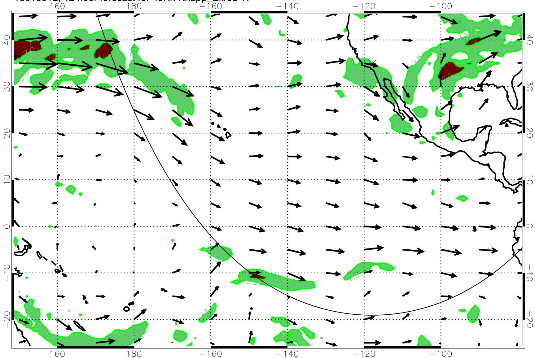
13010912, 12 hour forecast for 45Kft Knapp_Ellrod Tl
