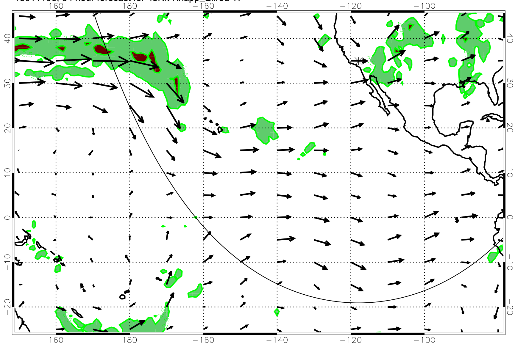
13011106, 54 hour forecast for 45Kft Knapp_Ellrod T1
