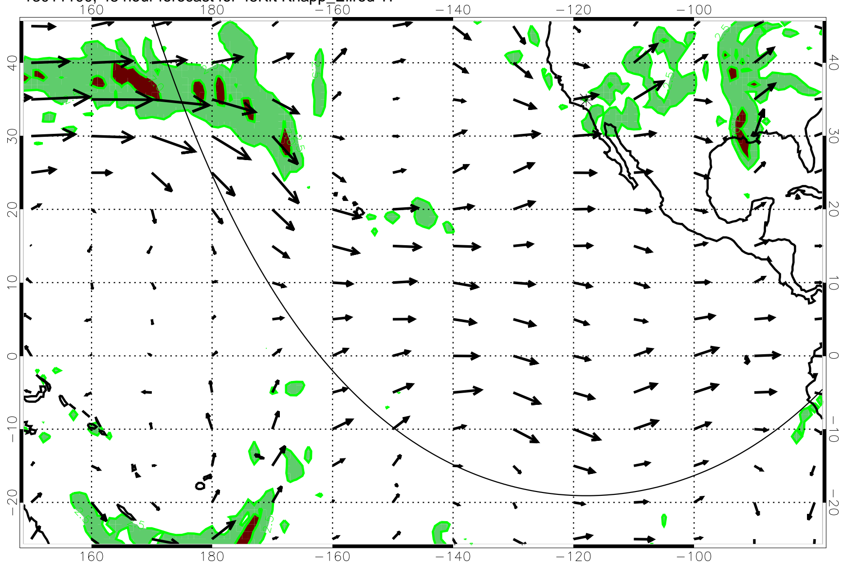
13011100, 48 hour forecast for 45Kft Knapp_Ellrod T1
