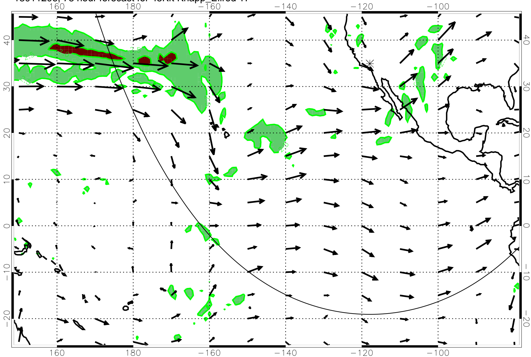
13011206, 78 hour forecast for 45Kft Knapp_Ellrod T1
