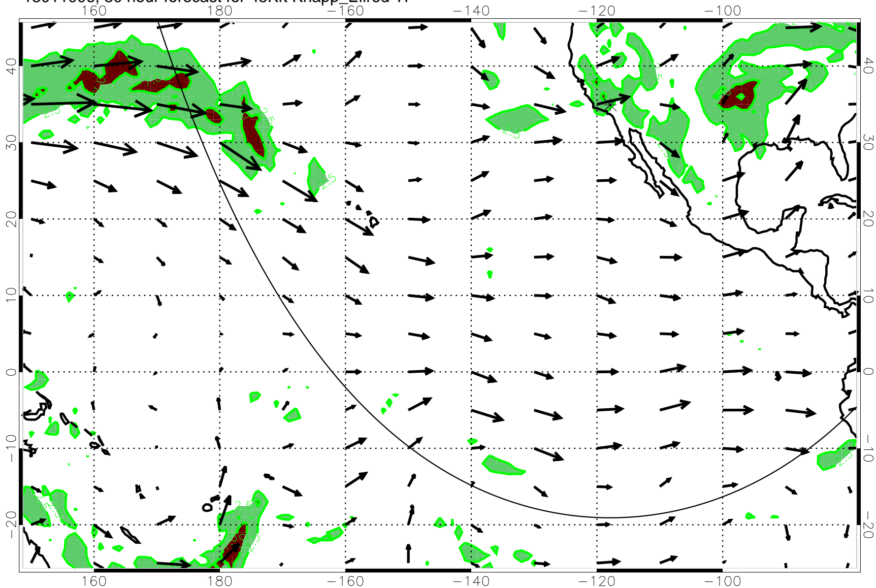
13011006, 30 hour forecast for 45Kft Knapp_Ellrod T1
