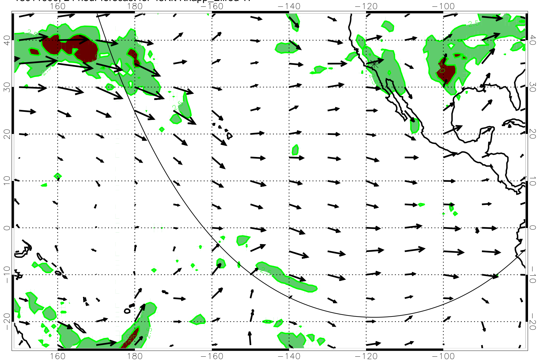
13011000, 24 hour forecast for 45Kft Knapp_Ellrod T1
