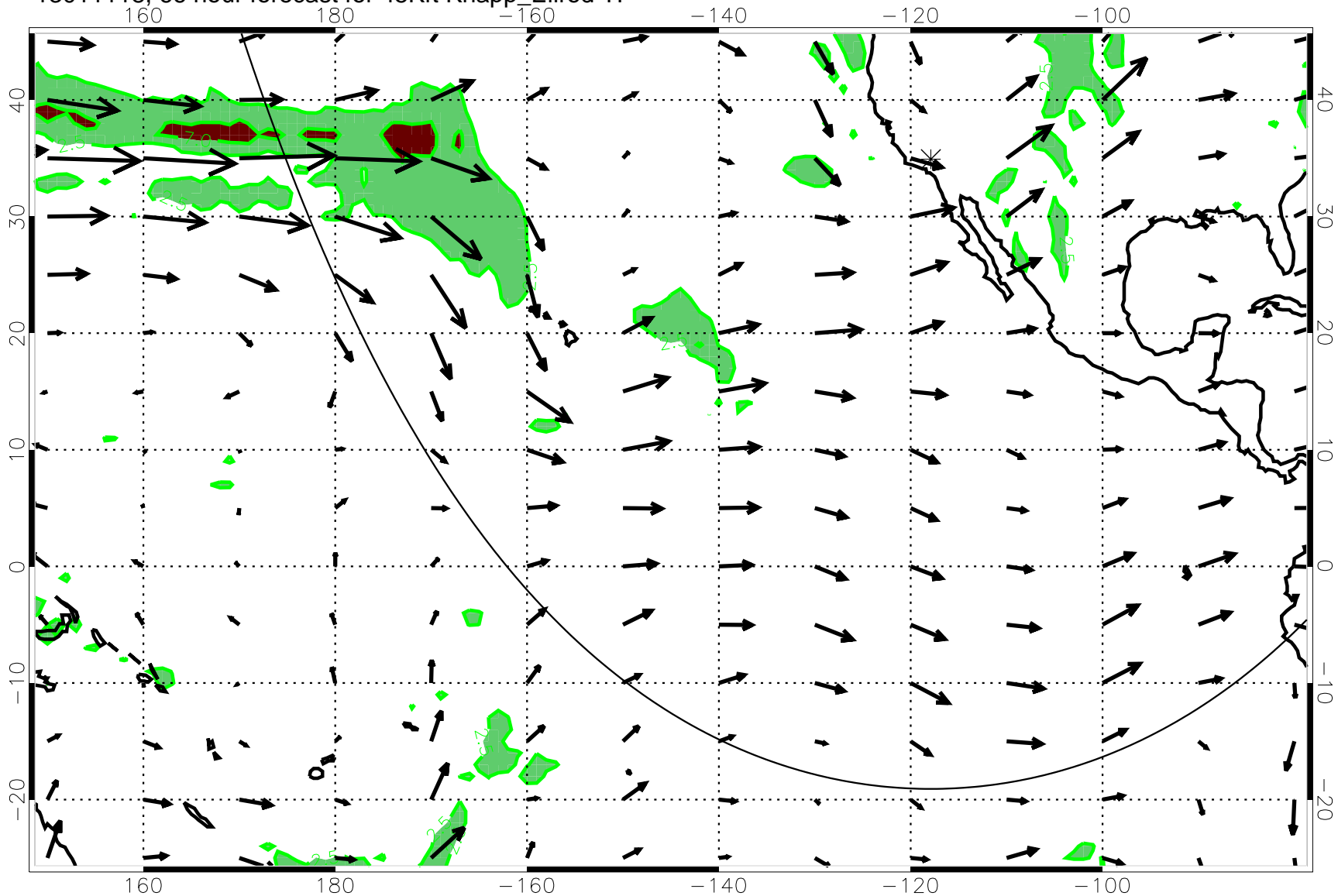
13011118, 66 hour forecast for 45Kft Knapp_Ellrod T1
