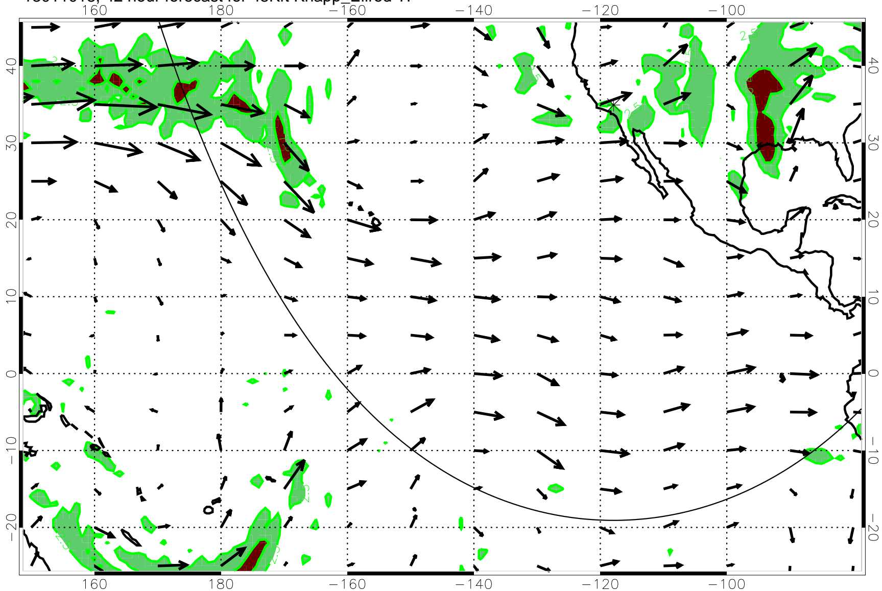
13011018, 42 hour forecast for 45Kft Knapp_Ellrod T1
