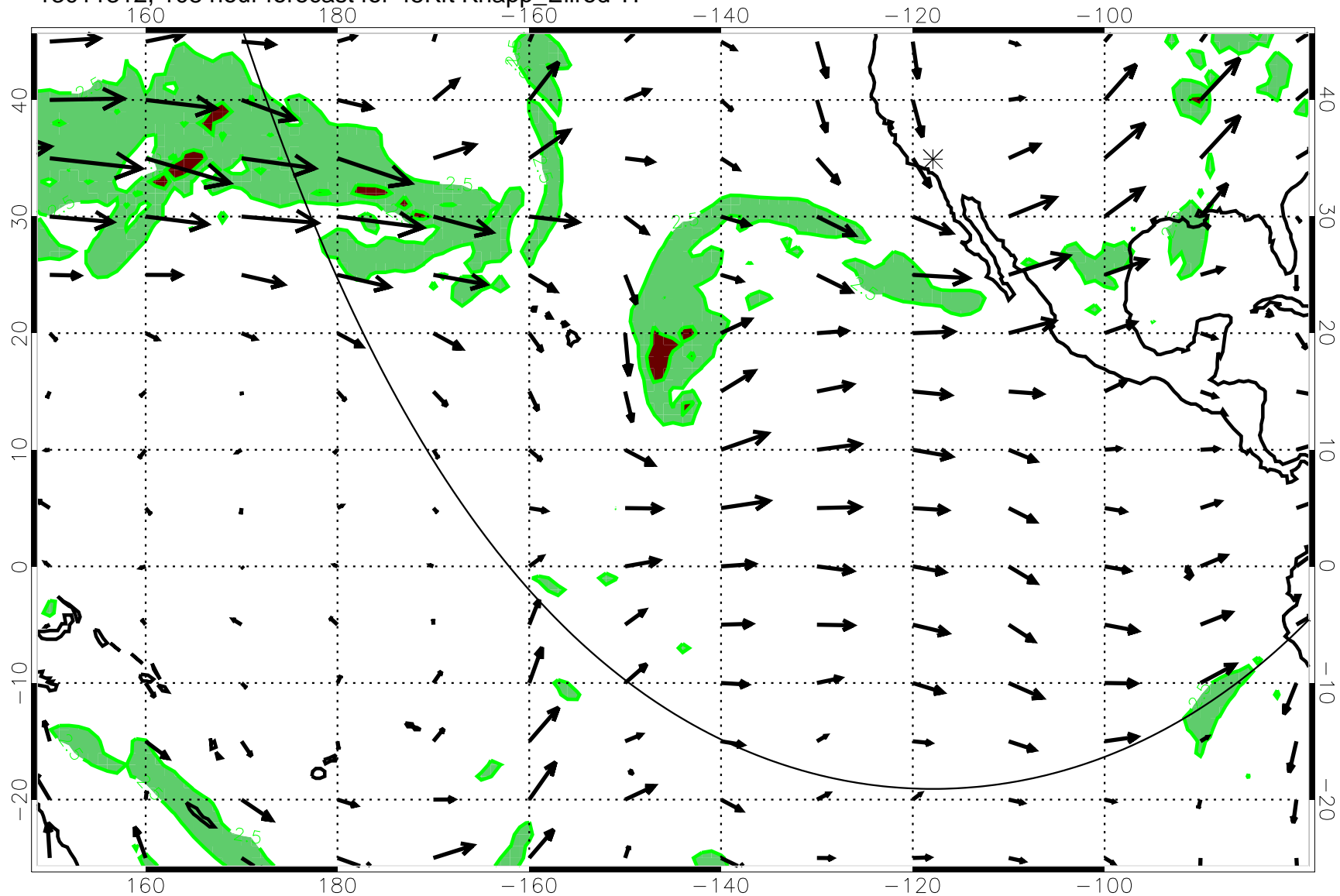
13011312, 108 hour forecast for 45Kft Knapp_Ellrod T1
