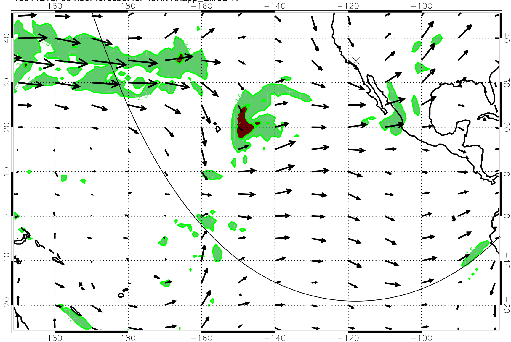
13011218, 90 hour forecast for 45Kft Knapp_Ellrod T1
