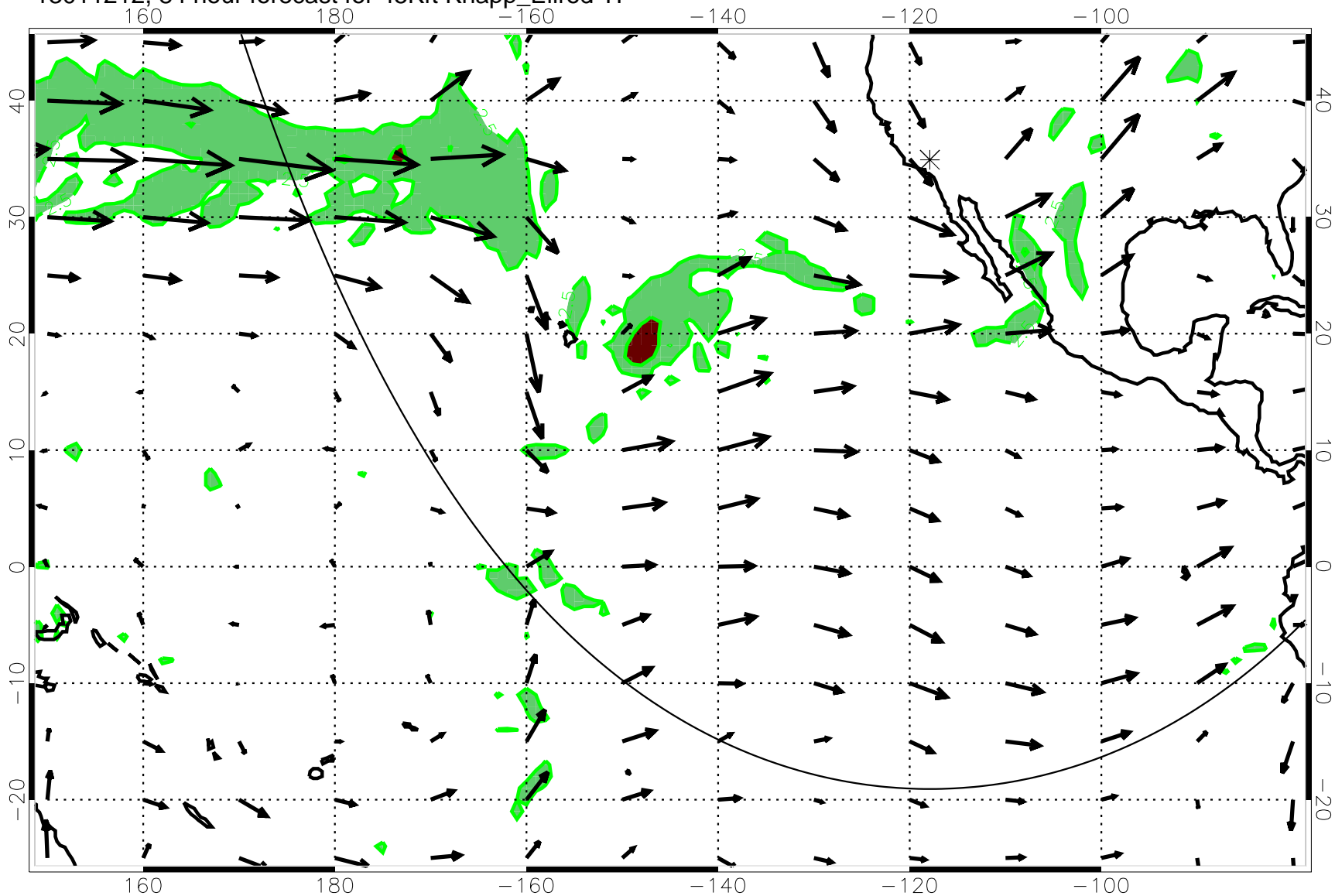
13011212, 84 hour forecast for 45Kft Knapp_Ellrod T1
