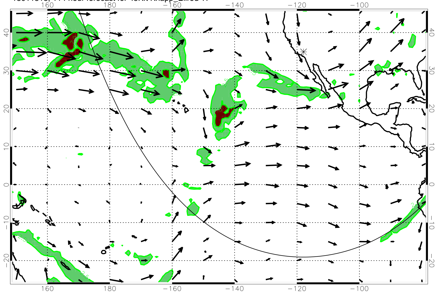
13011318, 114 hour forecast for 45Kft Knapp_Ellrod T1
