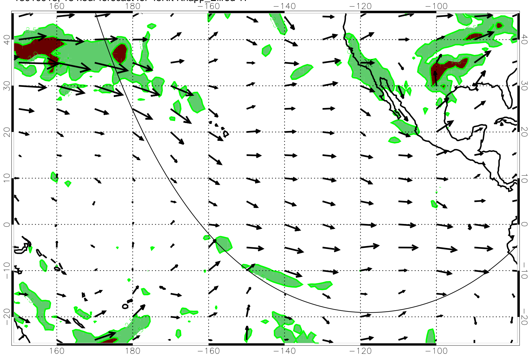
13010918, 18 hour forecast for 45Kft Knapp_Ellrod T1
