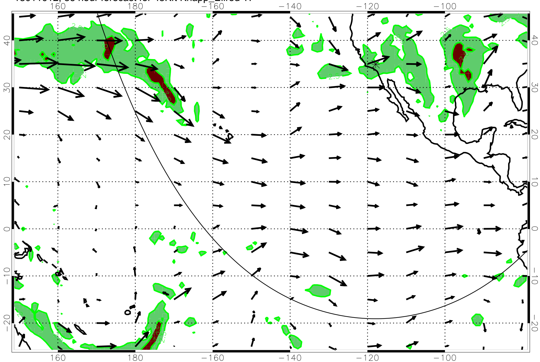
13011012, 36 hour forecast for 45Kft Knapp_Ellrod T1
