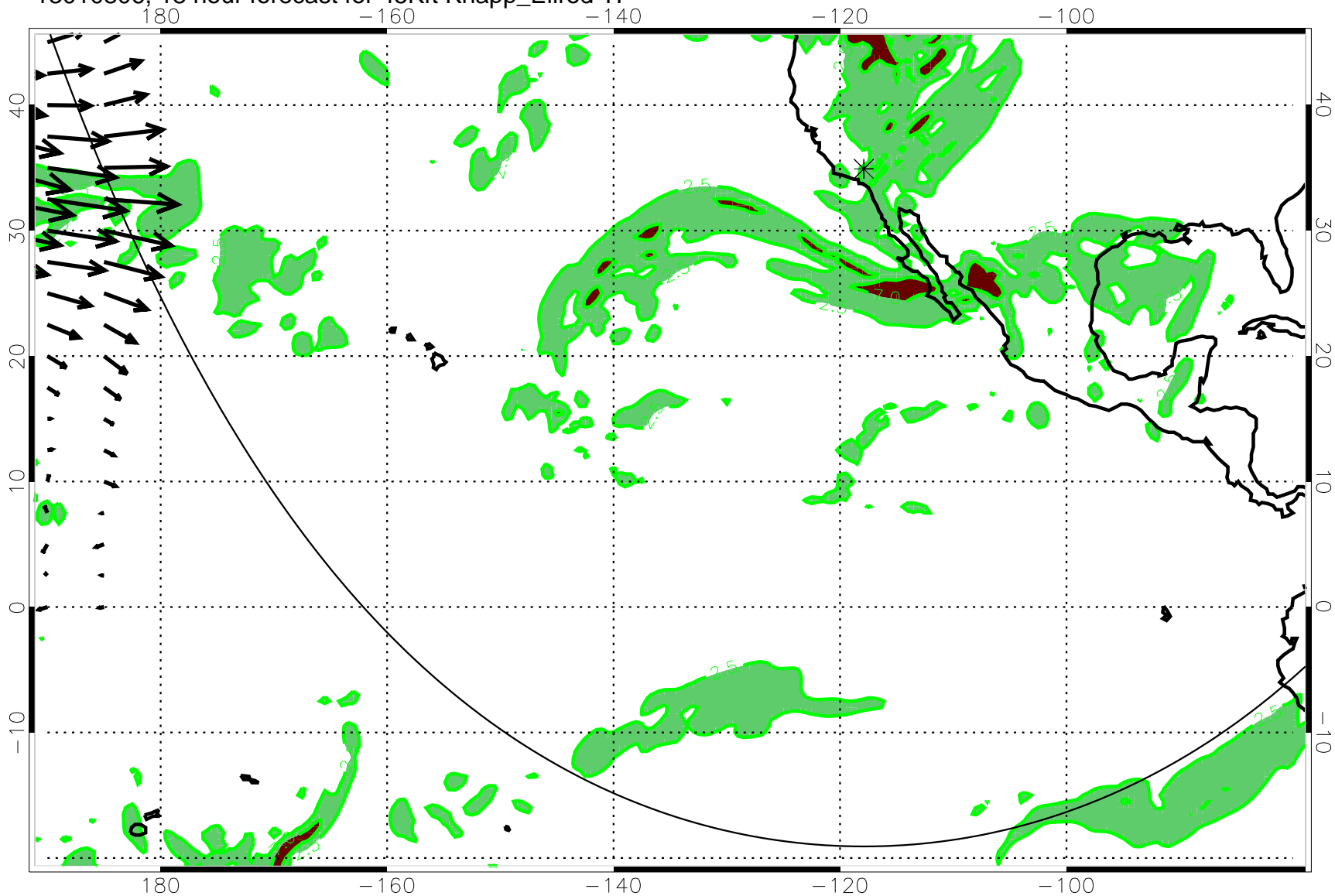
13010806, 18 hour forecast for 45Kft Knapp_Ellrod TI
