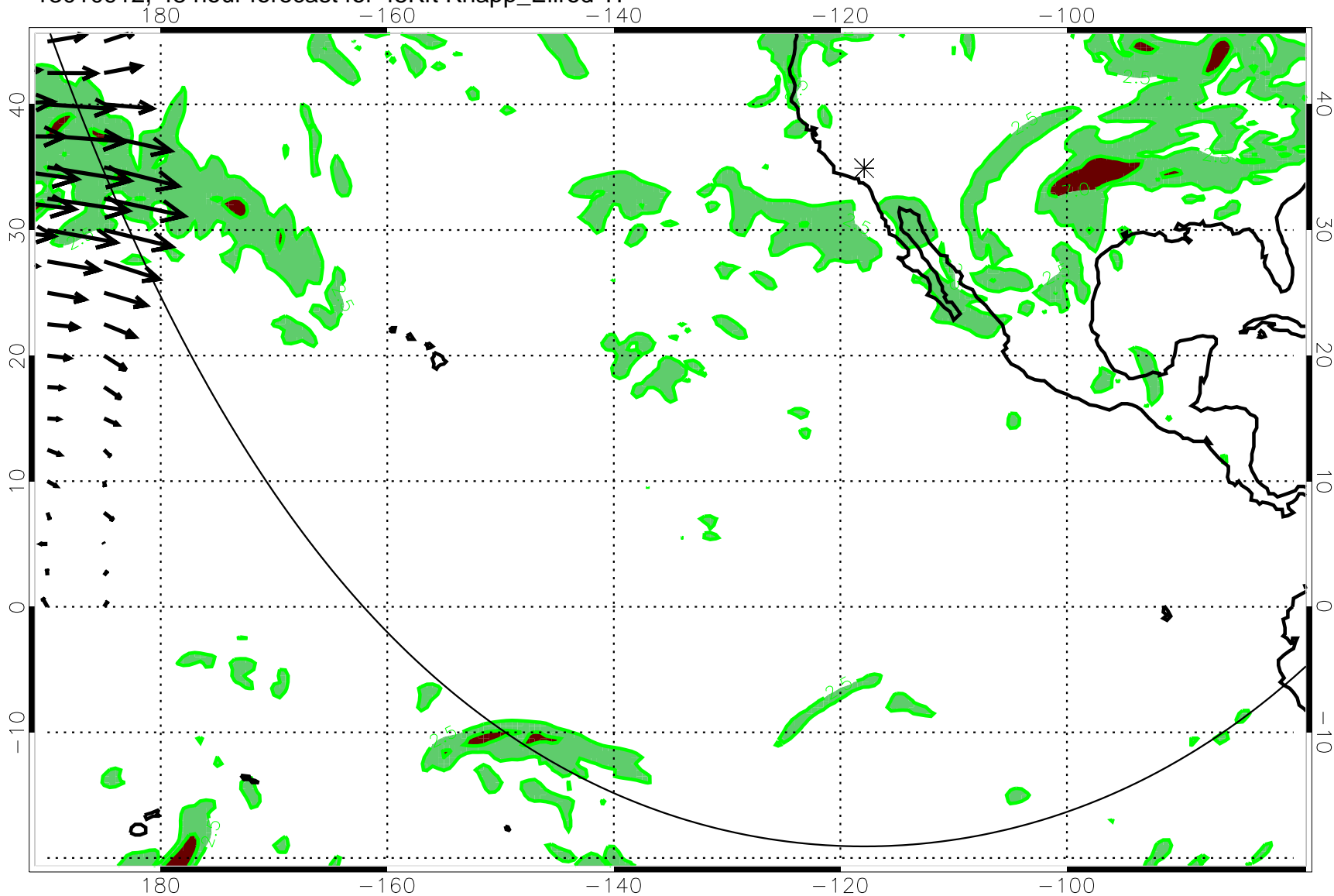
13010912, 48 hour forecast for 45Kft Knapp_Ellrod TI
