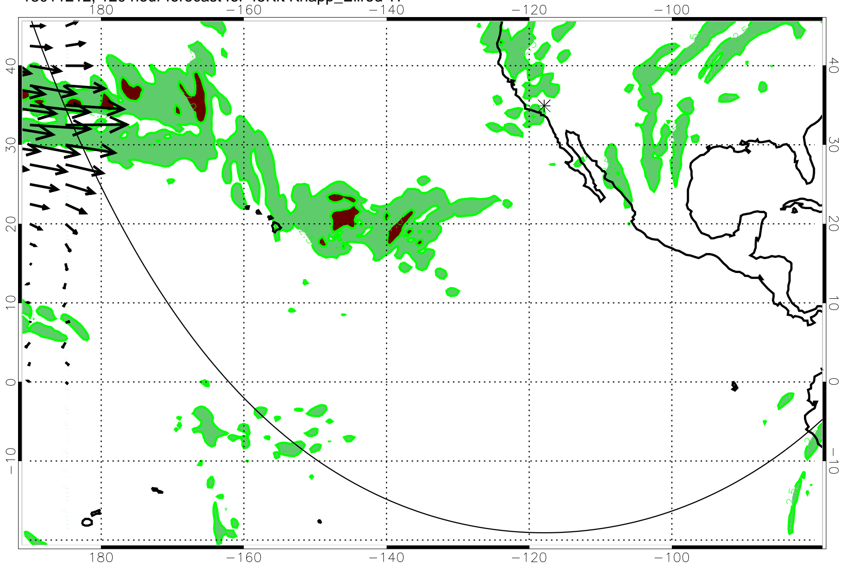
13011212, 120 hour forecast for 45Kft Knapp_Ellrod TI
