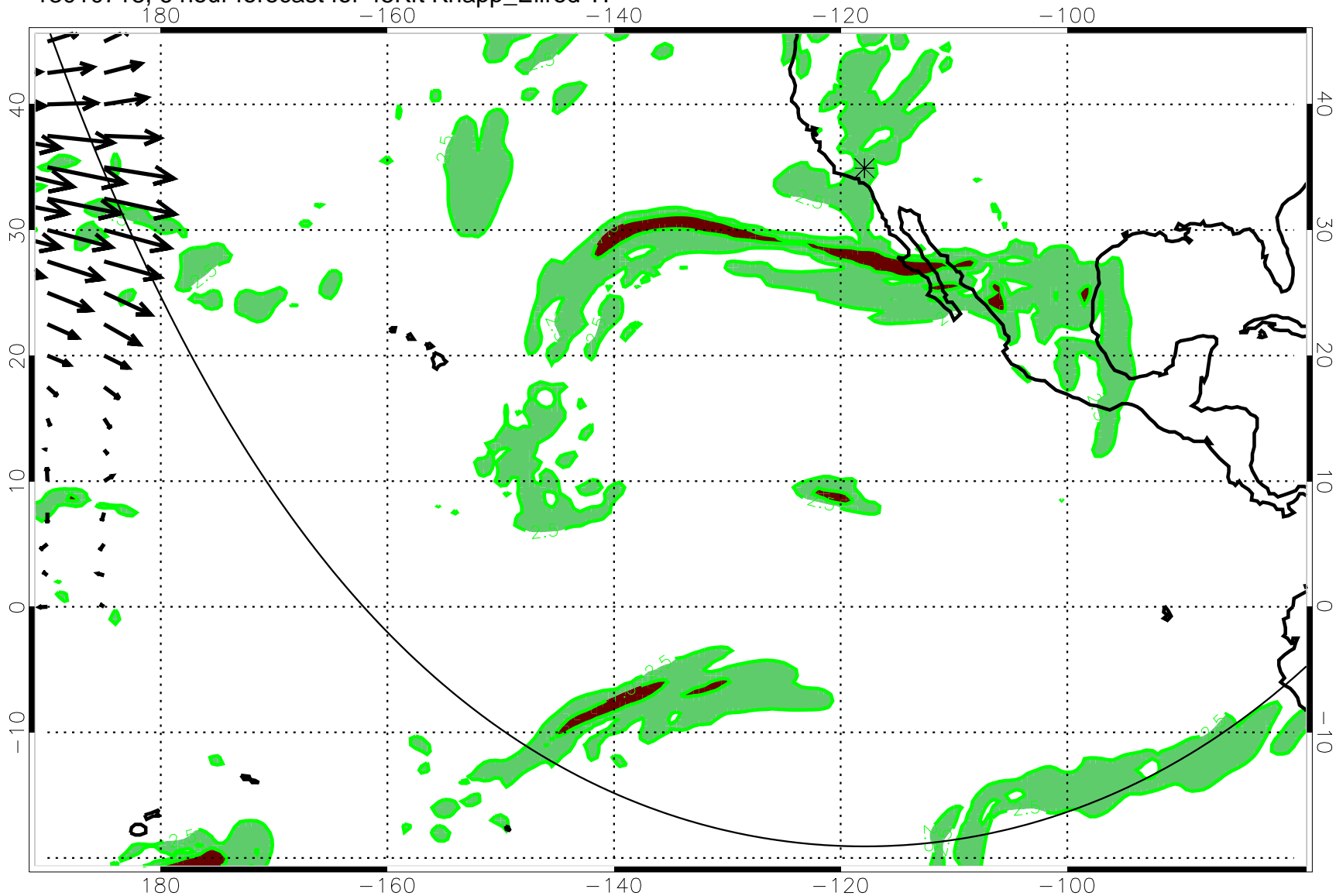
13010718, 6 hour forecast for 45Kft Knapp_Ellrod TI
