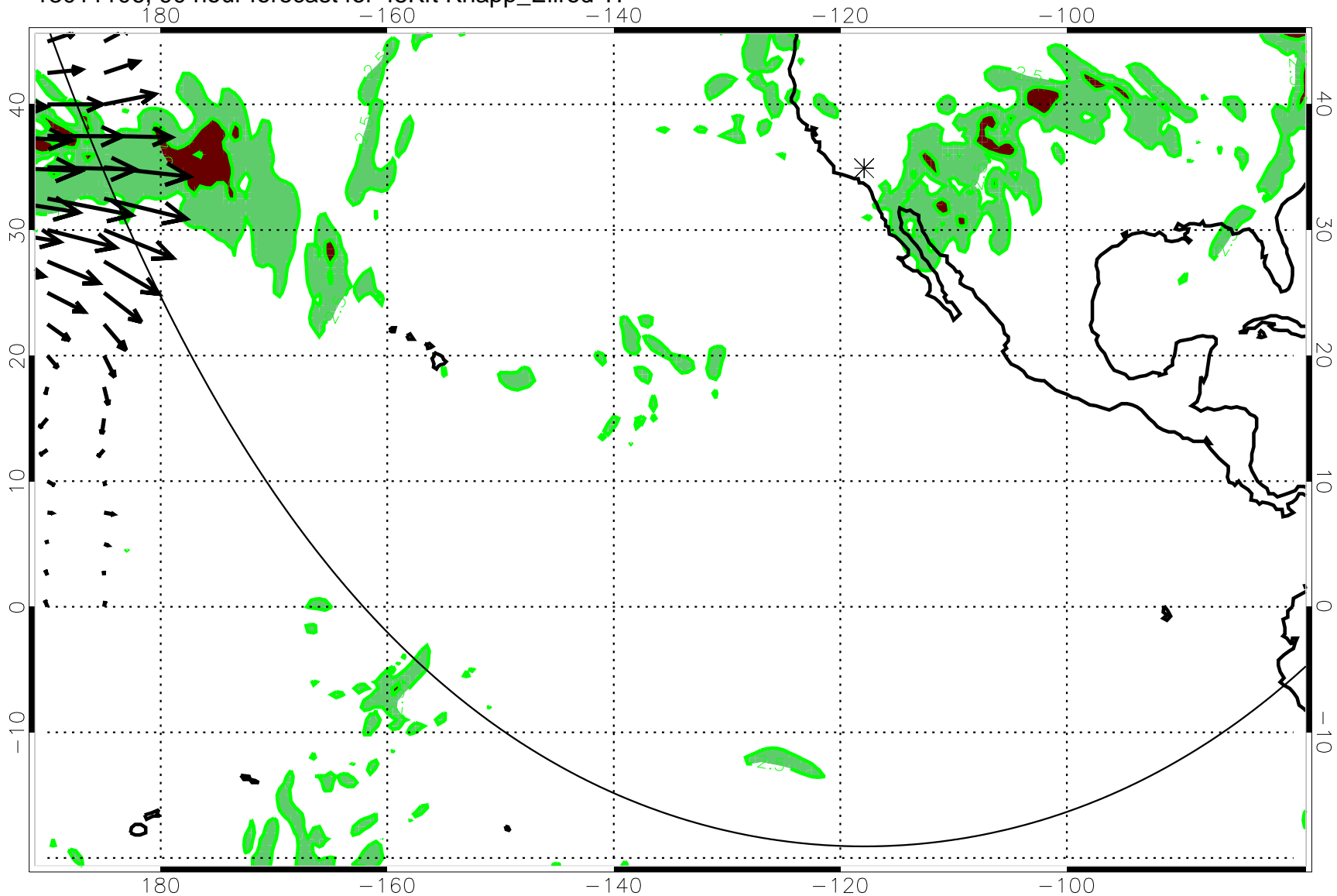
13011106, 90 hour forecast for 45Kft Knapp_Ellrod TI
