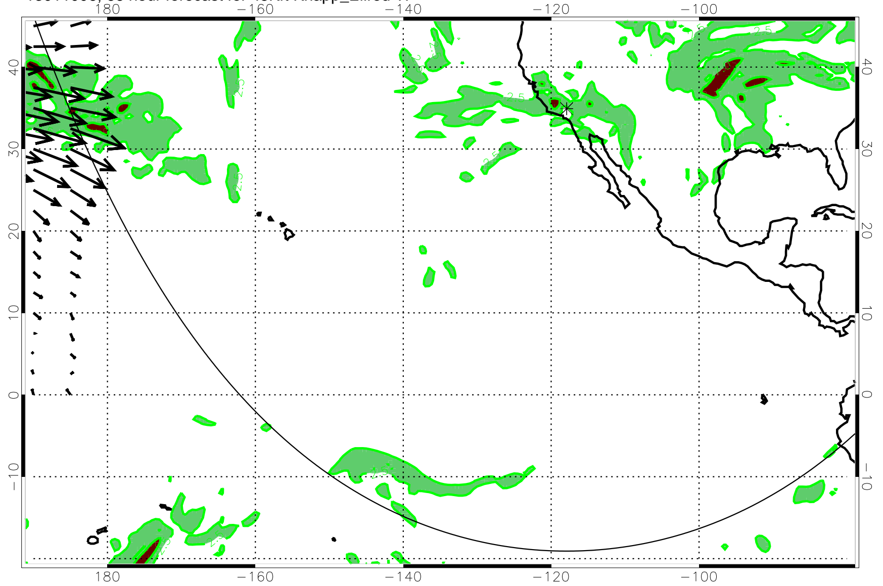
13011006, 66 hour forecast for 45Kft Knapp_Ellrod TI
