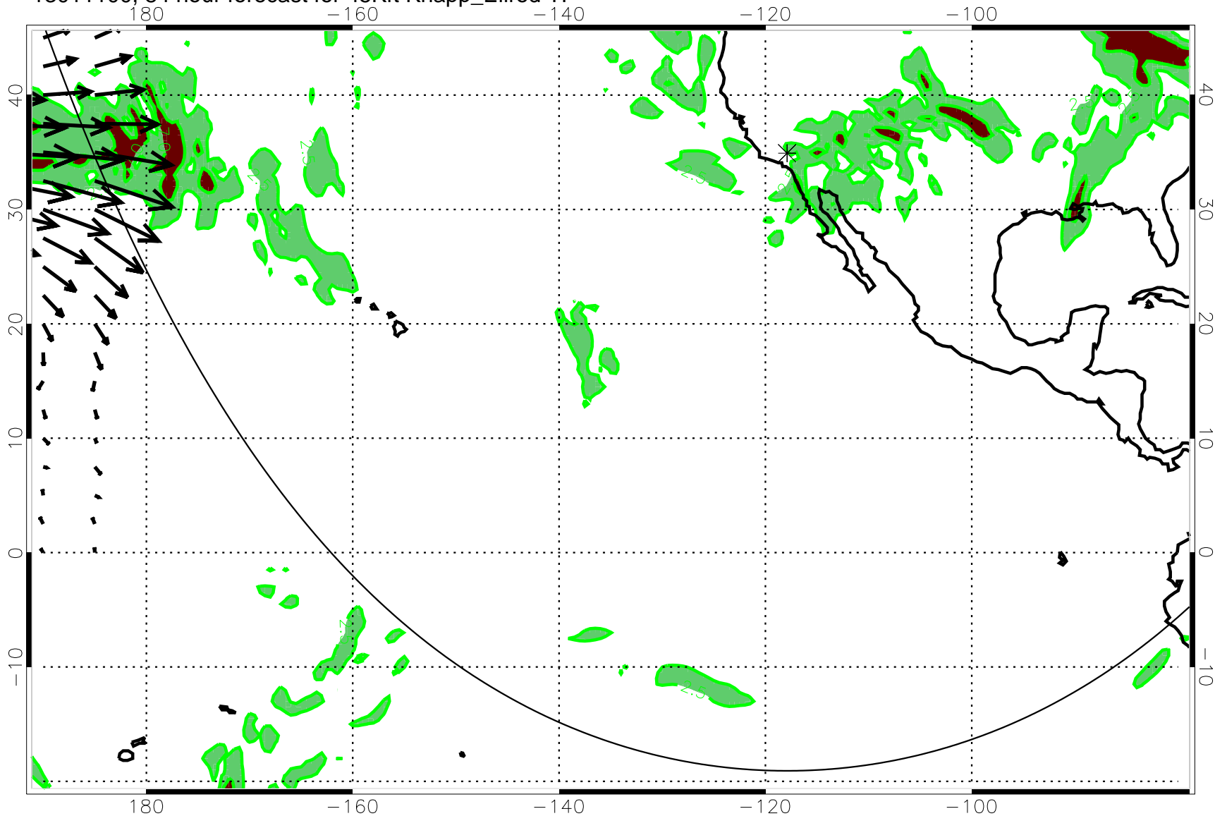
13011100, 84 hour forecast for 45Kft Knapp_Ellrod TI
