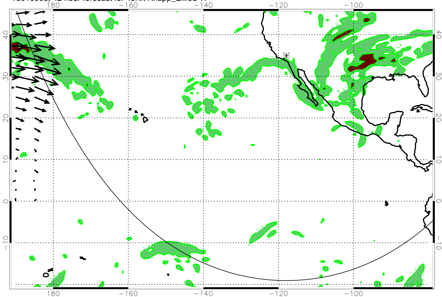
13010906, 42 hour forecast for 45Kft Knapp_Ellrod TI
