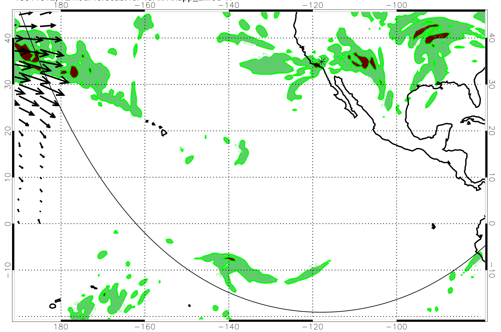
13011012, 72 hour forecast for 45Kft Knapp_Ellrod TI
