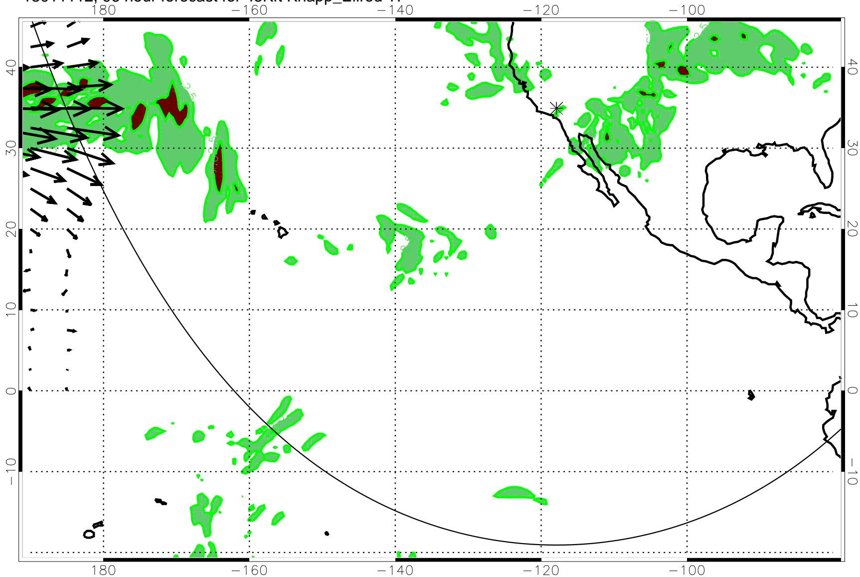
13011112, 96 hour forecast for 45Kft Knapp_Ellrod TI
