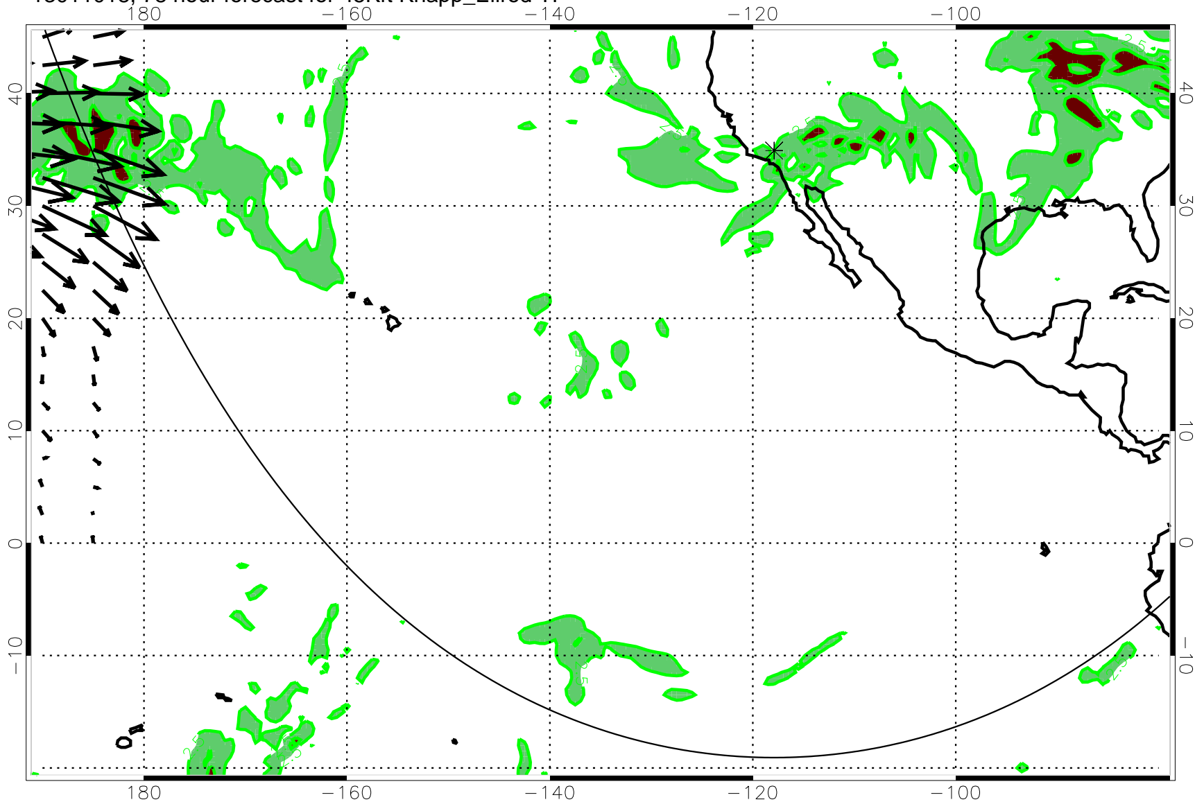
13011018, 78 hour forecast for 45Kft Knapp_Ellrod TI
