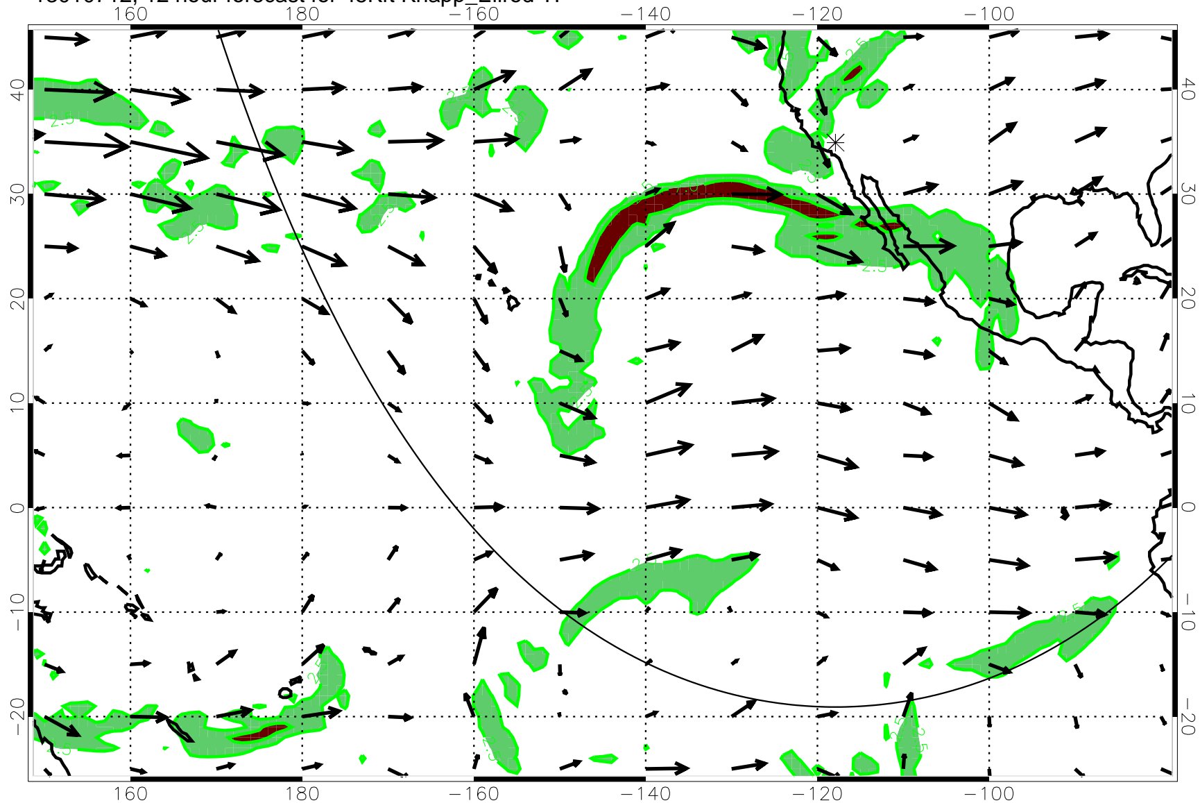
13010712, 12 hour forecast for 45Kft Knapp_Ellrod T1
