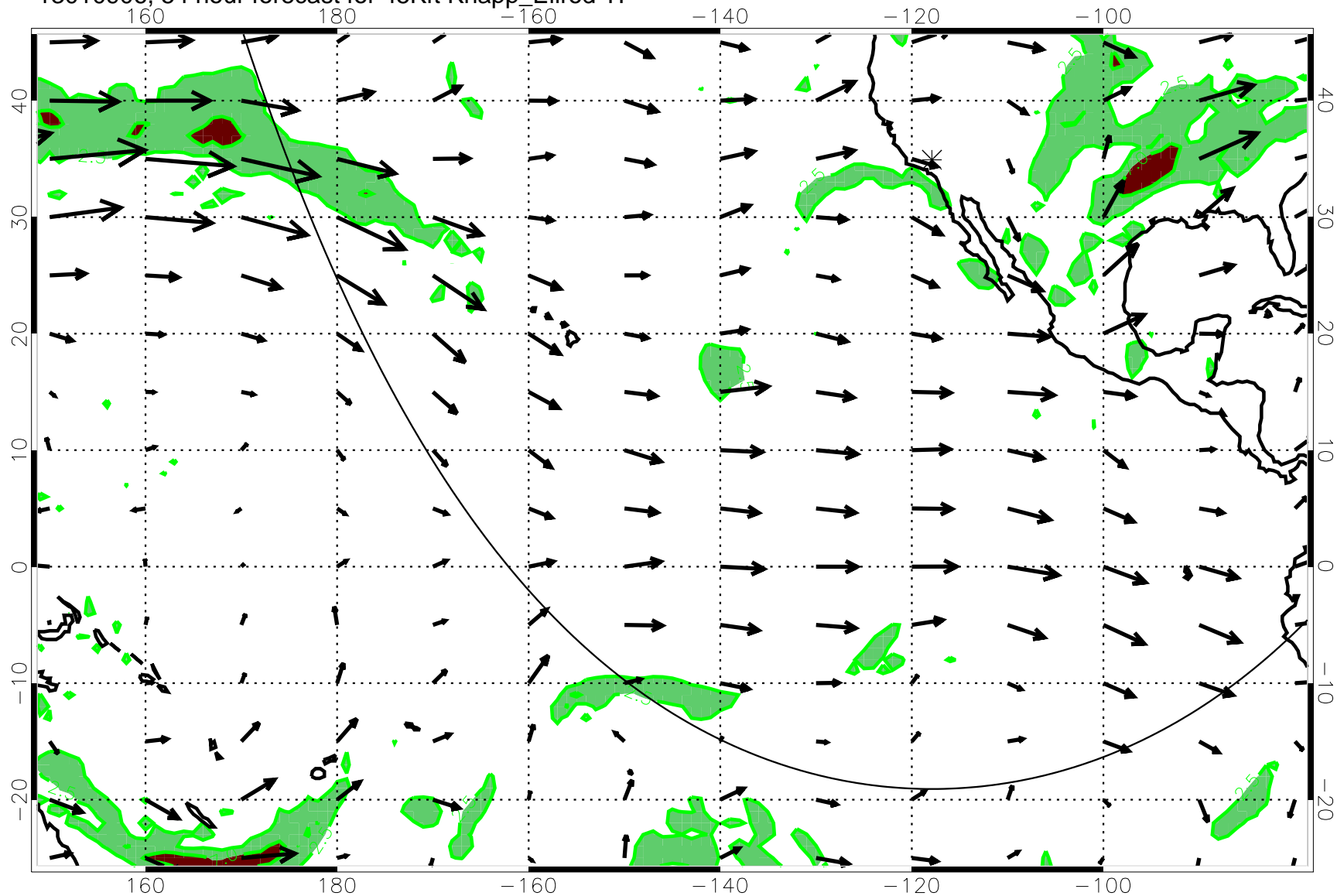
13010906, 54 hour forecast for 45Kft Knapp_Ellrod T1
