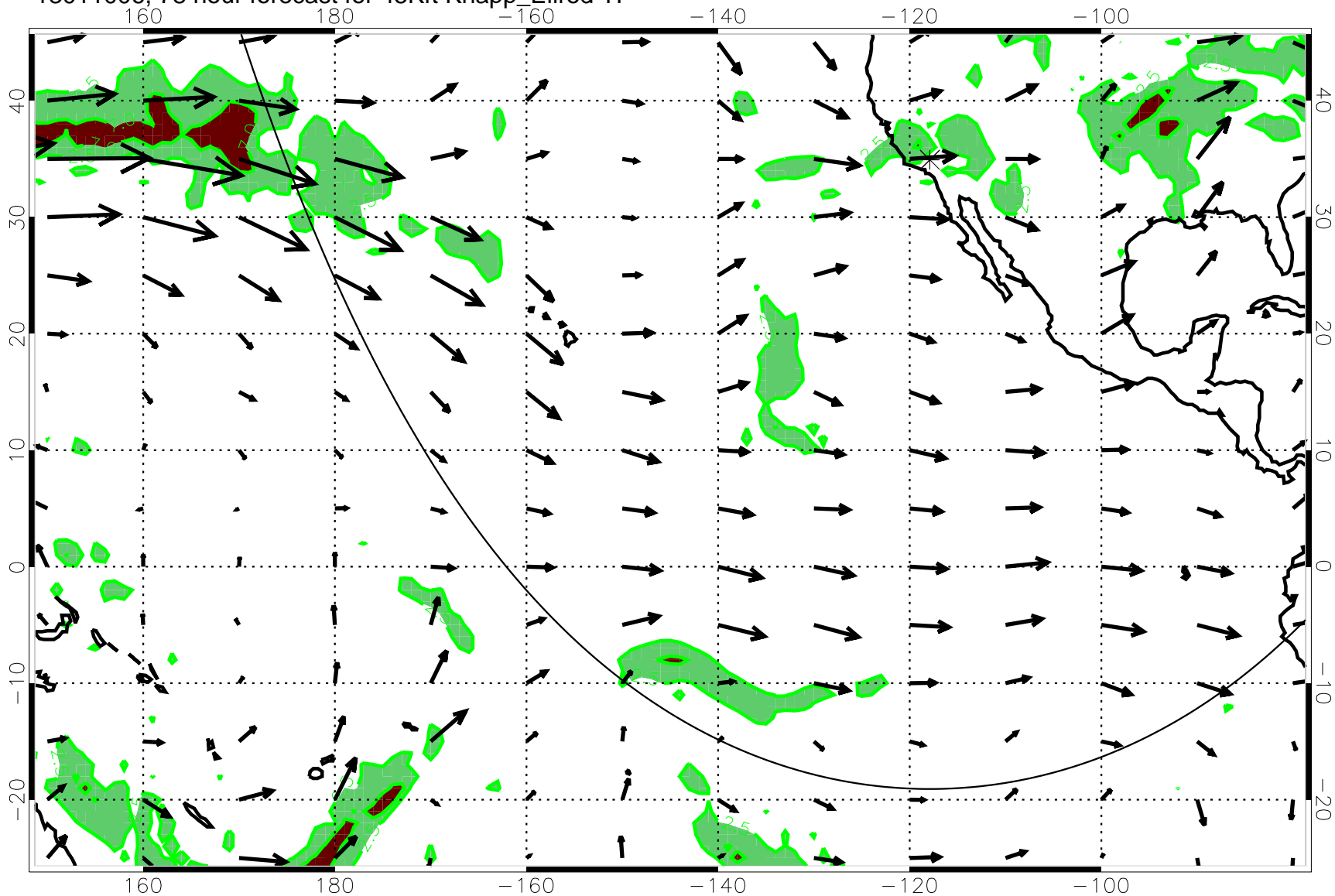
13011006, 78 hour forecast for 45Kft Knapp_Ellrod T1
