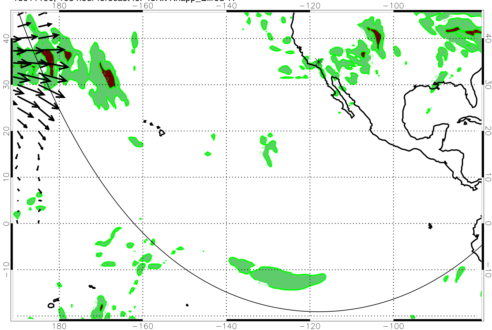
13011100, 108 hour forecast for 45Kft Knapp_Ellrod TI
