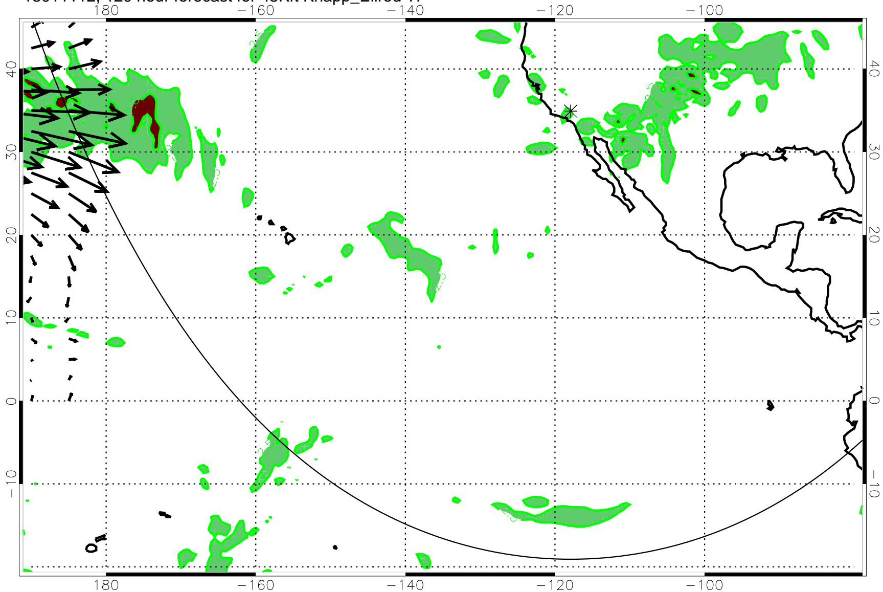
13011112, 120 hour forecast for 45Kft Knapp_Ellrod TI
