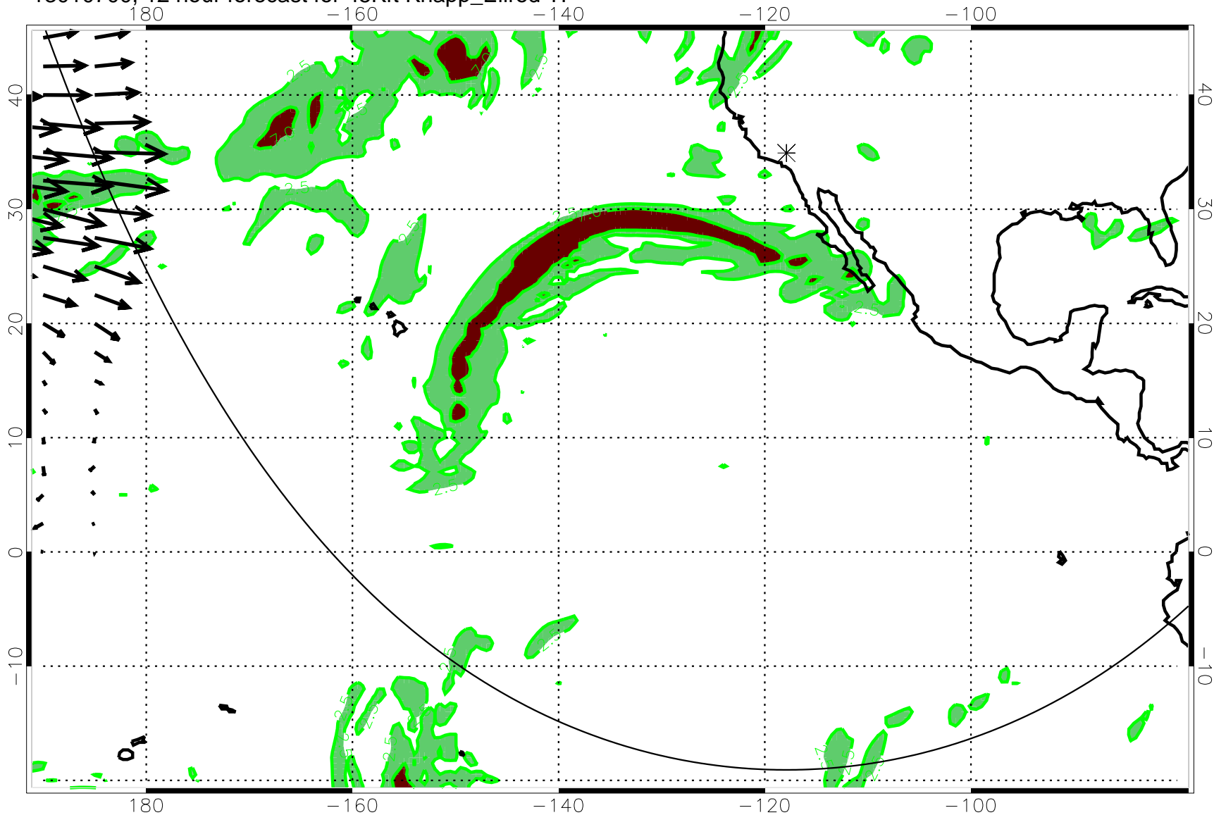
13010700, 12 hour forecast for 45Kft Knapp_Ellrod TI
