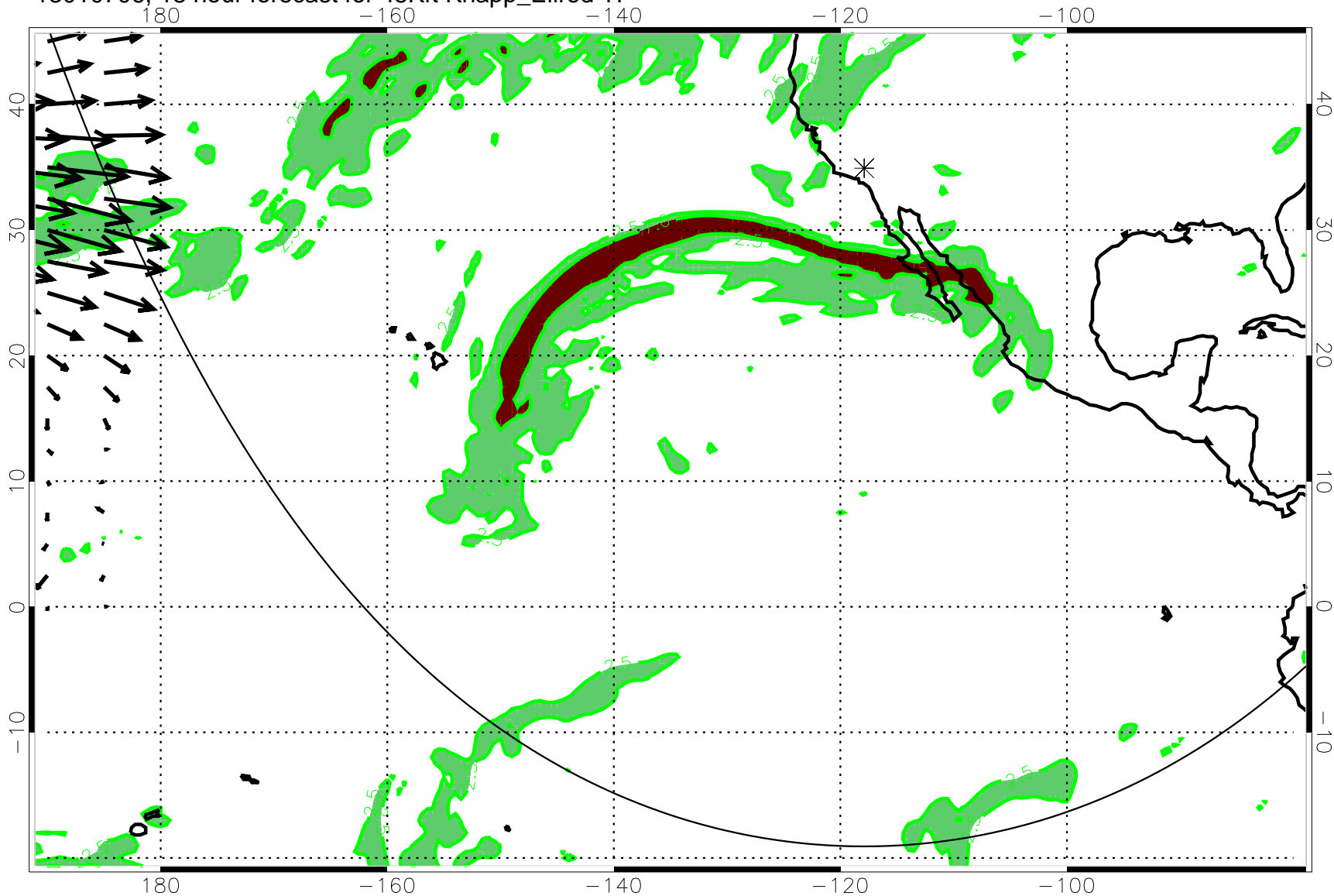
13010706, 18 hour forecast for 45Kft Knapp_Ellrod TI
