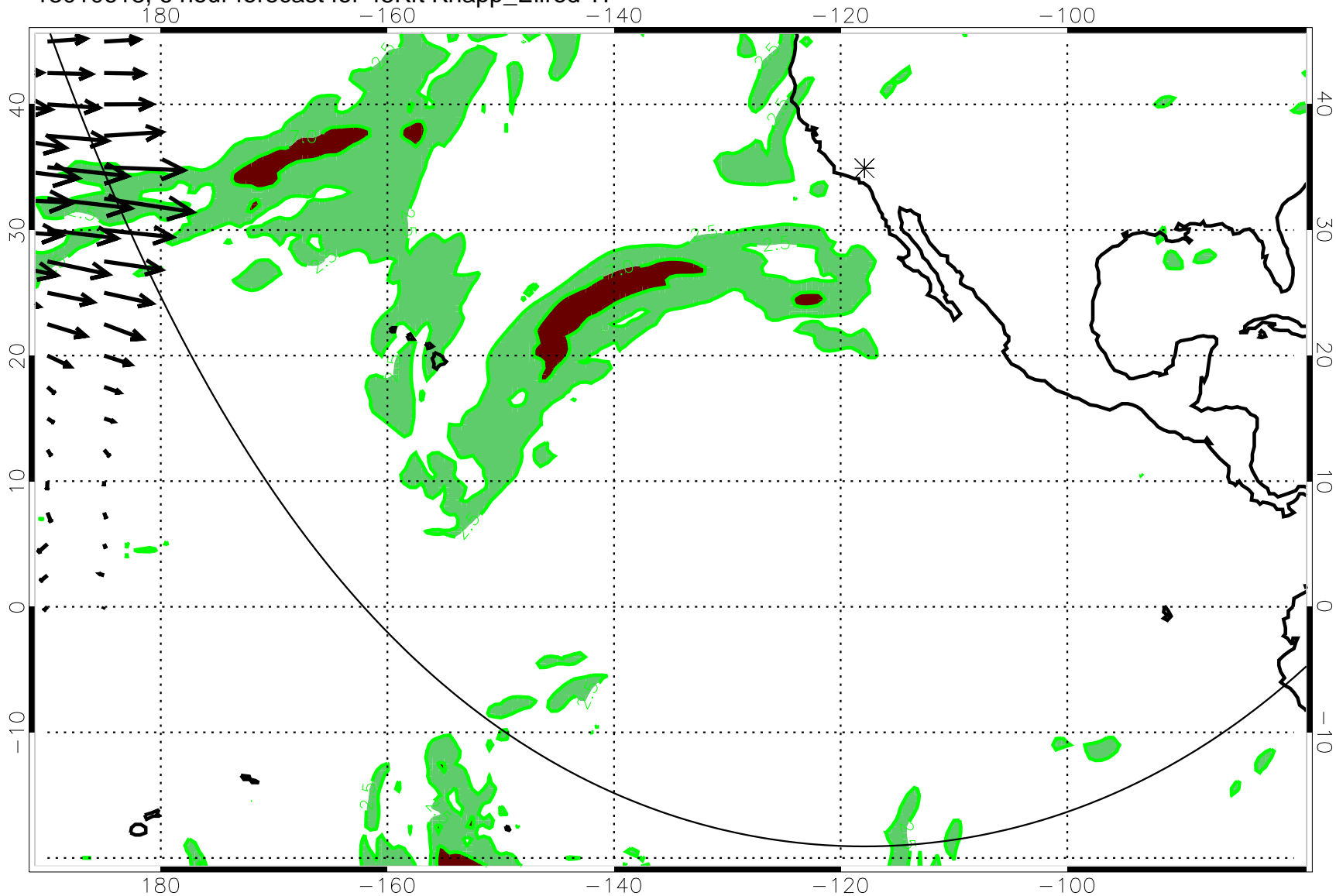
13010618, 6 hour forecast for 45Kft Knapp_Ellrod TI
