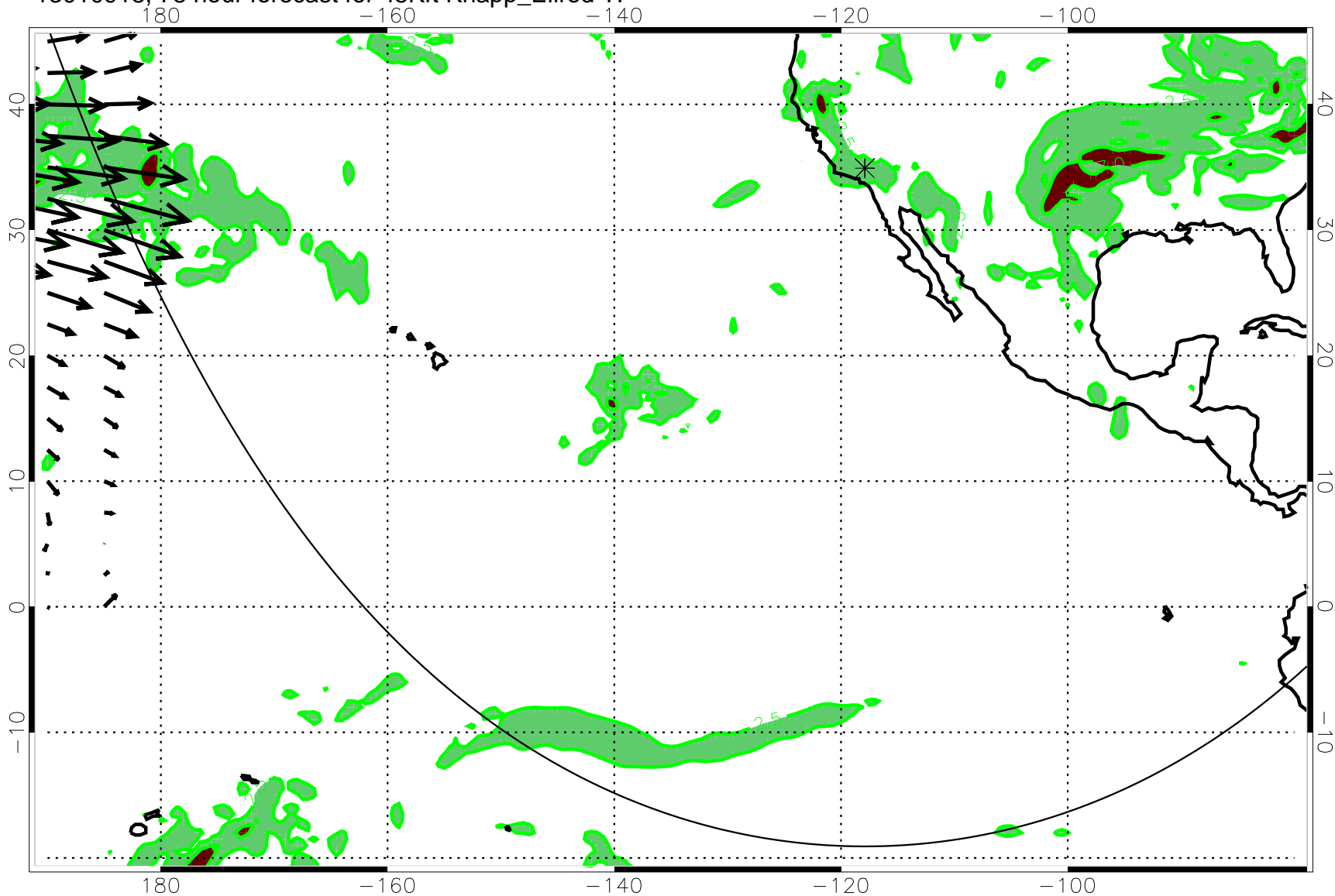
13010918, 78 hour forecast for 45Kft Knapp_Ellrod TI
