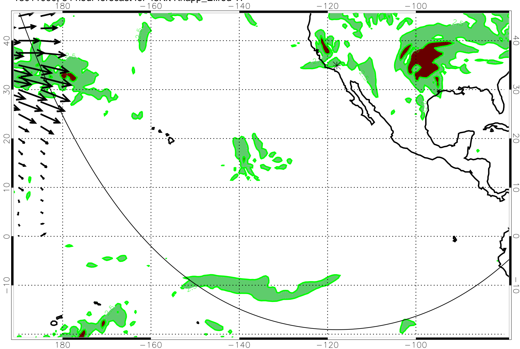
13011000, 84 hour forecast for 45Kft Knapp_Ellrod TI
