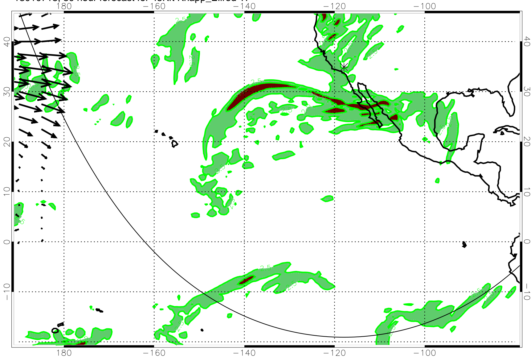
13010718, 30 hour forecast for 45Kft Knapp_Ellrod TI
