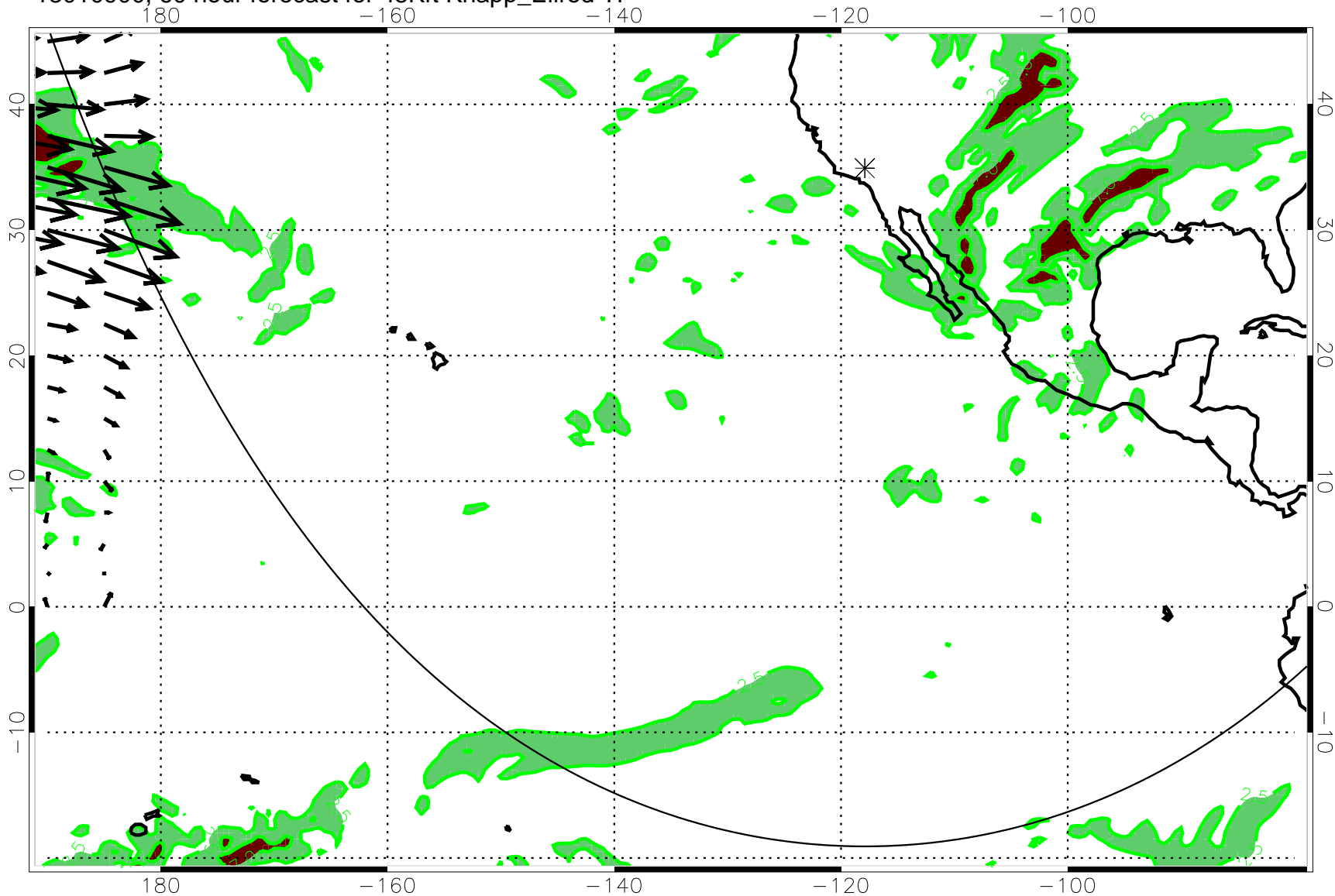
13010900, 60 hour forecast for 45Kft Knapp_Ellrod TI
