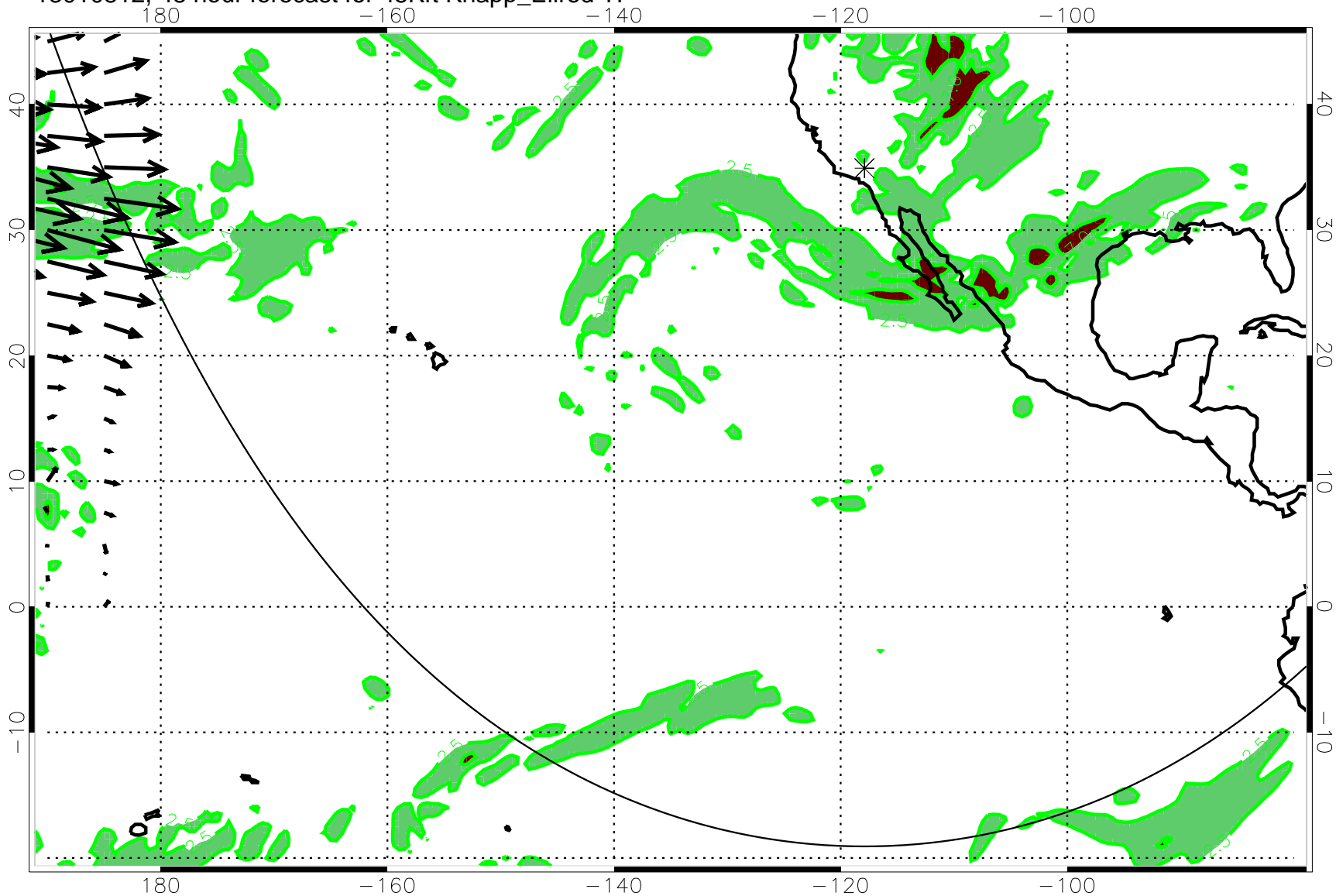
13010812, 48 hour forecast for 45Kft Knapp_Ellrod TI
