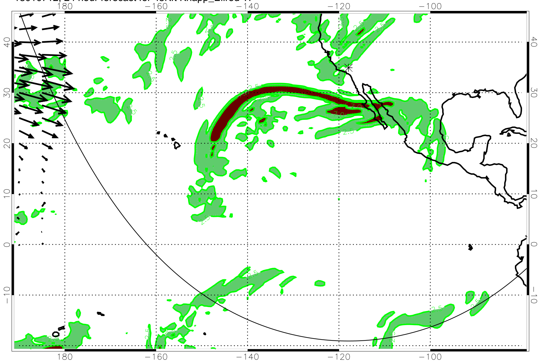
13010712, 24 hour forecast for 45Kft Knapp_Ellrod TI
