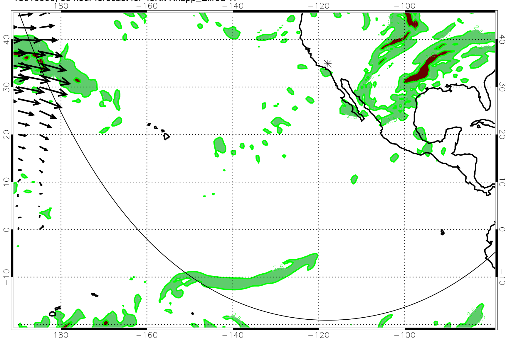
13010906, 66 hour forecast for 45Kft Knapp_Ellrod TI
