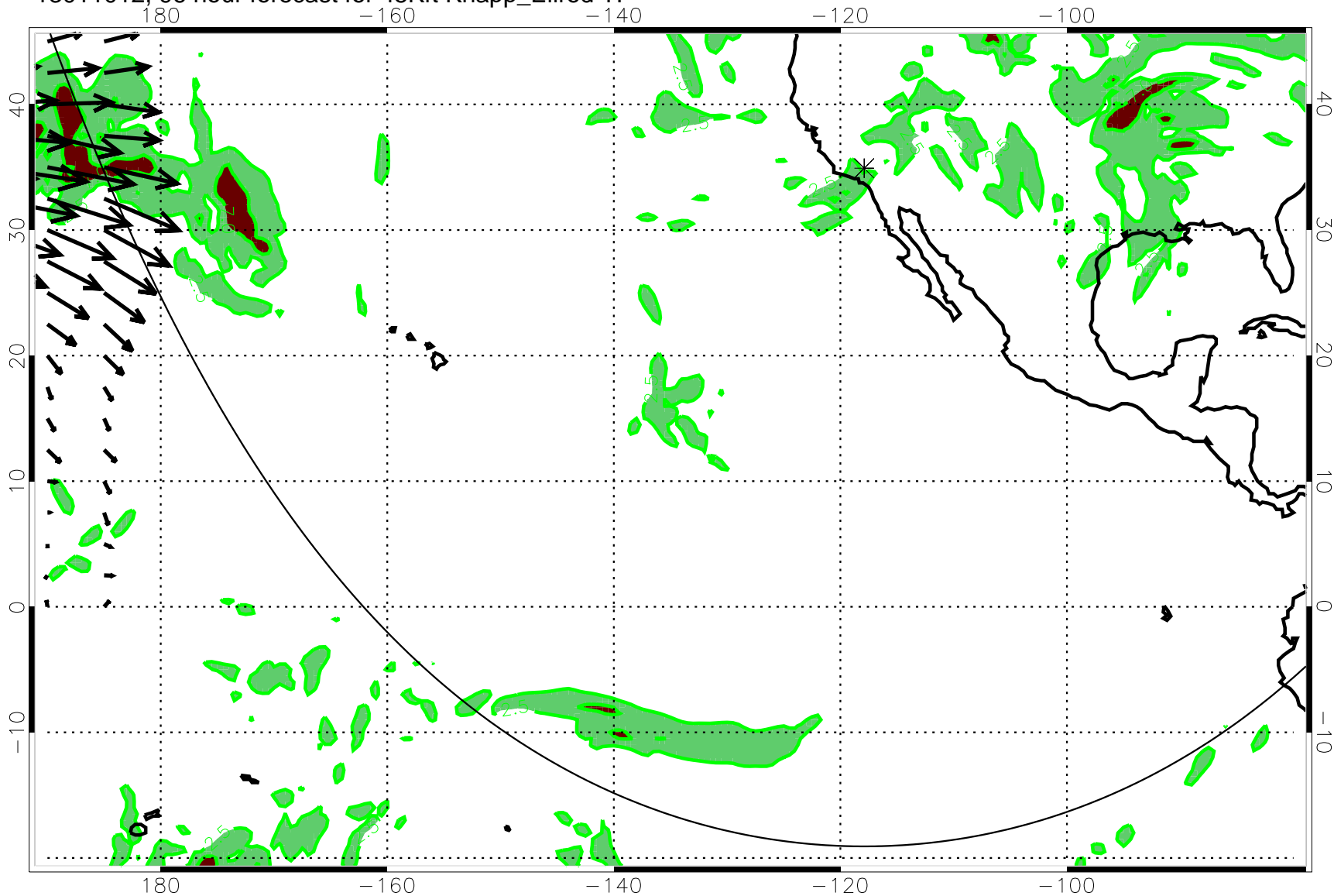
13011012, 96 hour forecast for 45Kft Knapp_Ellrod TI
