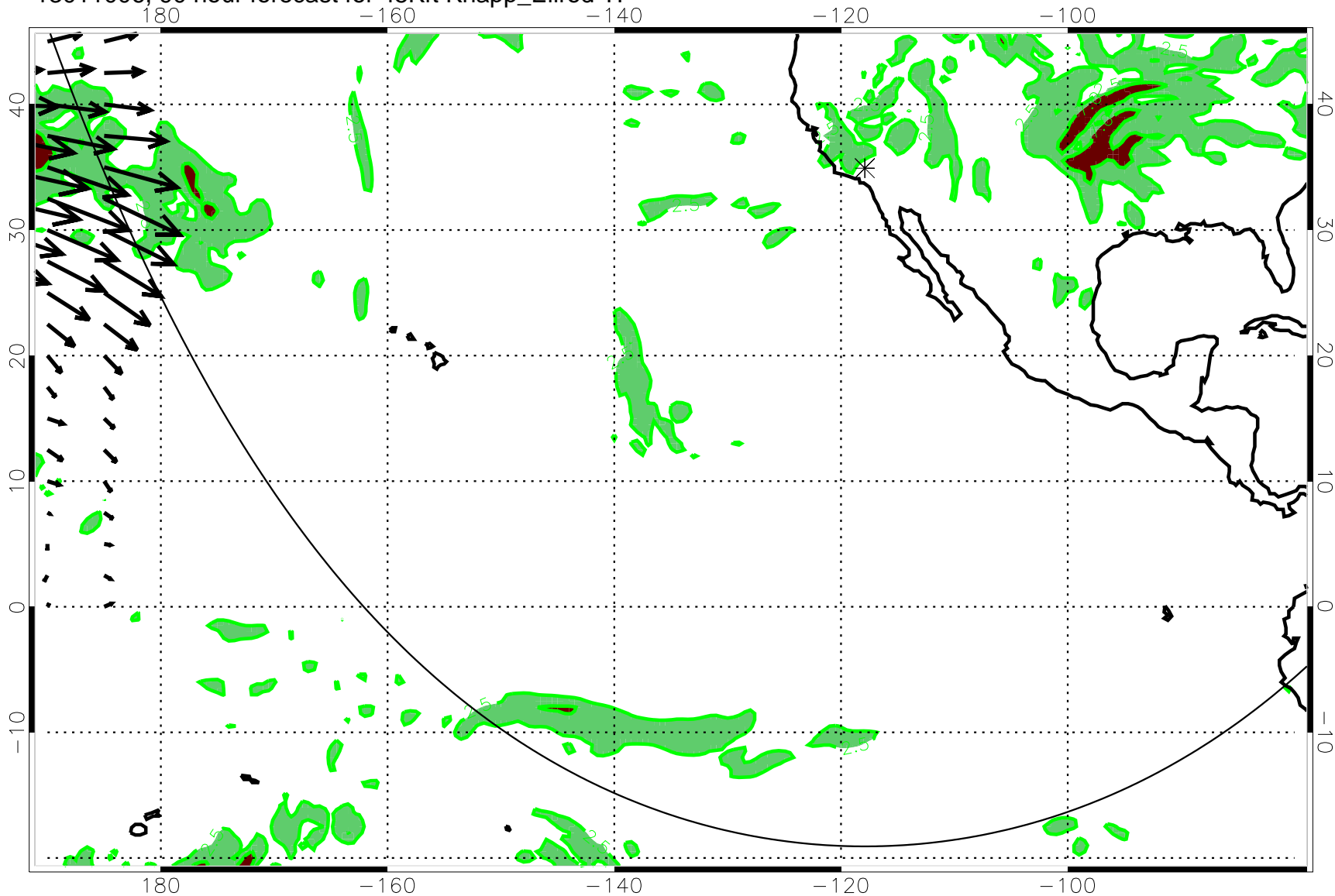
13011006, 90 hour forecast for 45Kft Knapp_Ellrod TI
