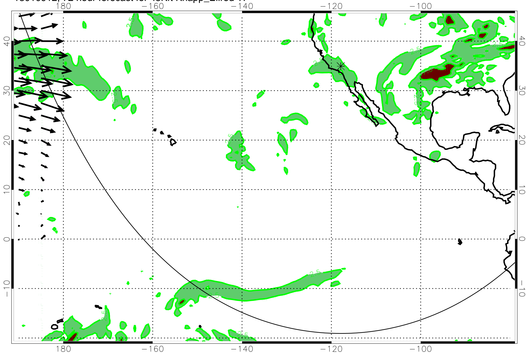
13010912, 72 hour forecast for 45Kft Knapp_Ellrod TI
