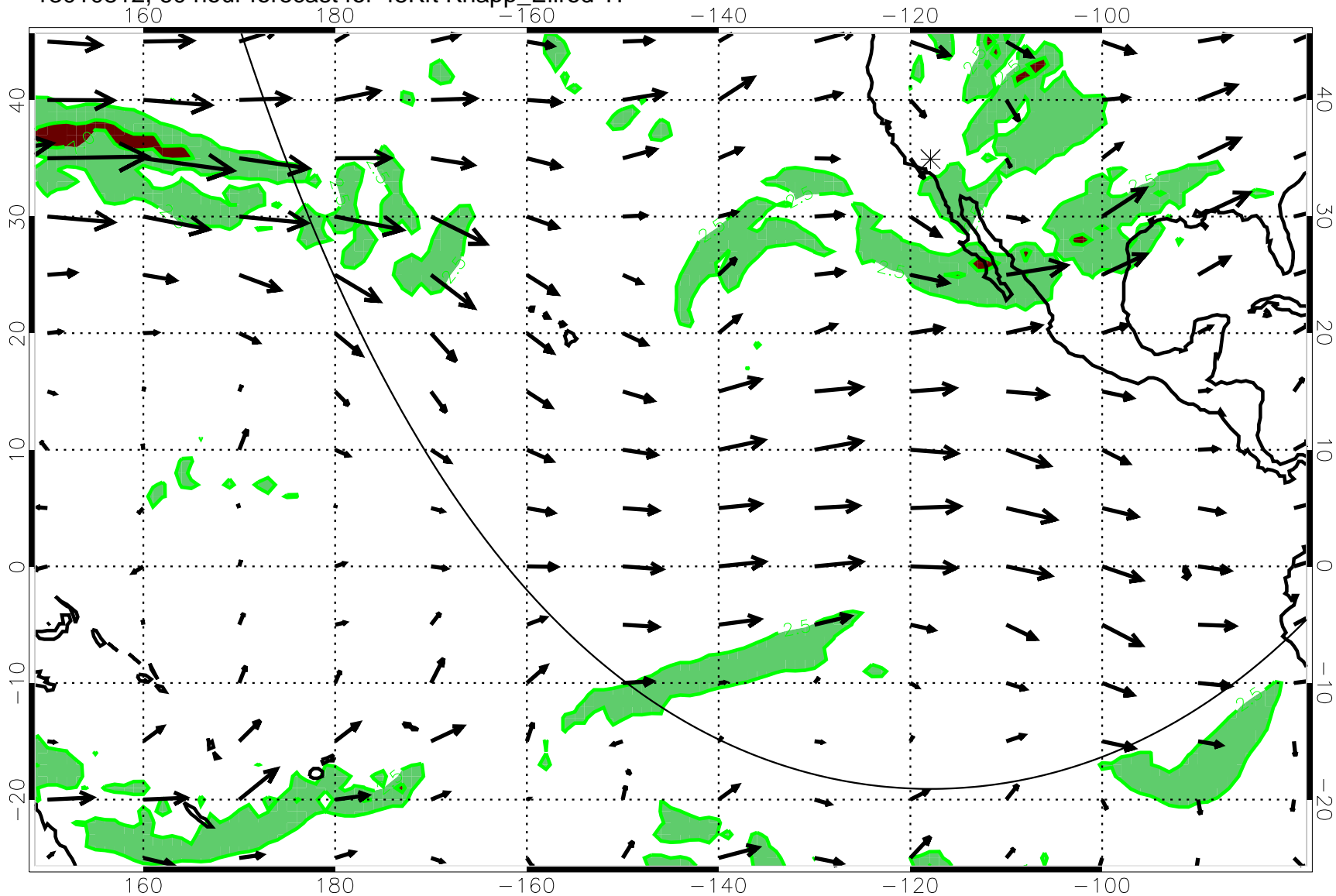
13010812, 60 hour forecast for 45Kft Knapp_Ellrod T1
