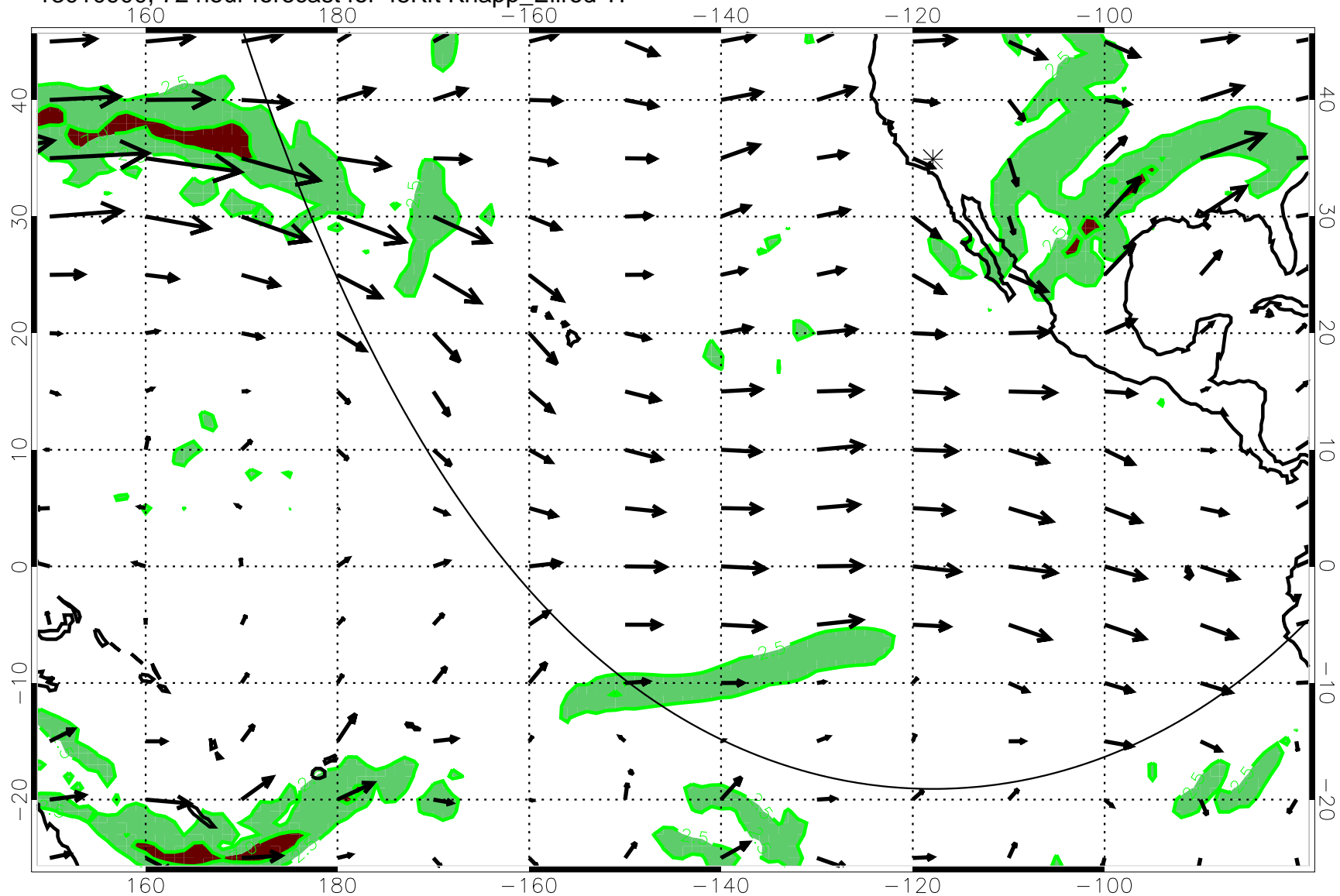
13010900, 72 hour forecast for 45Kft Knapp_Ellrod T1
