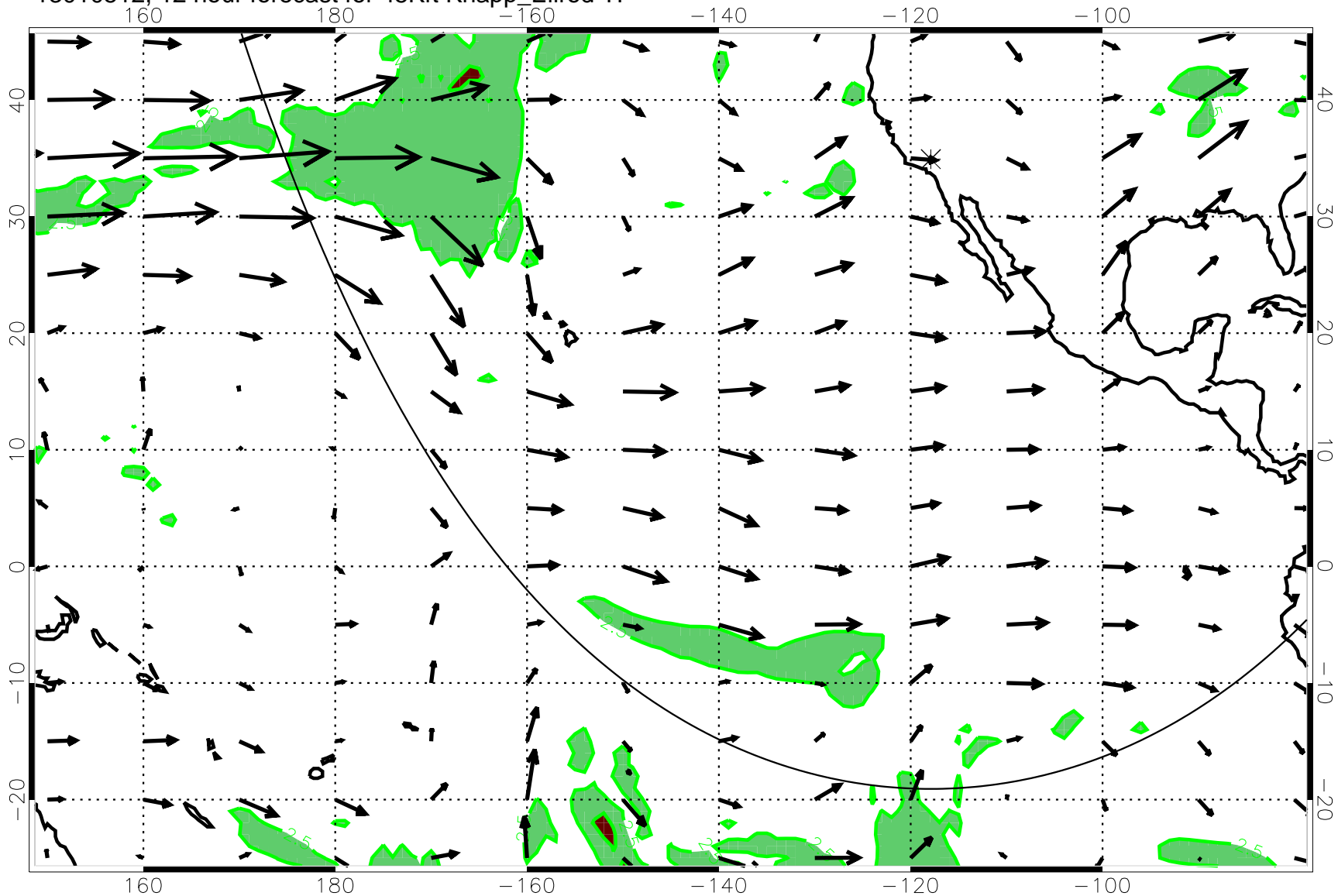
13010512, 12 hour forecast for 45Kft Knapp_Ellrod TI
