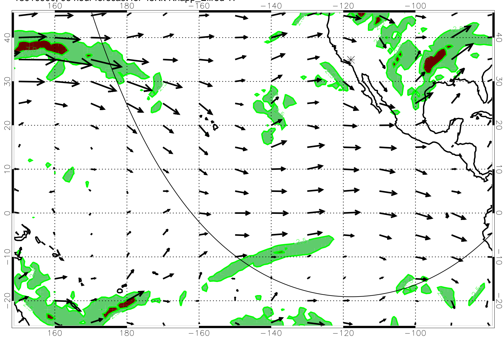
13010900, 96 hour forecast for 45Kft Knapp_Ellrod T1
