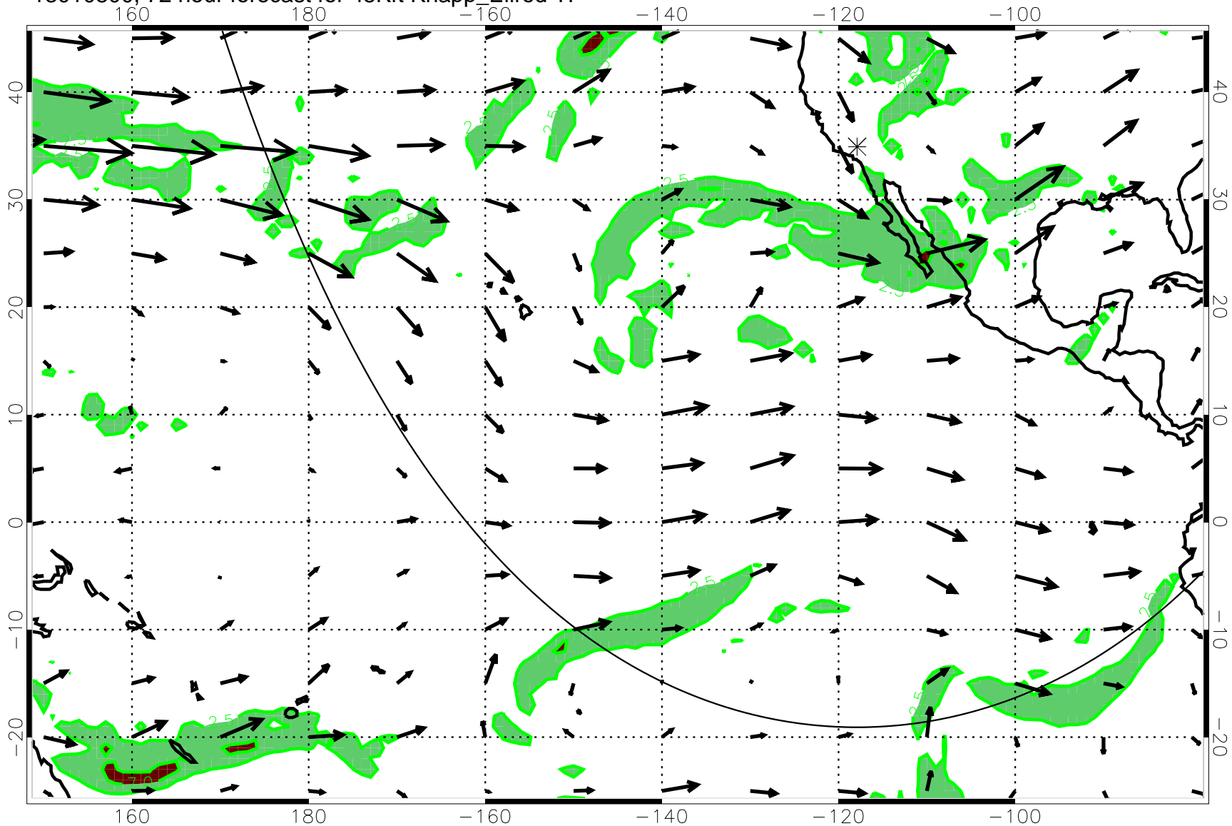
13010800, 72 hour forecast for 45Kft Knapp_Ellrod T1
