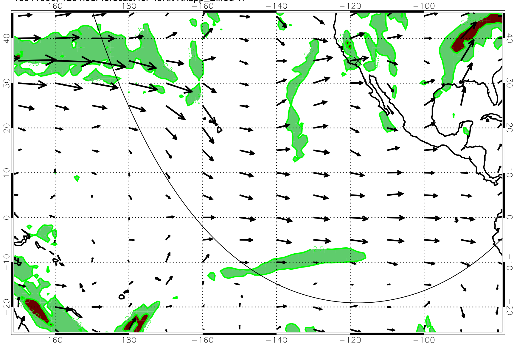
13011000, 120 hour forecast for 45Kft Knapp_Ellrod T1
