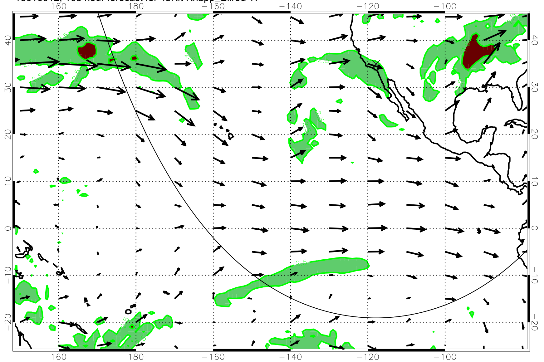
13010912, 108 hour forecast for 45Kft Knapp_Ellrod T1
