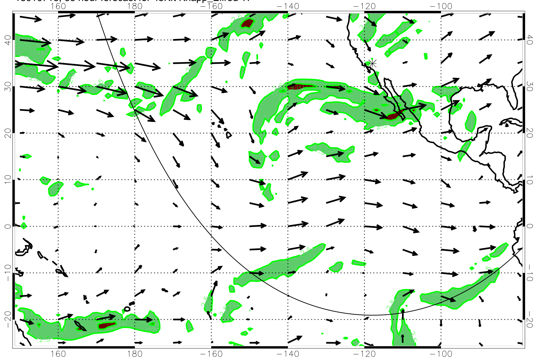
13010718, 66 hour forecast for 45Kft Knapp_Ellrod T1
