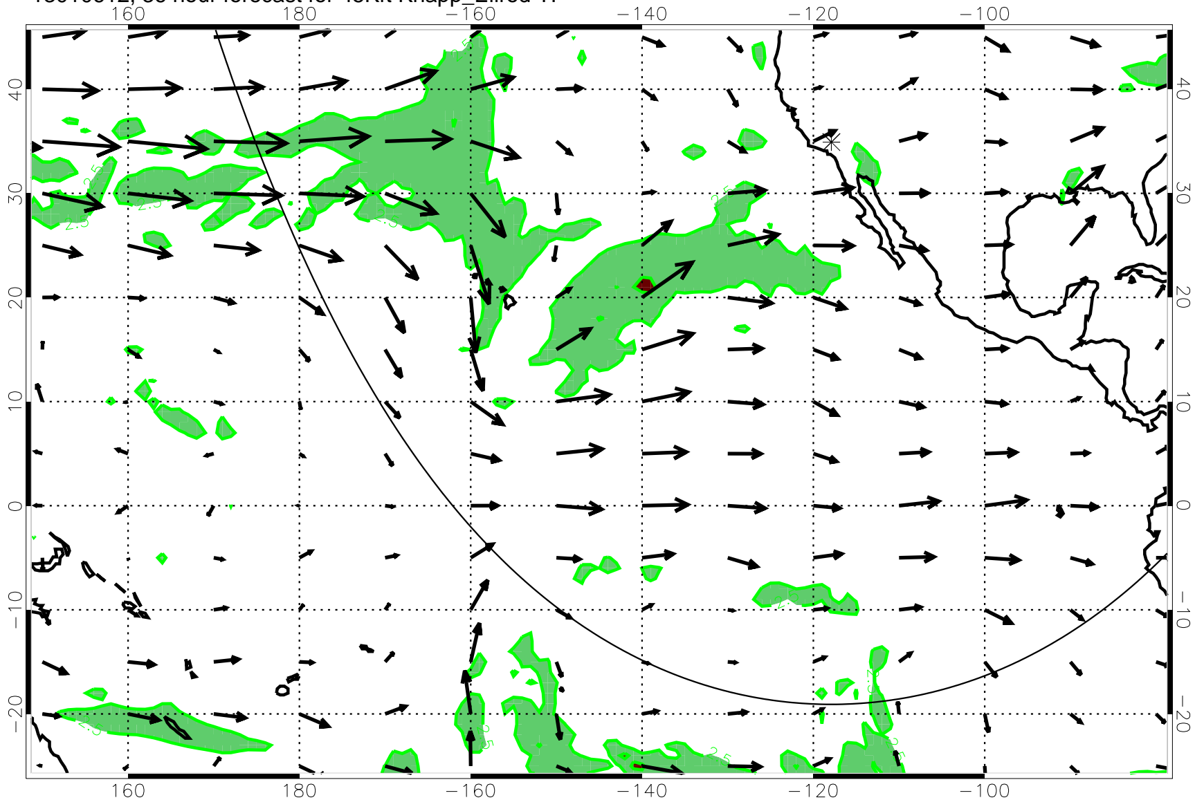
13010612, 36 hour forecast for 45Kft Knapp_Ellrod T1
