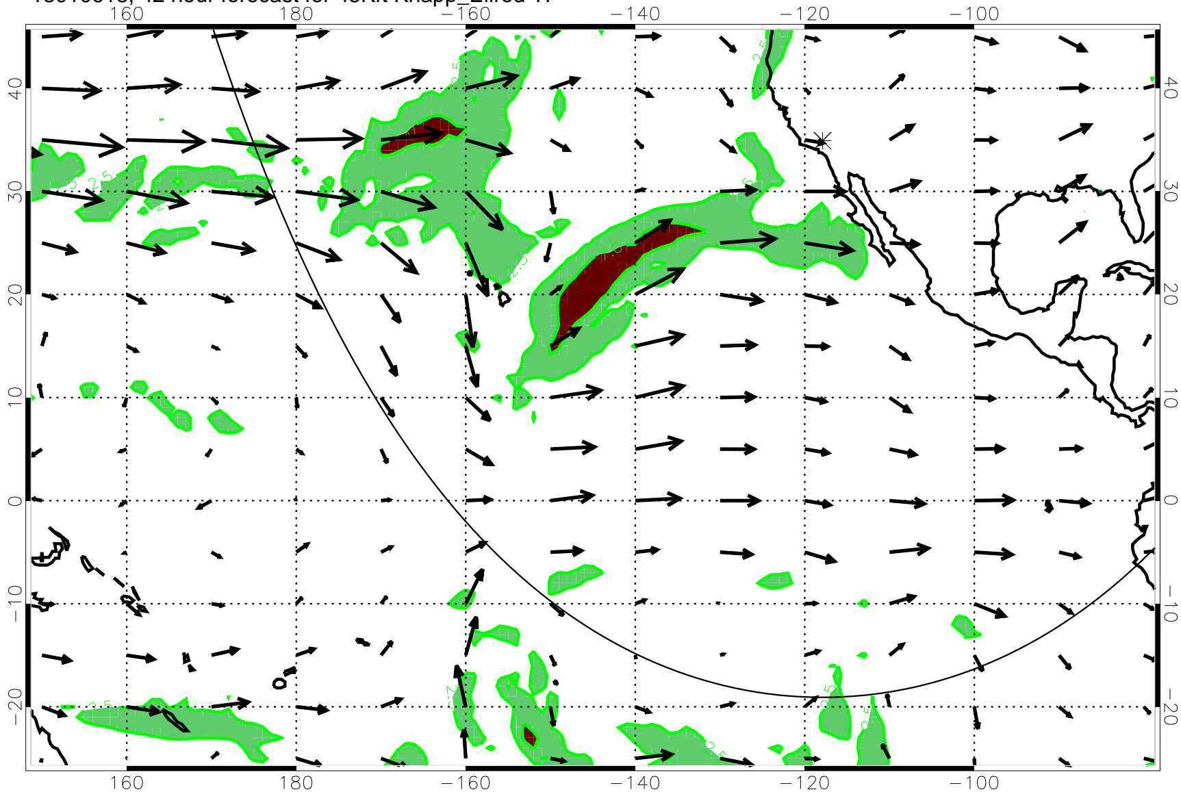
13010618, 42 hour forecast for 45Kft Knapp_Ellrod TI
