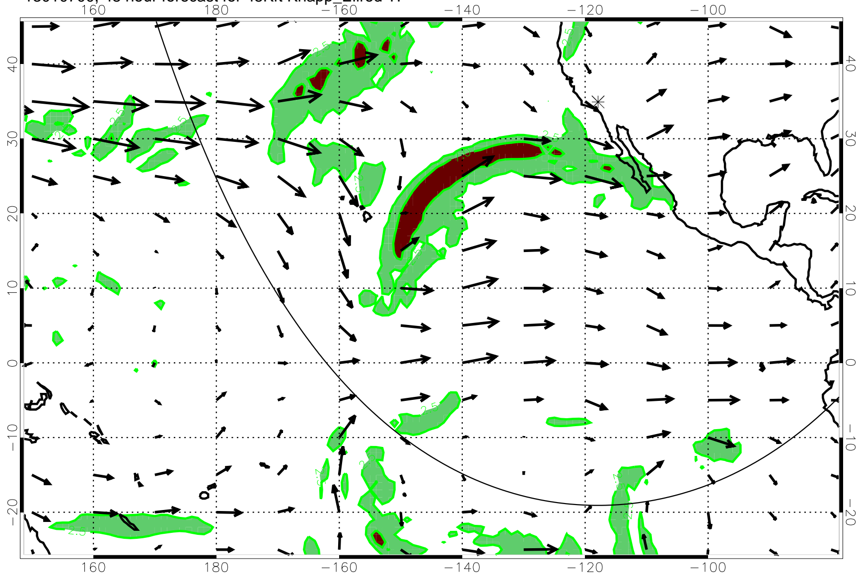
13010700, 48 hour forecast for 45Kft Knapp_Ellrod T1
