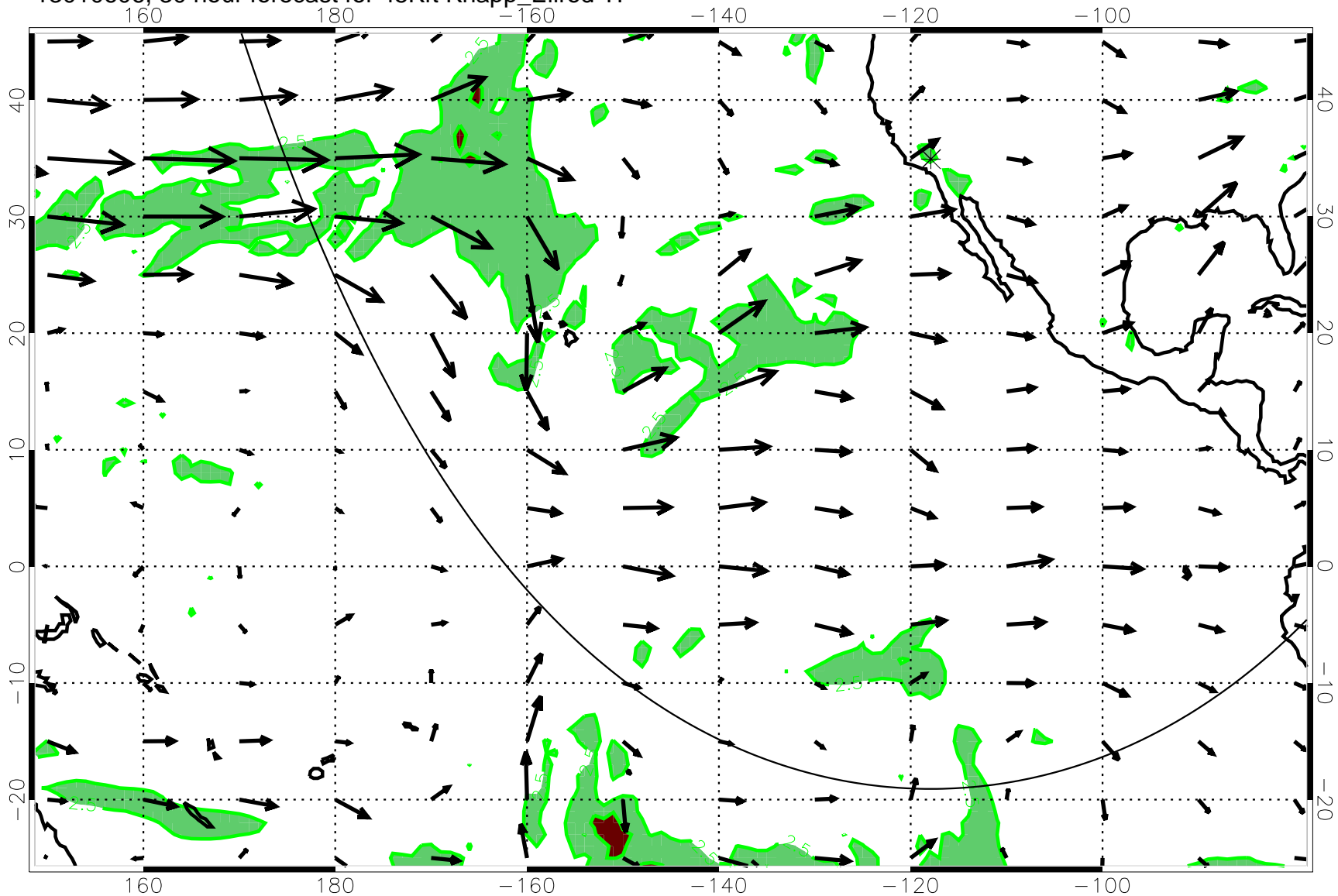
13010606, 30 hour forecast for 45Kft Knapp_Ellrod T1
