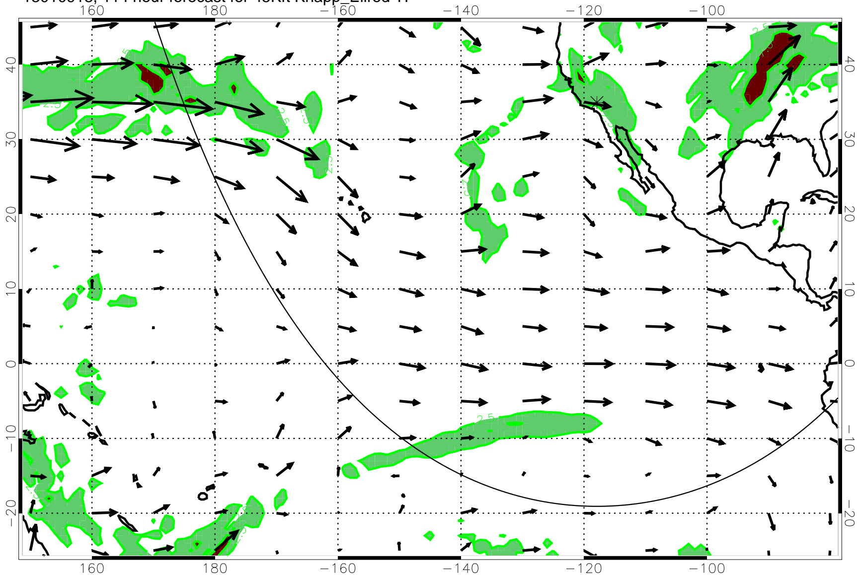
13010918, 114 hour forecast for 45Kft Knapp_Ellrod T1
