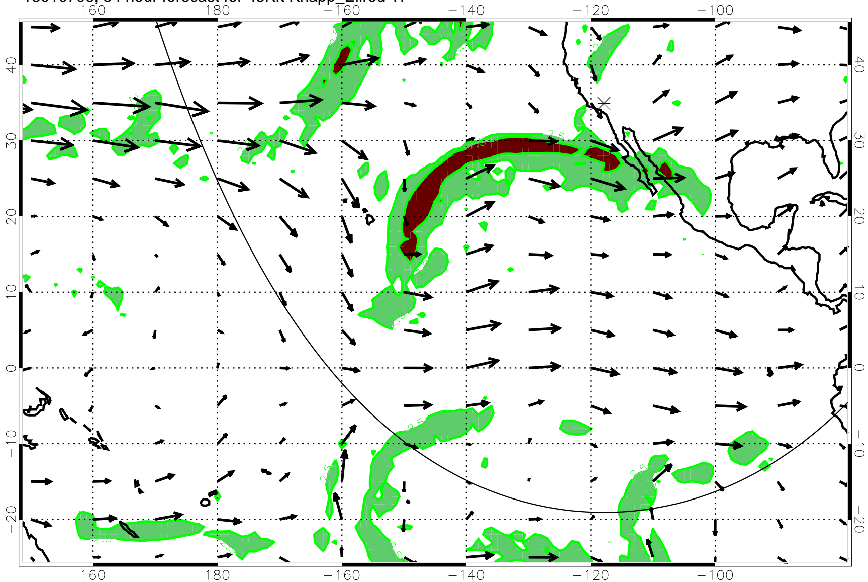
13010706, 54 hour forecast for 45Kft Knapp_Ellrod T1
