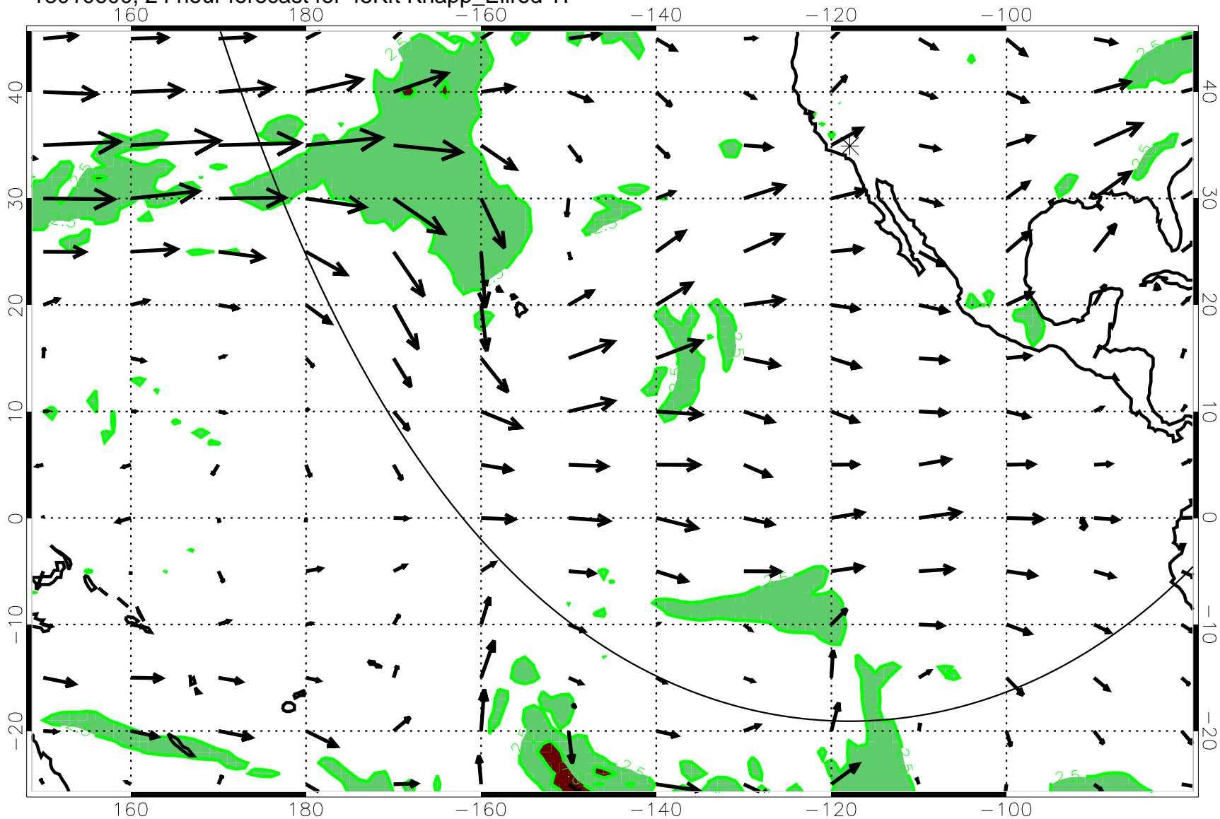
13010600, 24 hour forecast for 45Kft Knapp_Ellrod T1
