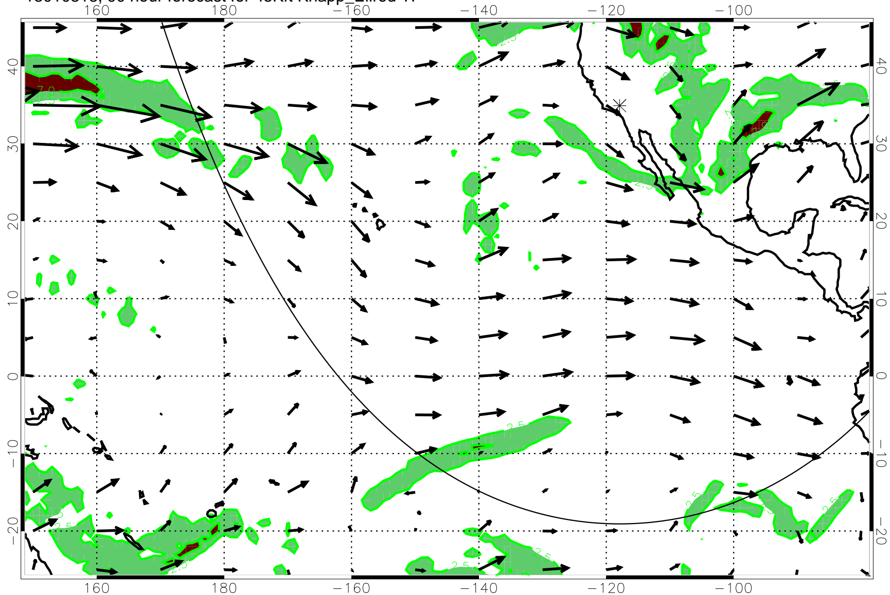
13010818, 90 hour forecast for 45Kft Knapp_Ellrod TI
