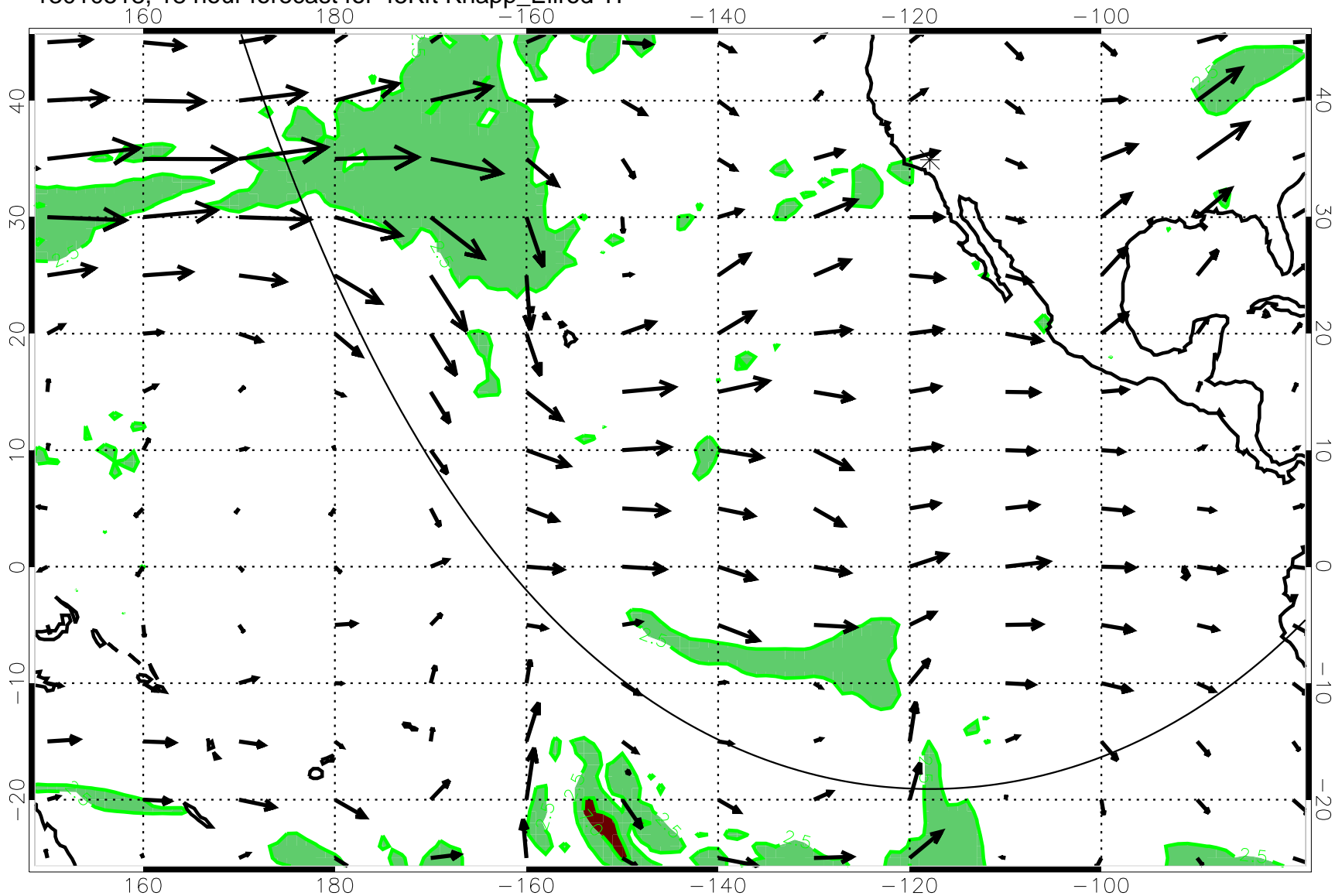
13010518, 18 hour forecast for 45Kft Knapp_Ellrod T1
