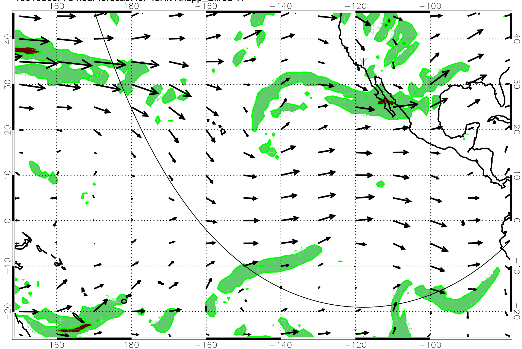
13010806, 78 hour forecast for 45Kft Knapp_Ellrod T1
