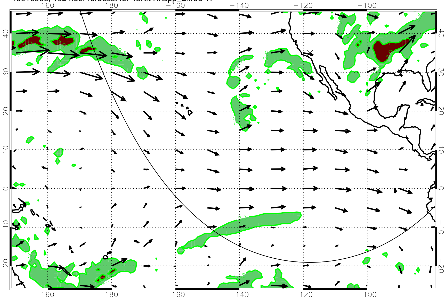
13010906, 102 hour forecast for 45Kft Knapp_Ellrod T1
