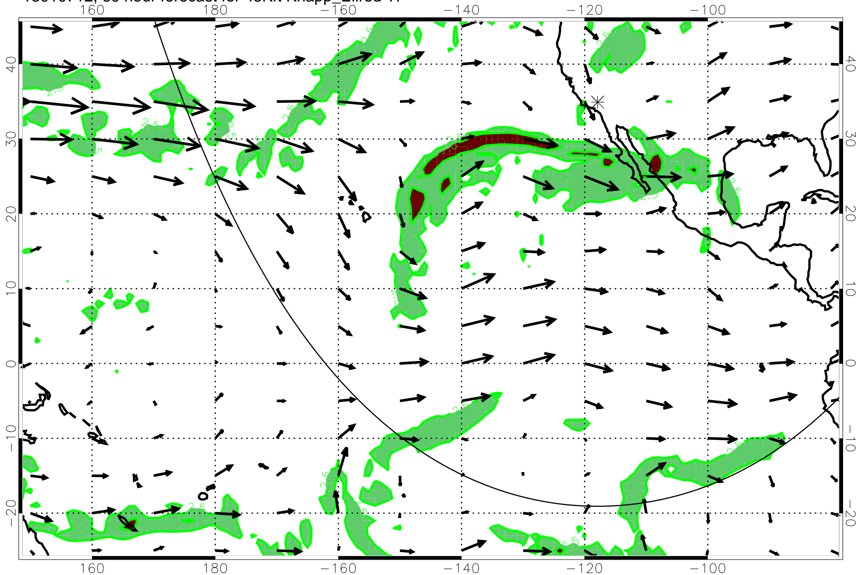
13010712, 60 hour forecast for 45Kft Knapp_Ellrod TI
