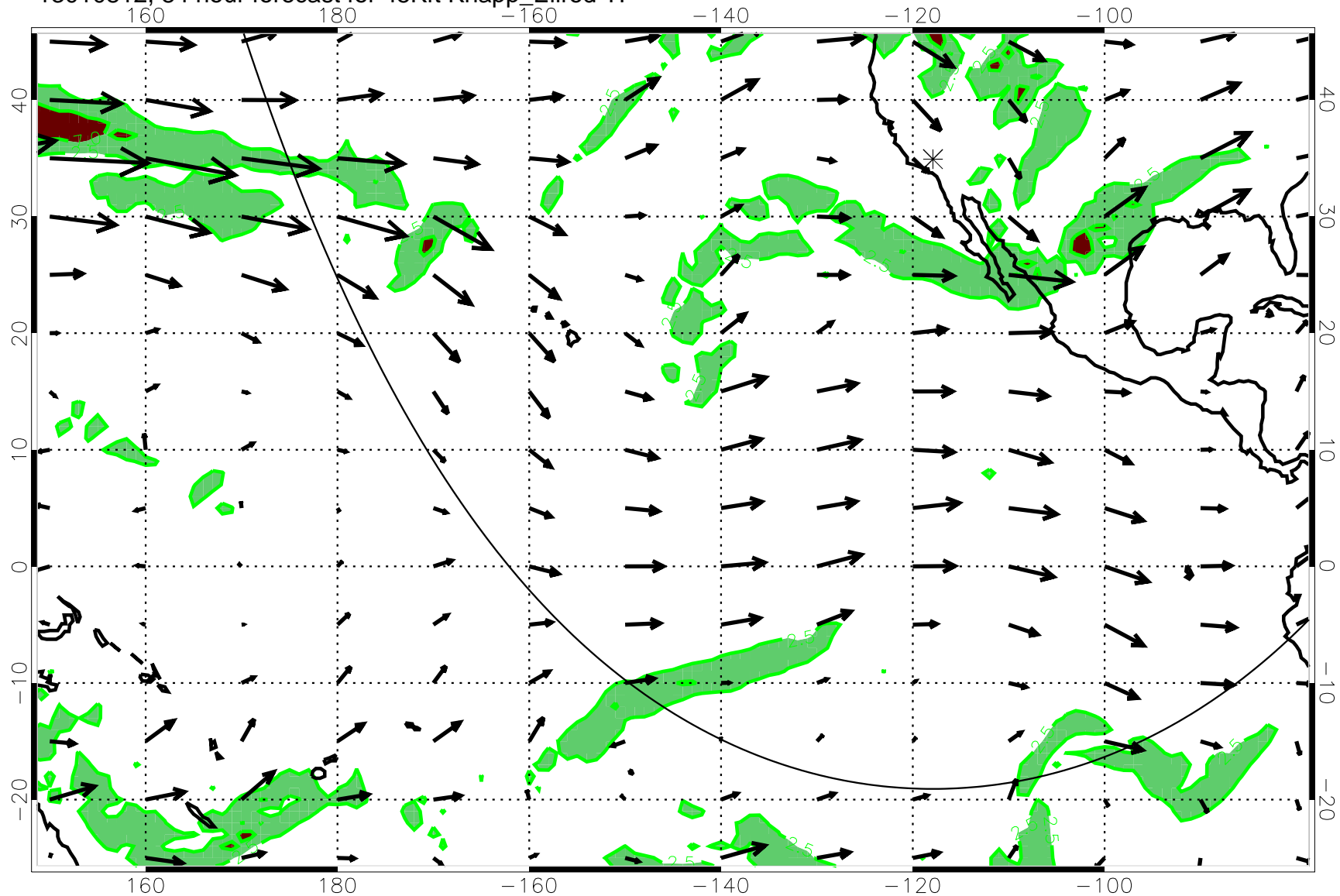
13010812, 84 hour forecast for 45Kft Knapp_Ellrod T1
