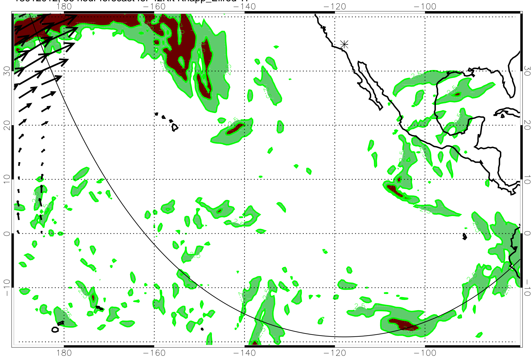
13012012, 36 hour forecast for 42Kft Knapp_Ellrod TI
