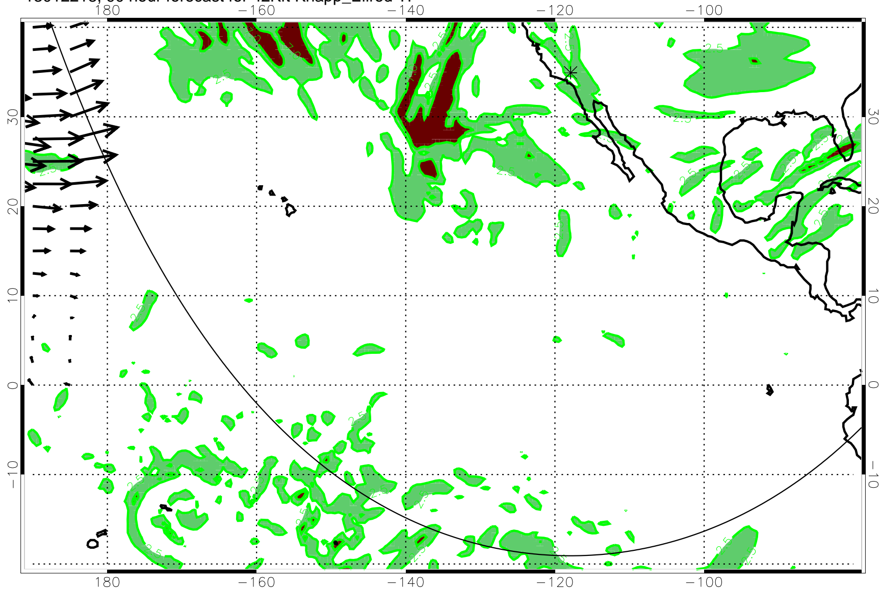
13012218, 90 hour forecast for 42Kft Knapp_Ellrod TI
