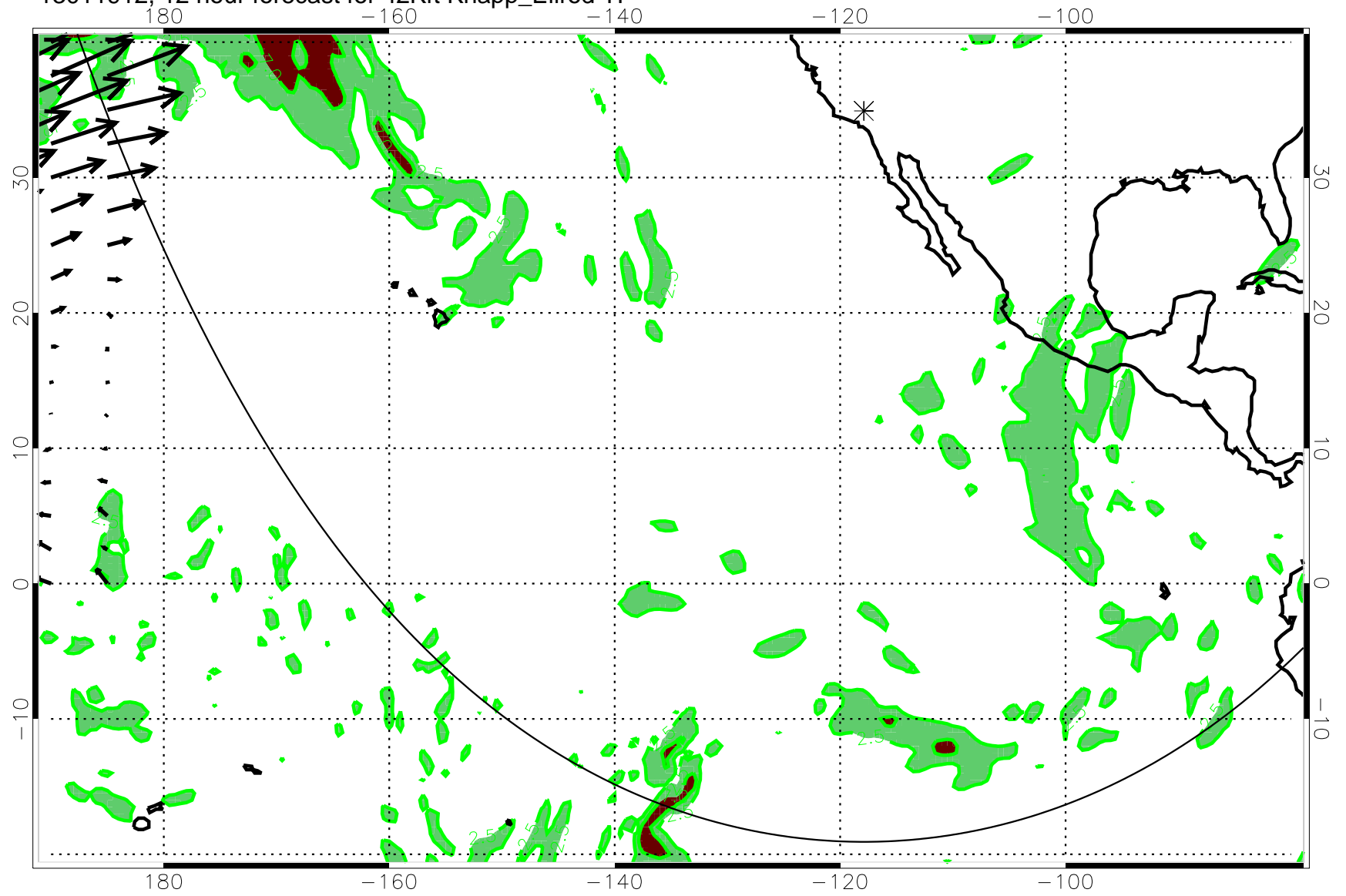
13011912, 12 hour forecast for 42Kft Knapp_Ellrod TI
