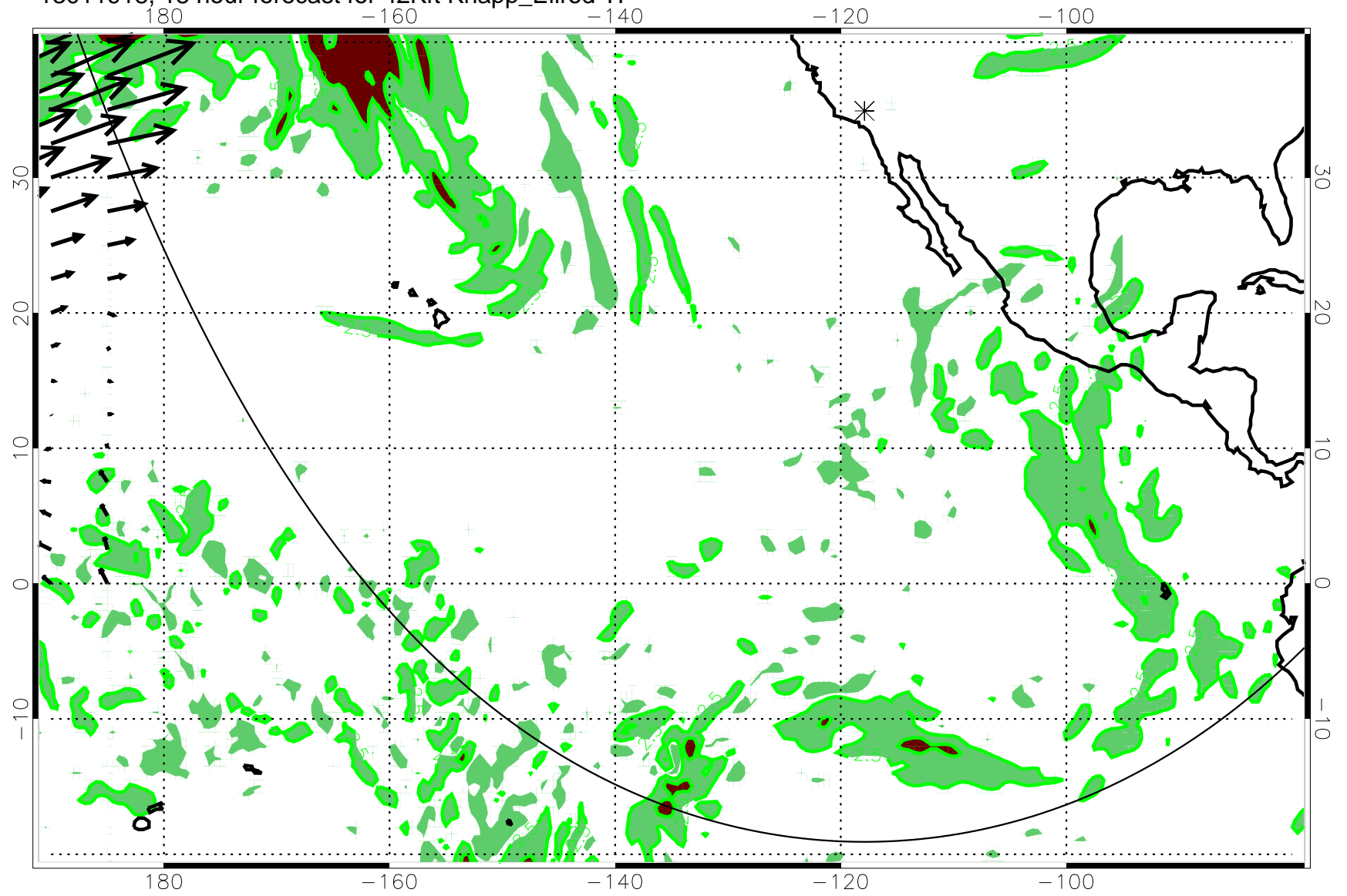
13011918, 18 hour forecast for 42Kft Knapp_Ellrod TI
