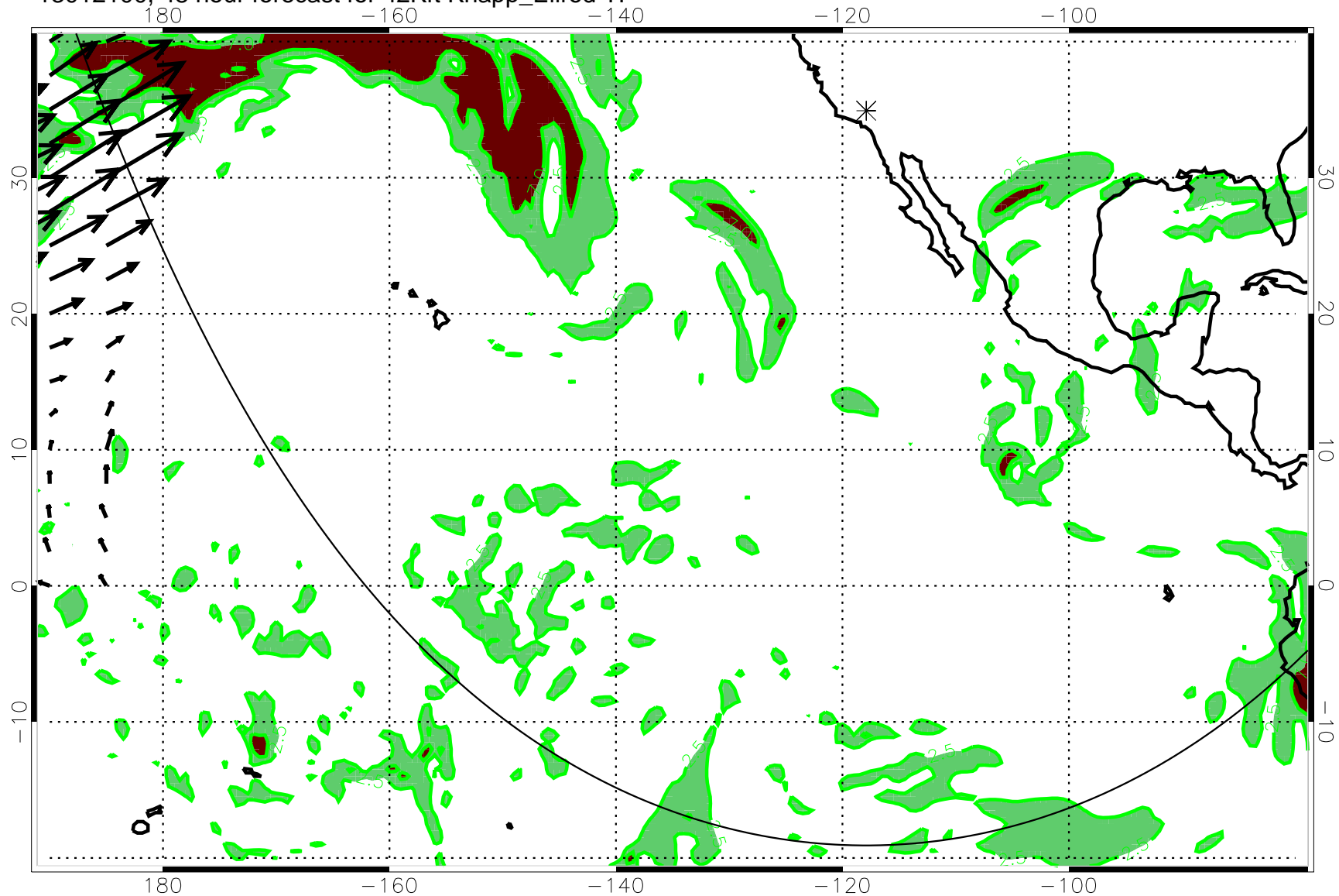
13012100, 48 hour forecast for 42Kft Knapp_Ellrod TI
