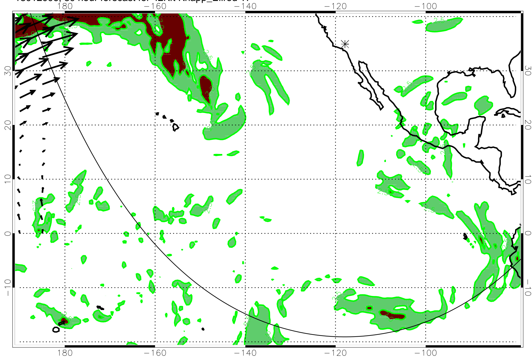
13012006, 30 hour forecast for 42Kft Knapp_Ellrod TI
