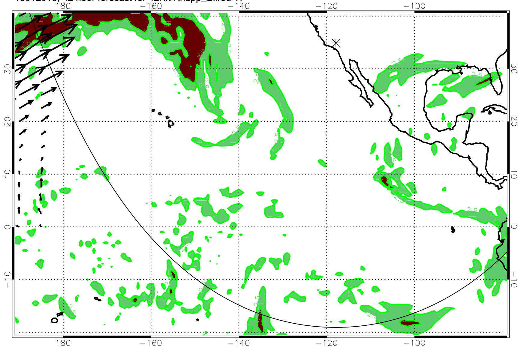
13012018, 42 hour forecast for 42Kft Knapp_Ellrod TI
