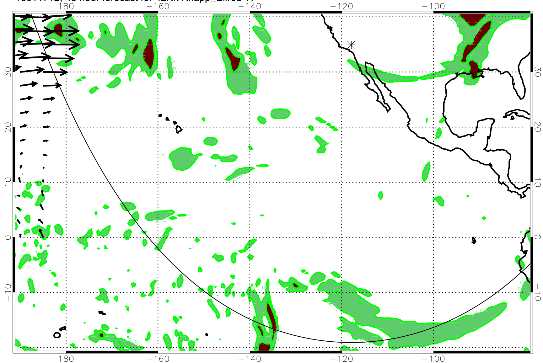
13011712, 48 hour forecast for 42Kft Knapp_Ellrod TI
