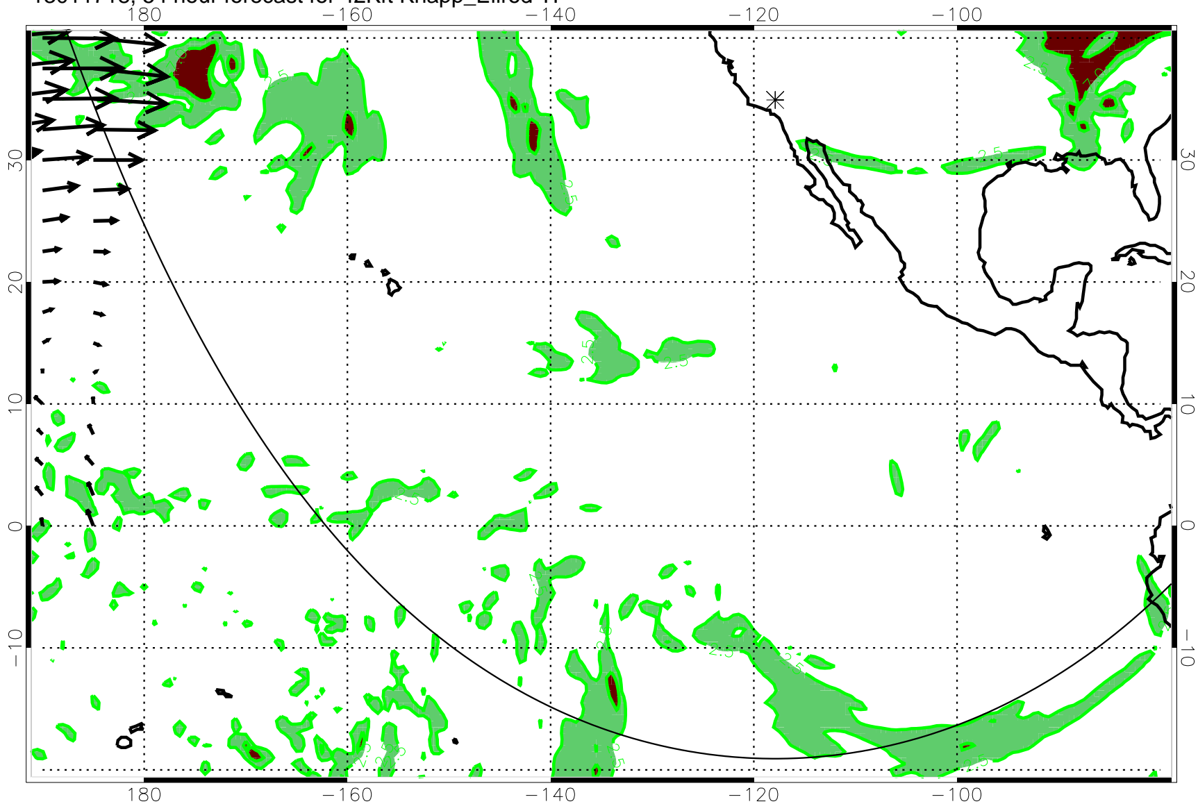
13011718, 54 hour forecast for 42Kft Knapp_Ellrod TI
