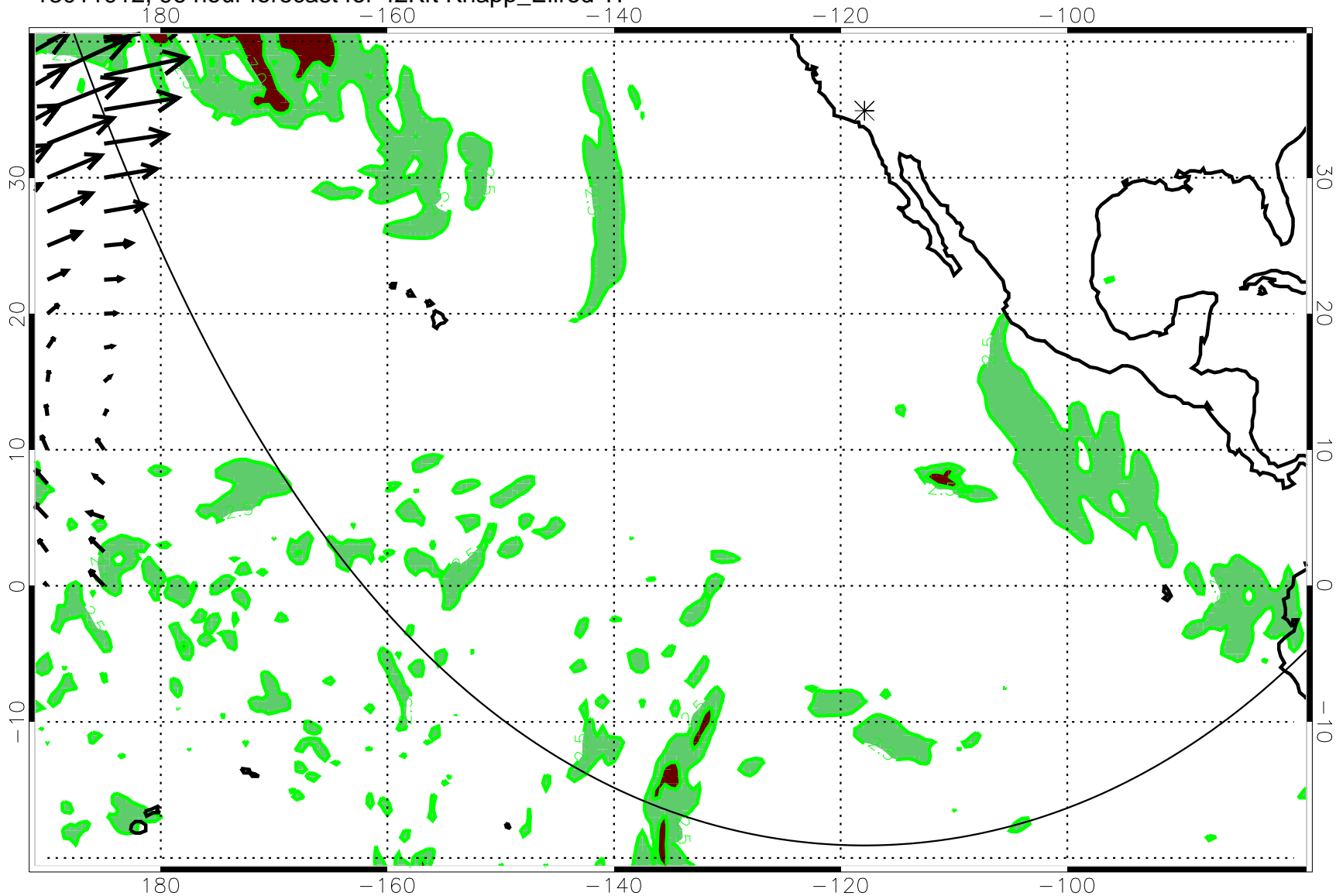
13011912, 96 hour forecast for 42Kft Knapp_Ellrod TI
