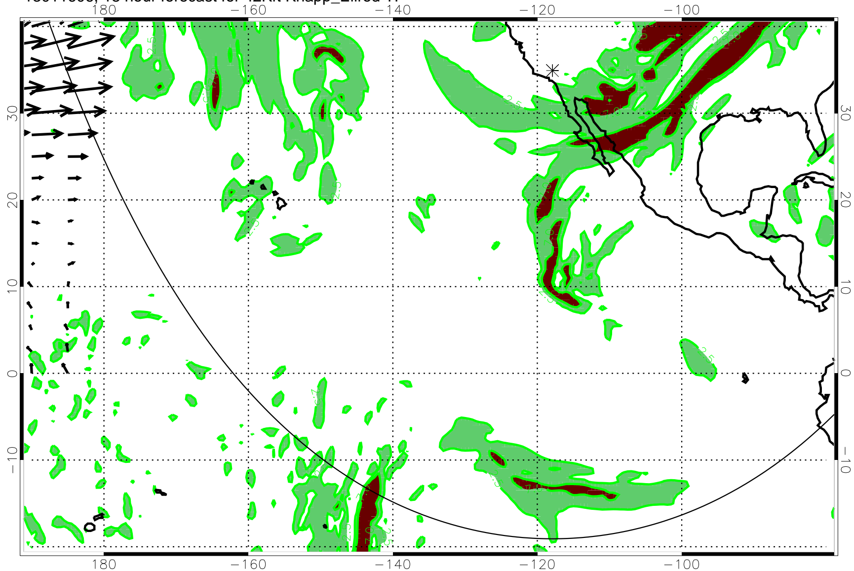
13011606, 18 hour forecast for 42Kft Knapp_Ellrod TI
