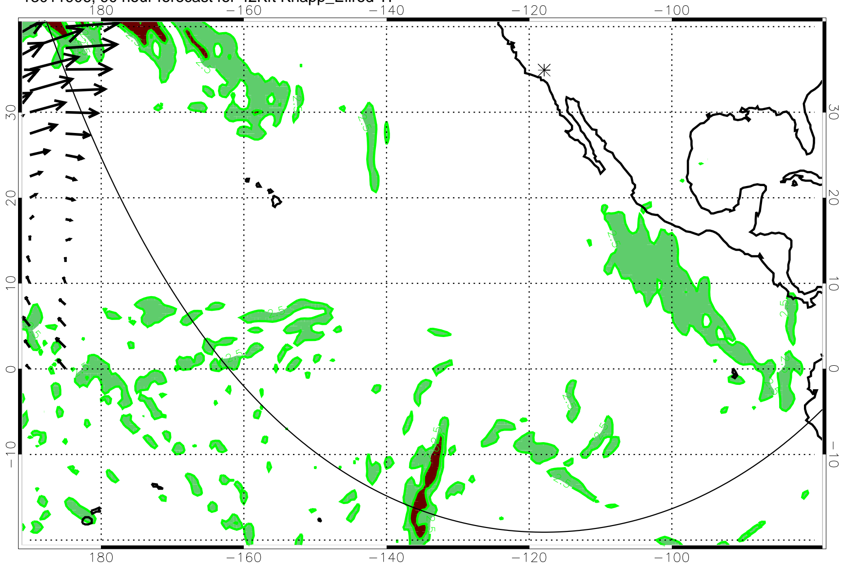
13011906, 90 hour forecast for 42Kft Knapp_Ellrod TI
