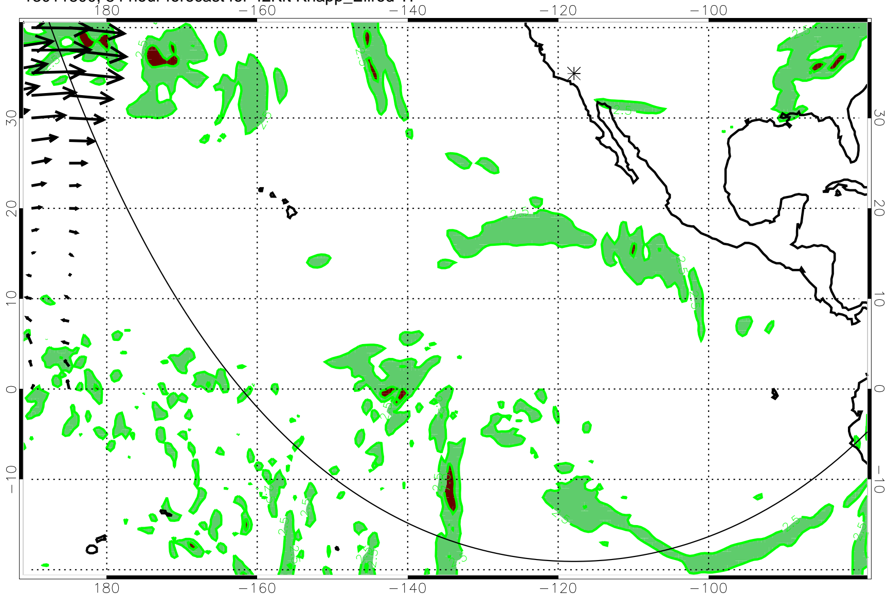
13011800, 84 hour forecast for 42Kft Knapp_Ellrod TI
