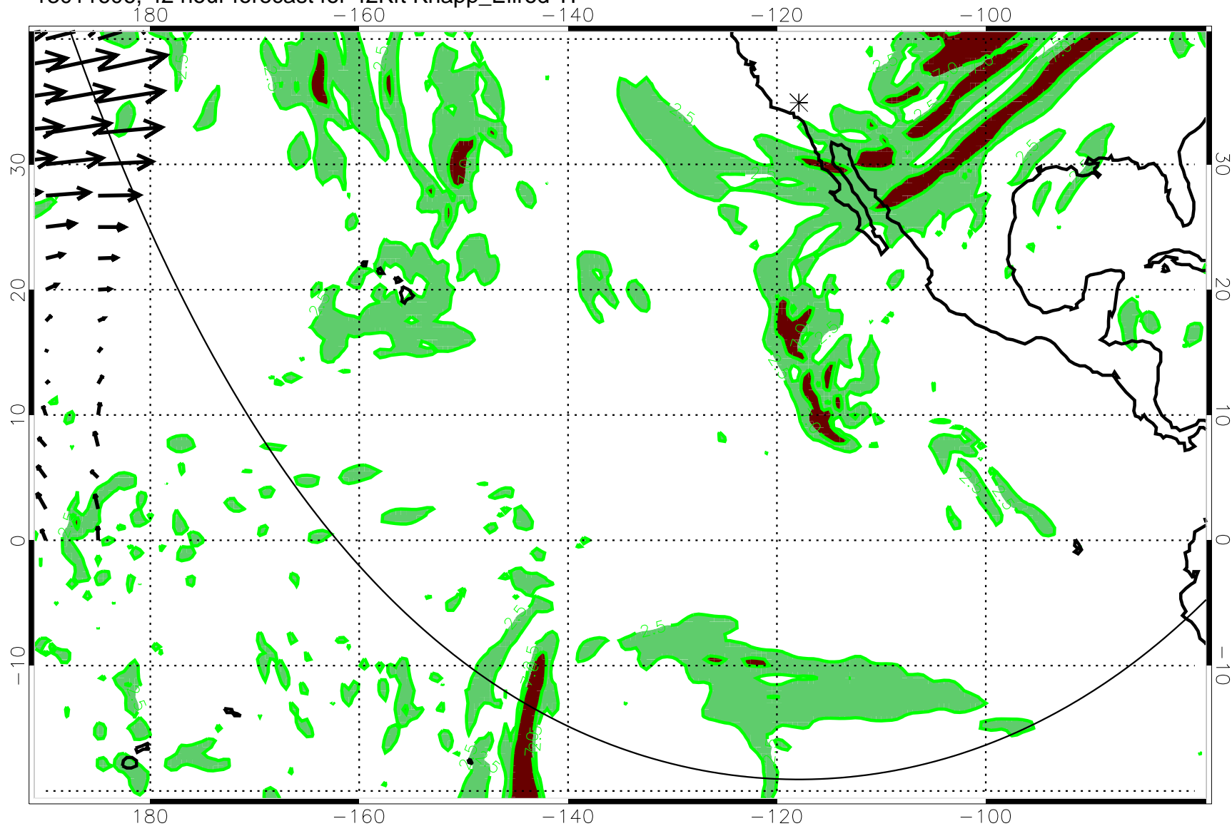
13011606, 42 hour forecast for 42Kft Knapp_Ellrod TI
