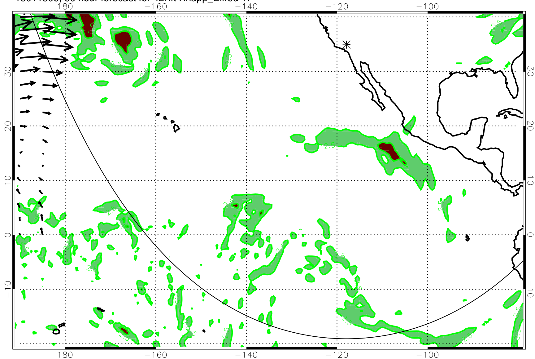
13011806, 90 hour forecast for 42Kft Knapp_Ellrod TI
