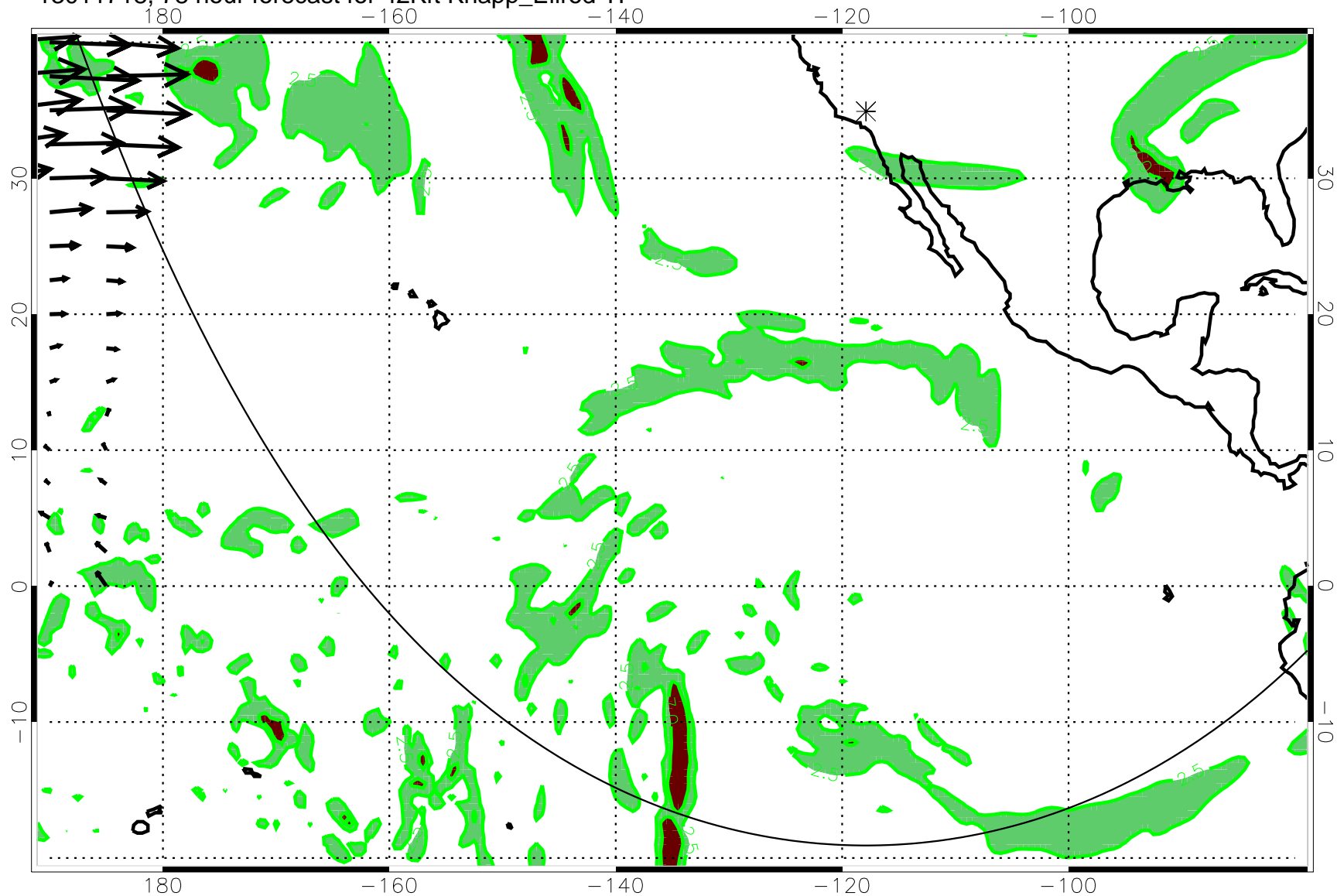
13011718, 78 hour forecast for 42Kft Knapp_Ellrod TI
