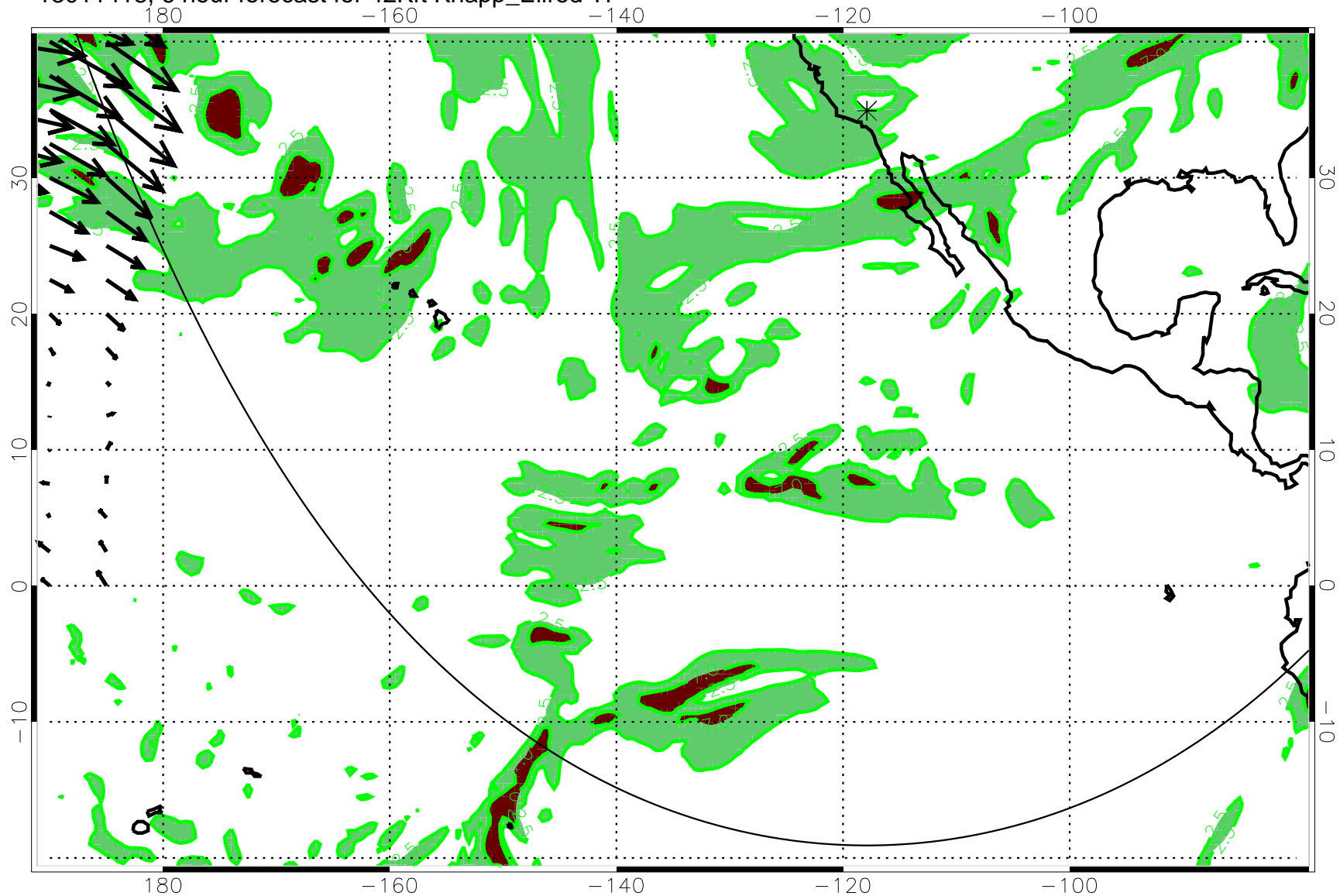
13011418, 6 hour forecast for 42Kft Knapp_Ellrod TI
