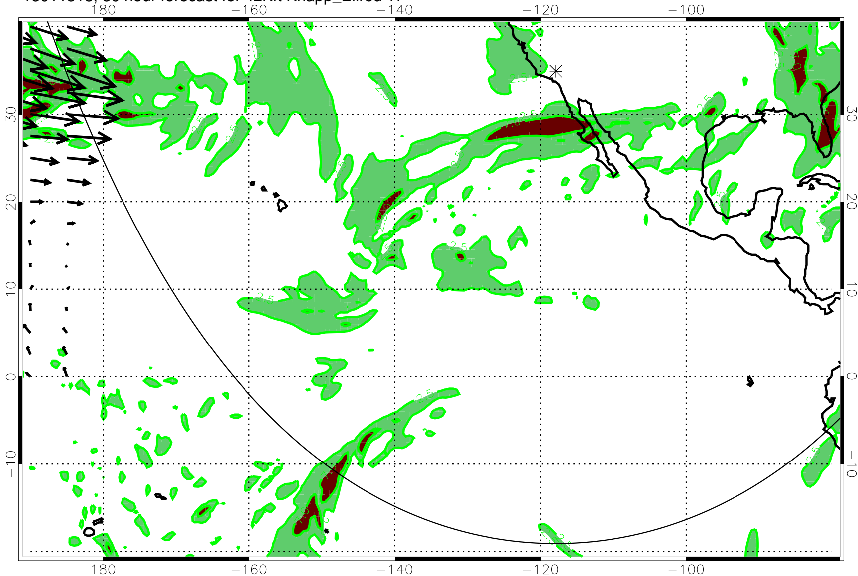
13011318, 30 hour forecast for 42Kft Knapp_Ellrod TI
