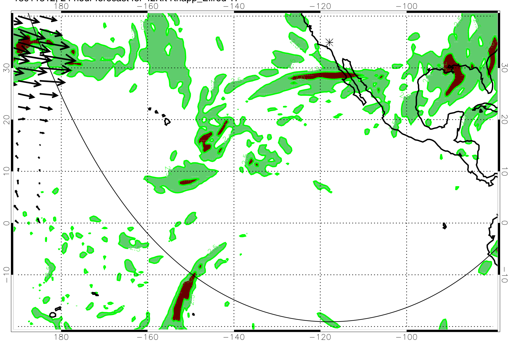
13011312, 24 hour forecast for 42Kft Knapp_Ellrod TI
