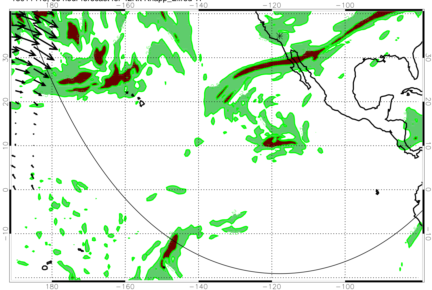
13011418, 66 hour forecast for 42Kft Knapp_Ellrod TI
