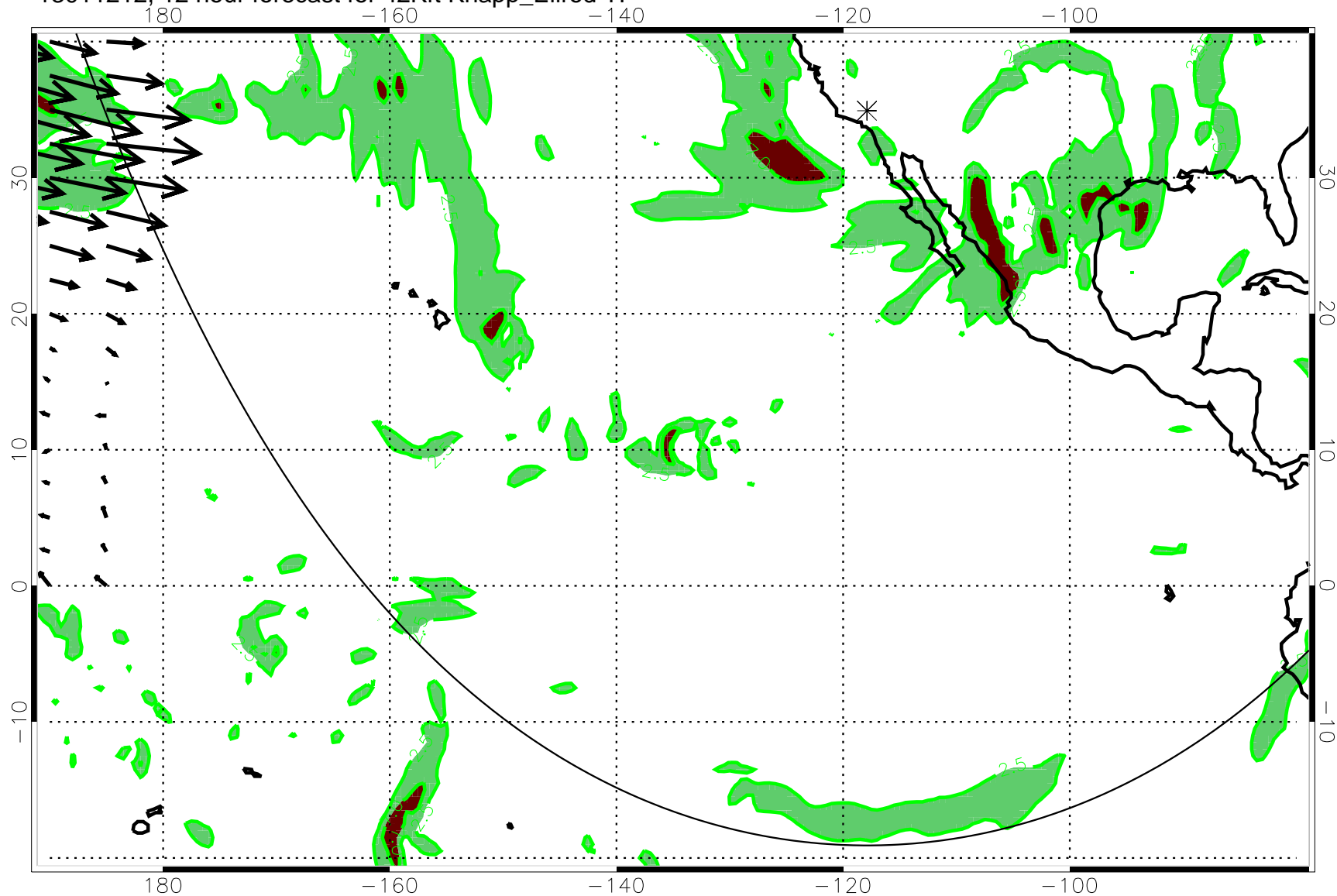
13011212, 12 hour forecast for 42Kft Knapp_Ellrod TI
