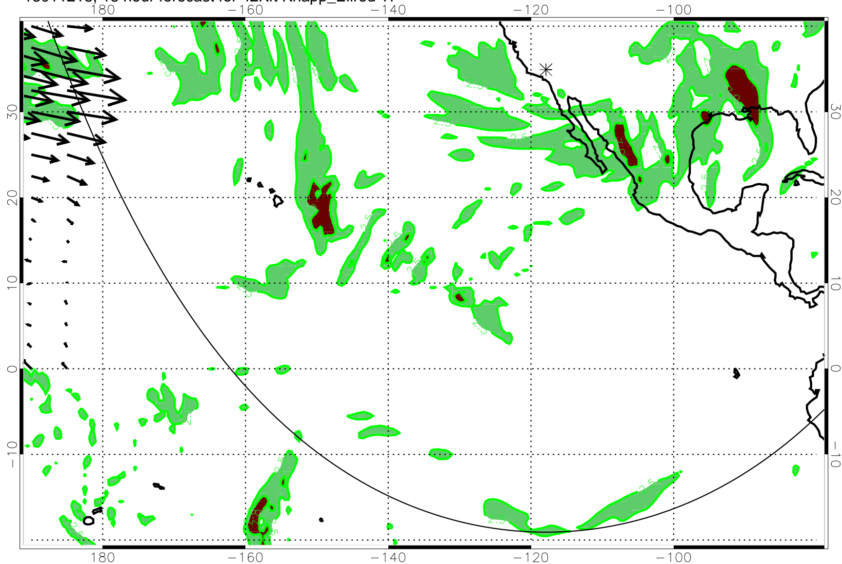
13011218, 18 hour forecast for 42Kft Knapp_Ellrod TI
