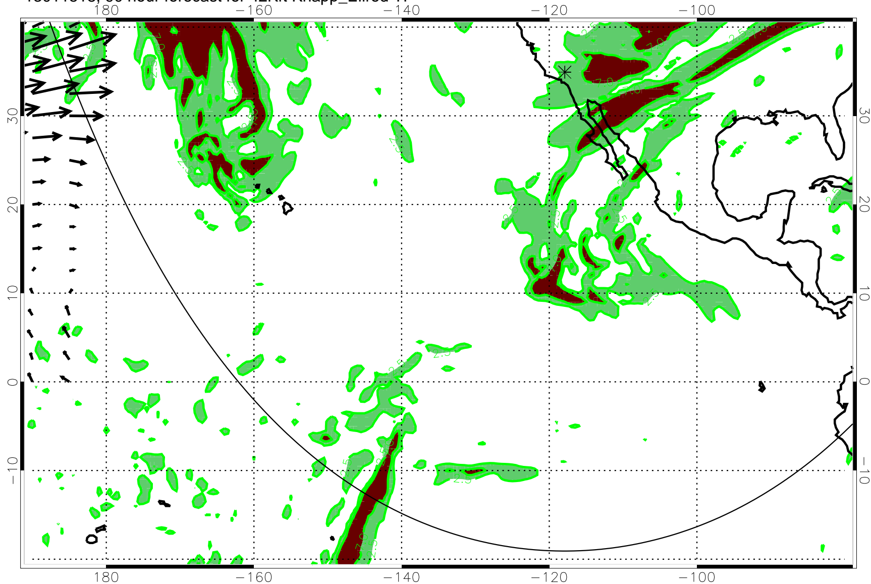
13011518, 90 hour forecast for 42Kft Knapp_Ellrod TI
