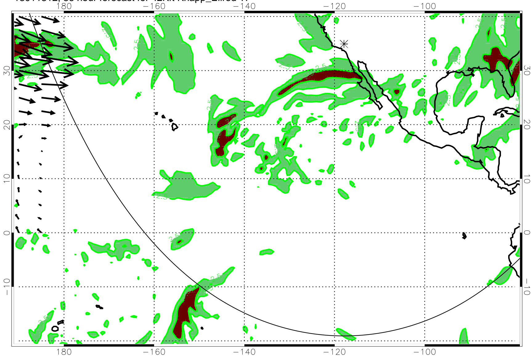
13011312, 36 hour forecast for 42Kft Knapp_Ellrod TI
