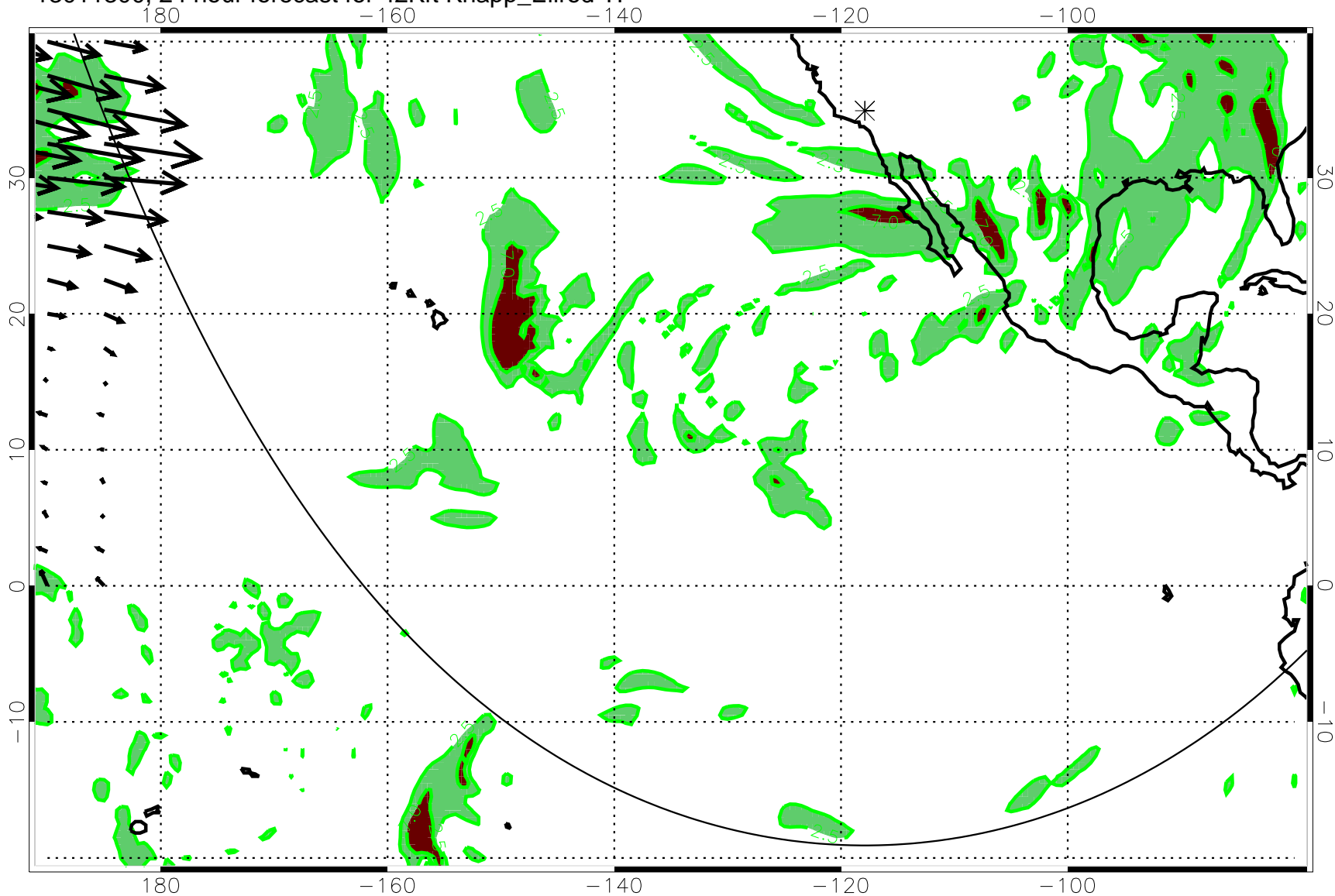
13011300, 24 hour forecast for 42Kft Knapp_Ellrod TI
