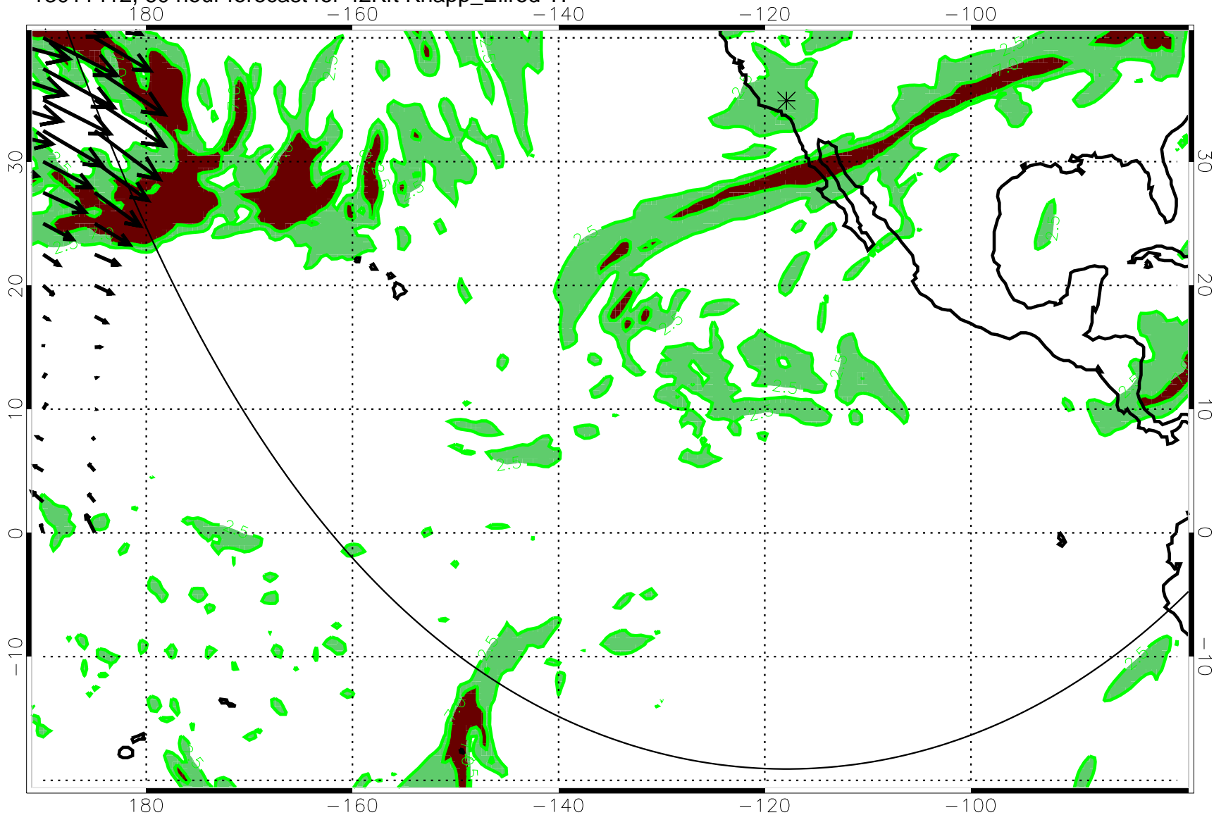
13011412, 60 hour forecast for 42Kft Knapp_Ellrod TI
