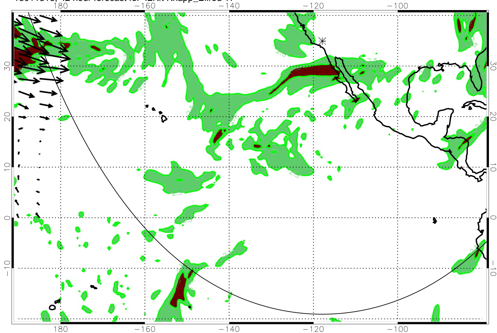
13011318, 42 hour forecast for 42Kft Knapp_Ellrod TI
