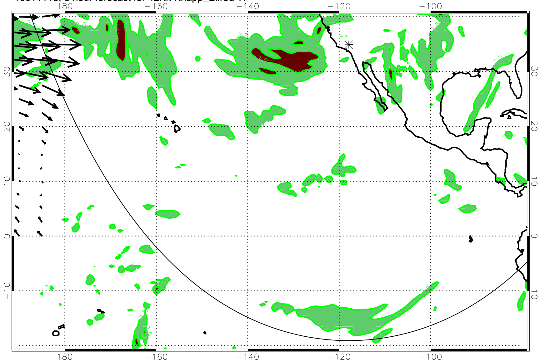
13011118, 6 hour forecast for 42Kft Knapp_Ellrod TI
