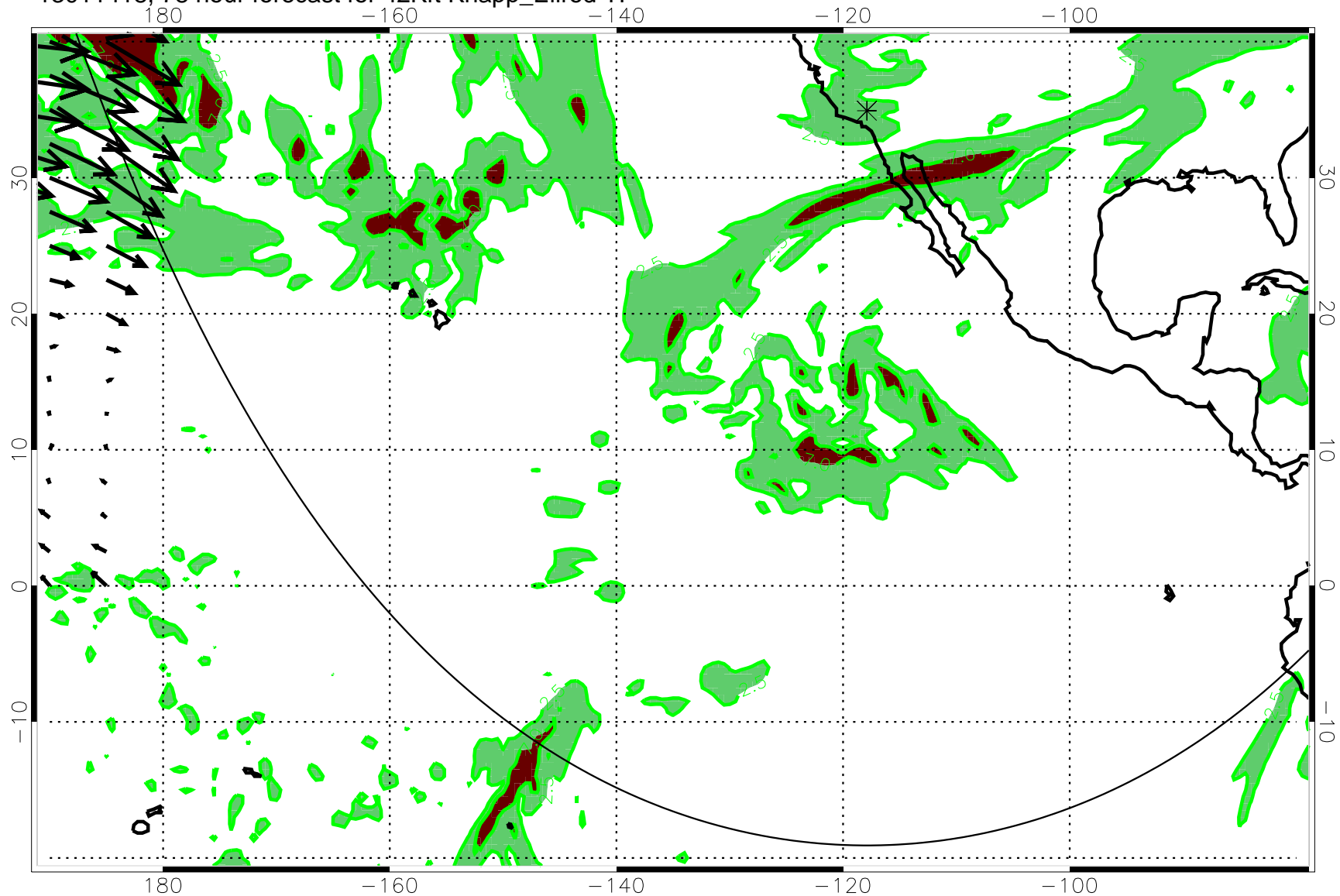
13011418, 78 hour forecast for 42Kft Knapp_Ellrod TI
