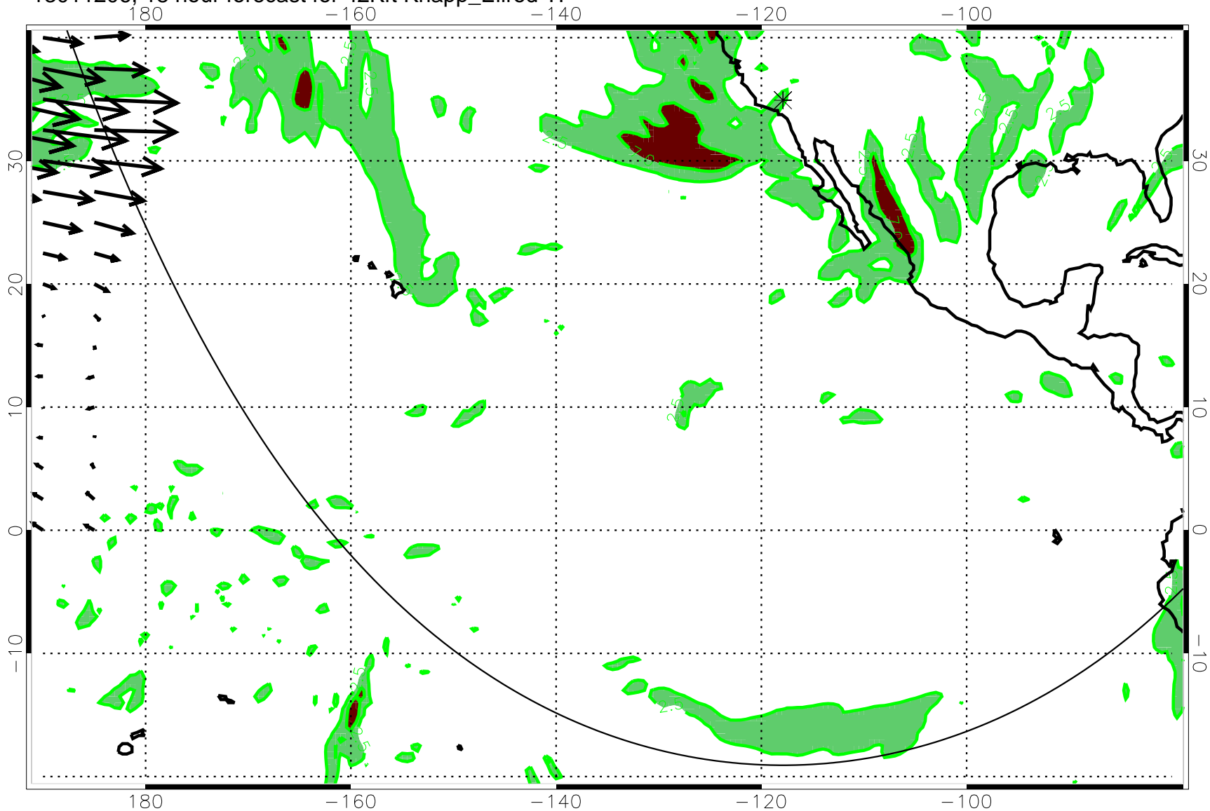
13011206, 18 hour forecast for 42Kft Knapp_Ellrod TI
