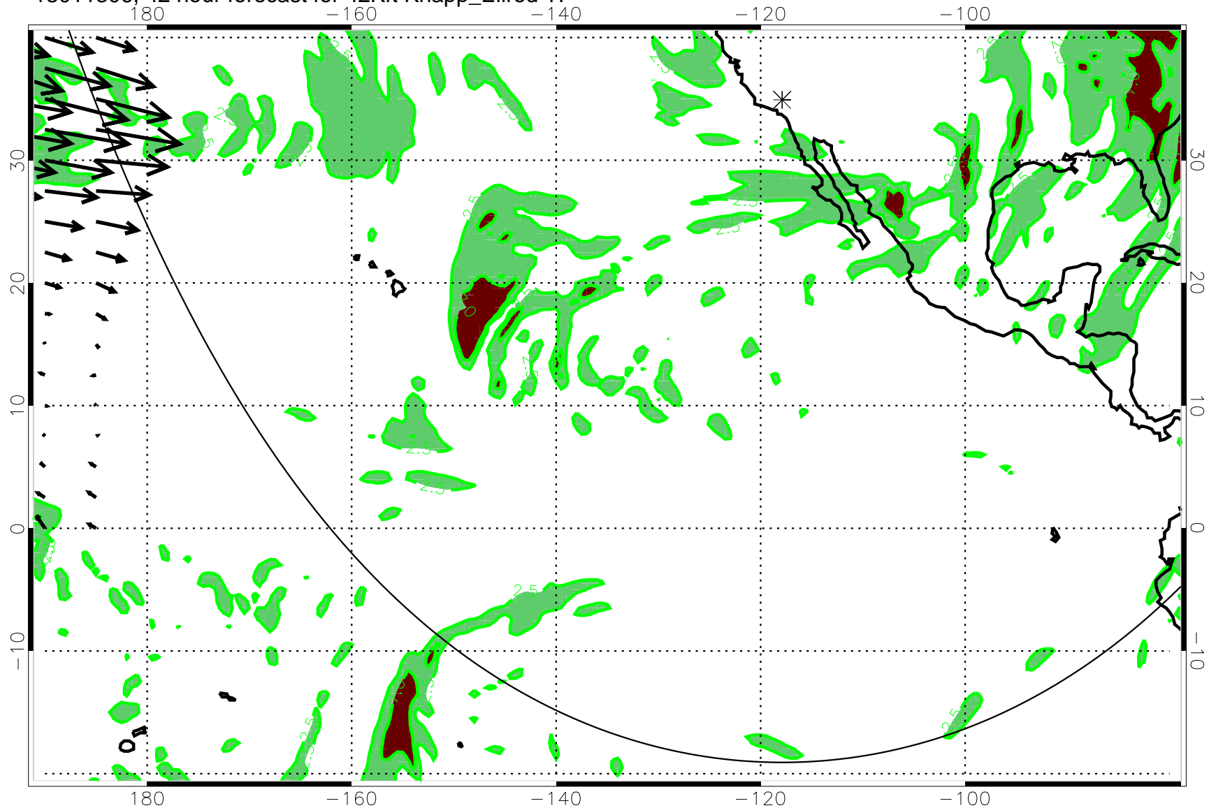
13011306, 42 hour forecast for 42Kft Knapp_Ellrod TI
