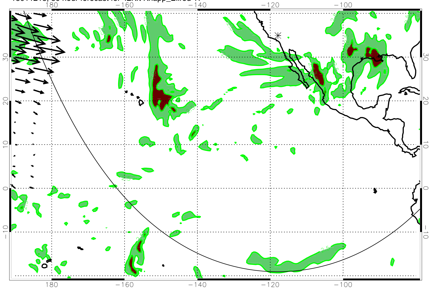
13011218, 30 hour forecast for 42Kft Knapp_Ellrod TI
