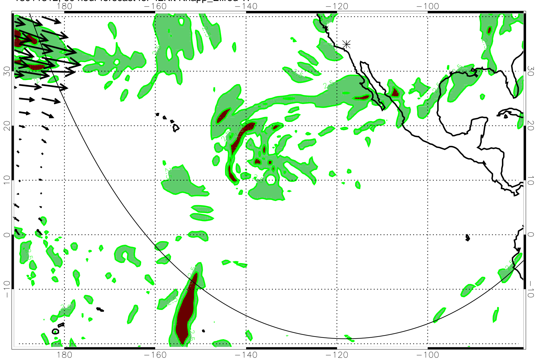
13011312, 60 hour forecast for 42Kft Knapp_Ellrod TI
