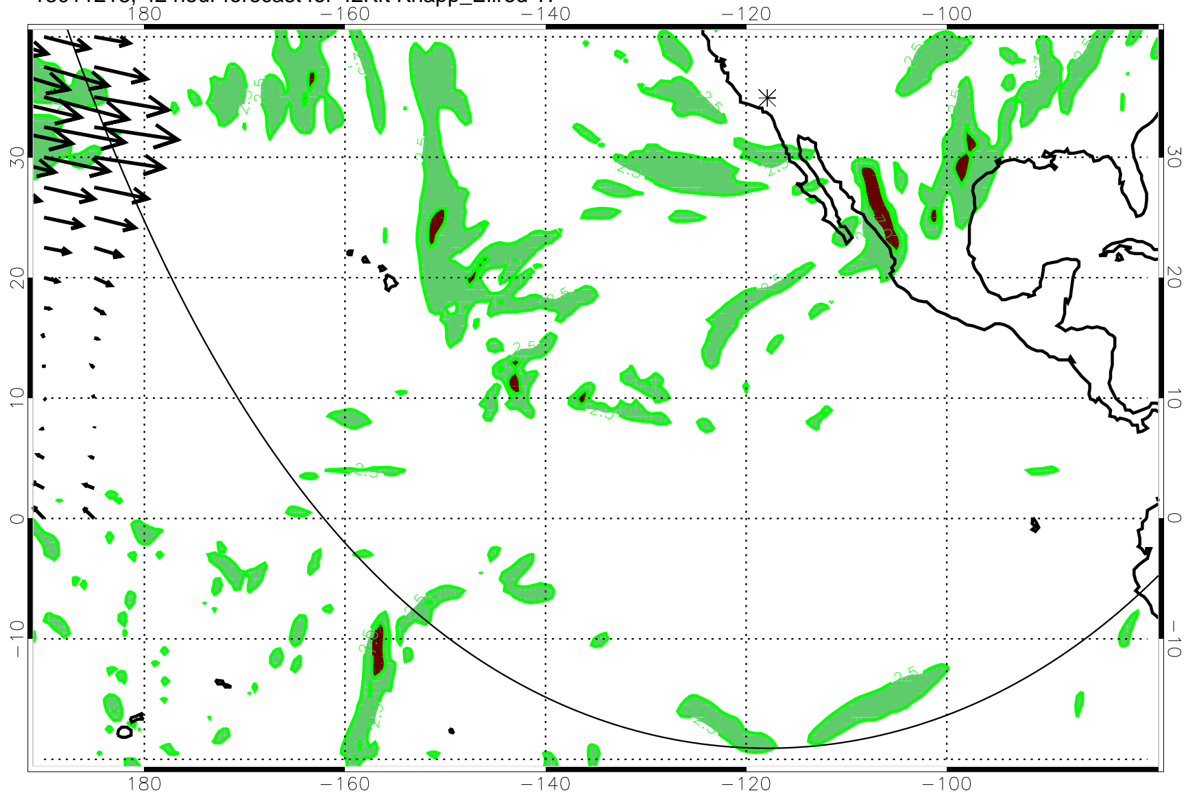
13011218, 42 hour forecast for 42Kft Knapp_Ellrod TI
