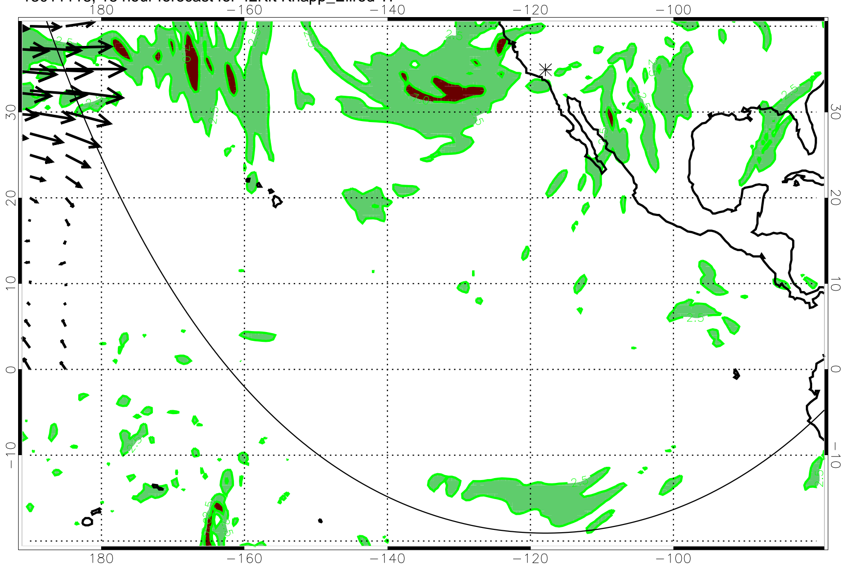
13011118, 18 hour forecast for 42Kft Knapp_Ellrod TI
