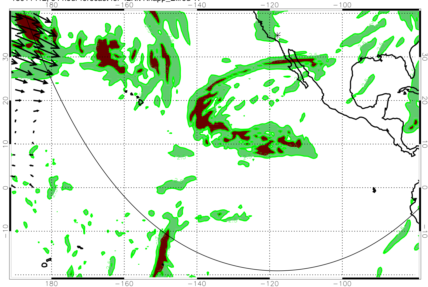
13011412, 84 hour forecast for 42Kft Knapp_Ellrod TI
