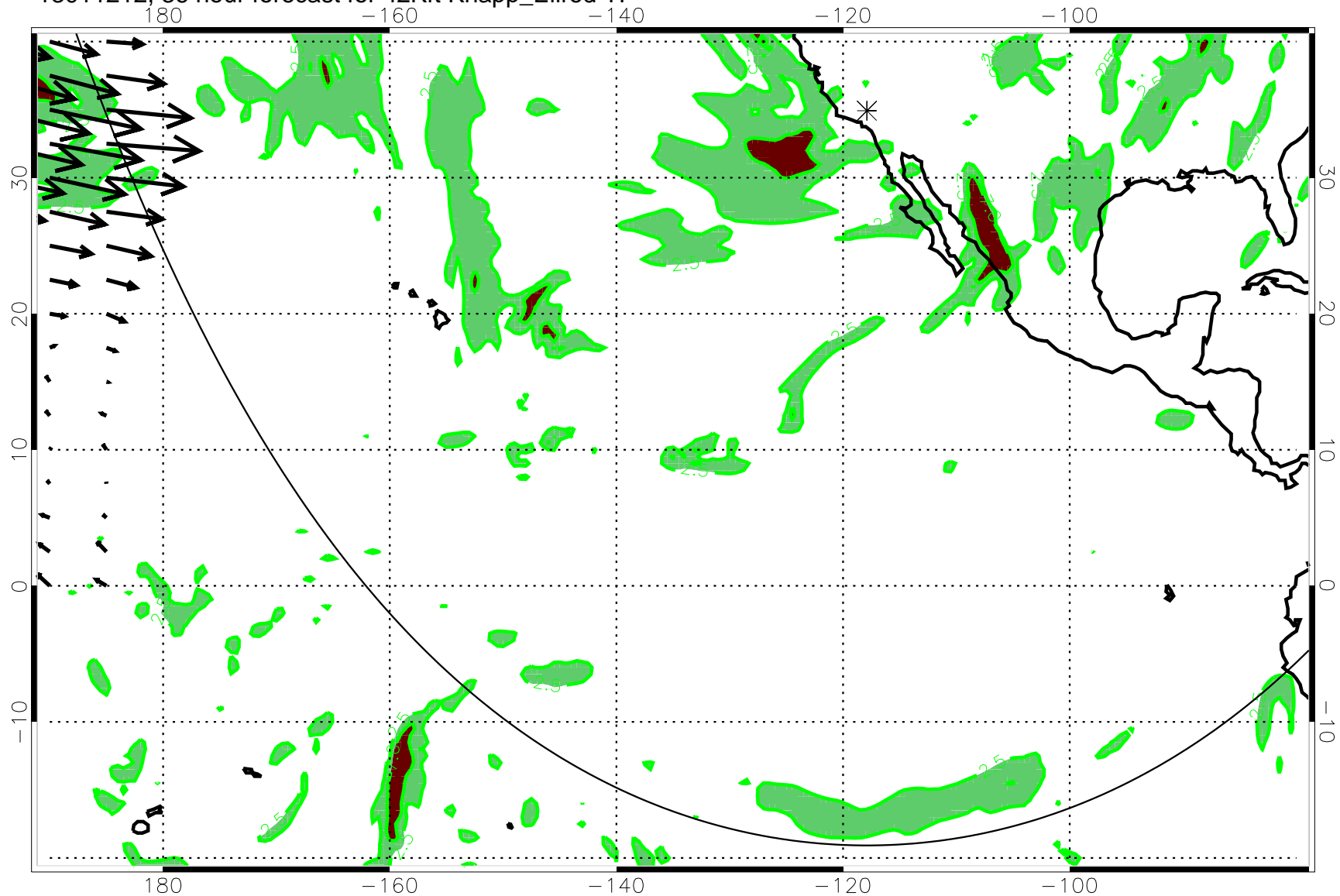
13011212, 36 hour forecast for 42Kft Knapp_Ellrod TI
