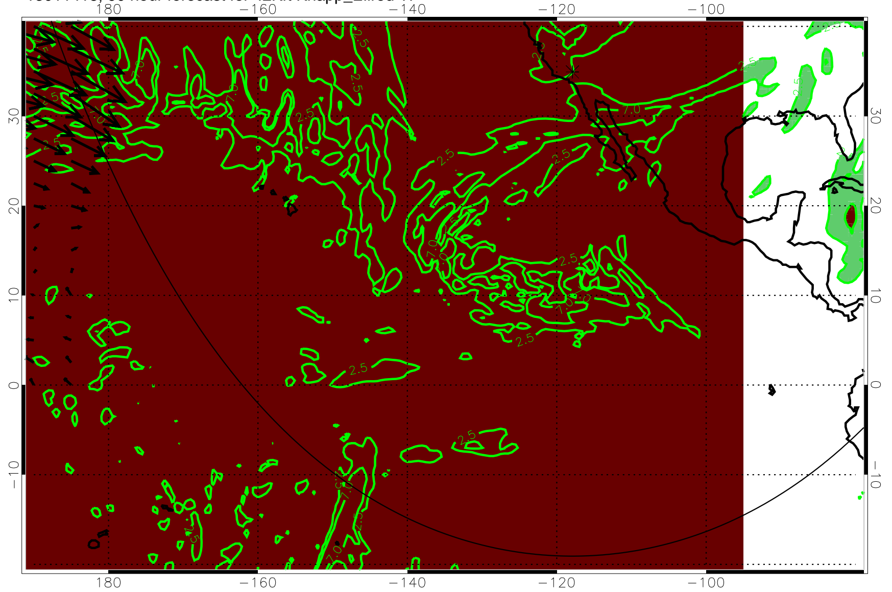
13011418, 90 hour forecast for 42Kft Knapp_Ellrod TI
