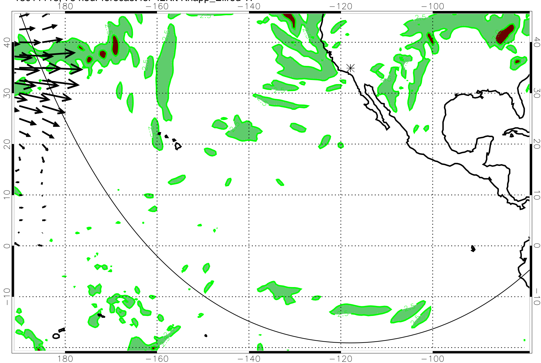
13011118, 78 hour forecast for 42Kft Knapp_Ellrod TI
