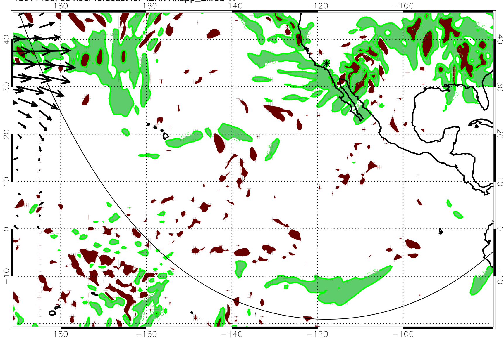
13011106, 66 hour forecast for 42Kft Knapp_Ellrod TI
