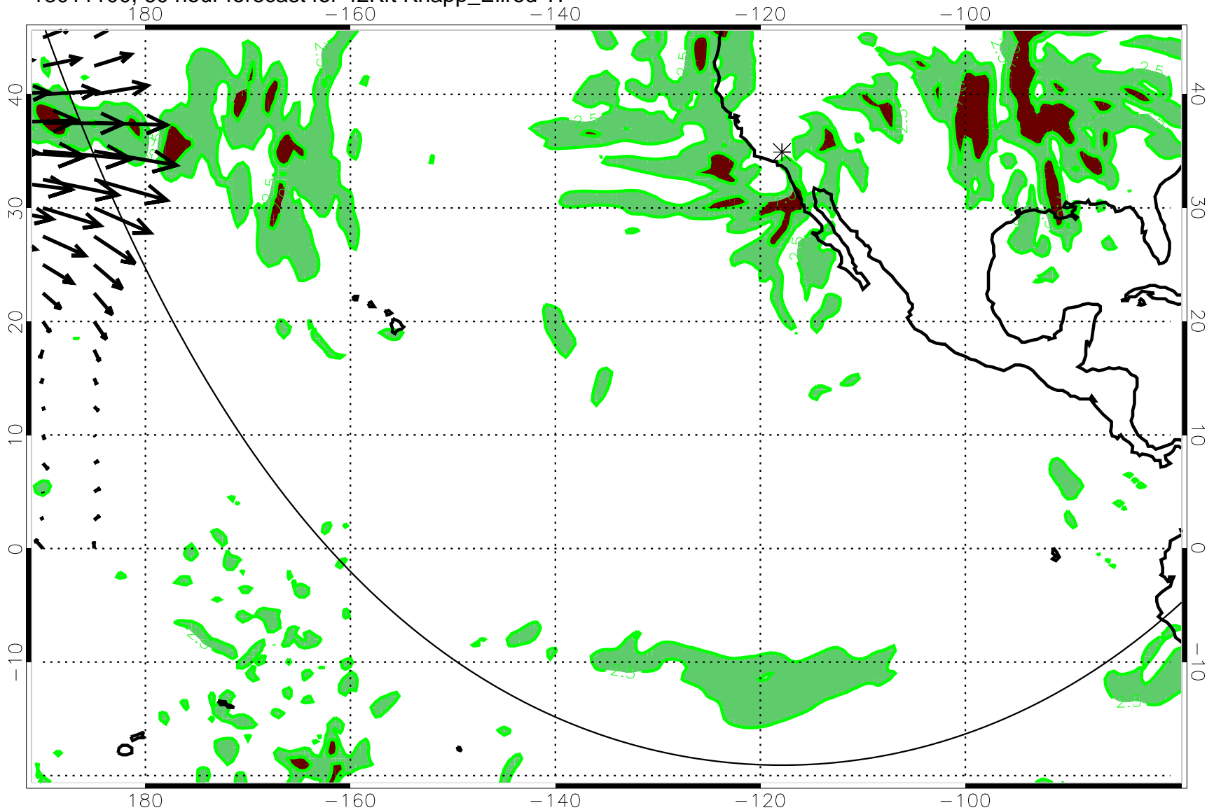
13011100, 60 hour forecast for 42Kft Knapp_Ellrod TI
