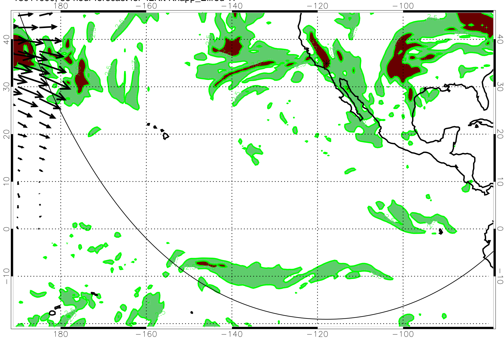
13011000, 36 hour forecast for 42Kft Knapp_Ellrod TI
