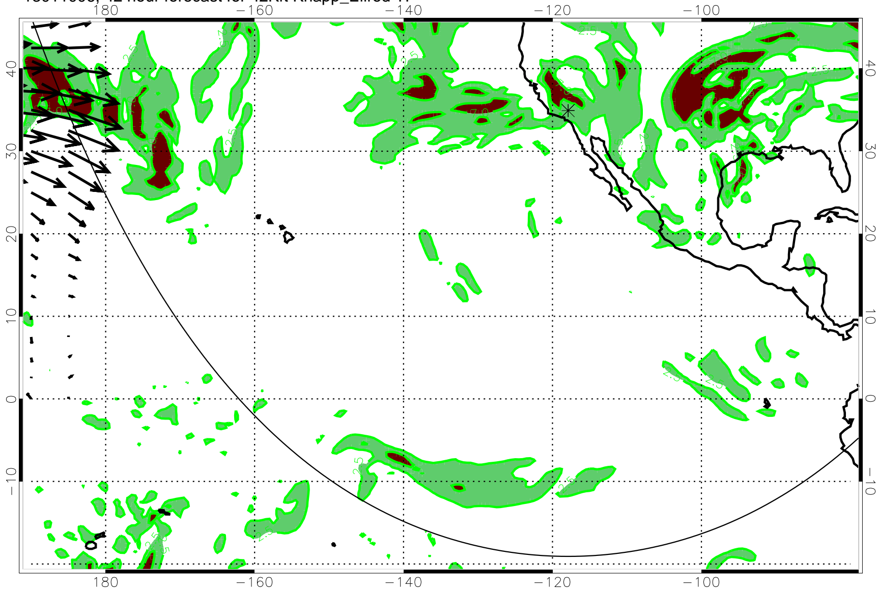
13011006, 42 hour forecast for 42Kft Knapp_Ellrod TI
