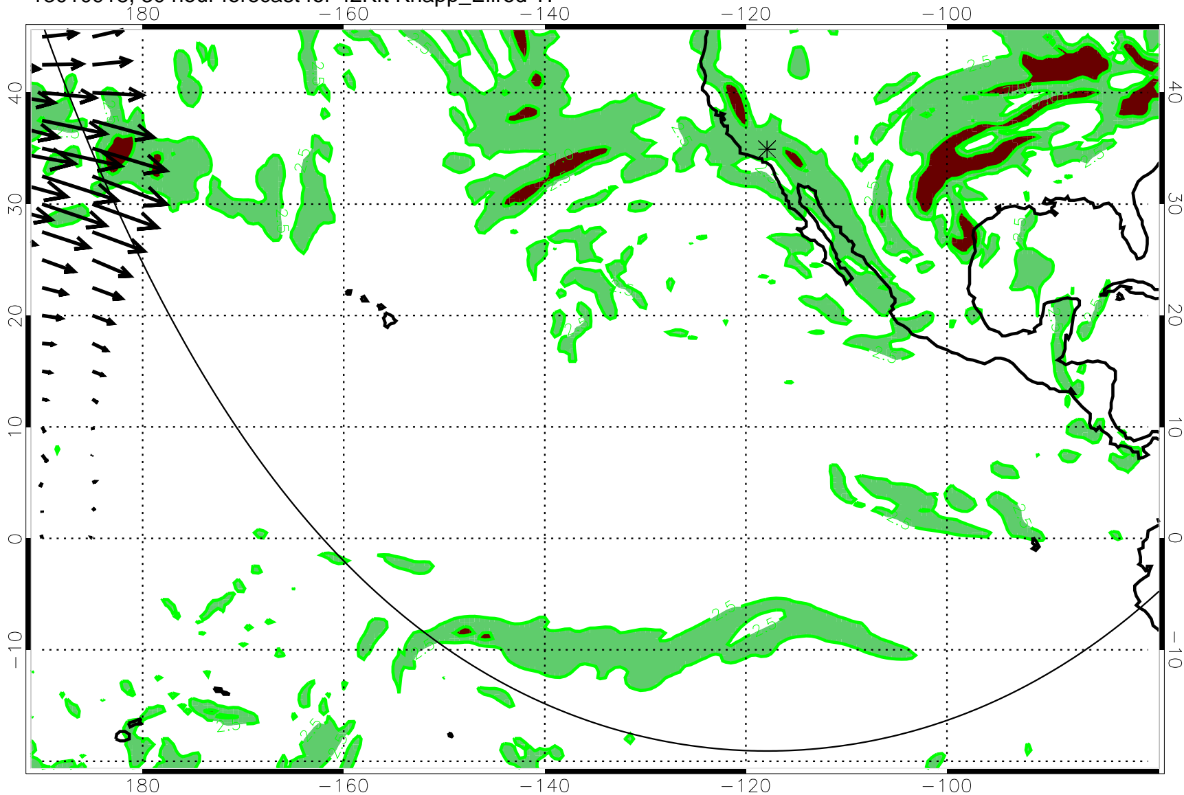
13010918, 30 hour forecast for 42Kft Knapp_Ellrod TI
