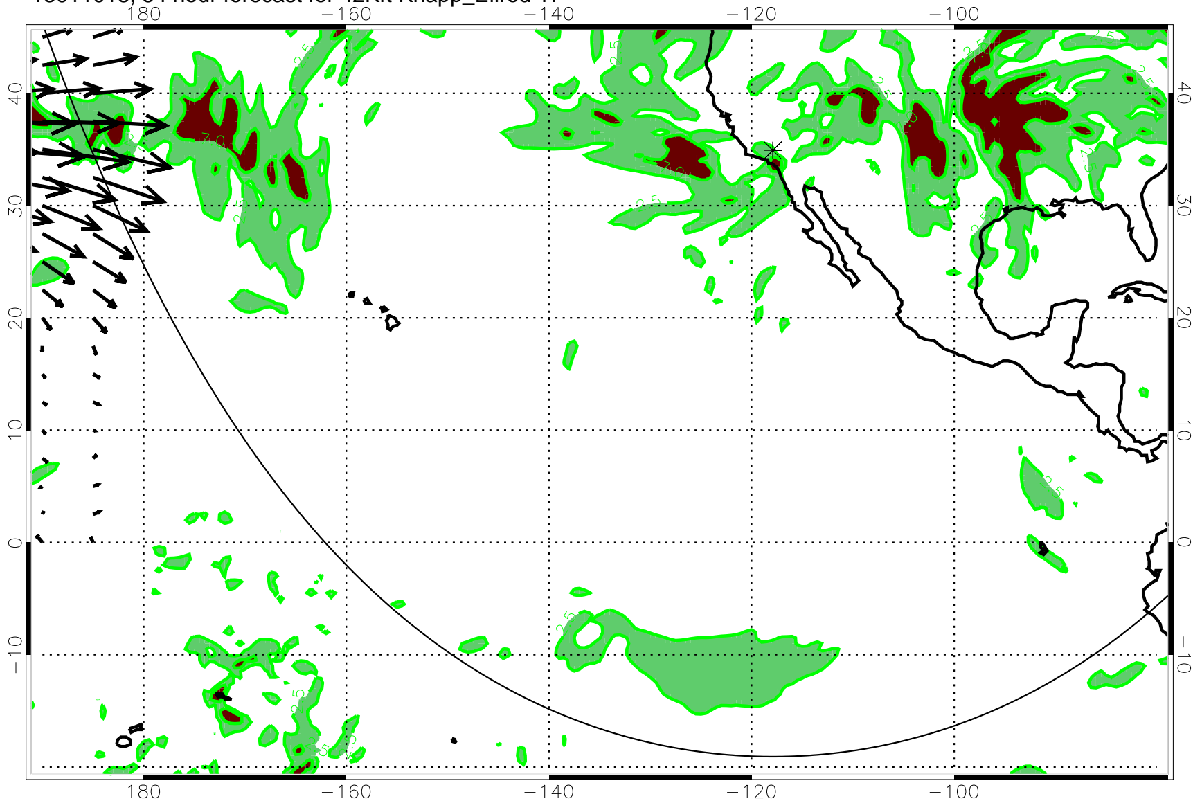
13011018, 54 hour forecast for 42Kft Knapp_Ellrod TI
