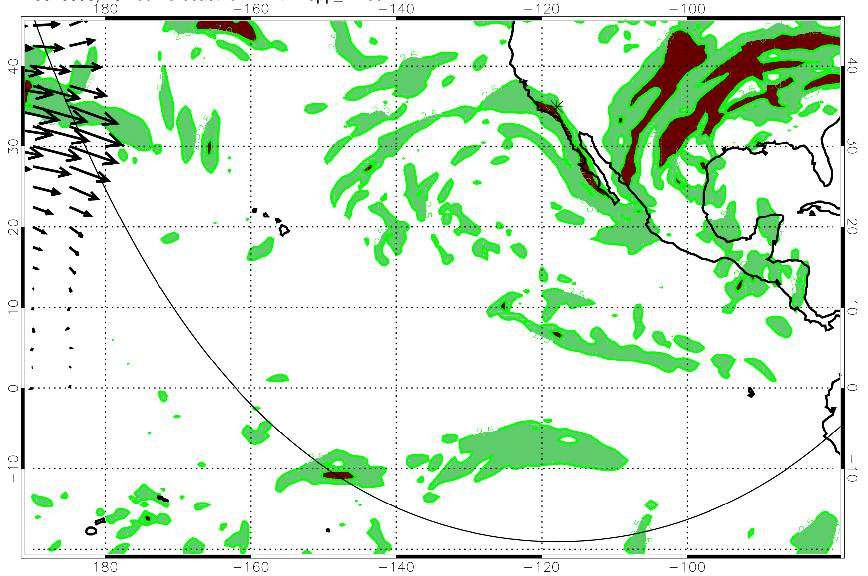
13010906, 18 hour forecast for 42Kft Knapp_Ellrod TI
