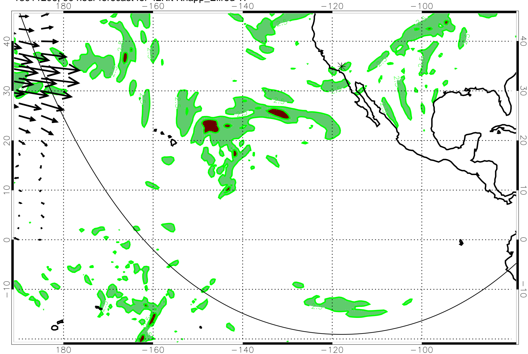
13011206, 90 hour forecast for 42Kft Knapp_Ellrod TI
