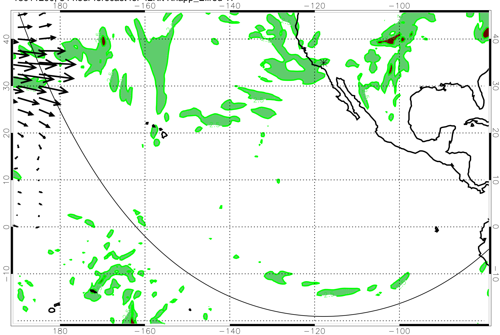
13011200, 84 hour forecast for 42Kft Knapp_Ellrod TI
