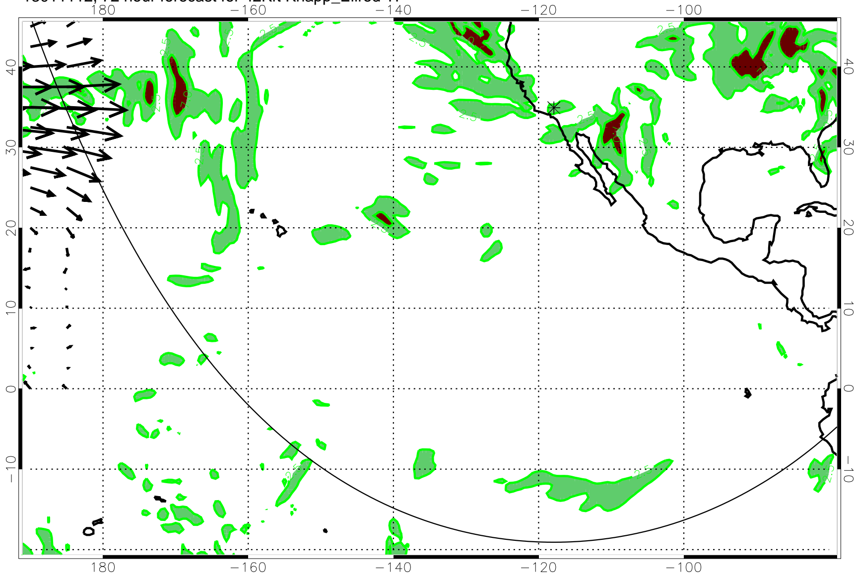
13011112, 72 hour forecast for 42Kft Knapp_Ellrod TI
