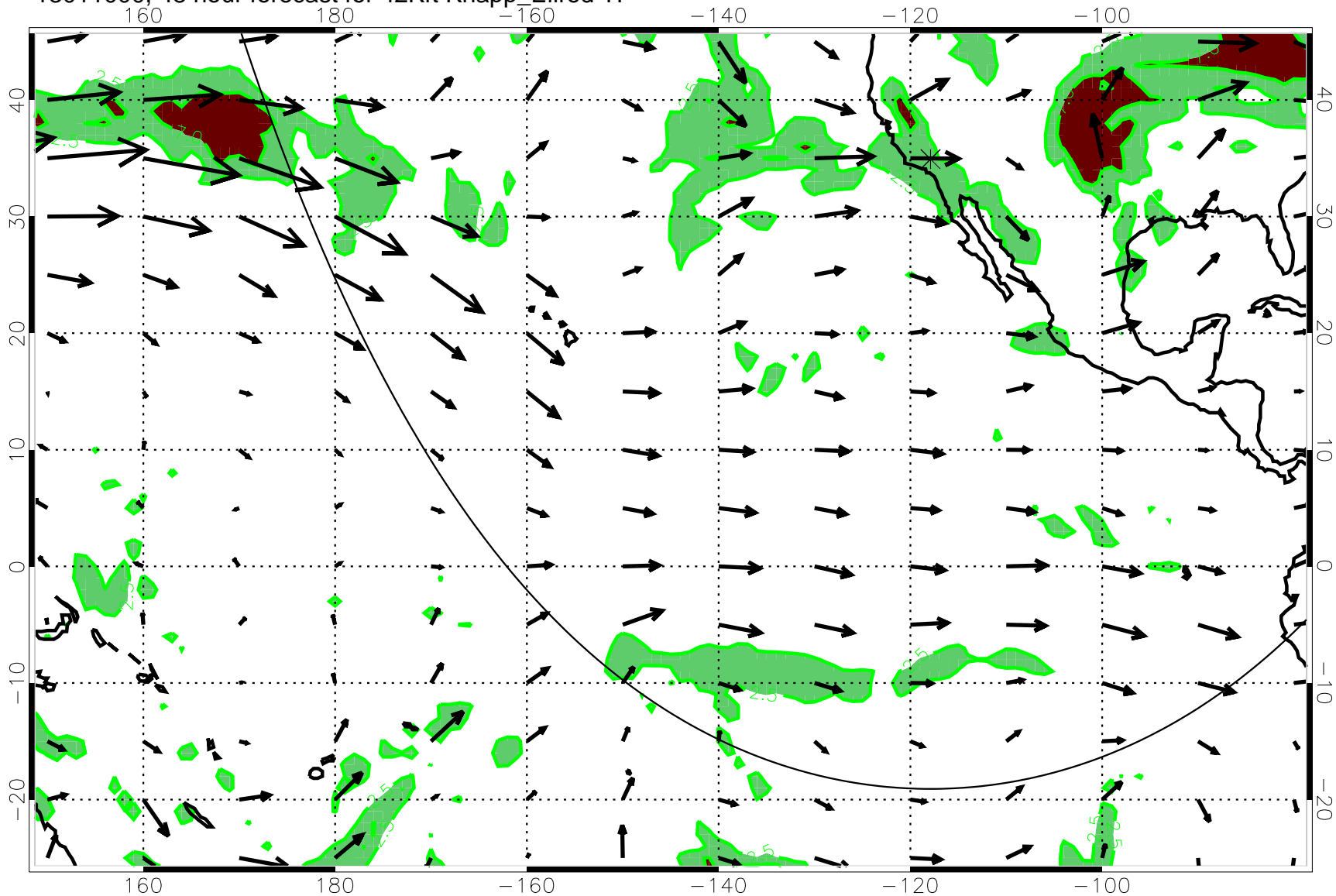
13011000, 48 hour forecast for 42Kft Knapp_Ellrod T1
