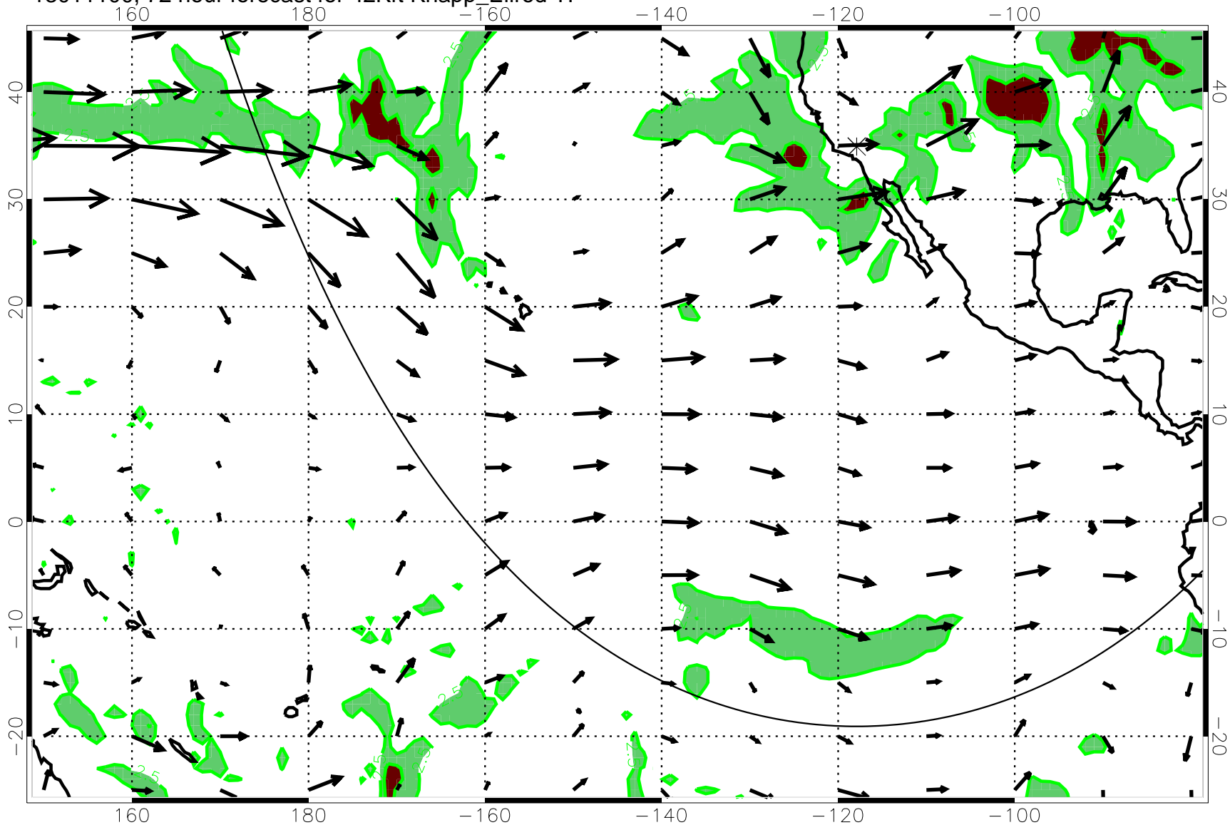
13011100, 72 hour forecast for 42Kft Knapp_Ellrod T1
