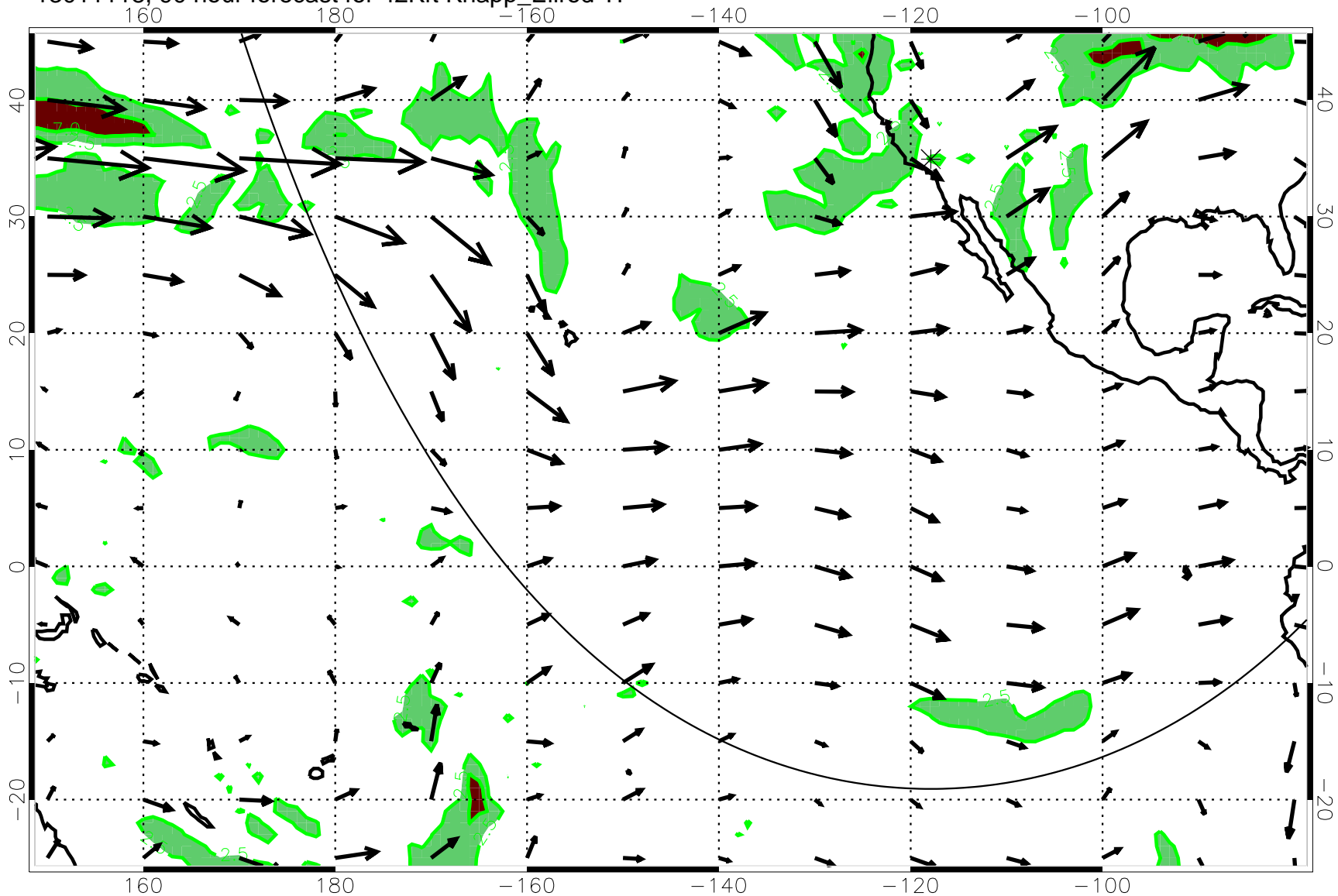
13011118, 90 hour forecast for 42Kft Knapp_Ellrod T1
