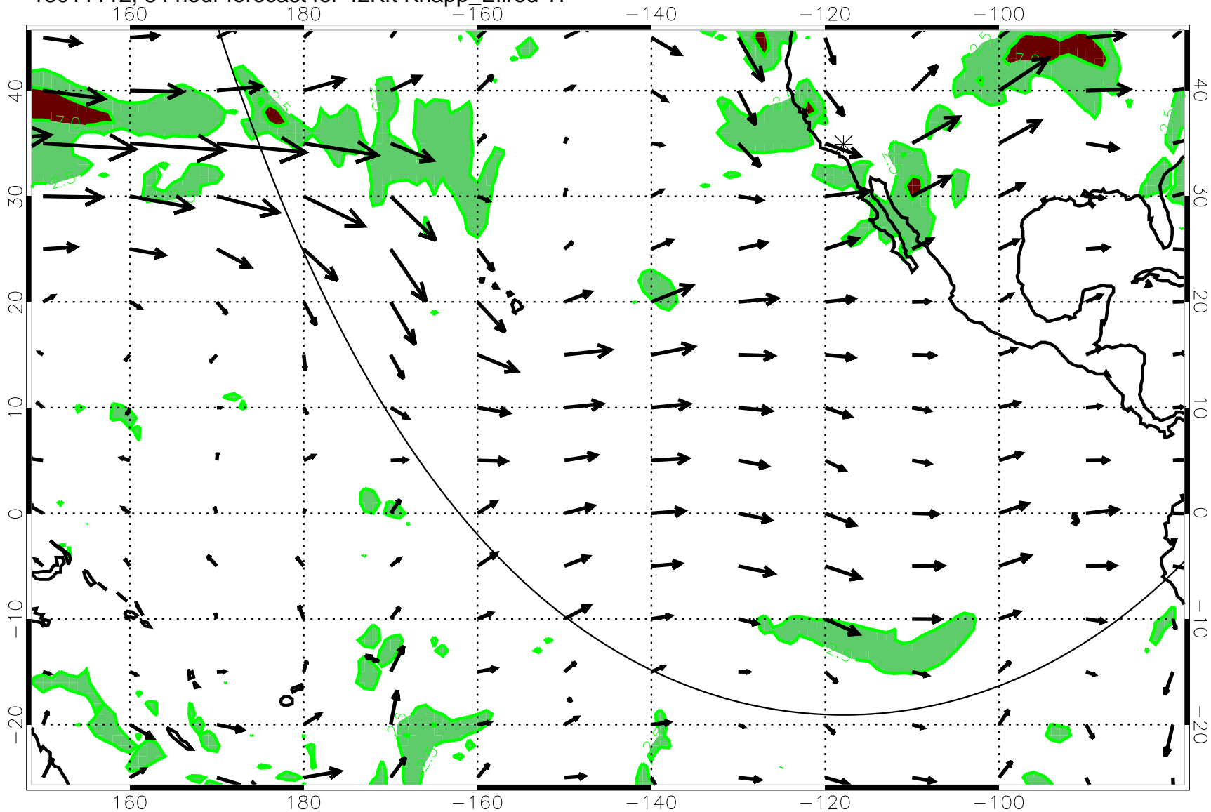
13011112, 84 hour forecast for 42Kft Knapp_Ellrod TI
