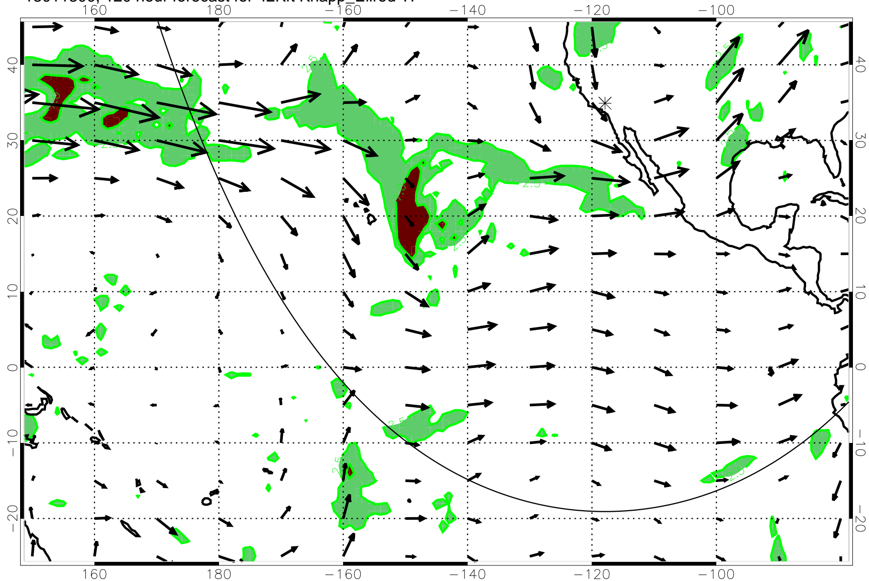
13011300, 120 hour forecast for 42Kft Knapp_Ellrod T1
