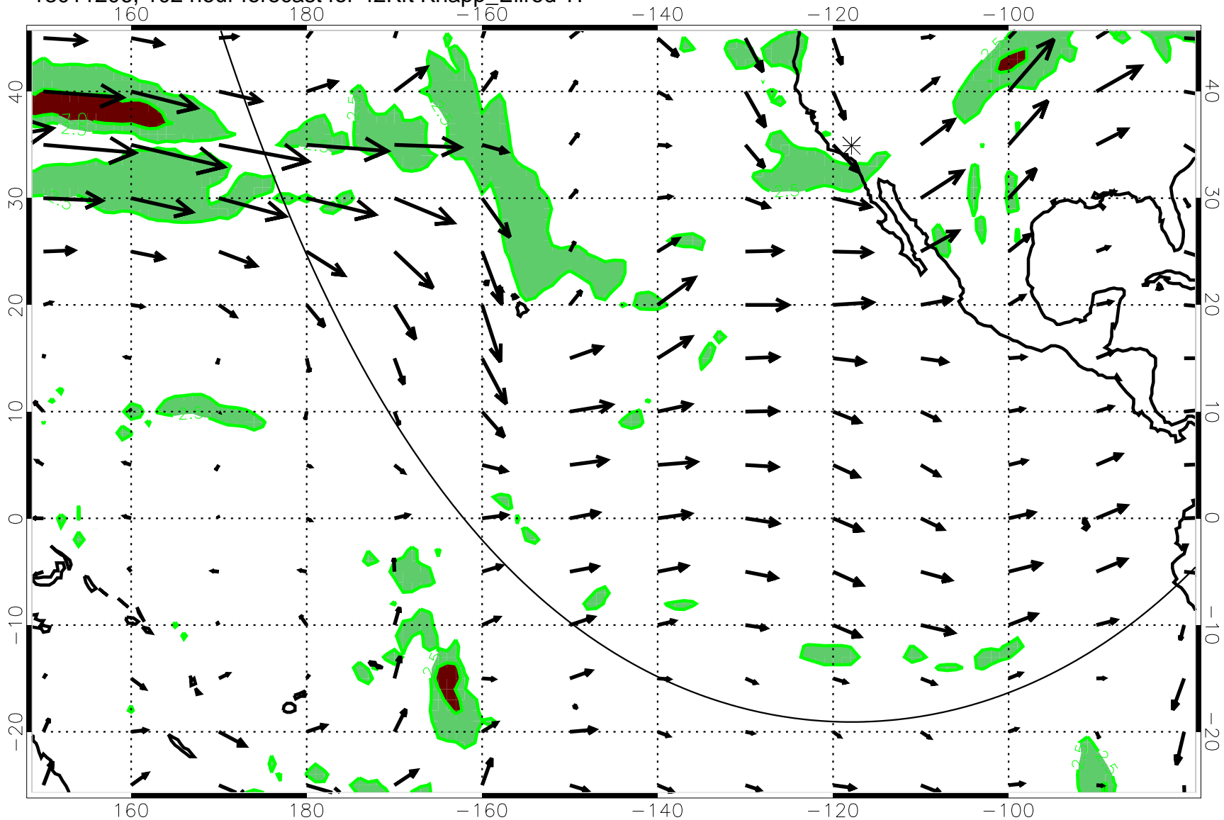
13011206, 102 hour forecast for 42Kft Knapp_Ellrod T1
