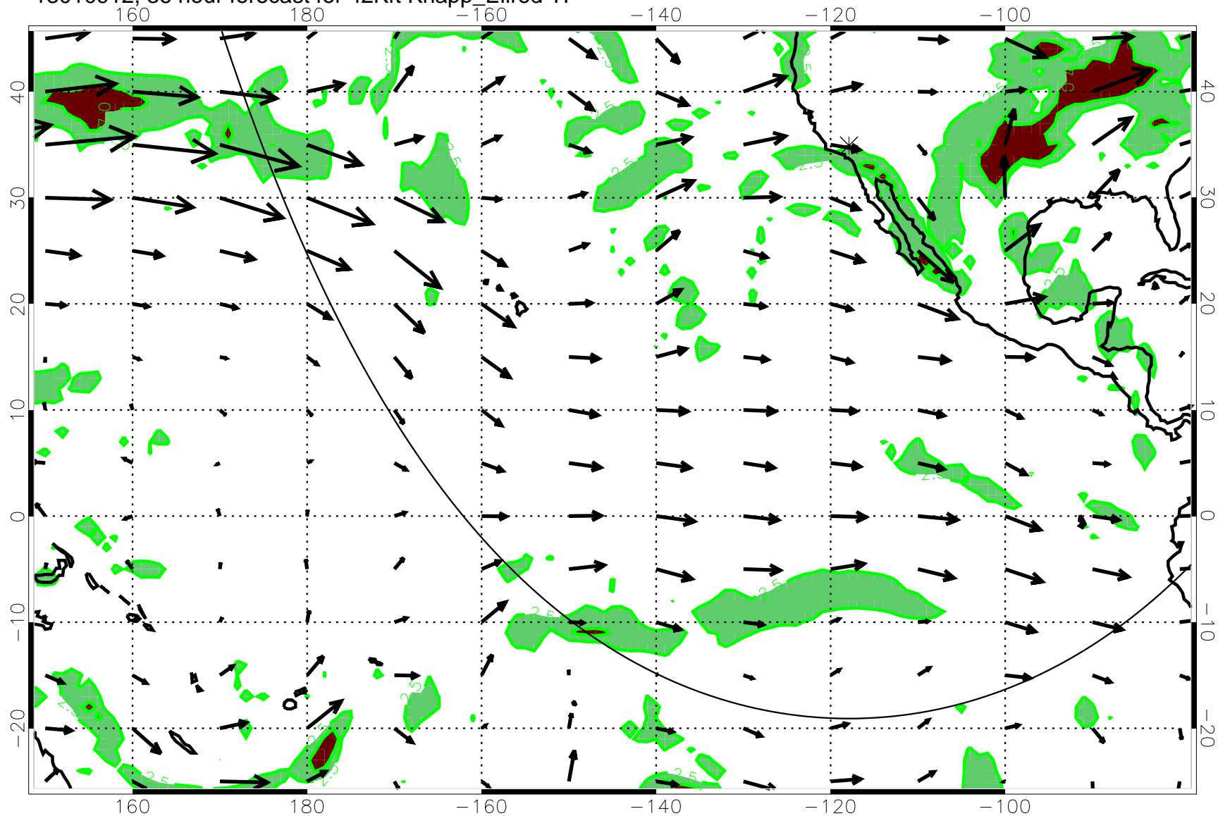
13010912, 36 hour forecast for 42Kft Knapp_Ellrod T1
