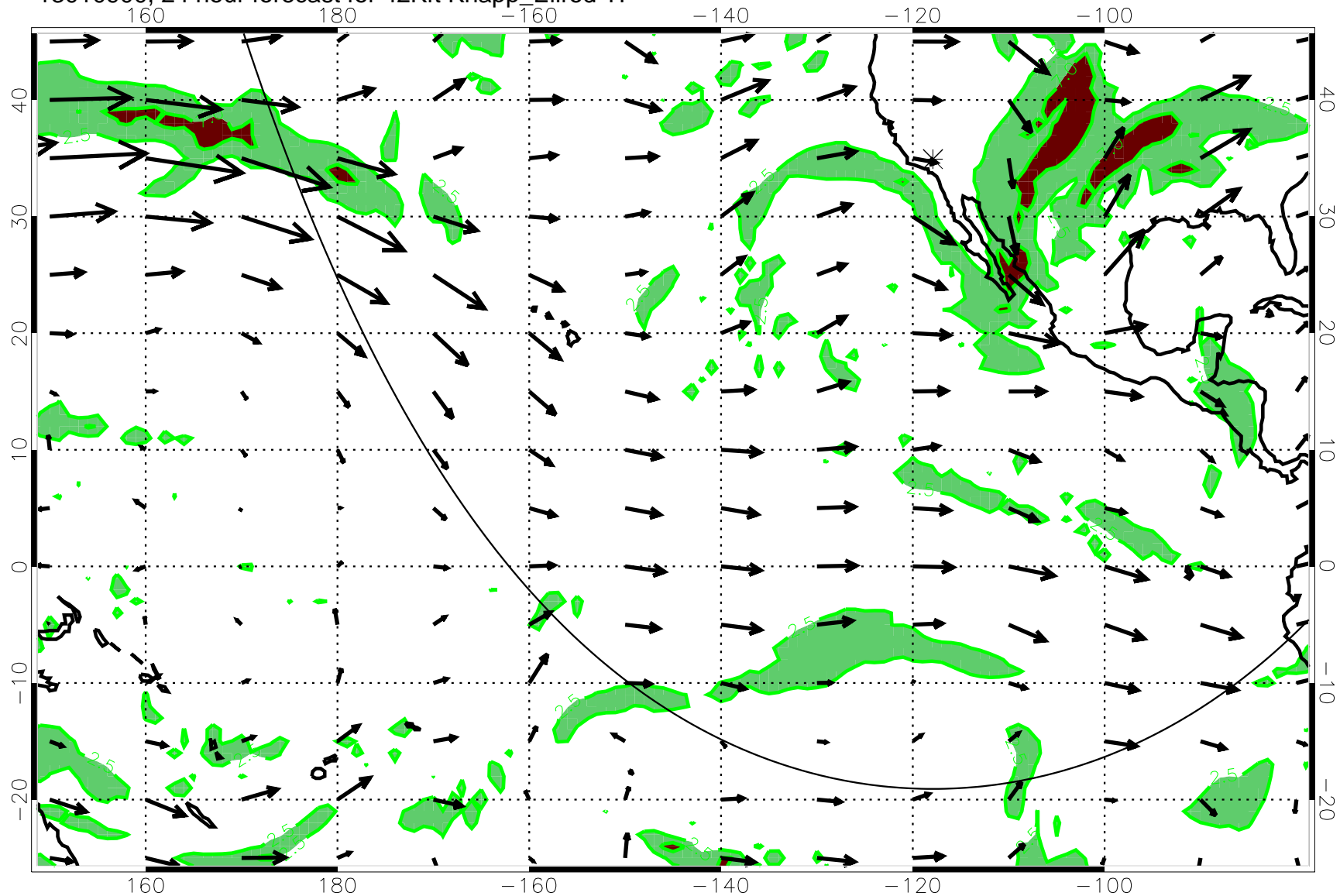
13010900, 24 hour forecast for 42Kft Knapp_Ellrod T1
