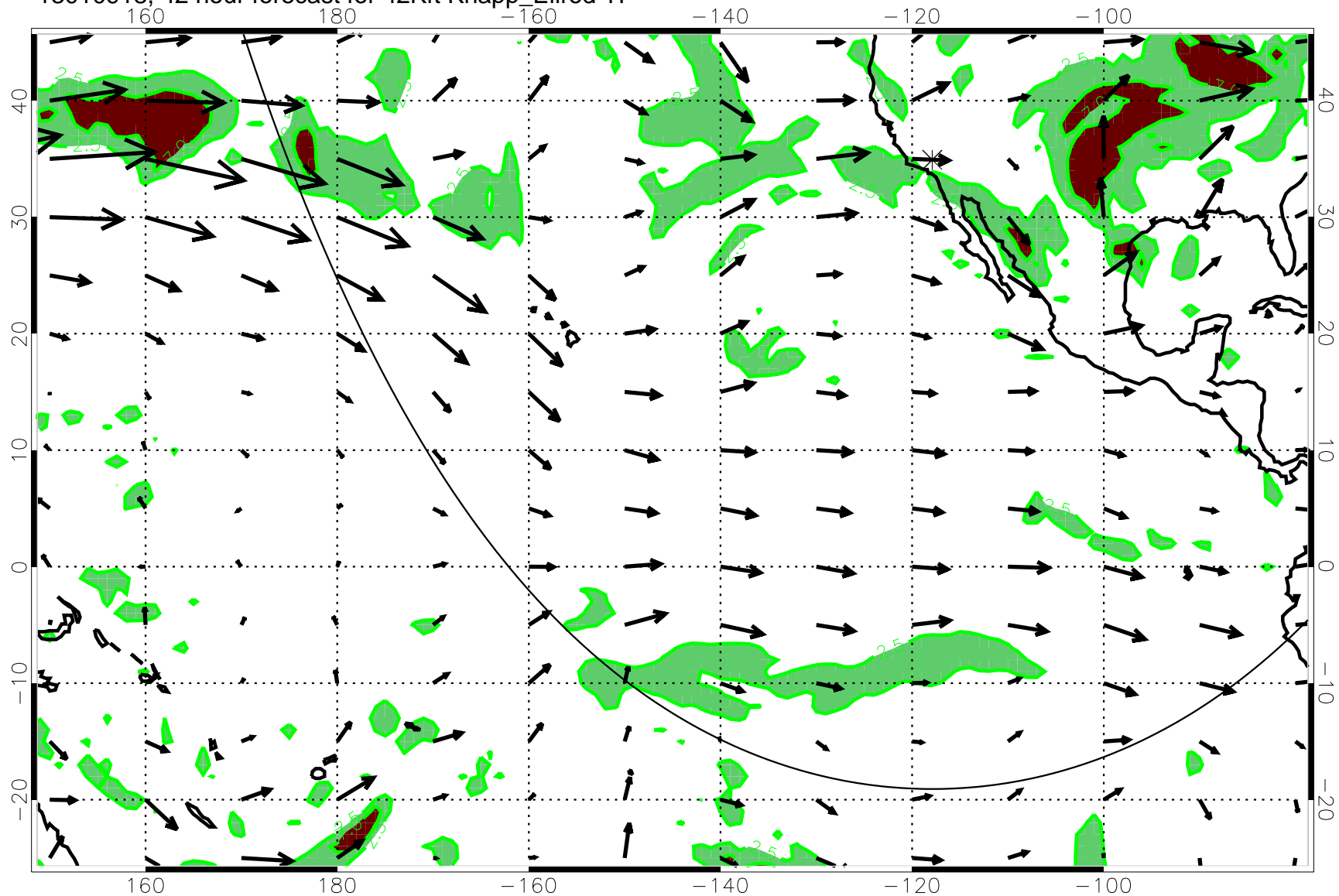
13010918, 42 hour forecast for 42Kft Knapp_Ellrod T1
