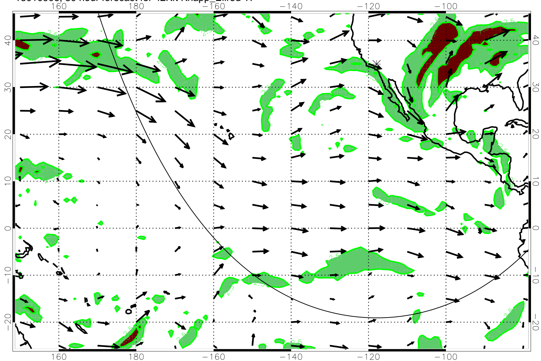
13010906, 30 hour forecast for 42Kft Knapp_Ellrod T1
