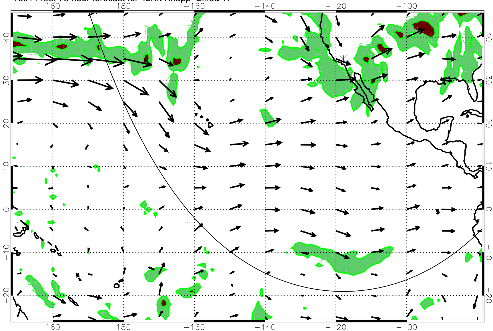
13011106, 78 hour forecast for 42Kft Knapp_Ellrod T1
