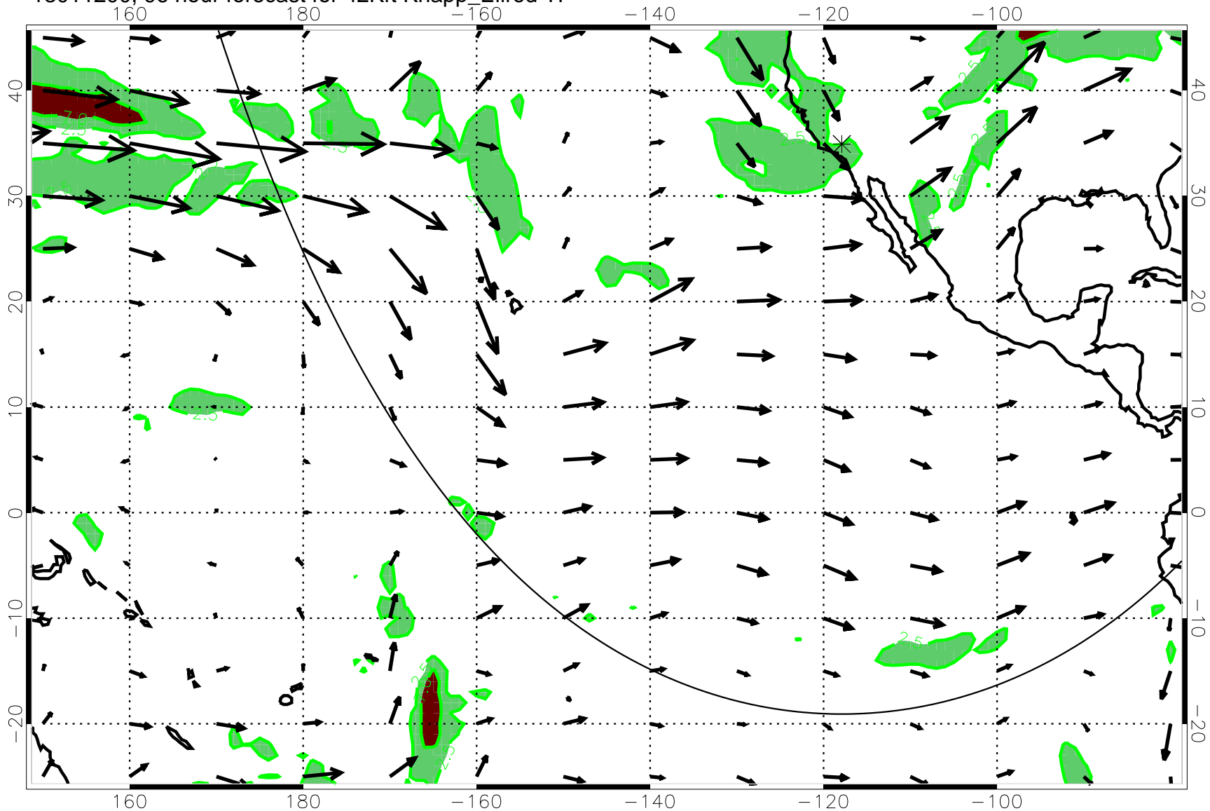
13011200, 96 hour forecast for 42Kft Knapp_Ellrod T1
