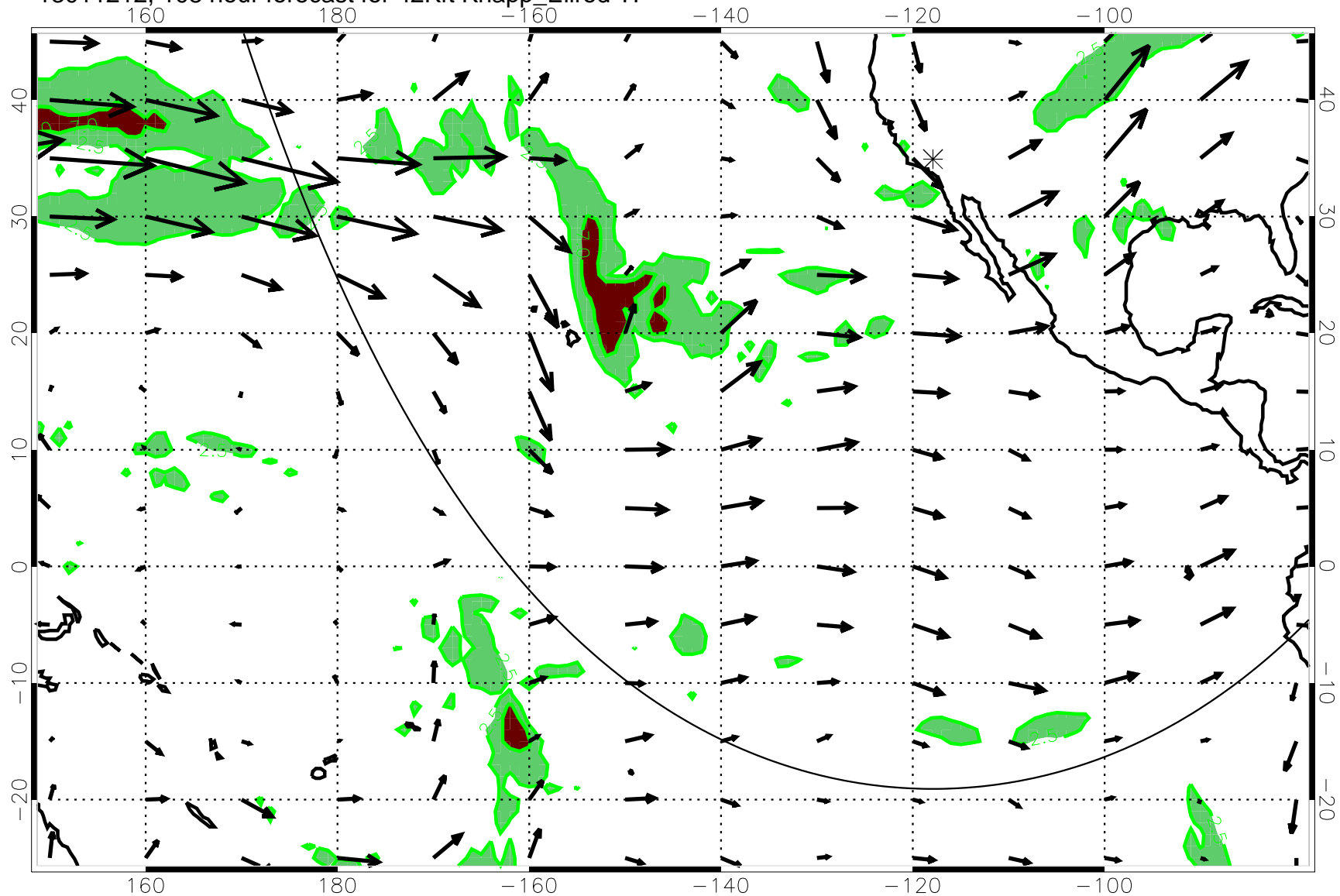
13011212, 108 hour forecast for 42Kft Knapp_Ellrod T1
