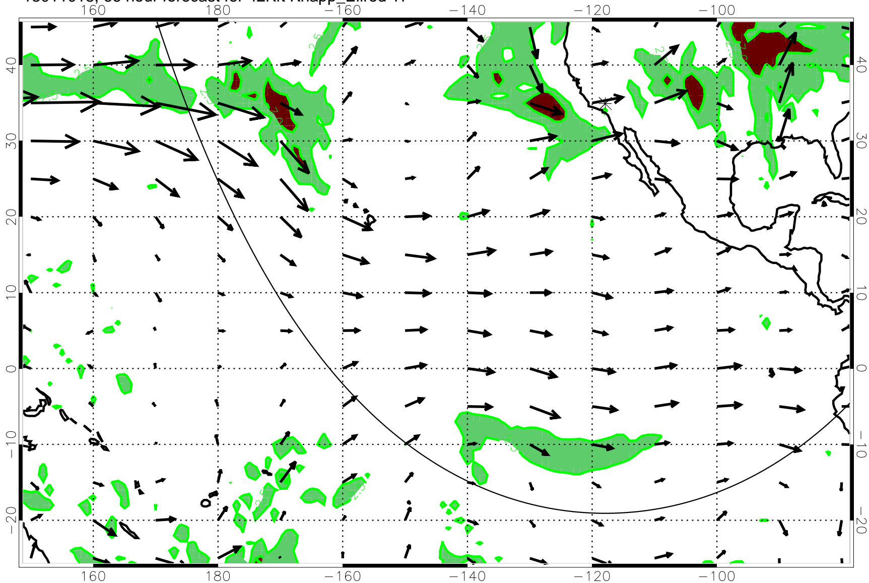
13011018, 66 hour forecast for 42Kft Knapp_Ellrod T1
