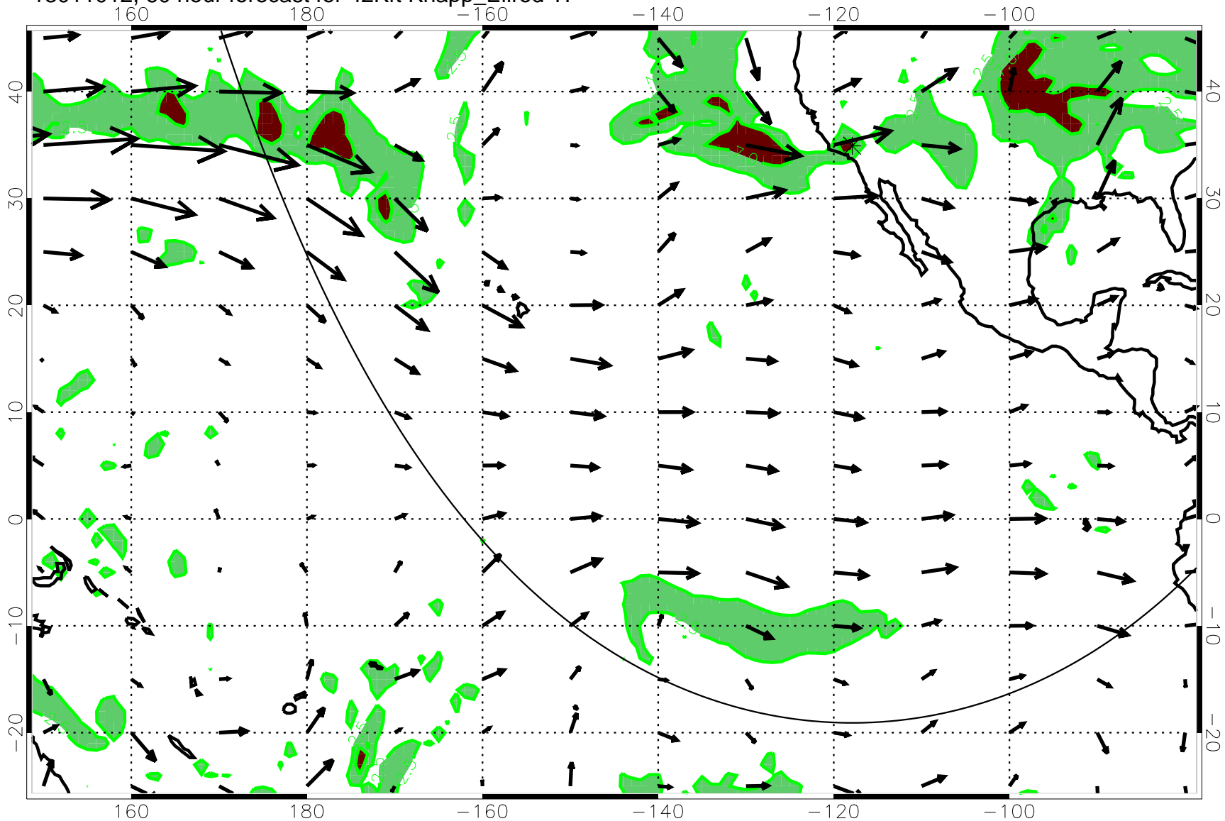
13011012, 60 hour forecast for 42Kft Knapp_Ellrod T1
