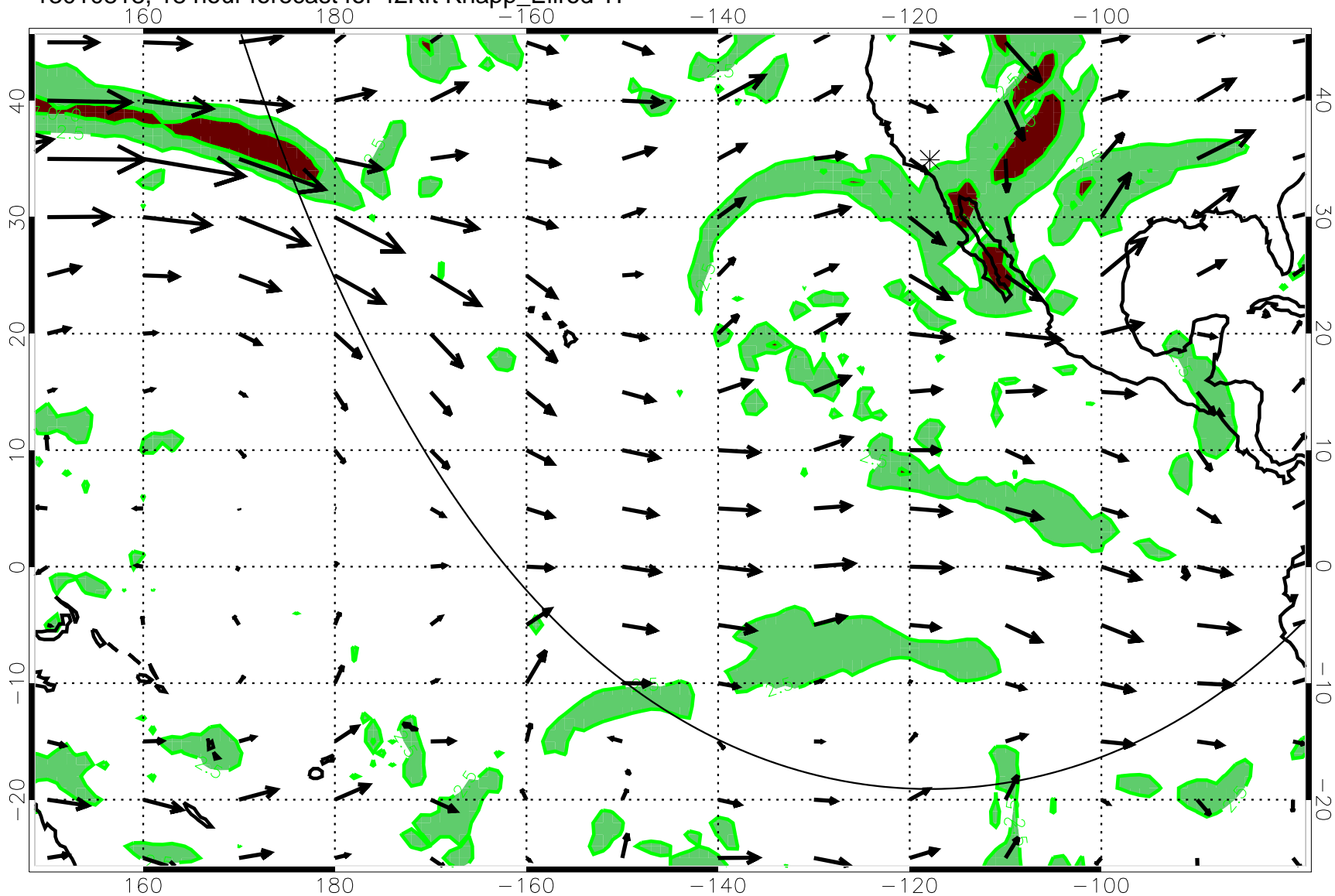
13010818, 18 hour forecast for 42Kft Knapp_Ellrod T1
