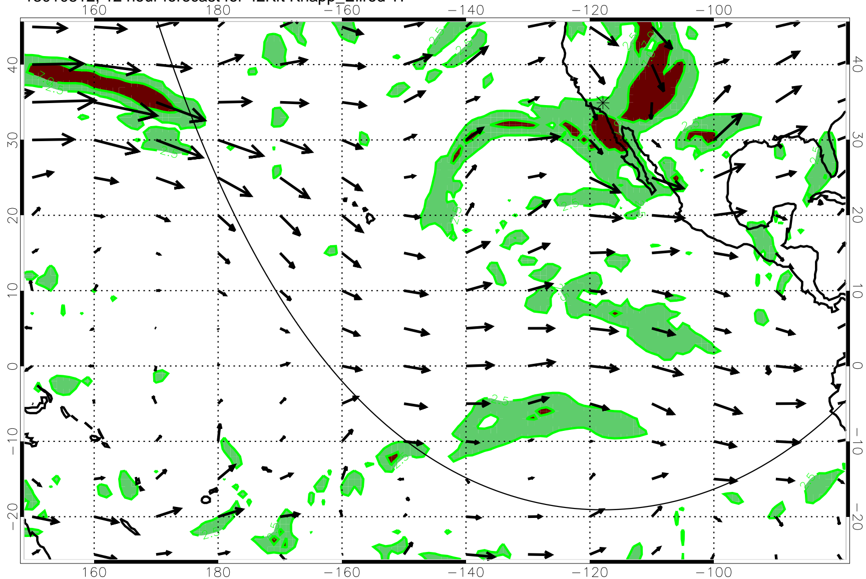
13010812, 12 hour forecast for 42Kft Knapp_Ellrod T1
