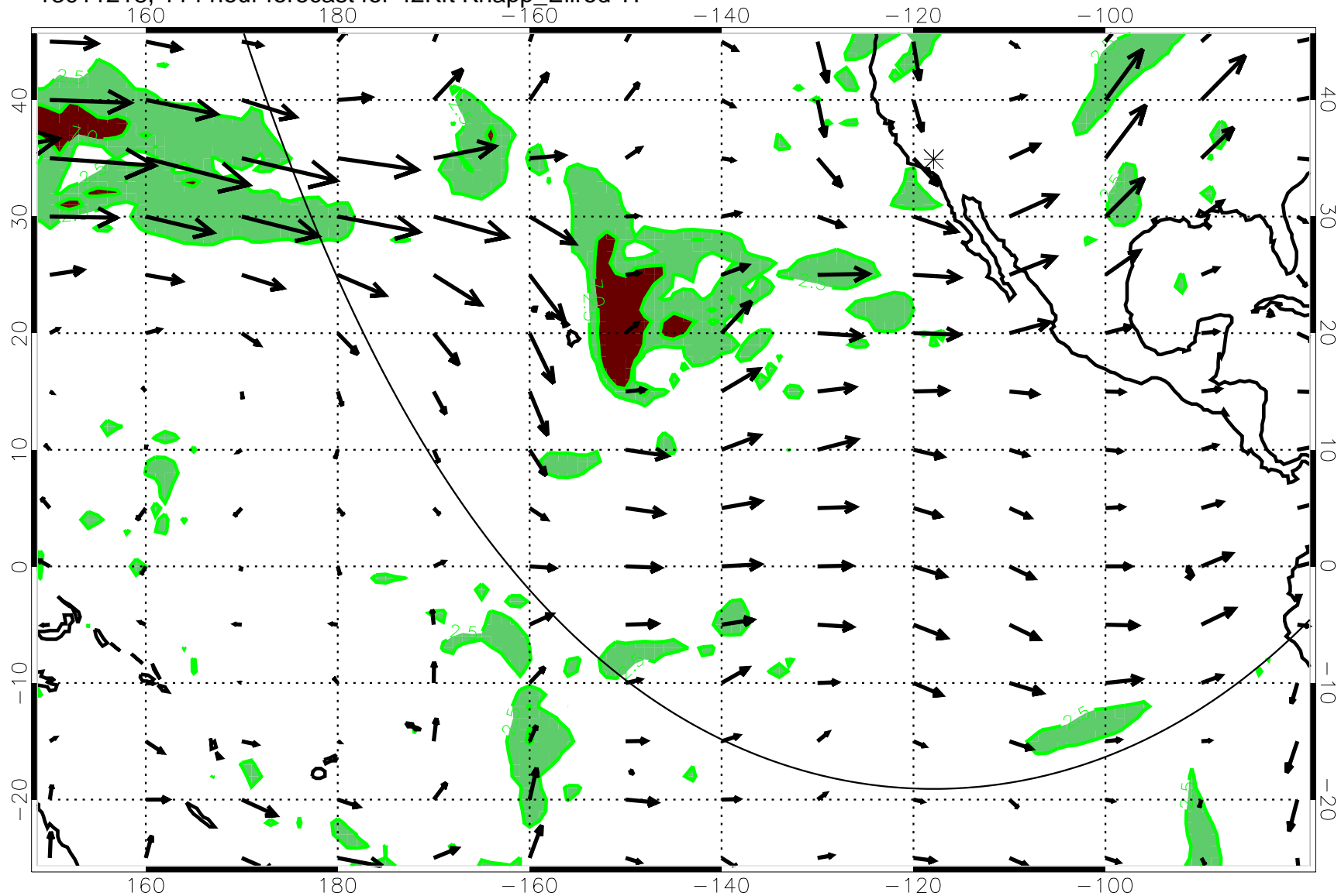
13011218, 114 hour forecast for 42Kft Knapp_Ellrod T1
