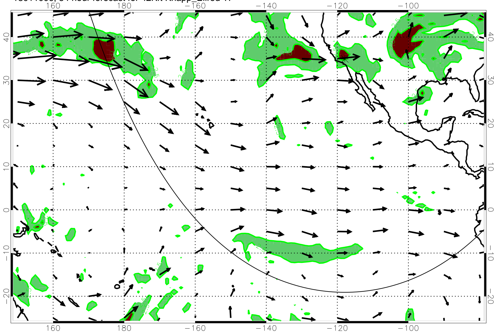
13011006, 54 hour forecast for 42Kft Knapp_Ellrod T1
