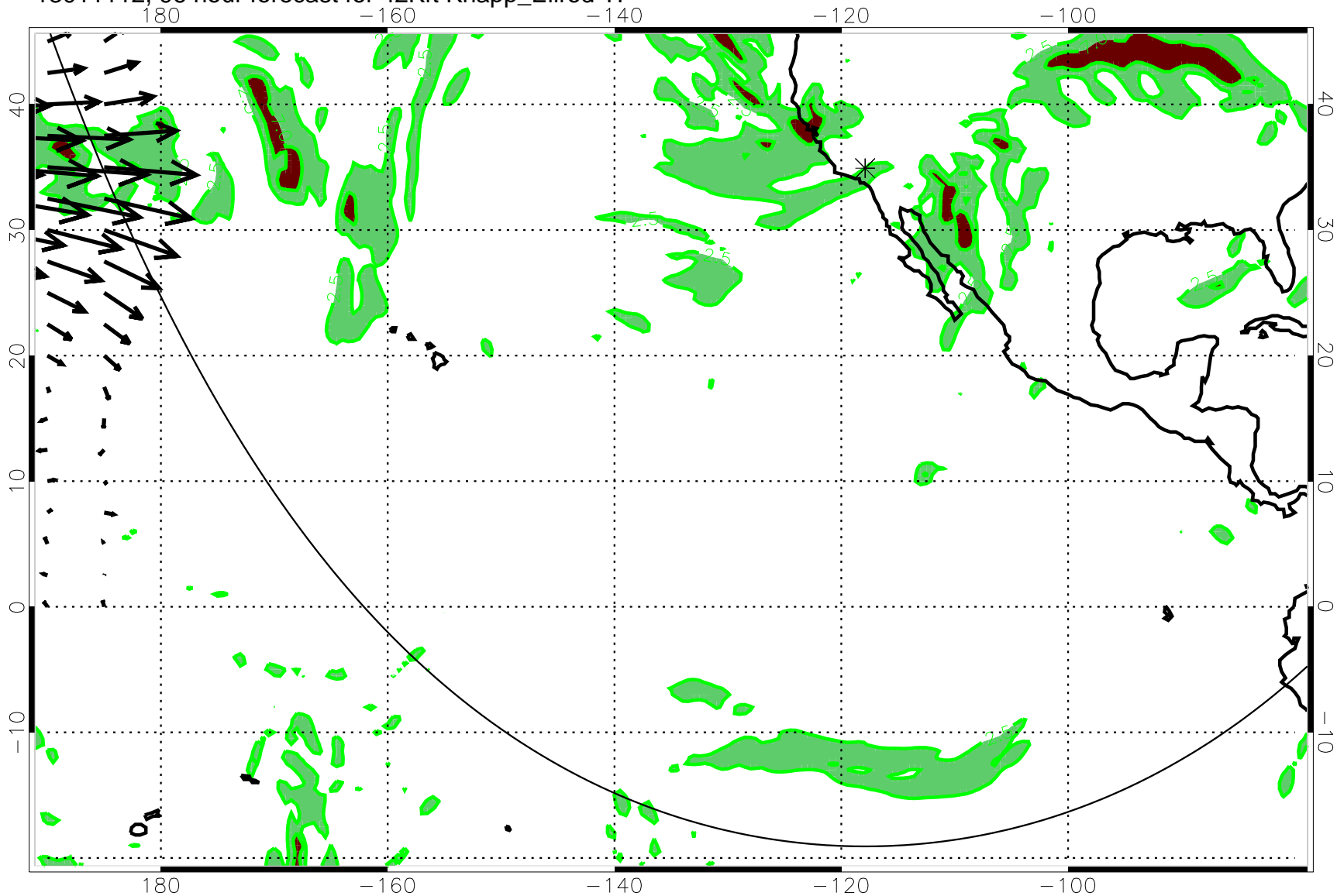
13011112, 96 hour forecast for 42Kft Knapp_Ellrod TI
