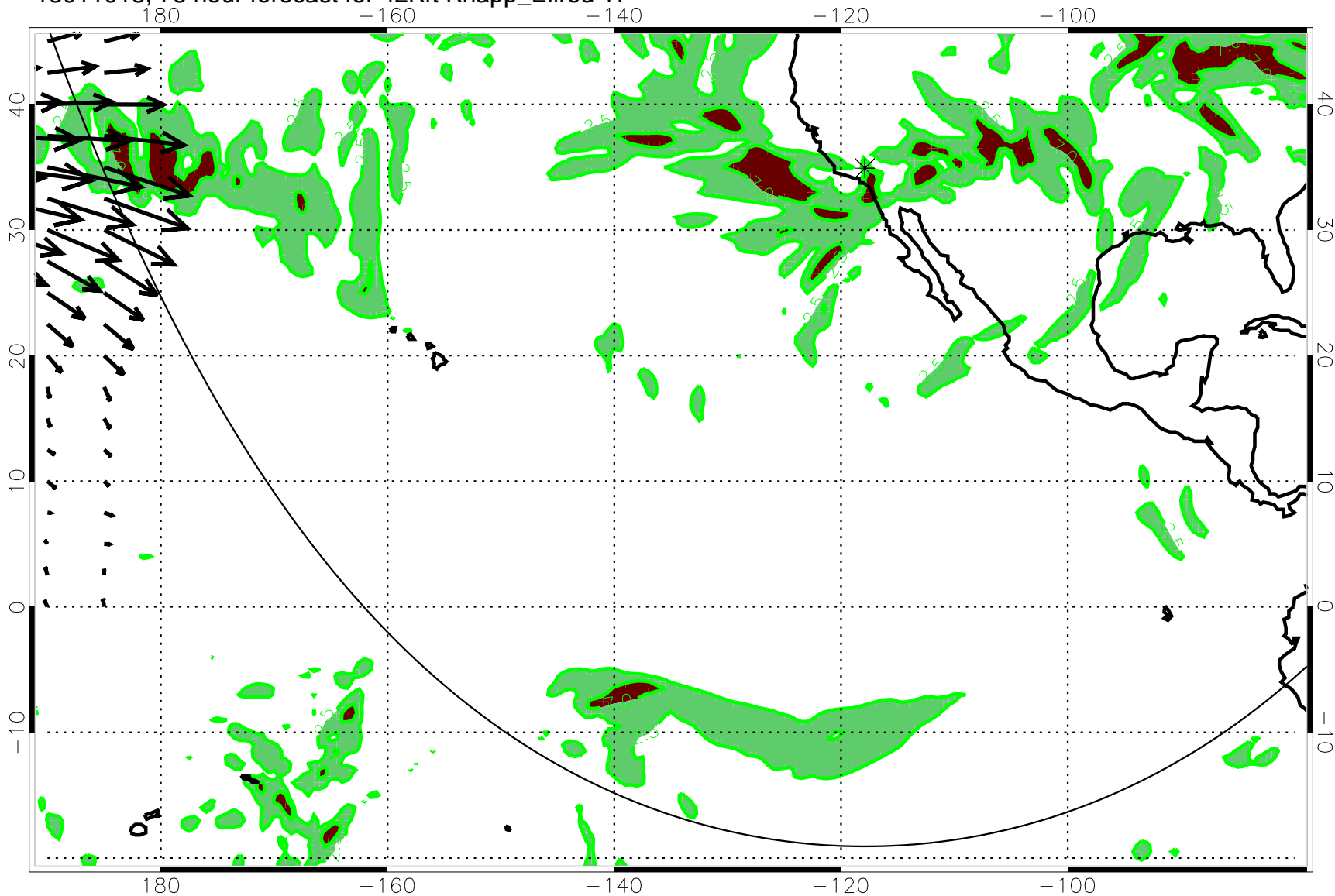
13011018, 78 hour forecast for 42Kft Knapp_Ellrod TI
