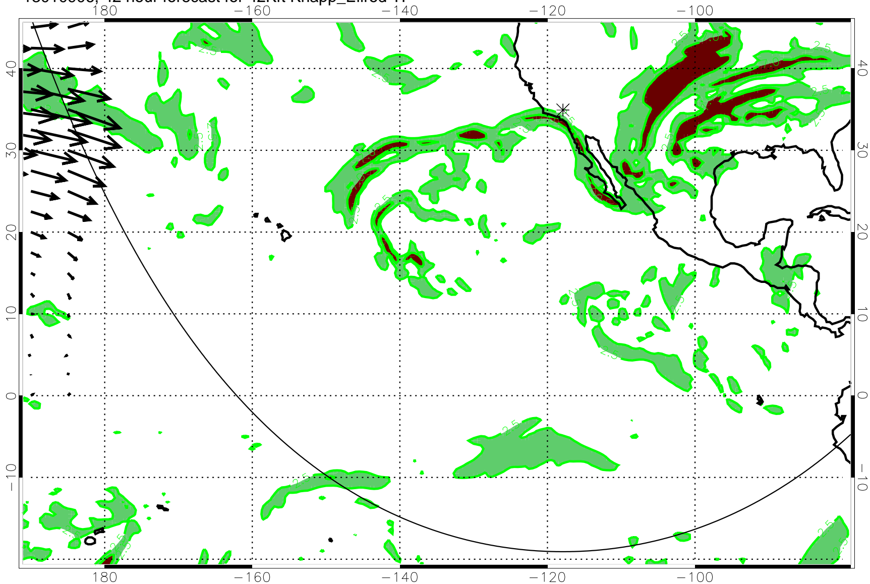
13010906, 42 hour forecast for 42Kft Knapp_Ellrod TI
