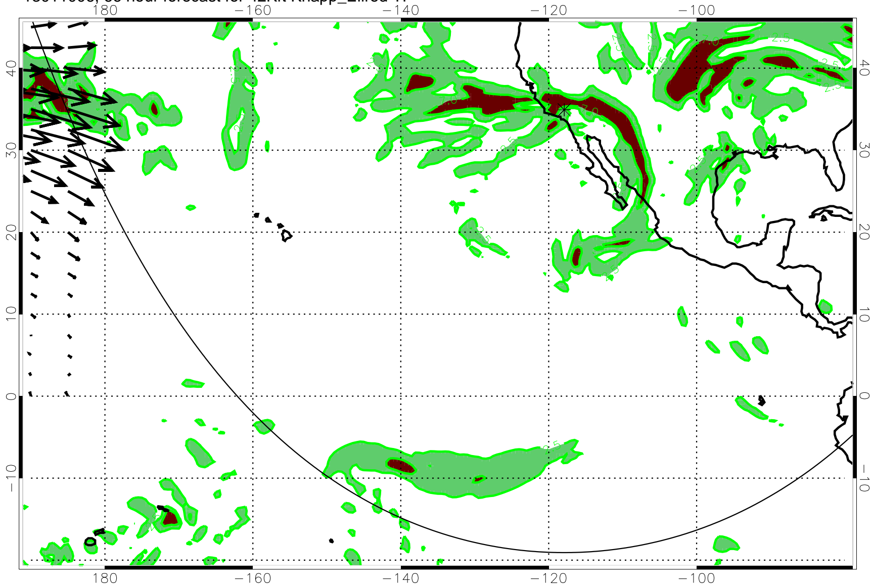
13011006, 66 hour forecast for 42Kft Knapp_Ellrod TI
