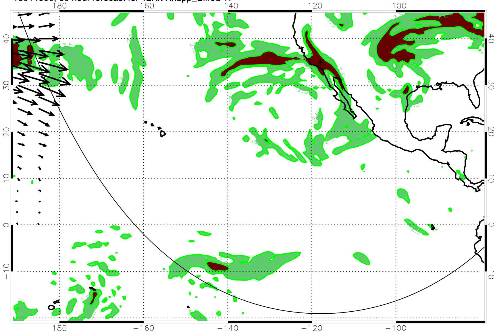
13011000, 60 hour forecast for 42Kft Knapp_Ellrod TI
