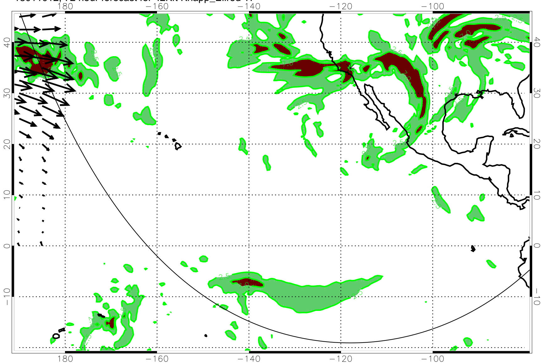
13011012, 72 hour forecast for 42Kft Knapp_Ellrod TI
