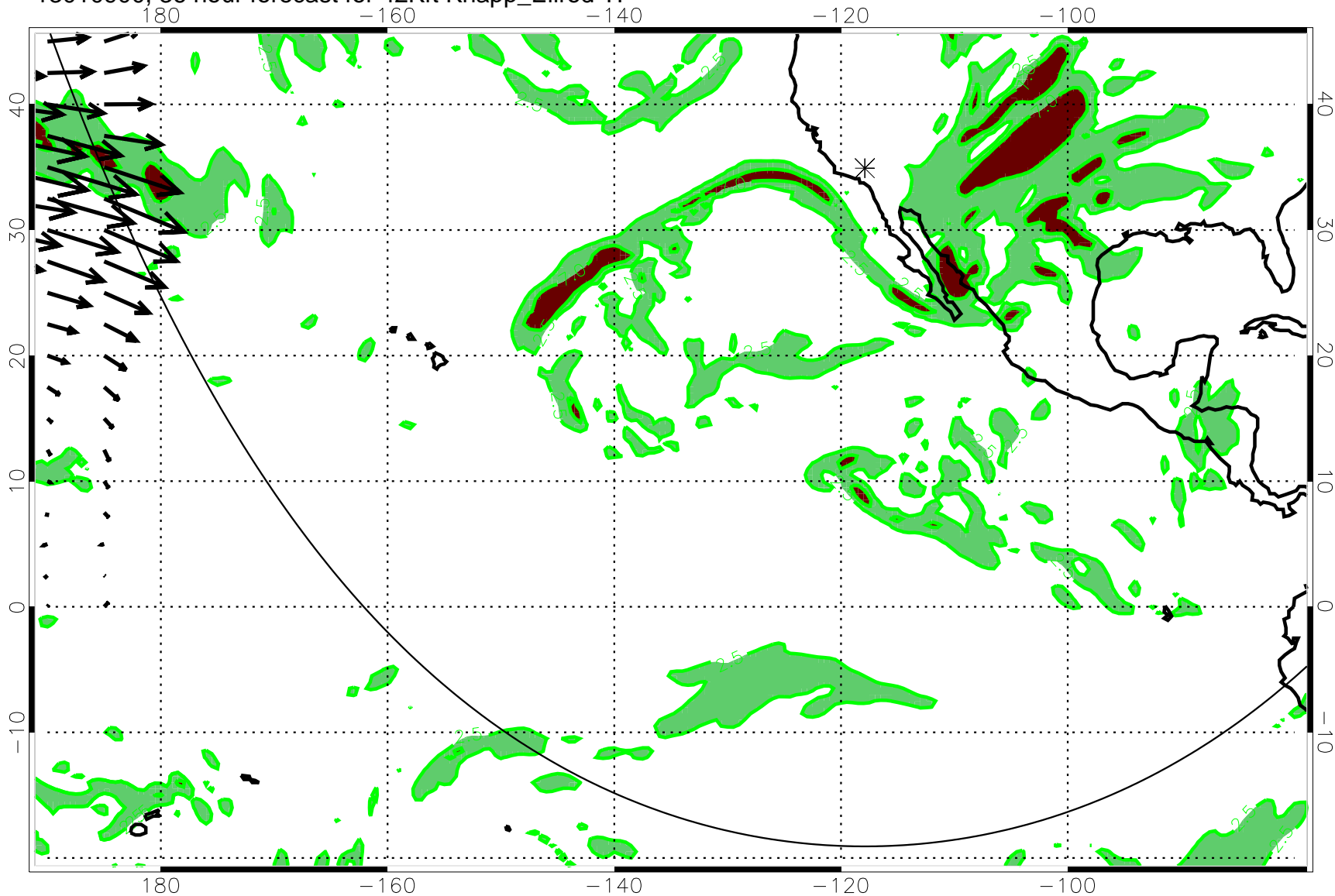
13010900, 36 hour forecast for 42Kft Knapp_Ellrod TI
