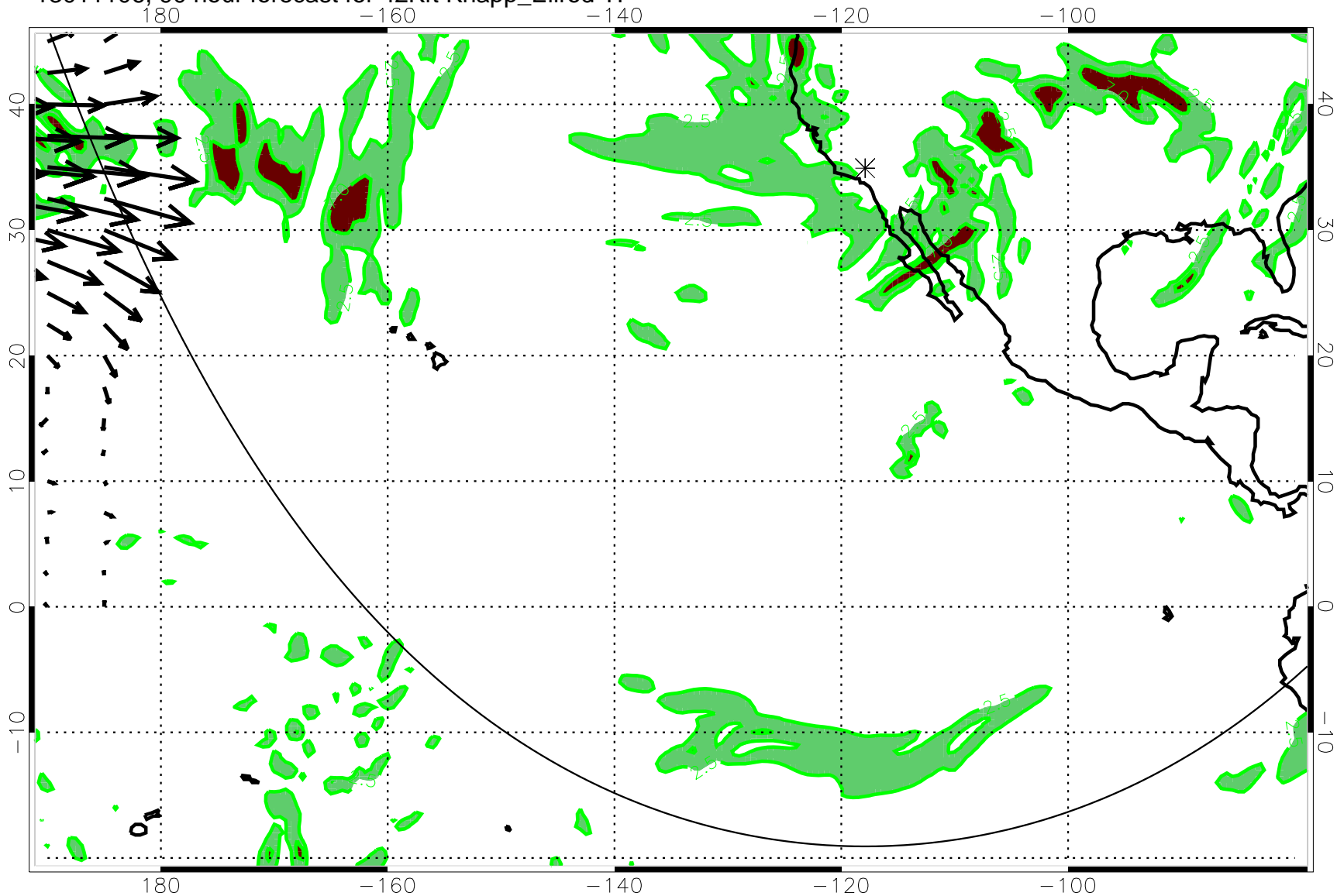
13011106, 90 hour forecast for 42Kft Knapp_Ellrod TI
