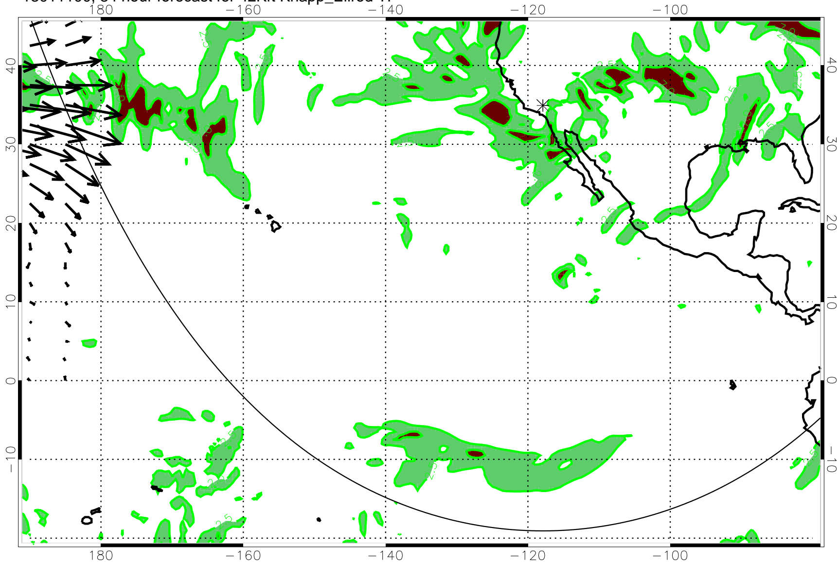
13011100, 84 hour forecast for 42Kft Knapp_Ellrod TI
