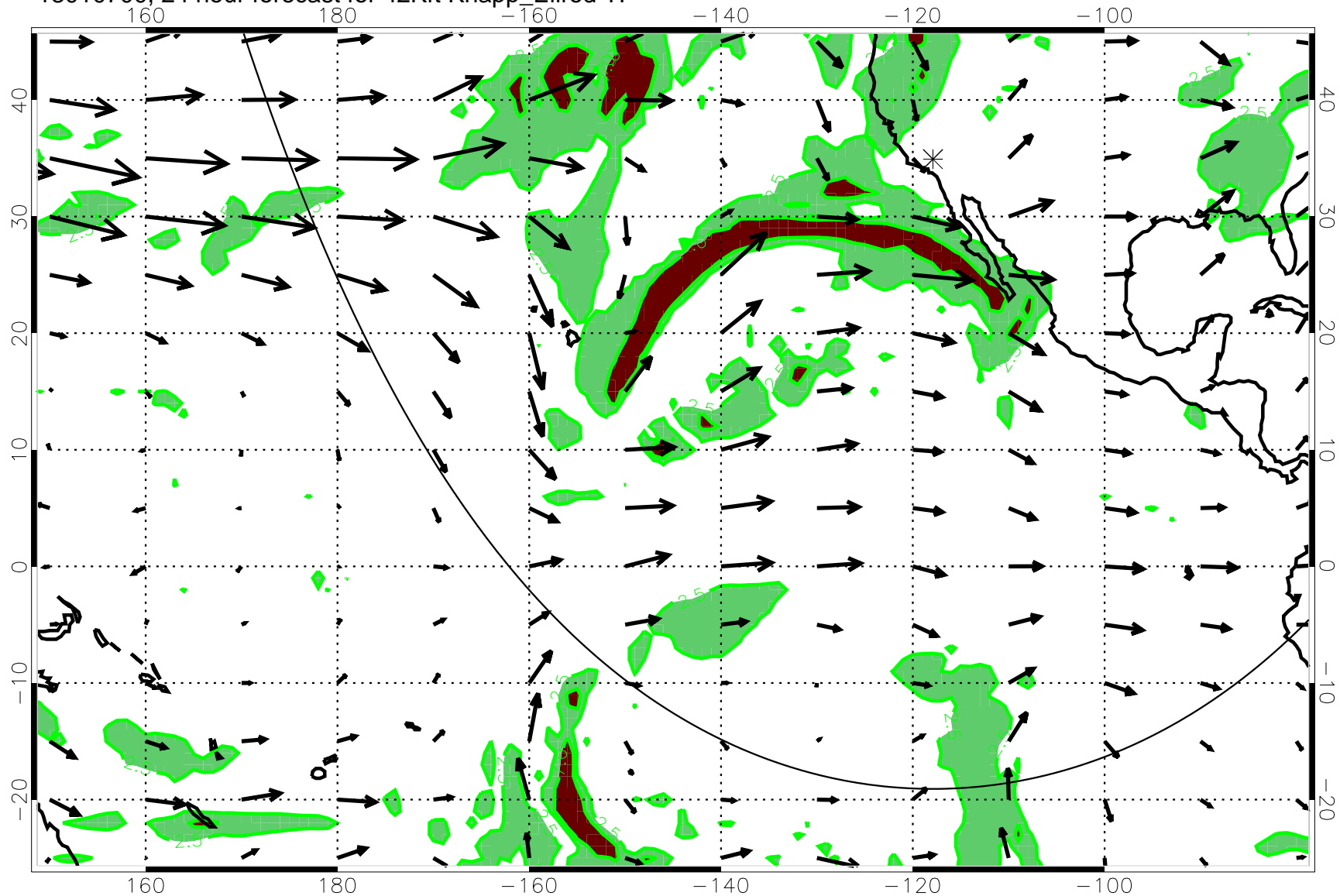
13010700, 24 hour forecast for 42Kft Knapp_Ellrod TI
