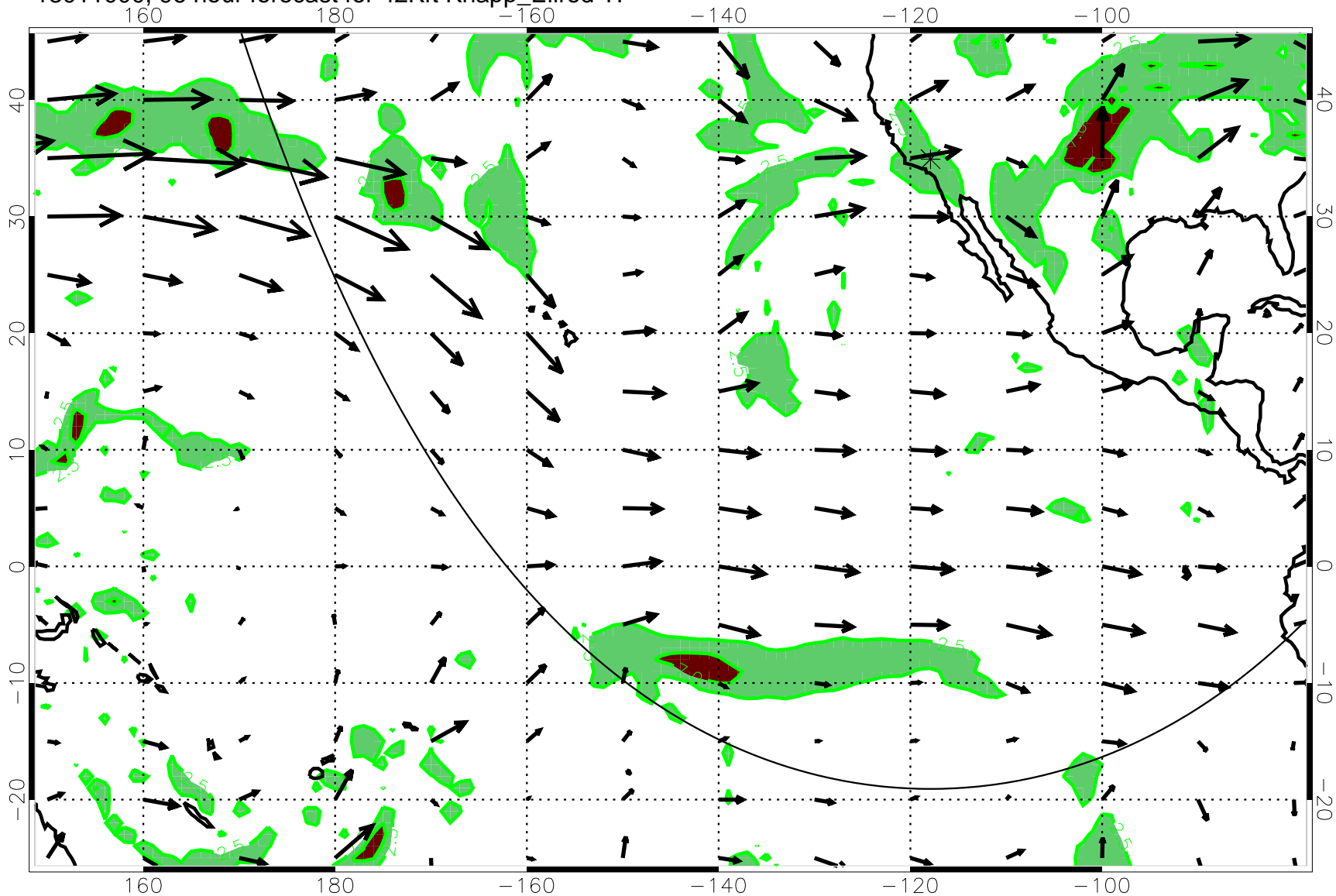
13011000, 96 hour forecast for 42Kft Knapp_Ellrod T1
