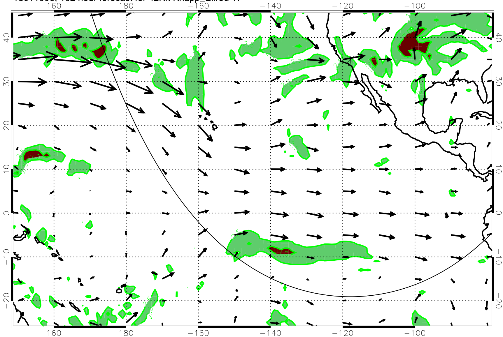
13011006, 102 hour forecast for 42Kft Knapp_Ellrod T1
