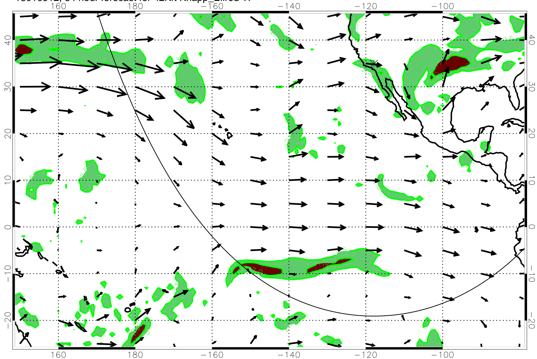
13010912, 84 hour forecast for 42Kft Knapp_Ellrod T1
