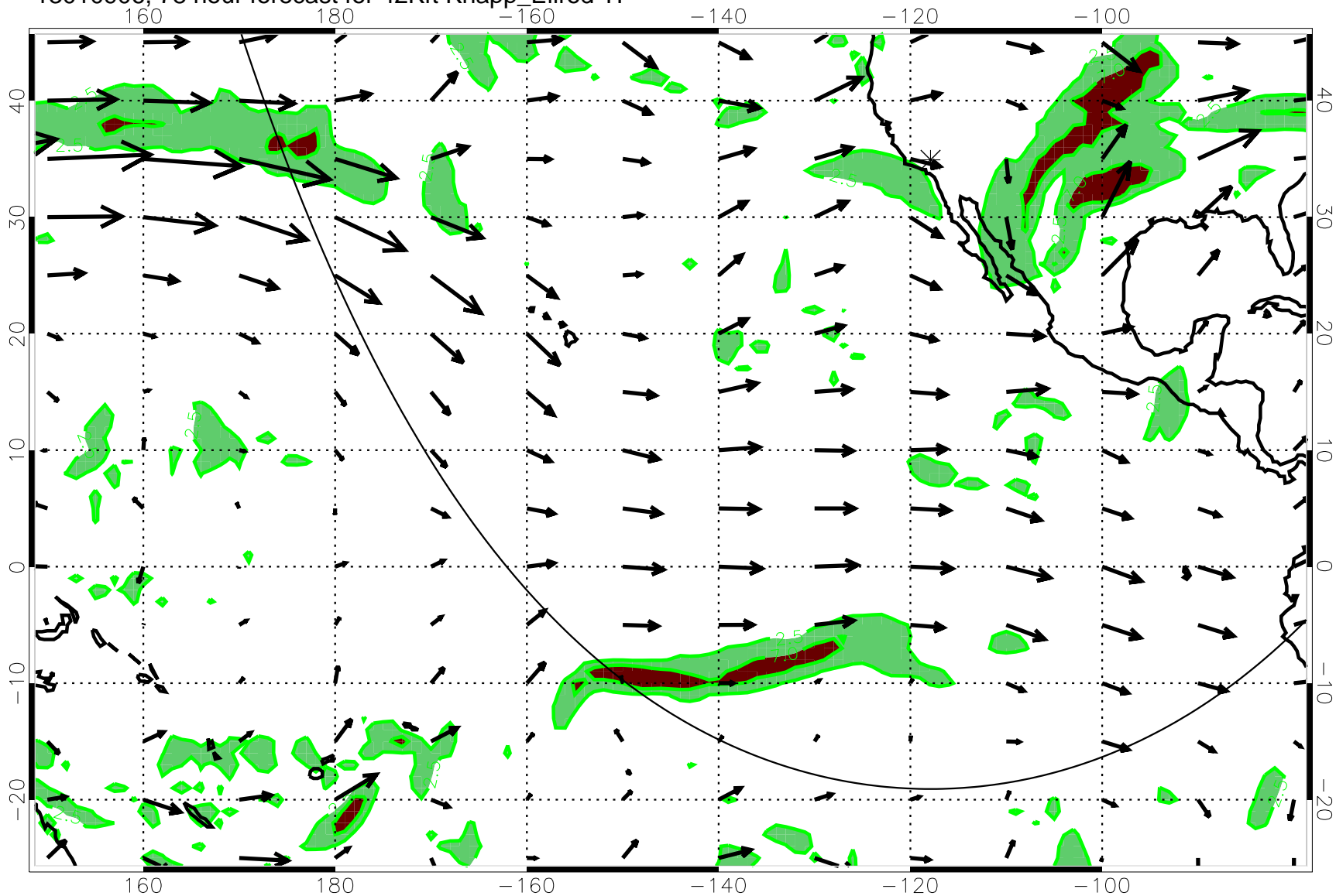
13010906, 78 hour forecast for 42Kft Knapp_Ellrod T1
