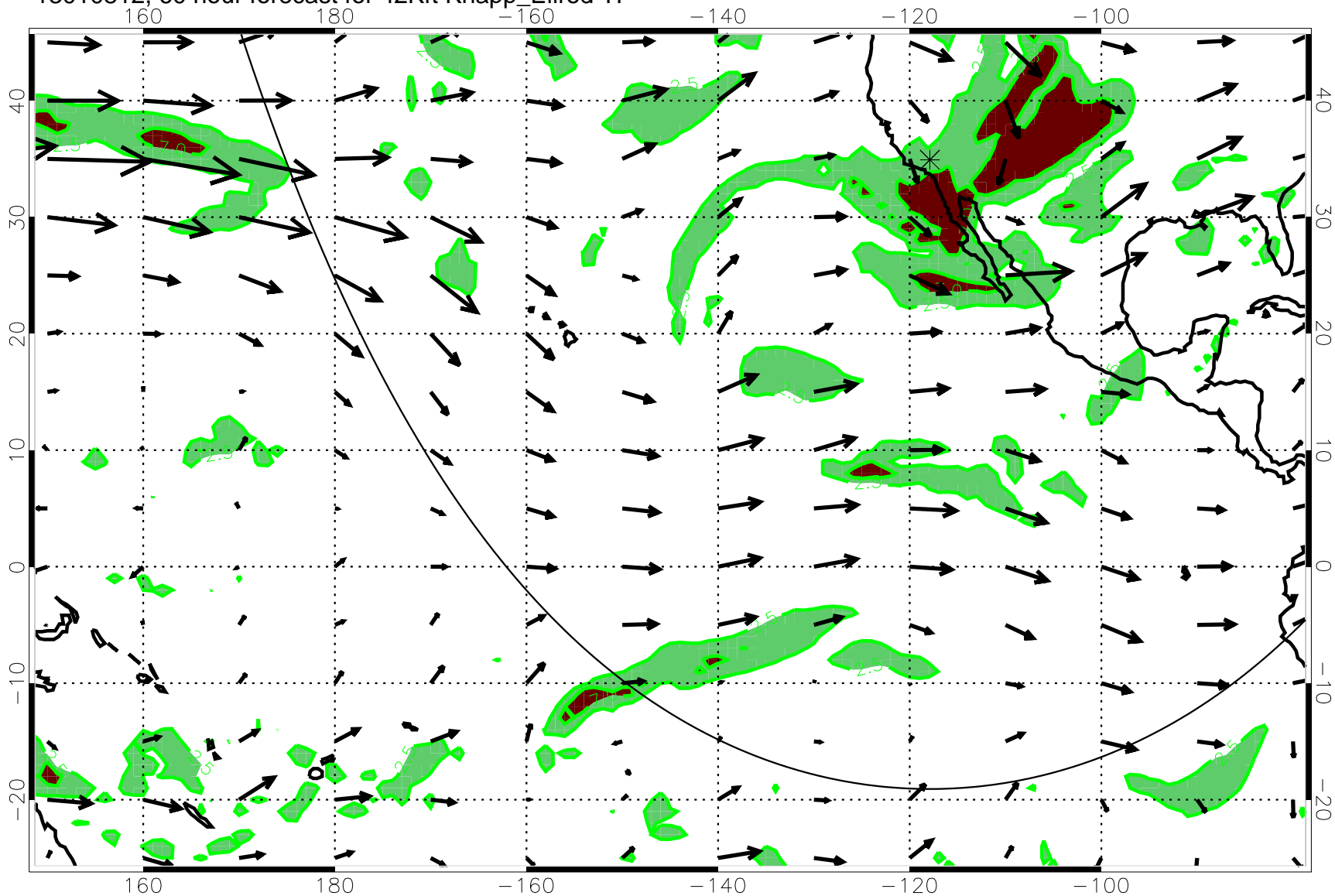
13010812, 60 hour forecast for 42Kft Knapp_Ellrod T1
