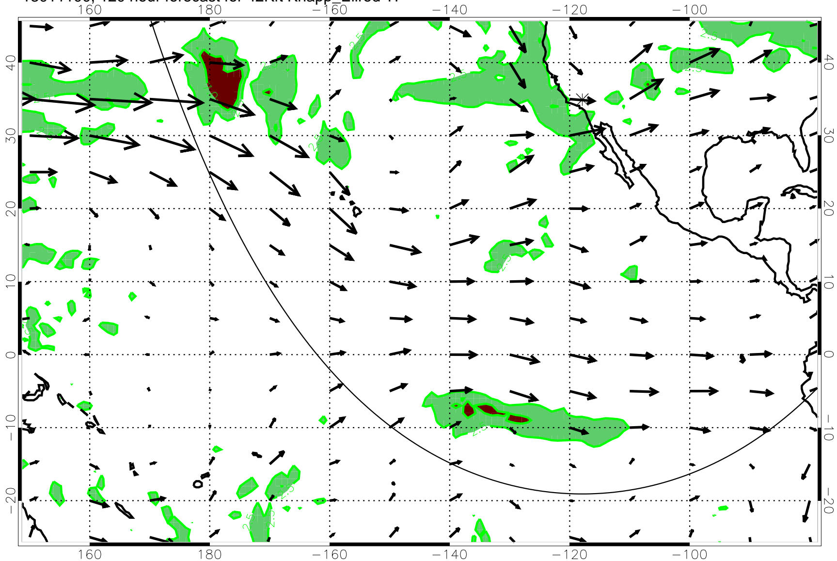
13011100, 120 hour forecast for 42Kft Knapp_Ellrod T1
