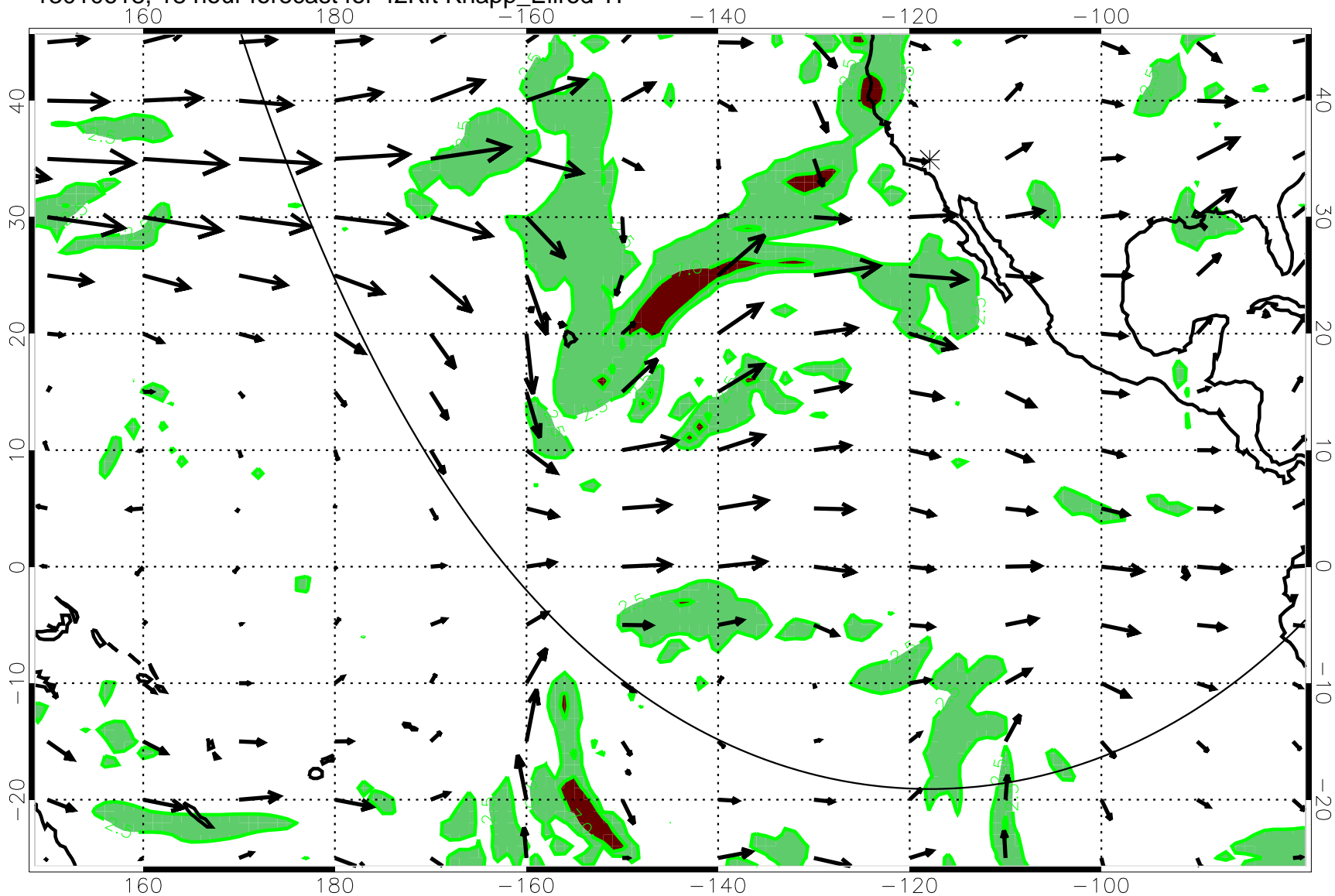
13010618, 18 hour forecast for 42Kft Knapp_Ellrod T1
