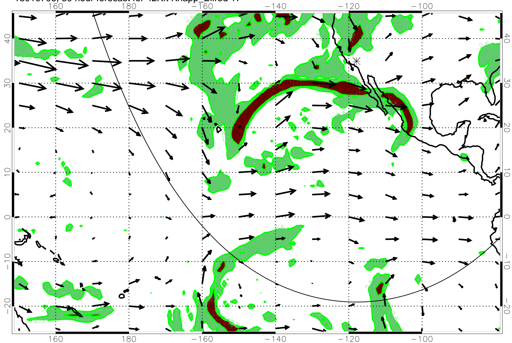
13010706, 30 hour forecast for 42Kft Knapp_Ellrod TI
