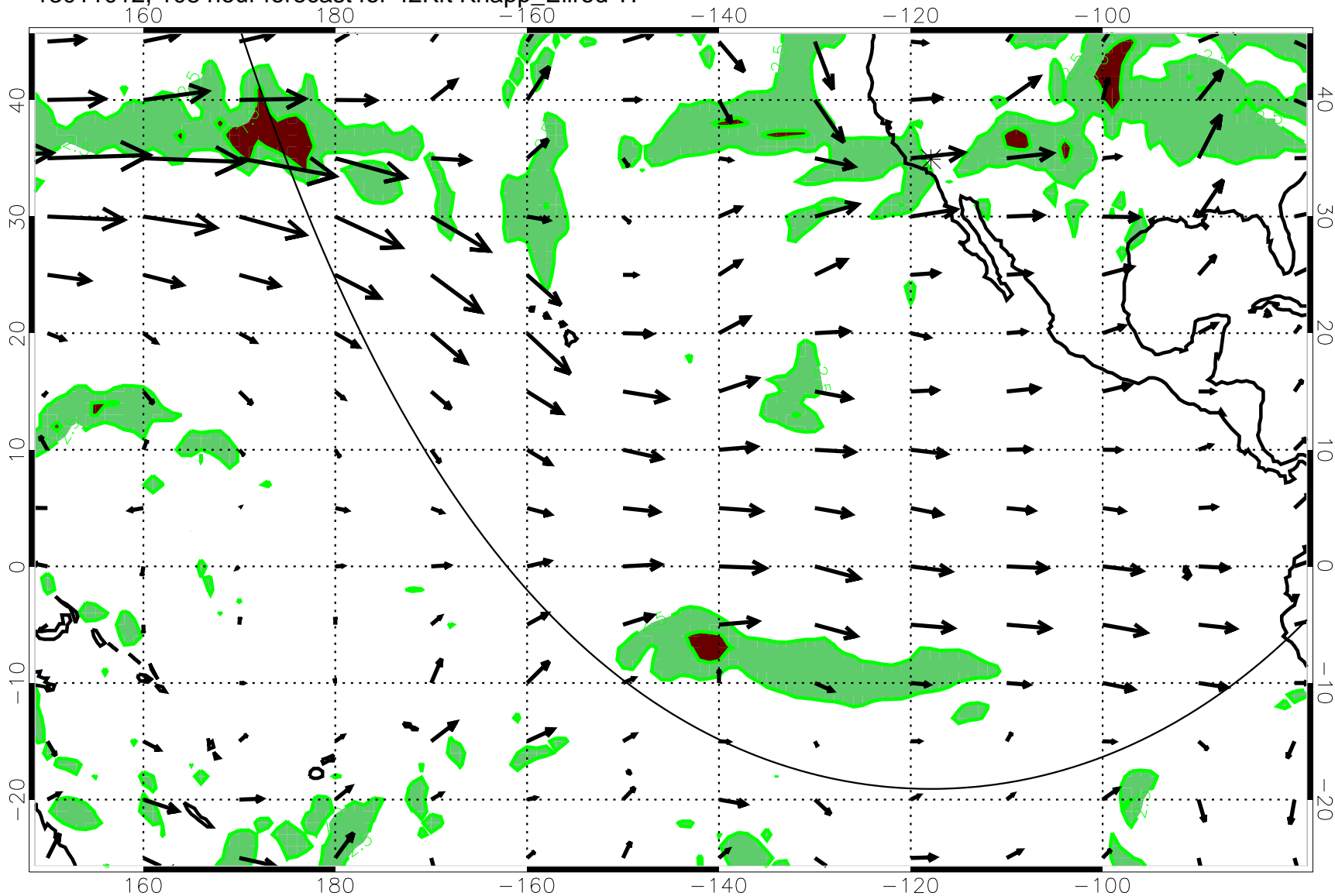
13011012, 108 hour forecast for 42Kft Knapp_Ellrod T1
