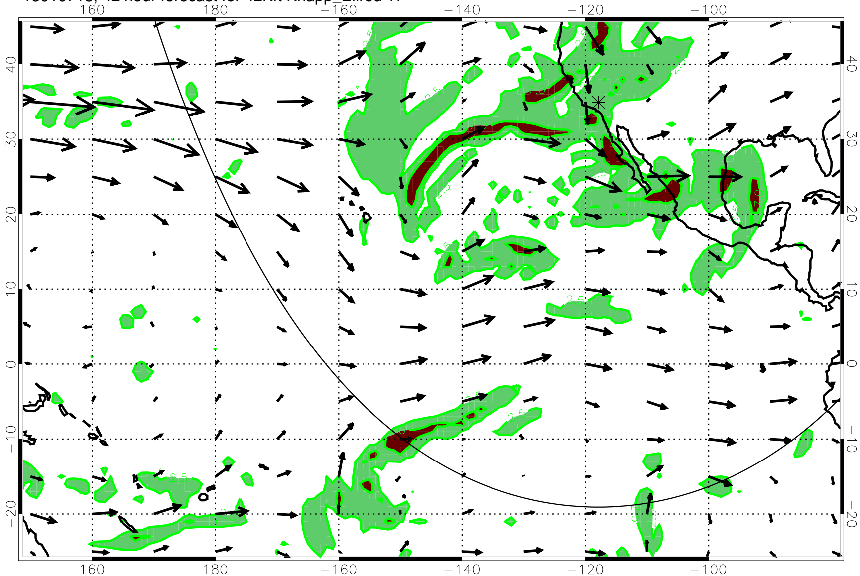
13010718, 42 hour forecast for 42Kft Knapp_Ellrod T1
