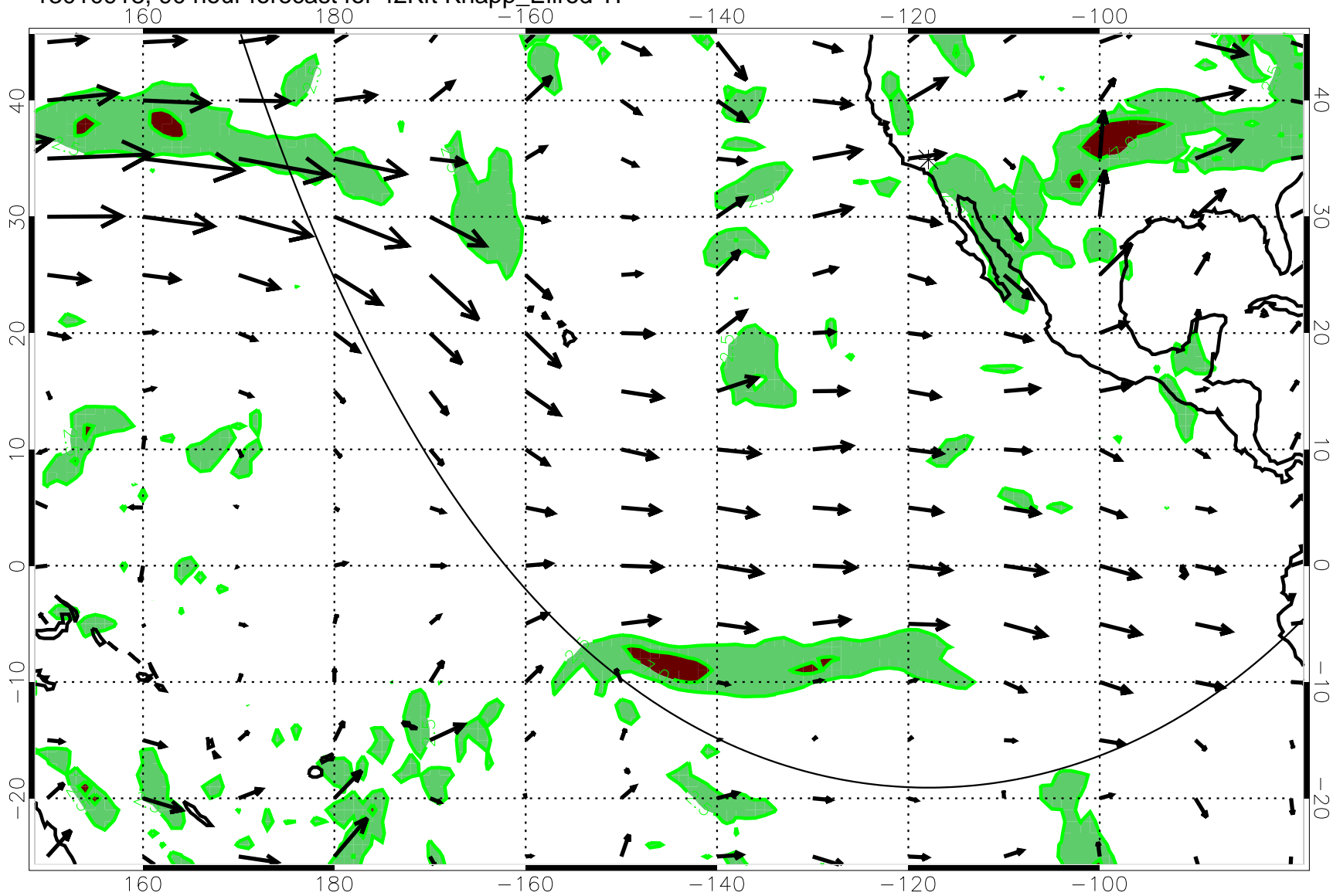
13010918, 90 hour forecast for 42Kft Knapp_Ellrod T1
