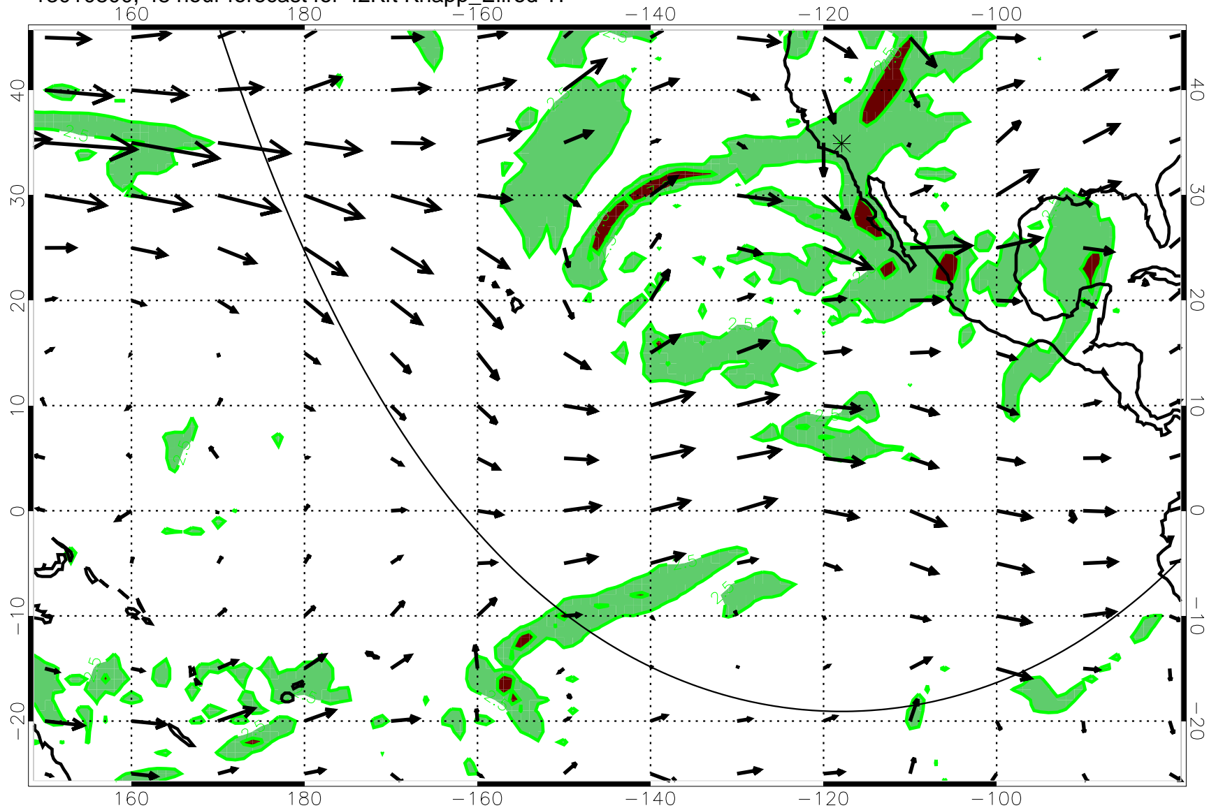
13010800, 48 hour forecast for 42Kft Knapp_Ellrod T1
