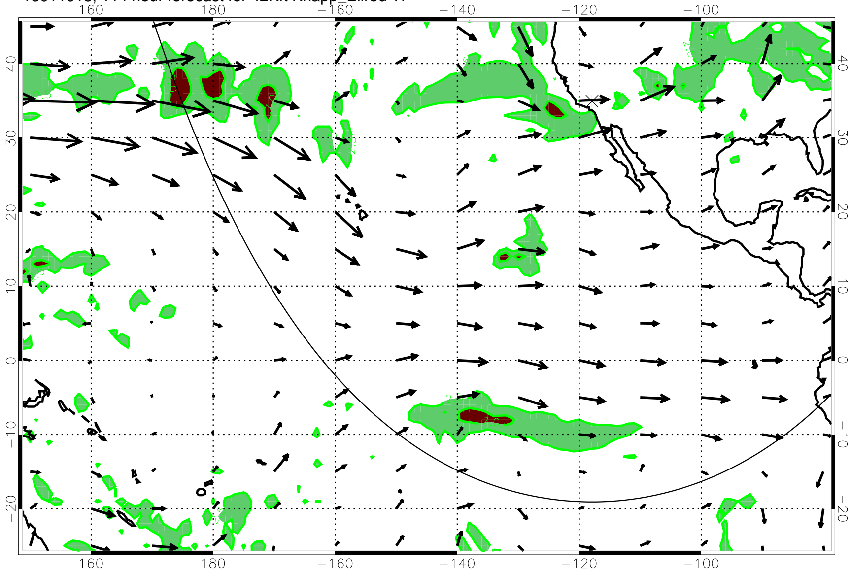
13011018, 114 hour forecast for 42Kft Knapp_Ellrod T1
