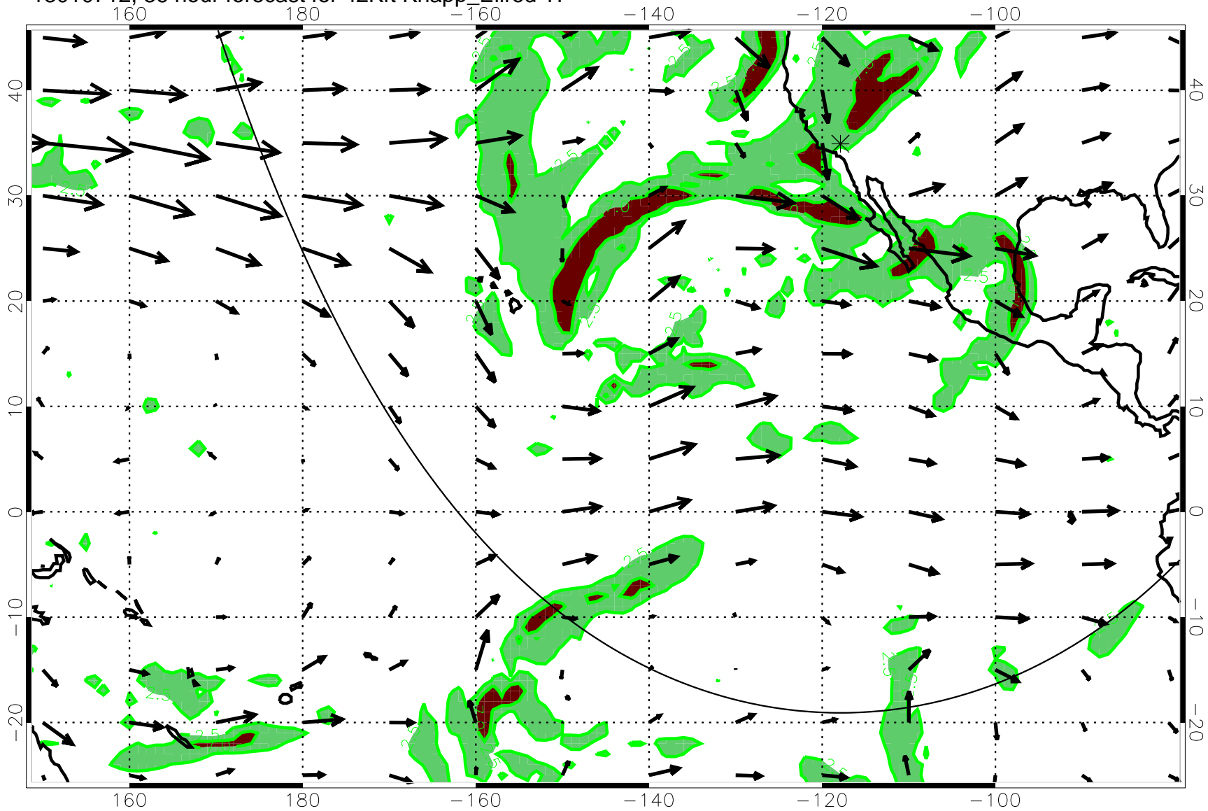
13010712, 36 hour forecast for 42Kft Knapp_Ellrod TI
