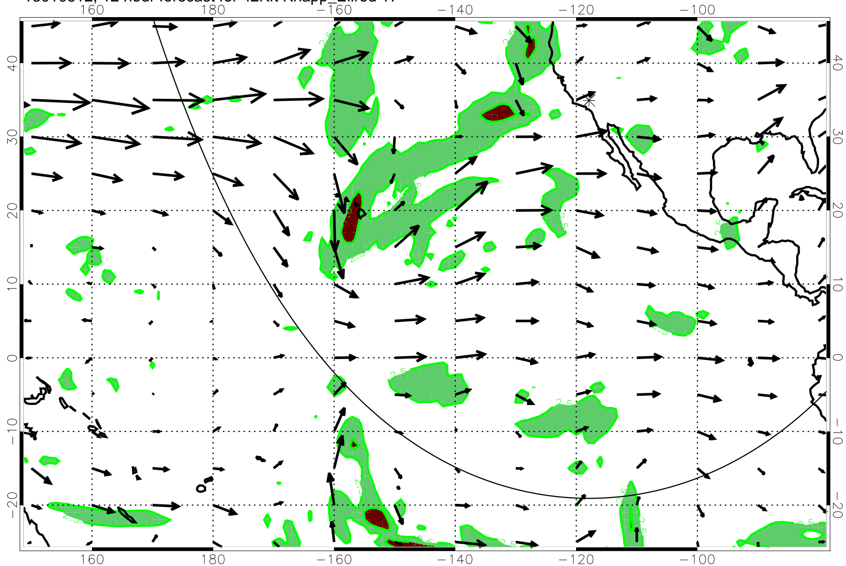
13010612, 12 hour forecast for 42Kft Knapp_Ellrod TI
