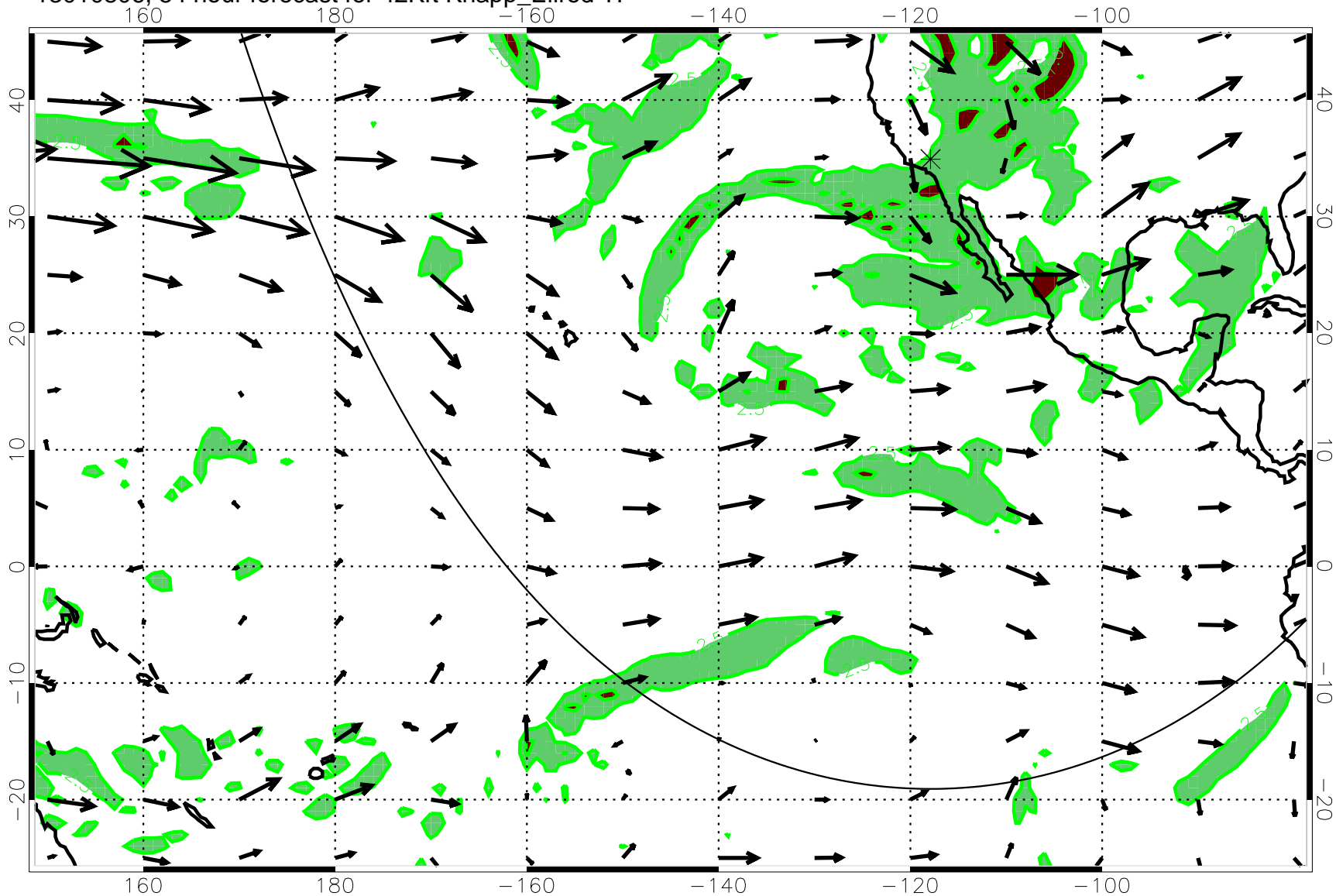
13010806, 54 hour forecast for 42Kft Knapp_Ellrod T1
