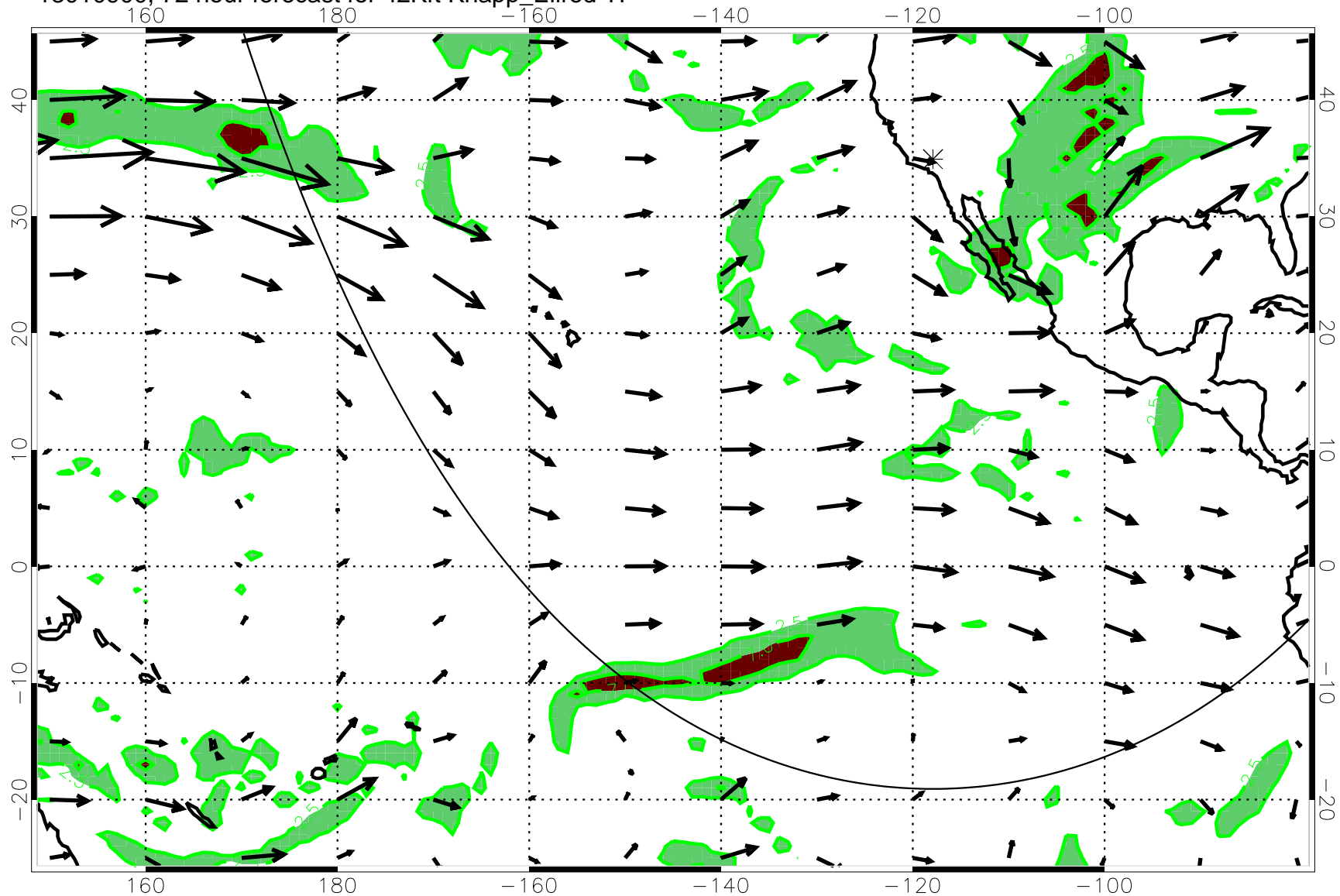
13010900, 72 hour forecast for 42Kft Knapp_Ellrod T1
