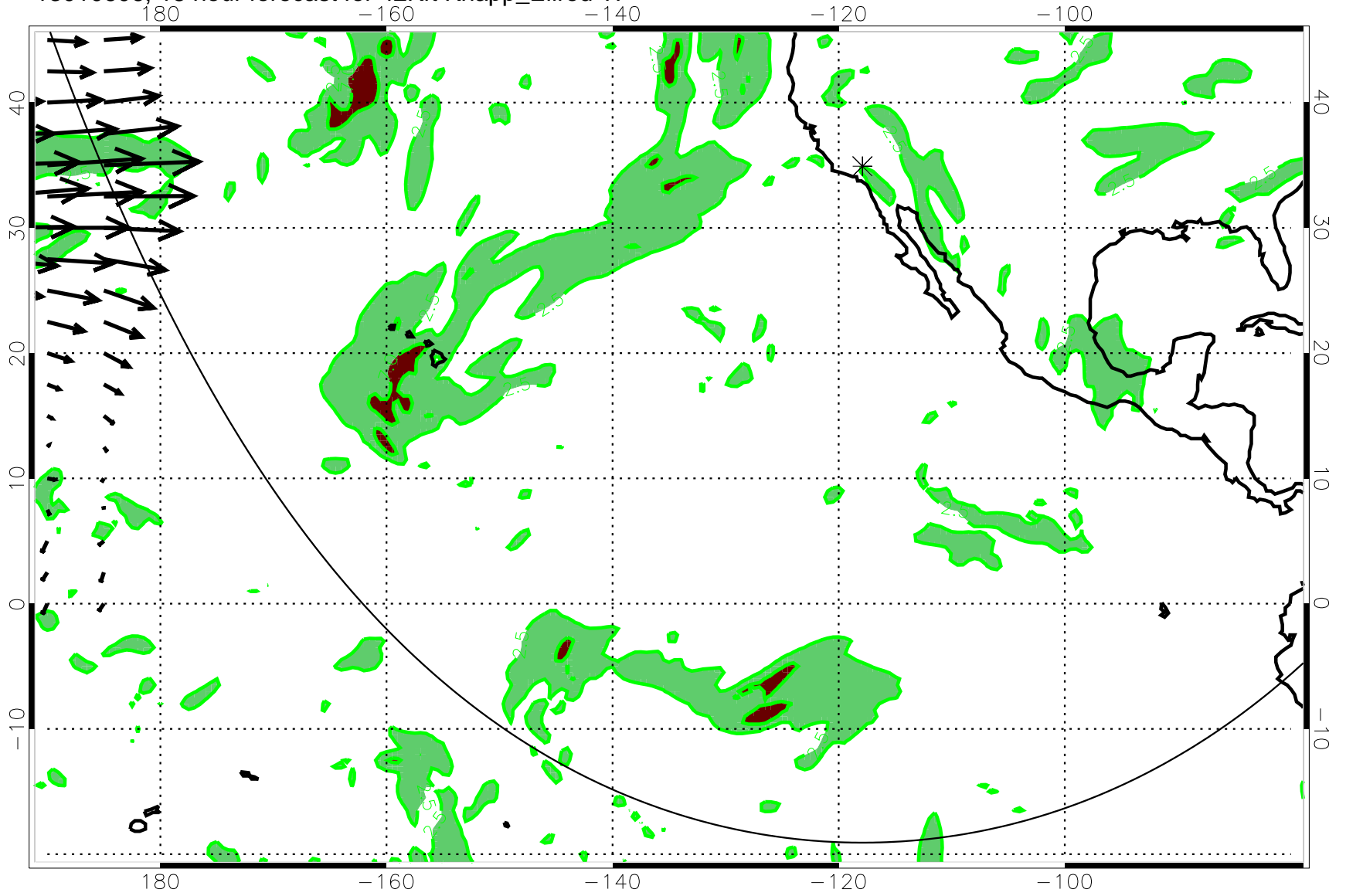
13010606, 18 hour forecast for 42Kft Knapp_Ellrod TI
