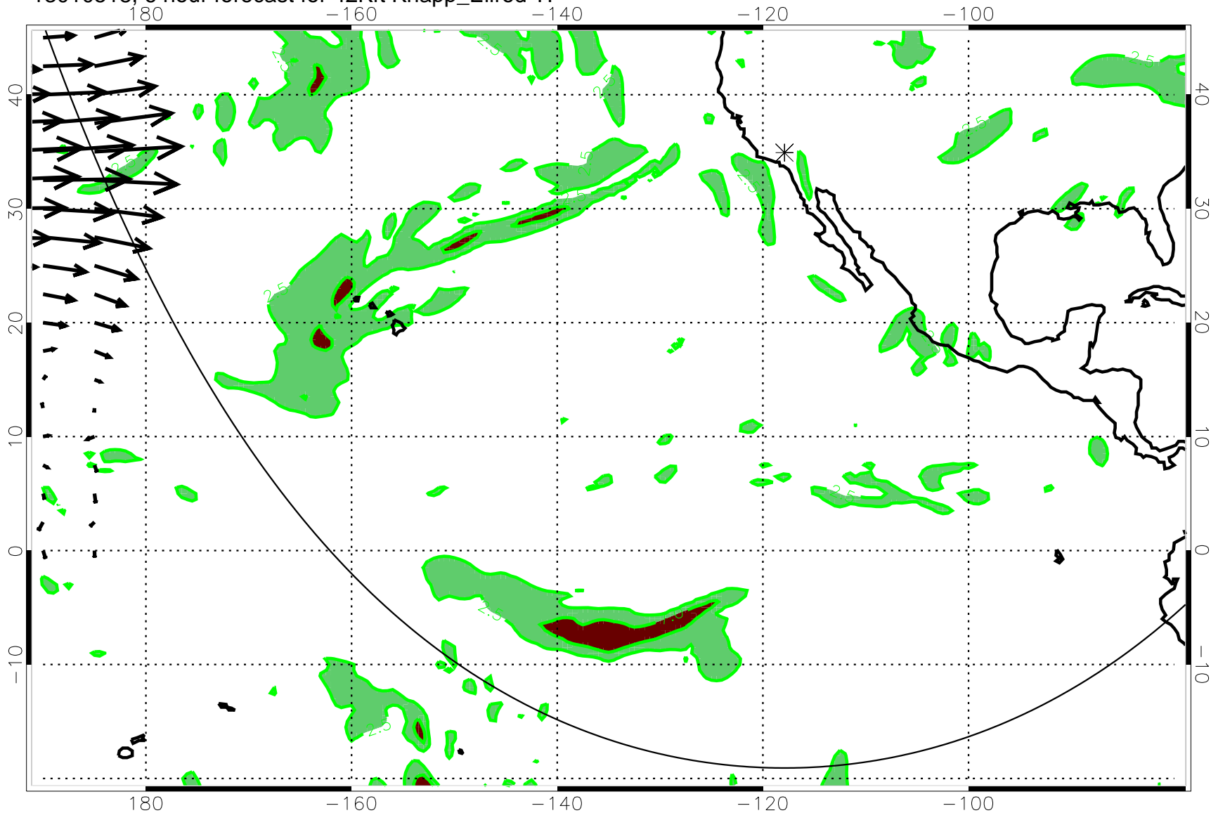
13010518, 6 hour forecast for 42Kft Knapp_Ellrod TI
