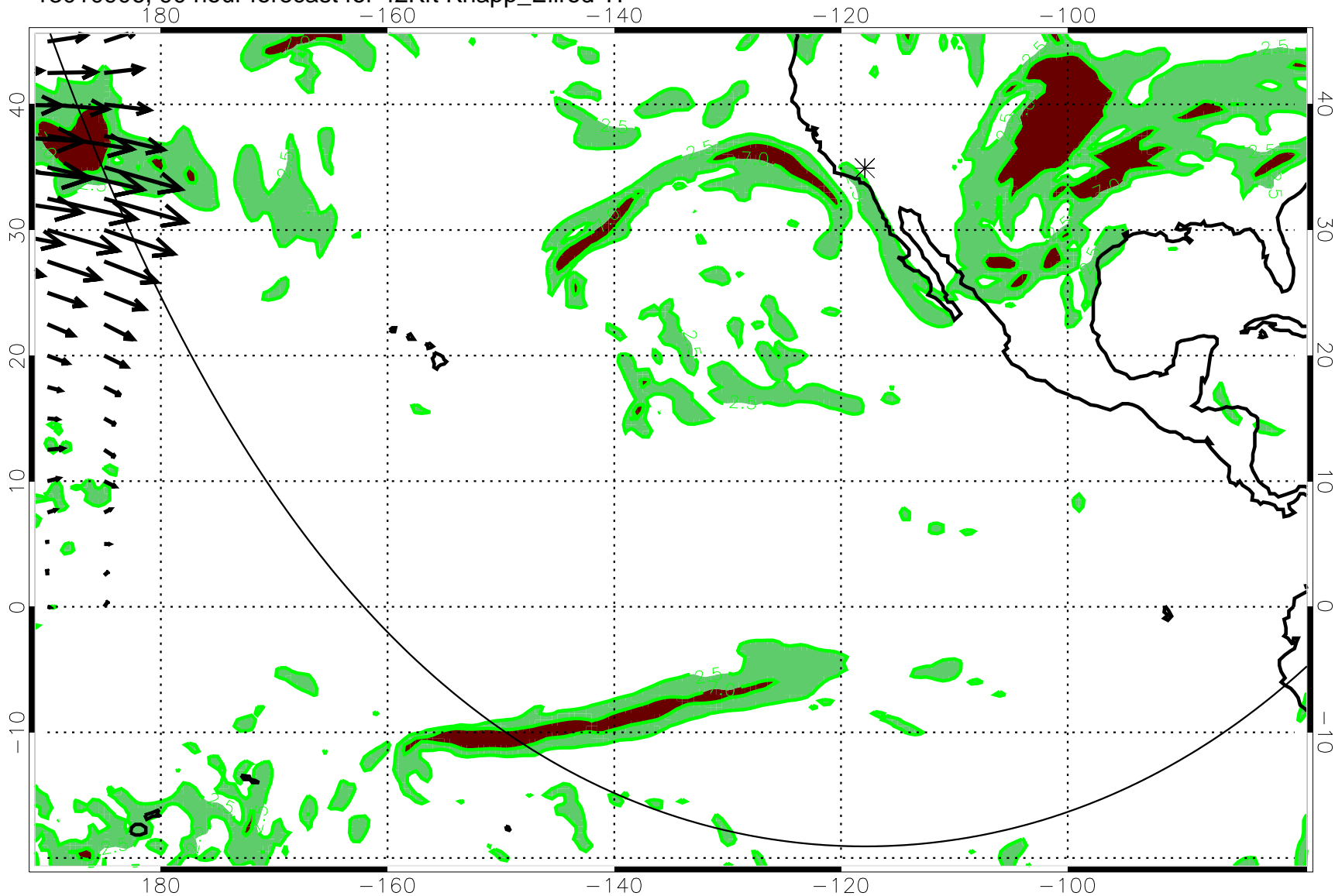
13010906, 90 hour forecast for 42Kft Knapp_Ellrod TI
