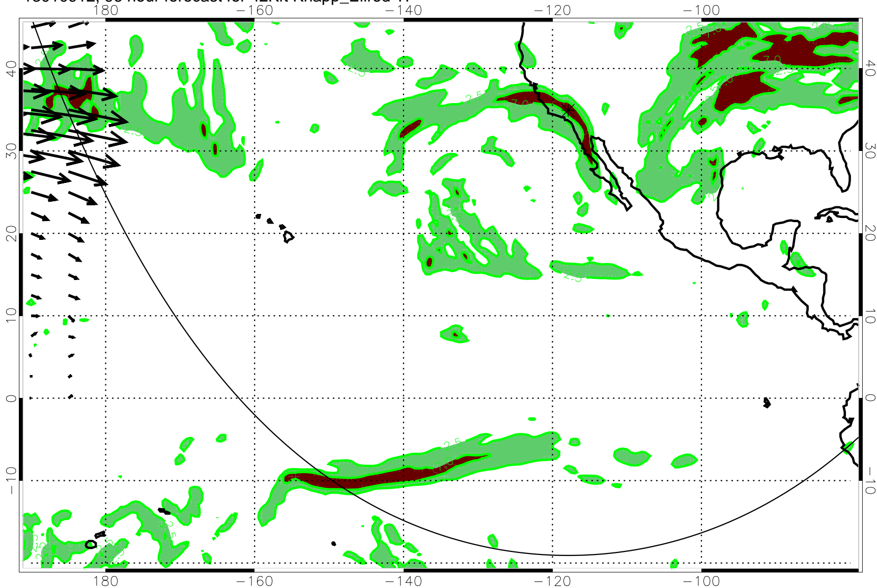
13010912, 96 hour forecast for 42Kft Knapp_Ellrod TI
