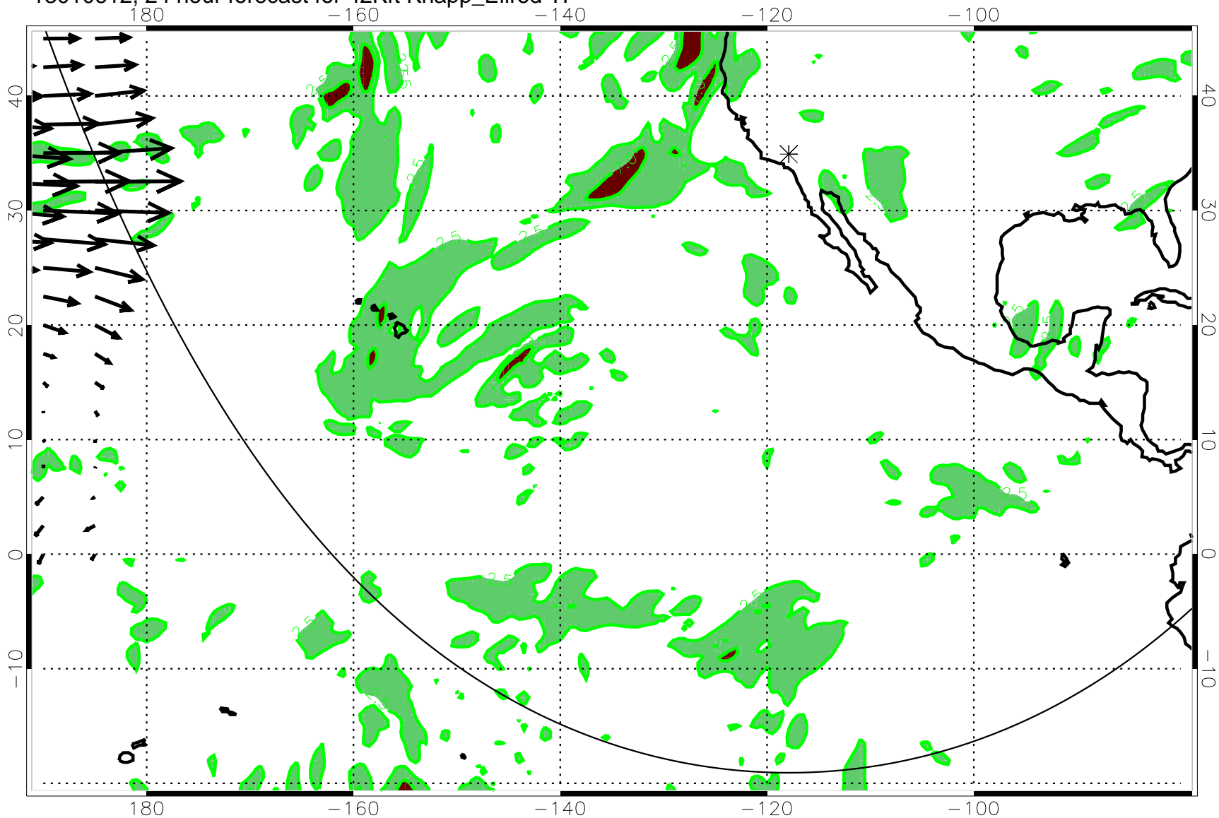
13010612, 24 hour forecast for 42Kft Knapp_Ellrod TI
