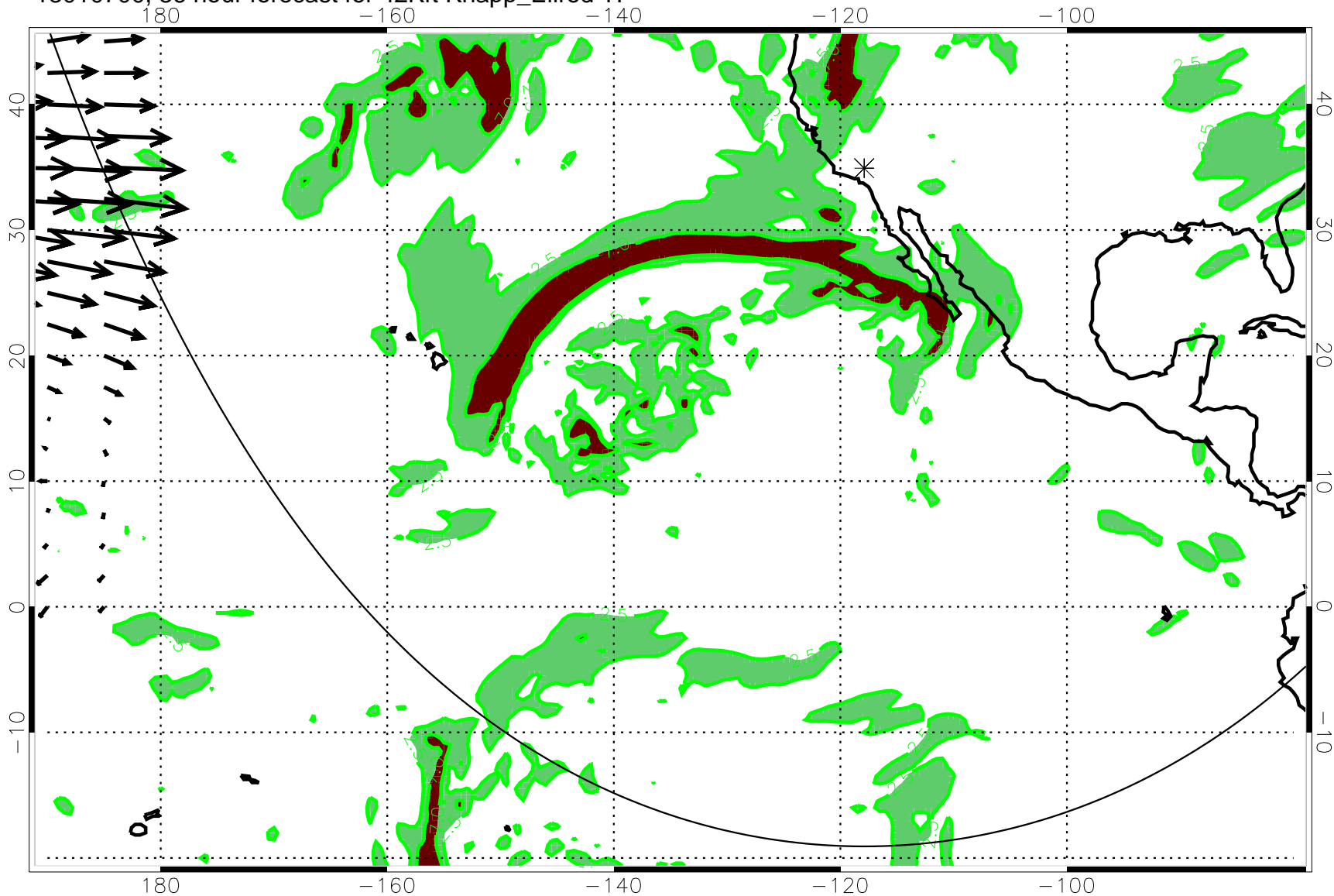
13010700, 36 hour forecast for 42Kft Knapp_Ellrod TI
