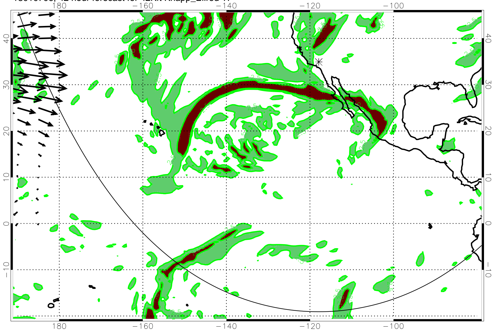
13010706, 42 hour forecast for 42Kft Knapp_Ellrod TI
