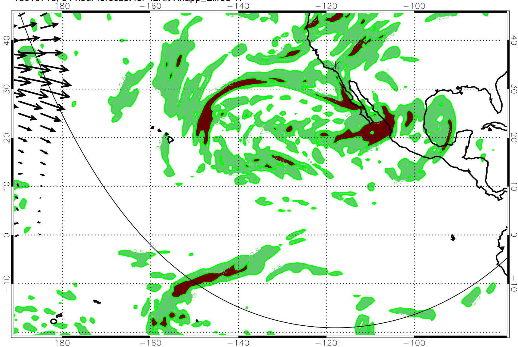
13010718, 54 hour forecast for 42Kft Knapp_Ellrod TI
