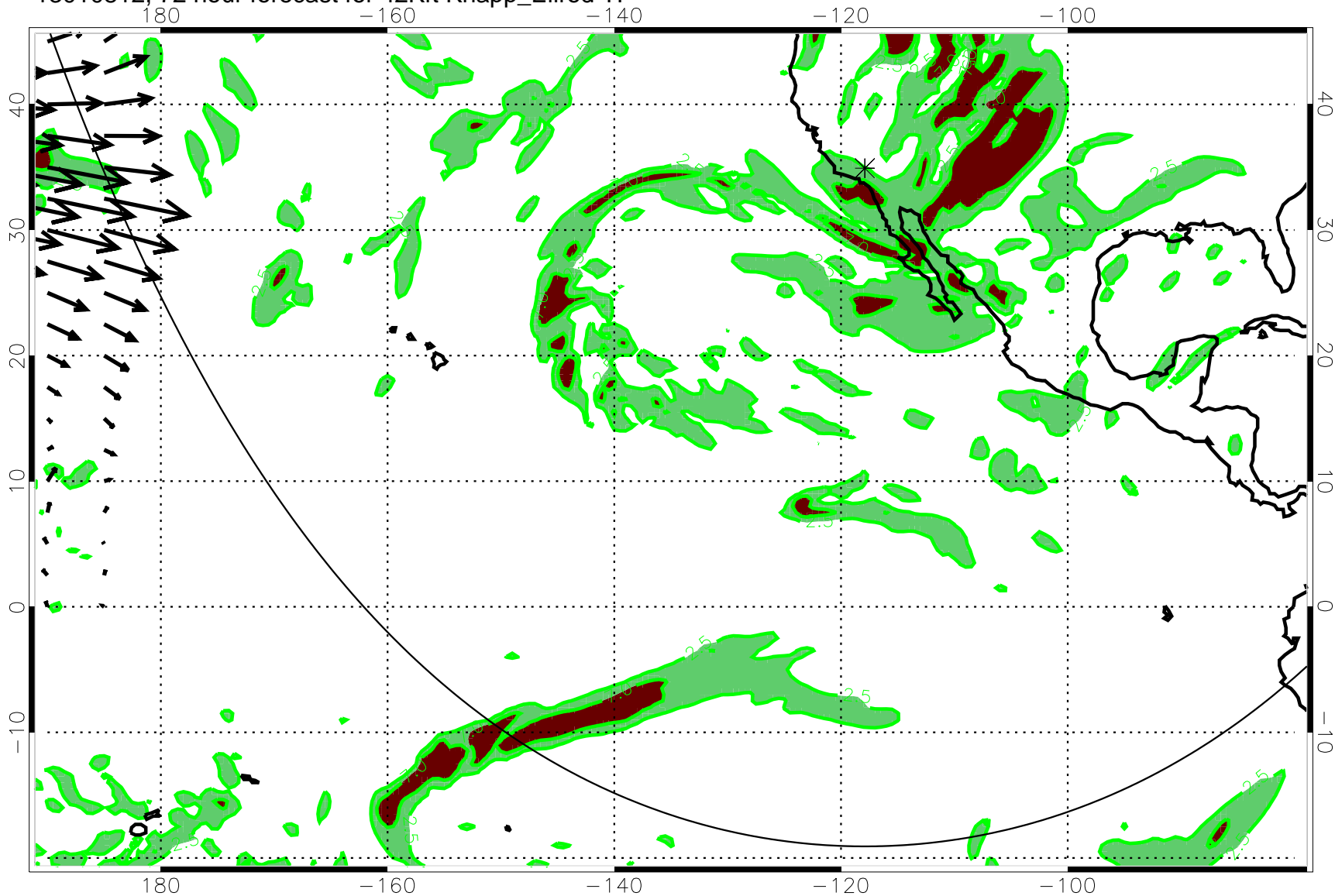
13010812, 72 hour forecast for 42Kft Knapp_Ellrod TI
